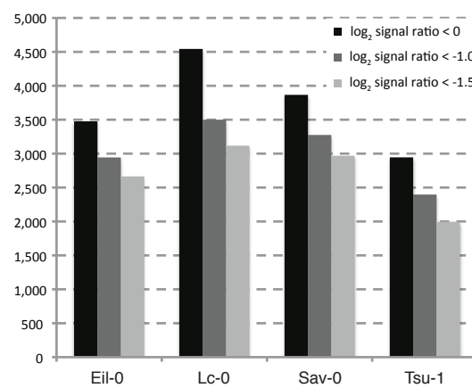
Supplemental Figure 2 Number of unique tiles from the Col-0 genome without UHTS coverage in the four accessions that have a tiling array signal ratio < 0, < -1.0, or < -1.5. Only tiles located within transcript regions were considered.
