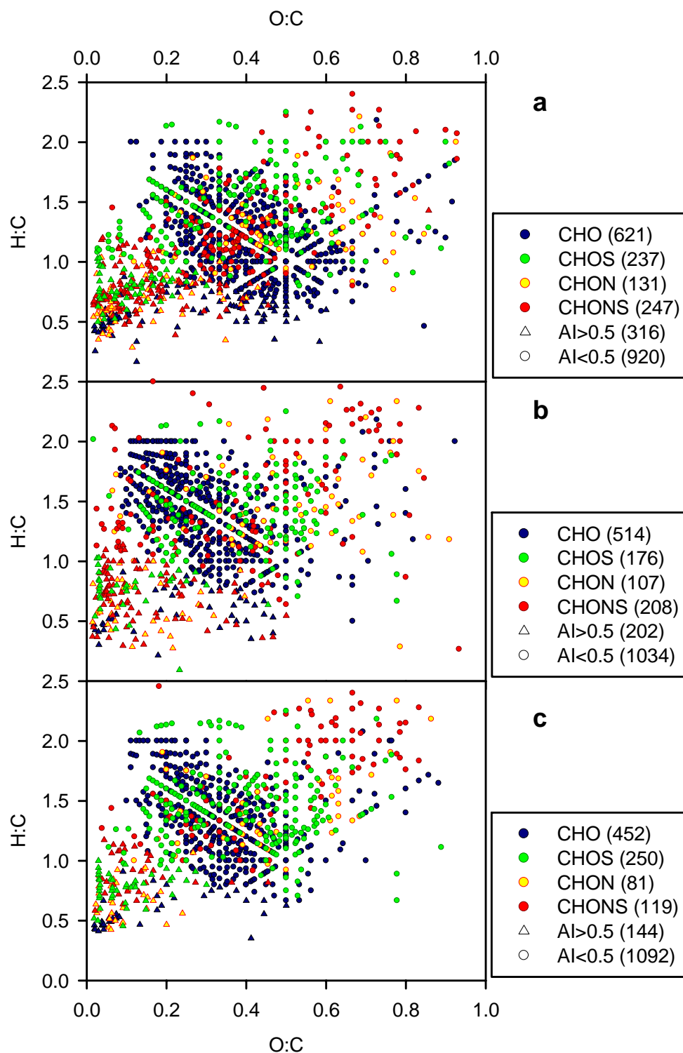
Figure S2. Van Krevelen diagrams of CHONS molecular compositions. (a) inflow DOC pool, (b) residual DOC pool in control flume without bedforms, (c) residual DOC pool in flume with highest bedforms (10cm). Colours indicate elemental composition, symbol type indicates presence of aromatic structures (aromaticity index > 0.5), values in parentheses indicate number of compounds identified.
