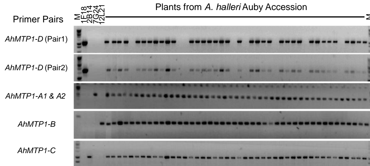
Figure S1; Analysis of the presence of the AhMTP1 paralogues in 44 plants from the Auby accession using gene copy specific primer pairs. Each of the horizontal panel show the amplification obtained from a primer pair specific to the MTP1 paralogue named at the left of the panel. Samples from BAC clones 1F18, 2B14, 7G24 and 12L21 were used as controls for specificity of the primer pairs. The lane M represents 1kb invitrogen DNA ladder.
