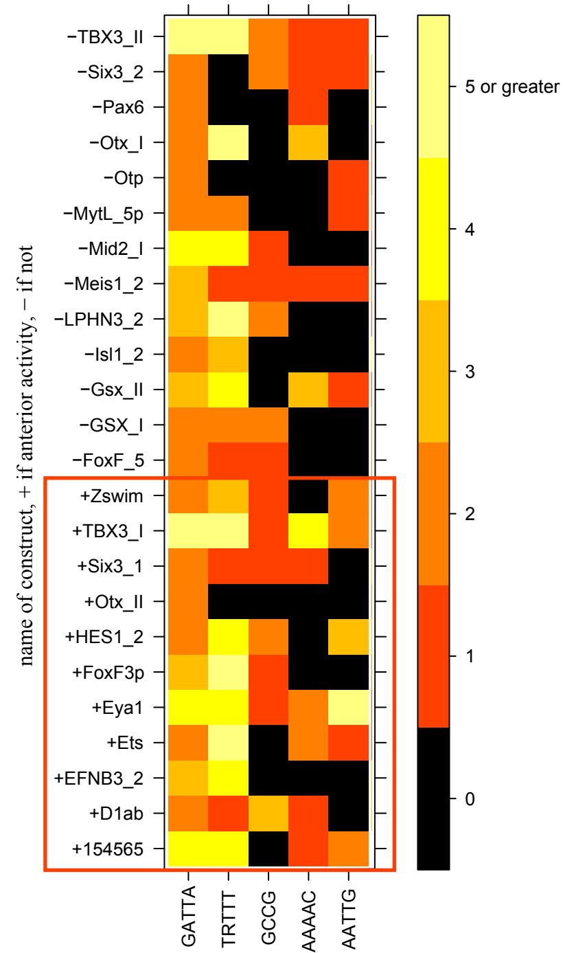
Figure S4 Motif occurrences in predicted enhancers.
