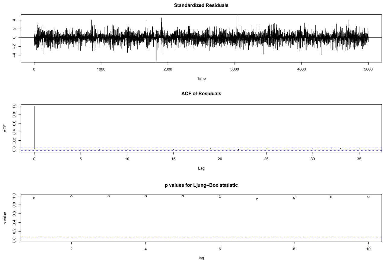
Figure 3: Diagnostic plots for AR( \gamma ) model fitted to the data in Krig et al. (2007).
