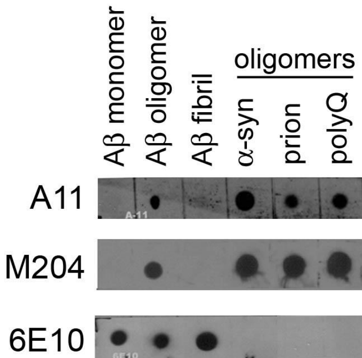
Supplementary Figure S1. Polyclonal A11 antibody and monoclonal M204 antibody recognize oligomers but not monomers or fibrils. Similar quantities of proteins or peptides (40 nmol) were spotted onto nitrocellulose membrane and incubated with the respective antibodies. Signals were detected by enhanced chemiluminescence (ECL).
