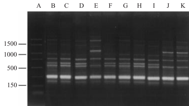
Fig. 1. RAPD fingerprints obtained for the Ph. damselae subsp. piscicida isolates employing the primer 4. Lanes: A, AmpliSize™ Molecular Ruler (50–2000 bp ladder; BioRad); B, DI 21; C, IT-1; D, B3; E, ATCC 29690; F, Pp 5; G, 666-1; H, 10831; I, 069A; J, MZS-8001; K, EPOY-8803-II. The molecular sizes (in kb) are indicated on the left.
