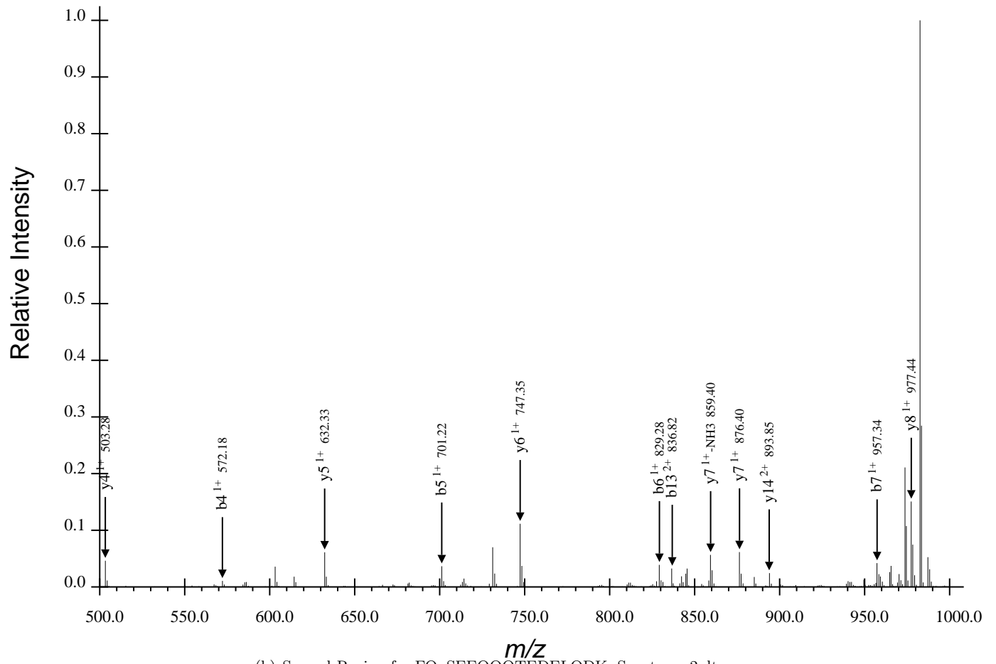
(b) Second Region for FQpSEEQQQTEDELQDK, Spectrum 2.dta
