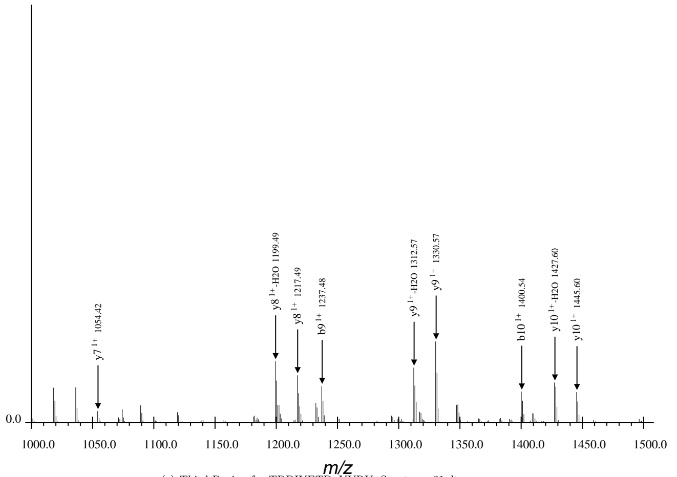
(c) Third Region for TRDIYETDpYYRK, Spectrum 31.dta
