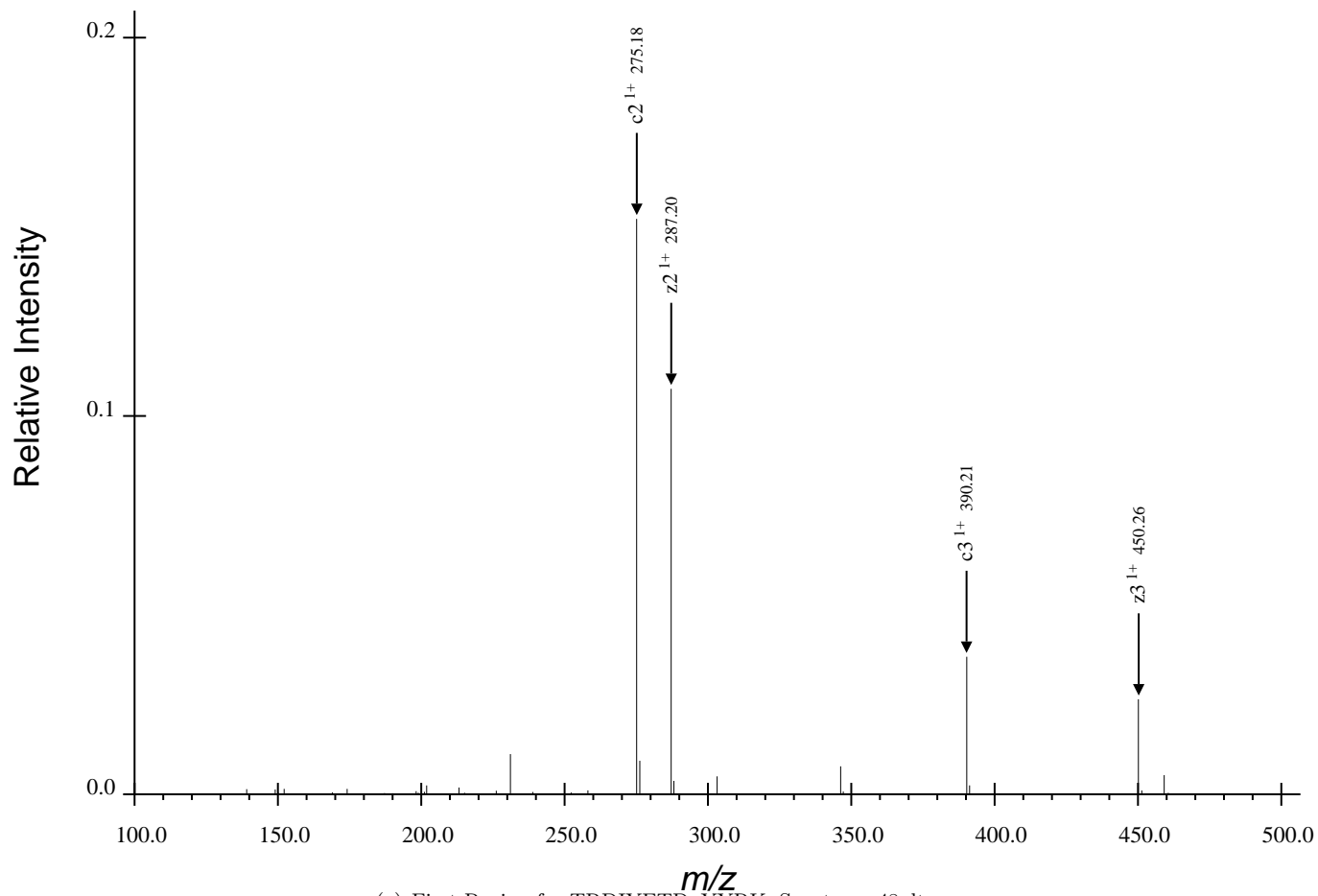
(a) First Region for TRDIYETDpYYRK, Spectrum 48.dta
