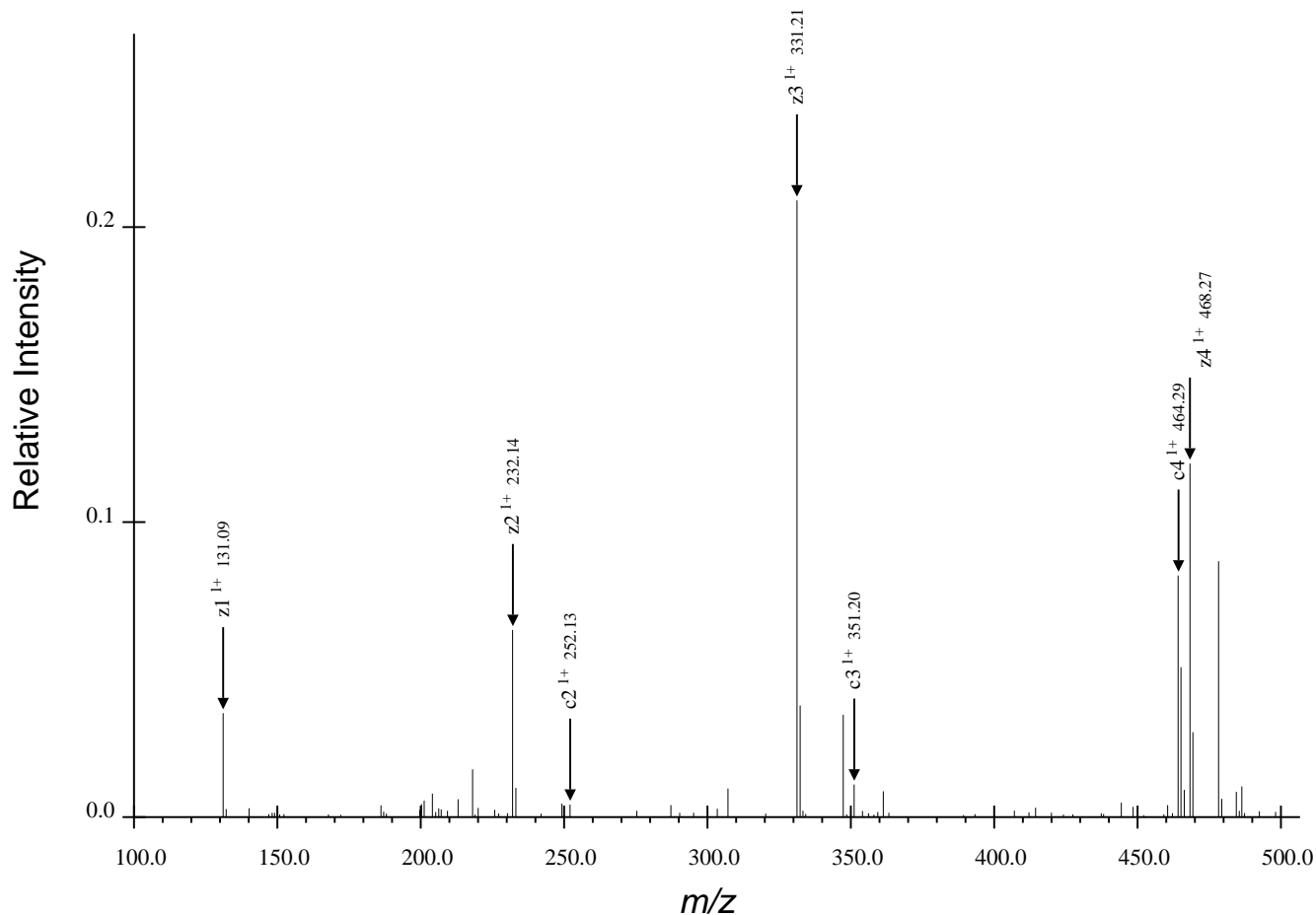
(a) First Region for SFVLNPTNIGMpSKSSQGHVTK, Spectrum 28.dta
