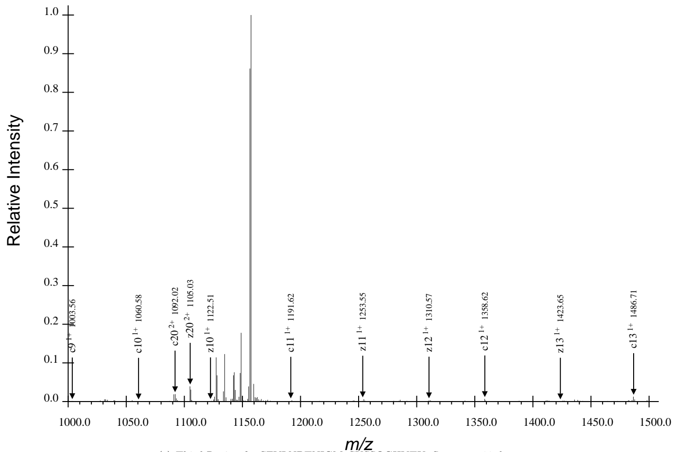
(c) Third Region for SFVLNPTNIGMpSKSSQGHVTK, Spectrum 23.dta
