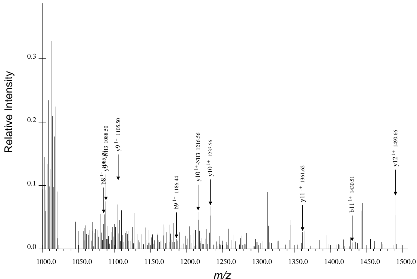
(c) Third Region for FQpSEEQQQTEDELQDK, Spectrum 6.dta
