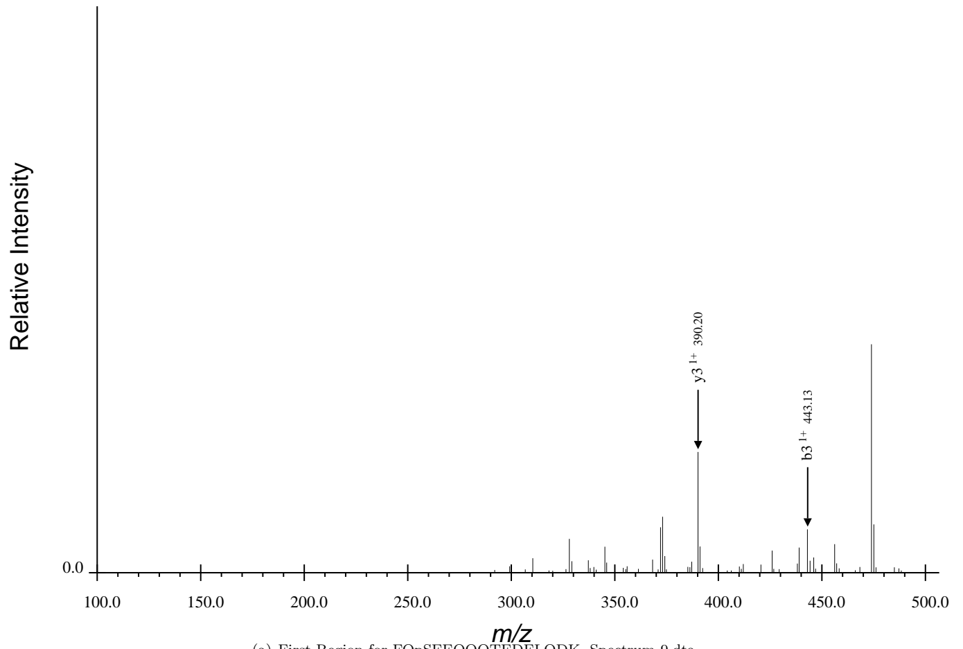
(a) First Region for FQpSEEQQQTEDELQDK, Spectrum 9.dta
