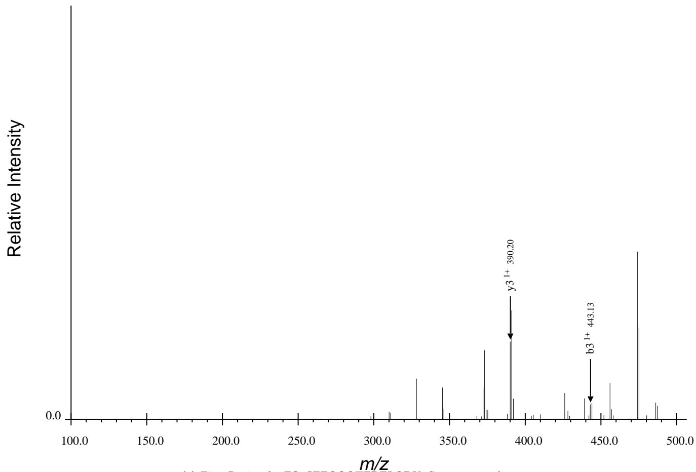
(a) First Region for FQpSEEQQQTEDELQDK, Spectrum 11.dta
