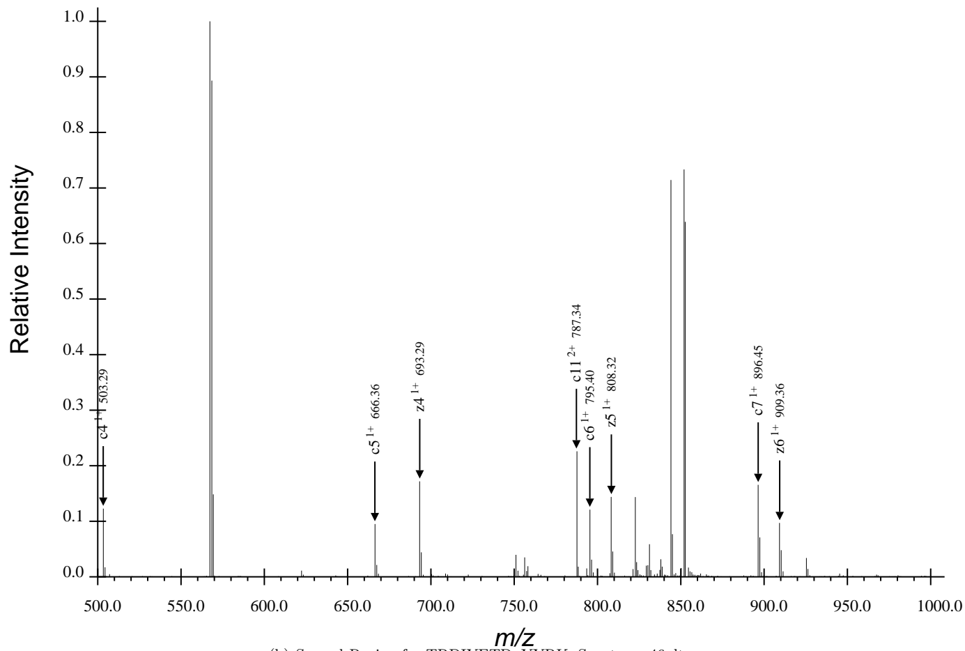
(b) Second Region for TRDIYETDpYYRK, Spectrum 46.dta
