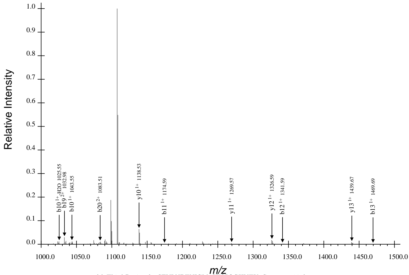
(c) Third Region for SFVLNPTNIGMpSKSSQGHVTK, Spectrum 20.dta
