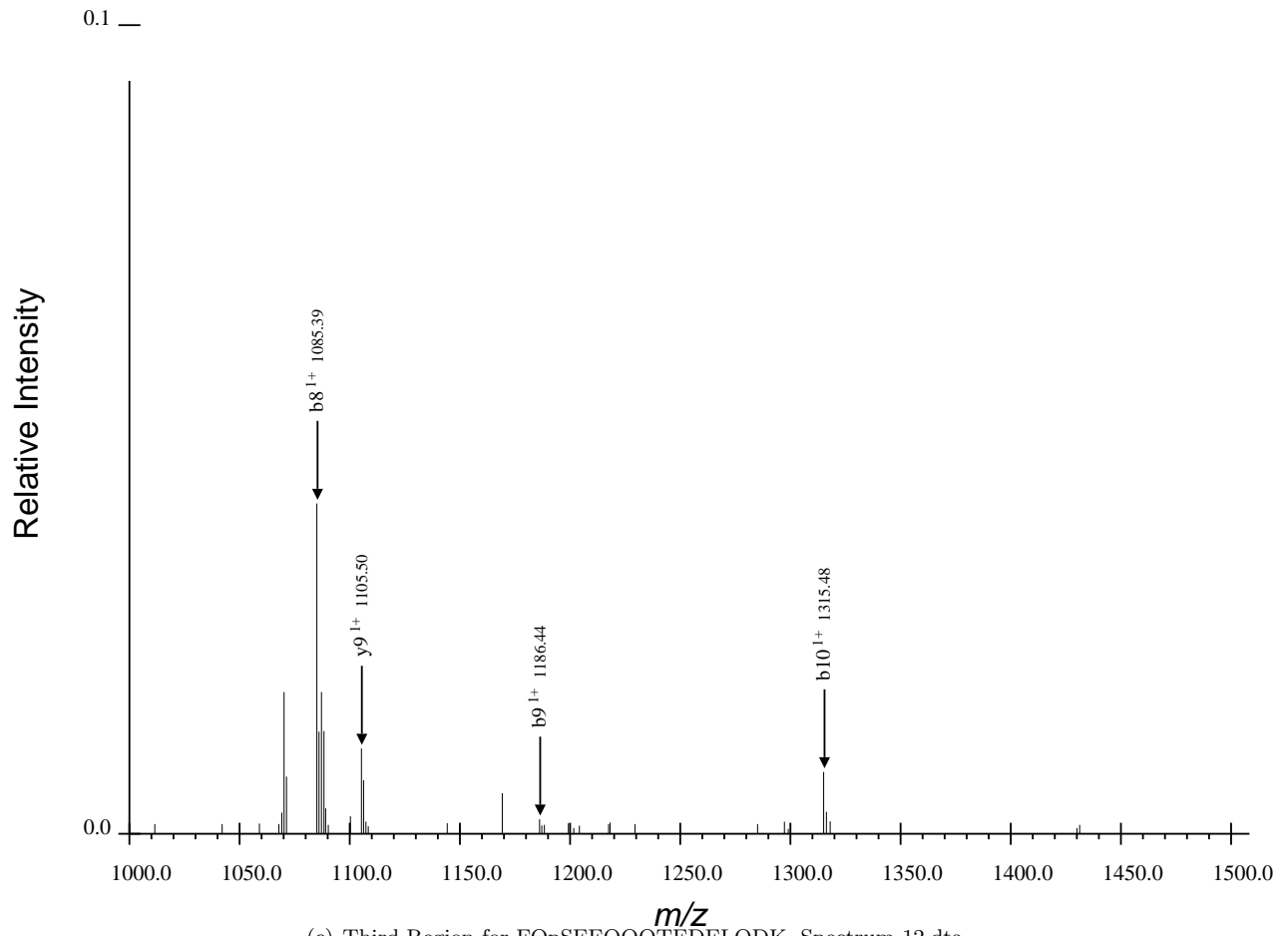
(c) Third Region for FQpSEEQQQTEDELQDK, Spectrum 12.dta
