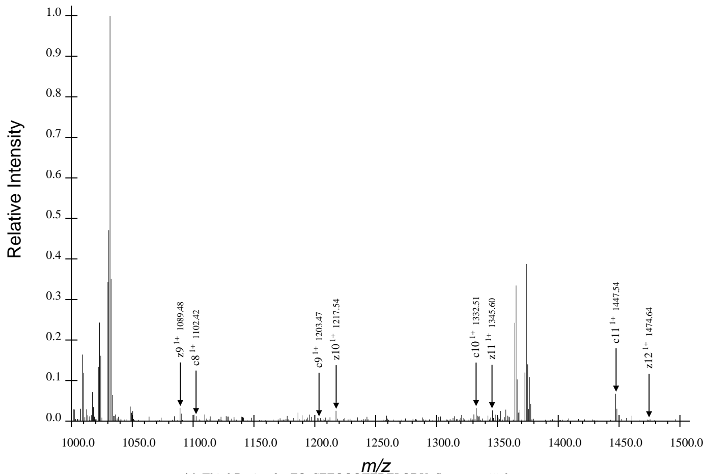
(c) Third Region for FQpSEEQQQTEDELQDK, Spectrum 15.dta
