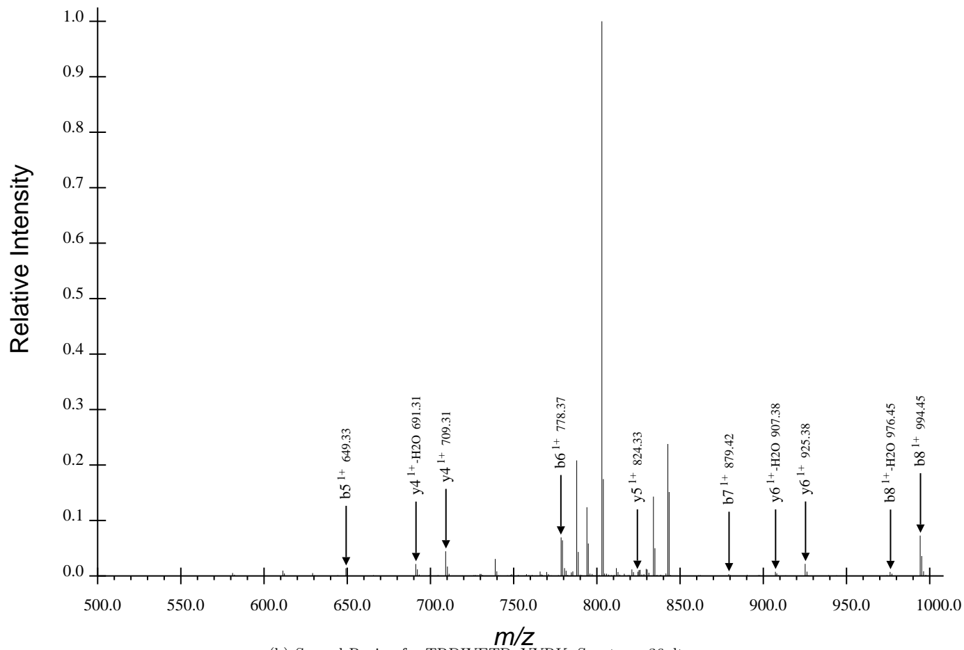
(b) Second Region for TRDIYETDpYYRK, Spectrum 36.dta
