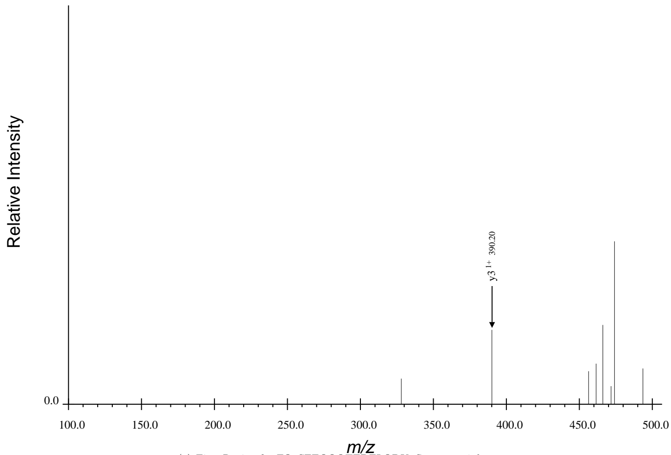
(a) First Region for FQpSEEQQQTEDELQDK, Spectrum 6.dta
