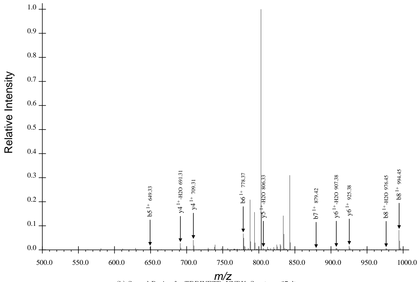
(b) Second Region for TRDIYETDpYYRK, Spectrum 37.dta
