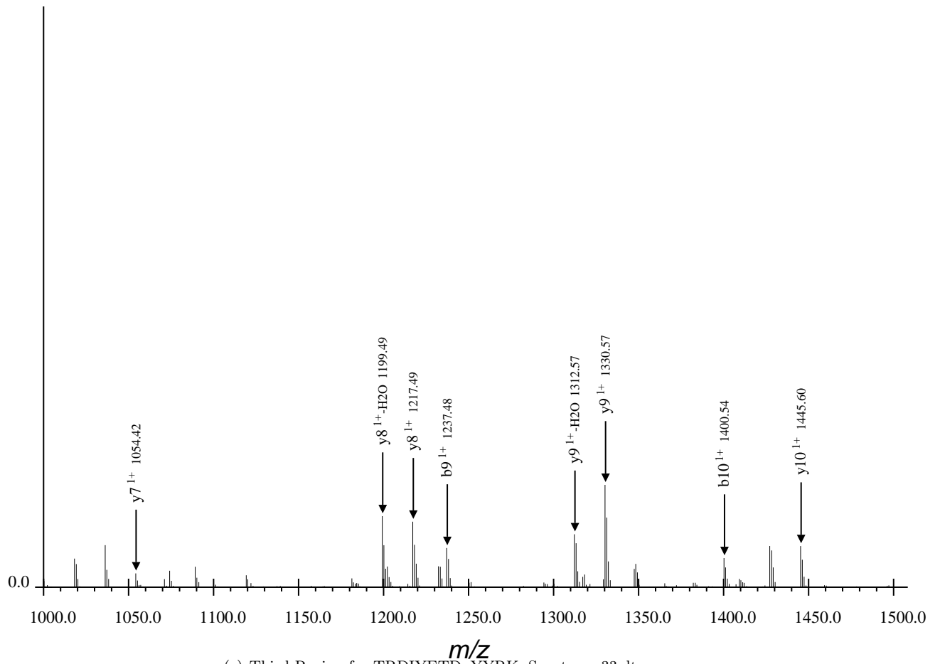
(c) Third Region for TRDIYETDpYYRK, Spectrum 33.dta
