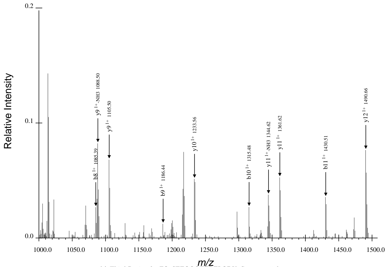
(c) Third Region for FQpSEEQQQTEDELQDK, Spectrum 5.dta
