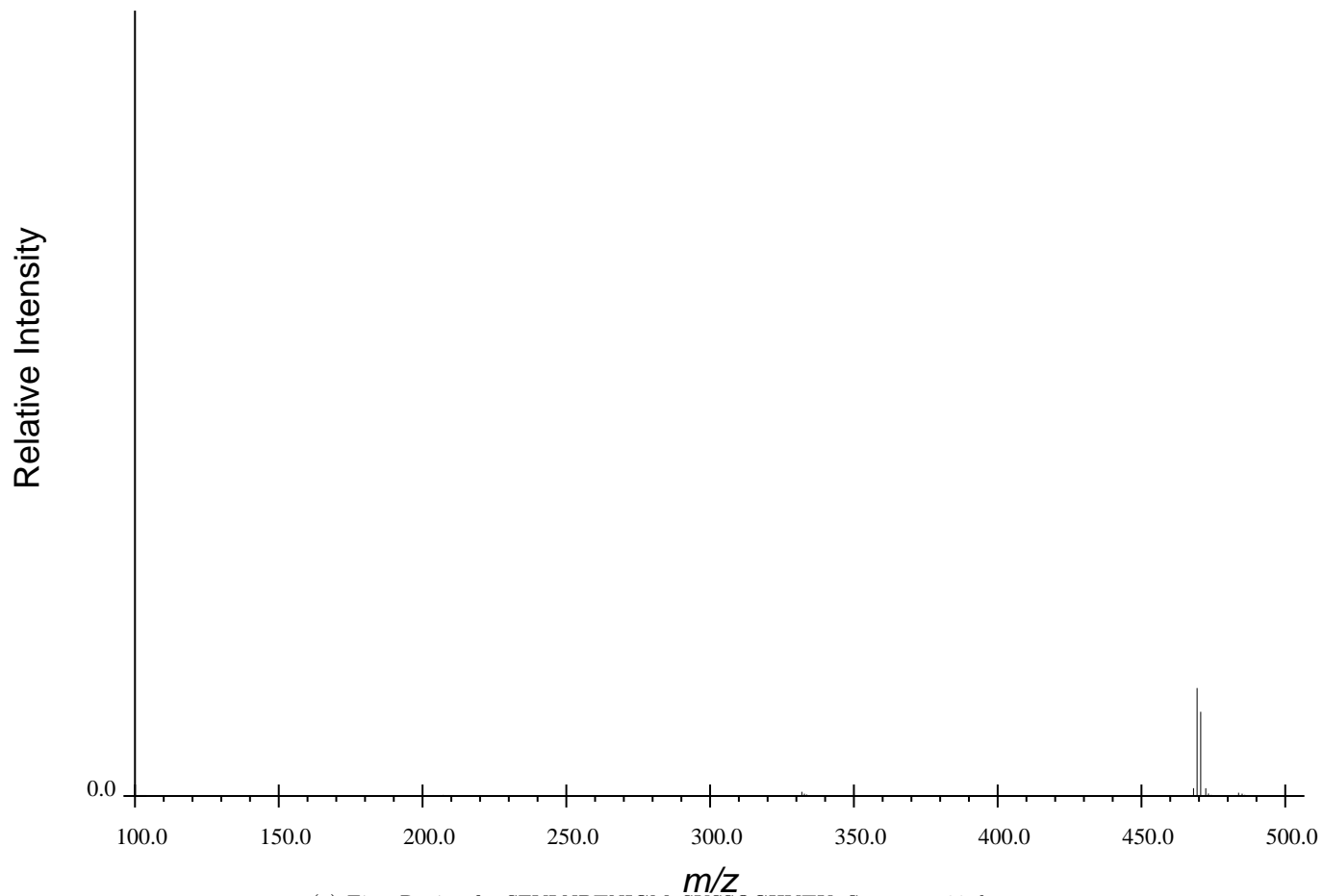
(a) First Region for SFVLNPTNIGMpSKSSQGHVTK, Spectrum 22.dta
