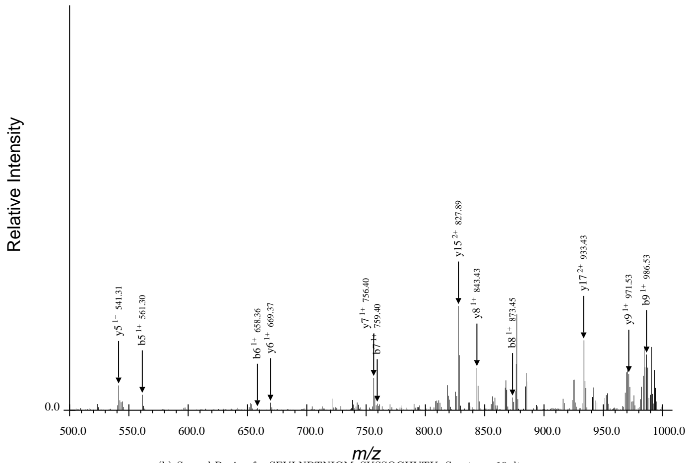
(b) Second Region for SFVLNPTNIGMpSKSSQGHVTK, Spectrum 19.dta
