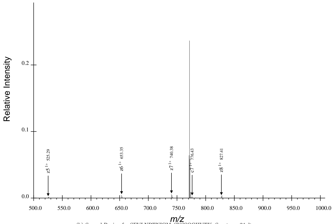
(b) Second Region for SFVLNPTNIGMpSKSSQGHVTK, Spectrum 24.dta
