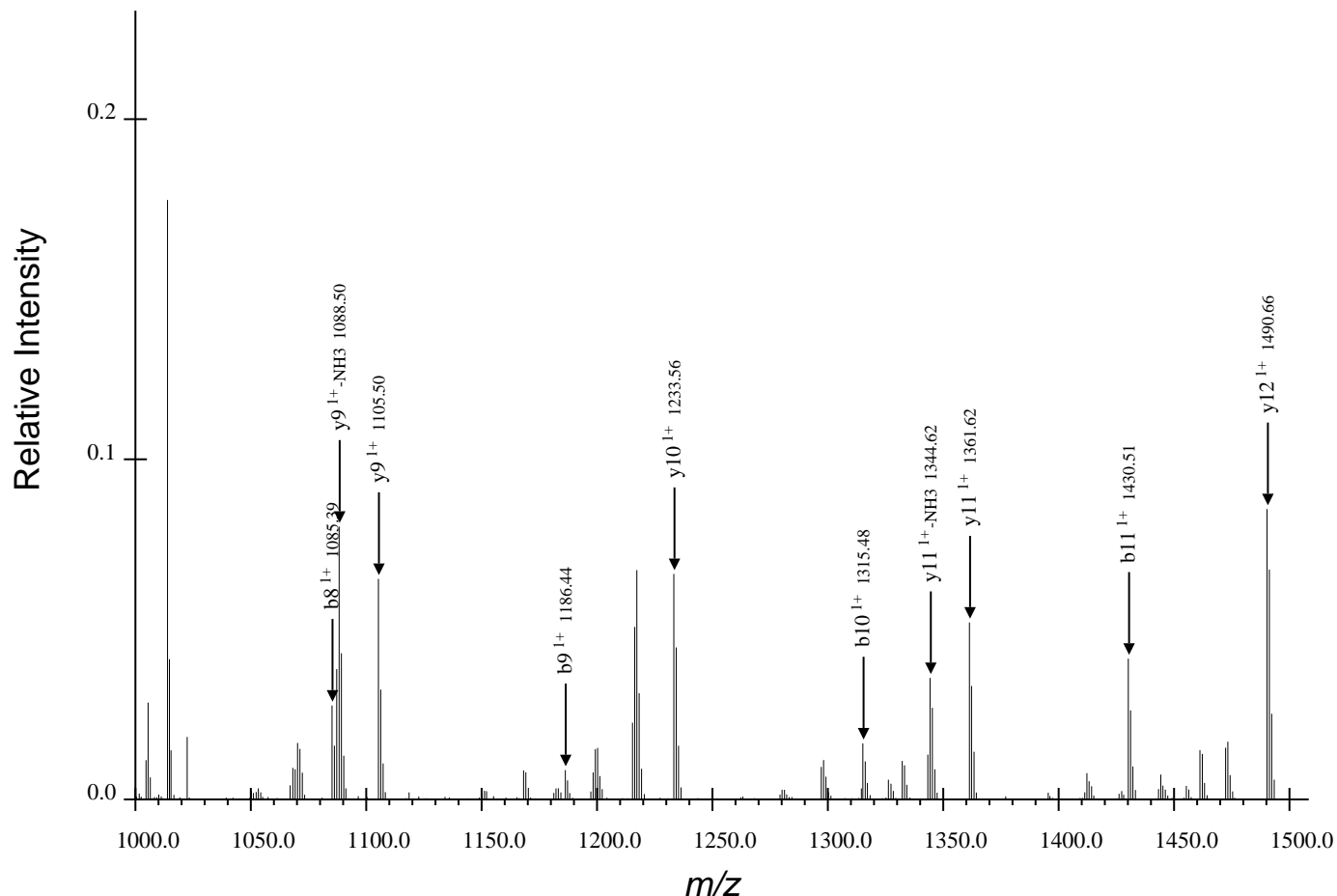
(c) Third Region for FQpSEEQQQTEDELQDK, Spectrum 2.dta
