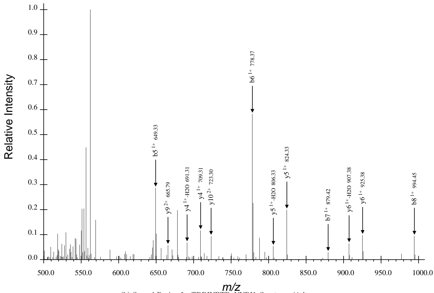
(b) Second Region for TRDIYETDpYYRK, Spectrum 44.dta
