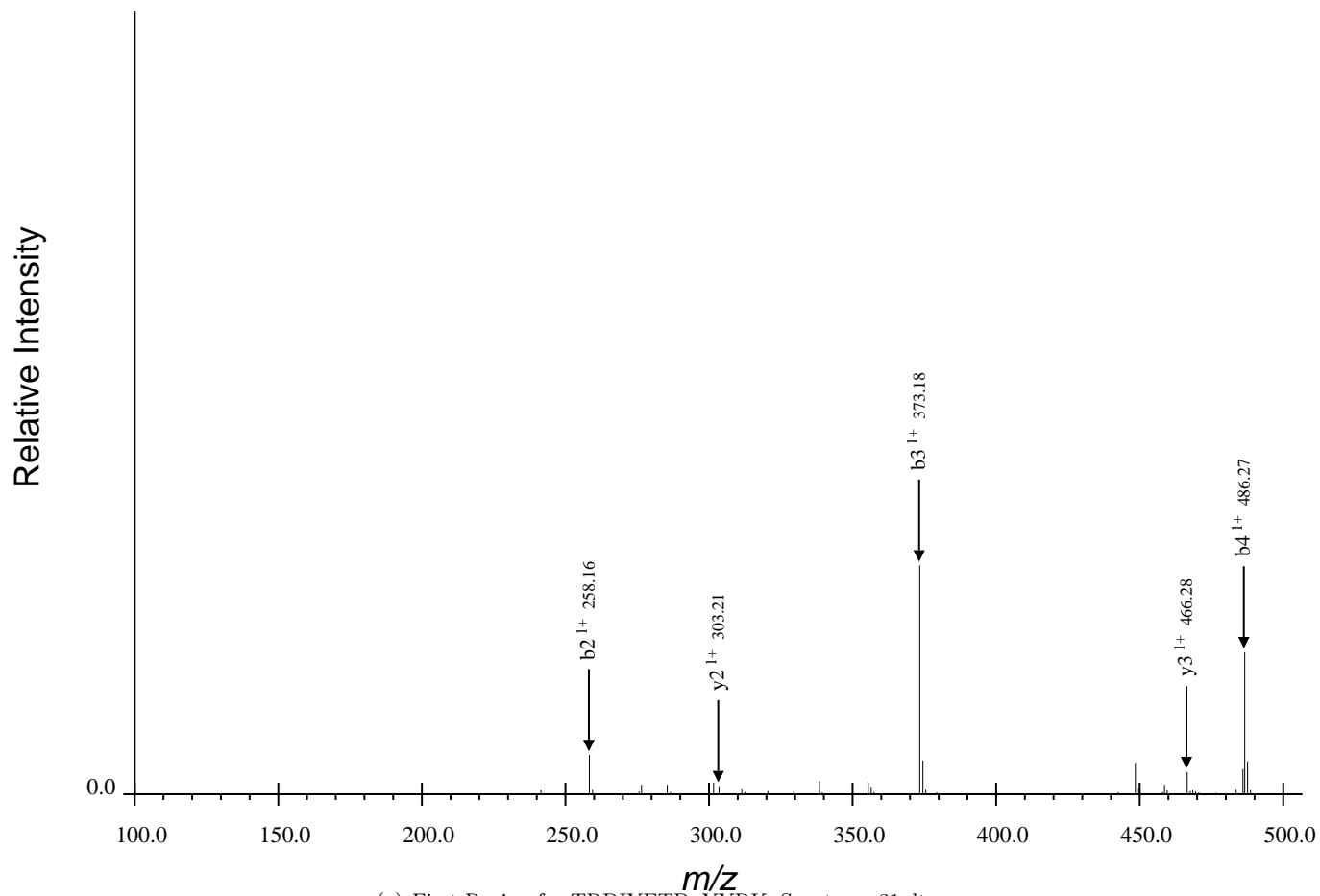
(a) First Region for TRDIYETDpYYRK, Spectrum 31.dta
