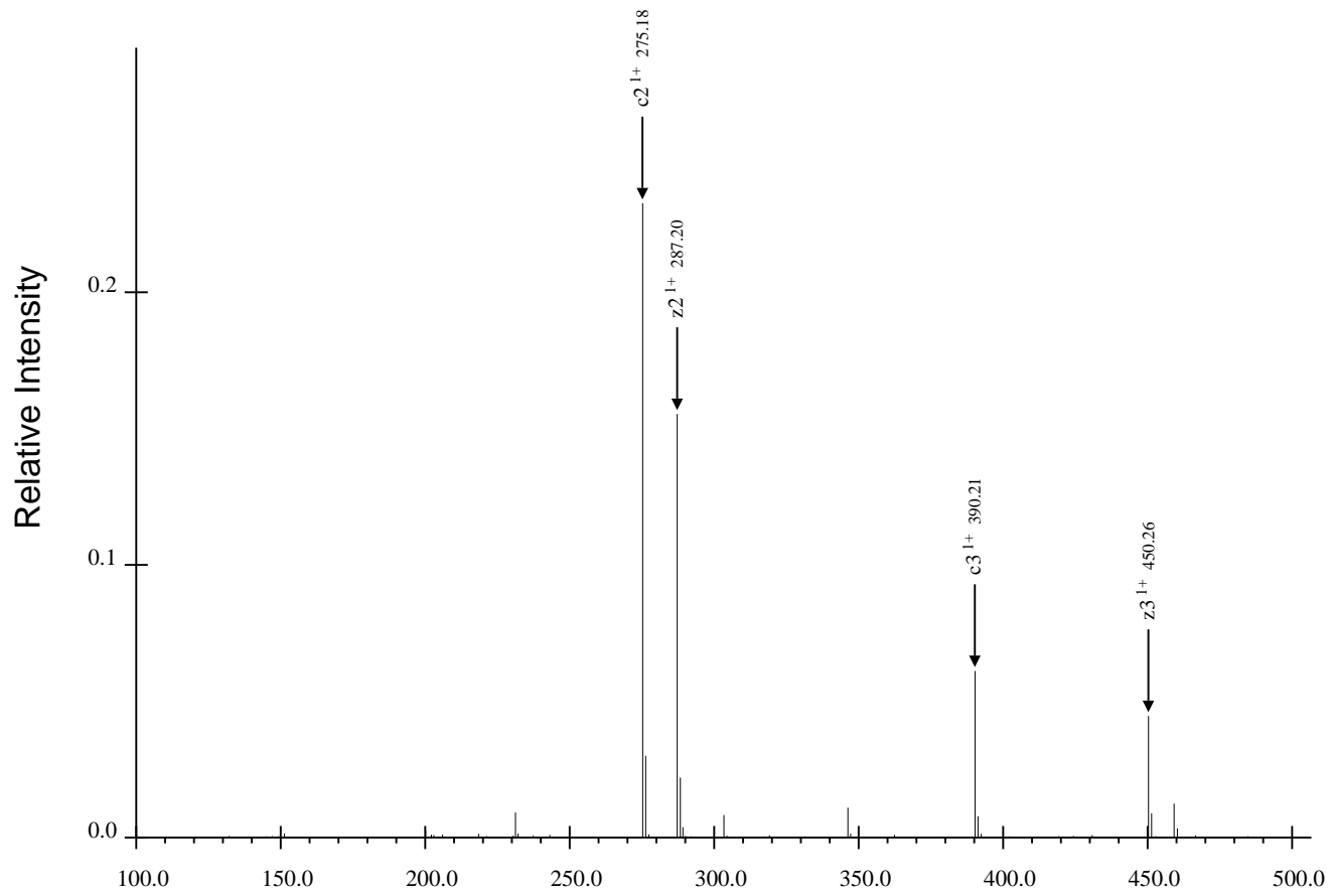
(a) First Region for TRDIYETDpYYRK, Spectrum 47.dta
