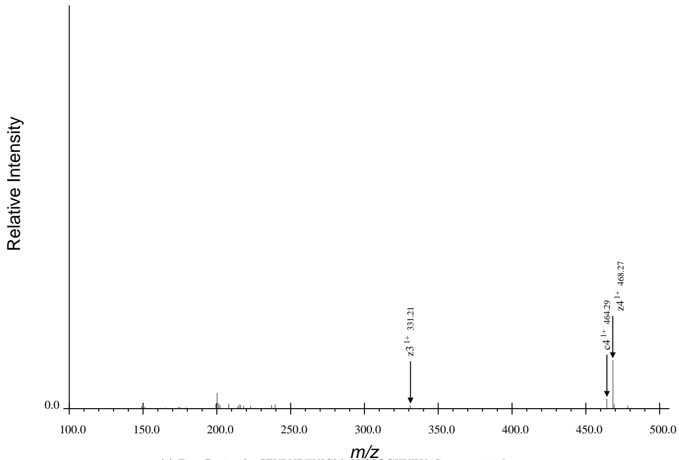
(a) First Region for SFVLNPTNIGMpSKSSQGHVTK, Spectrum 23.dta
