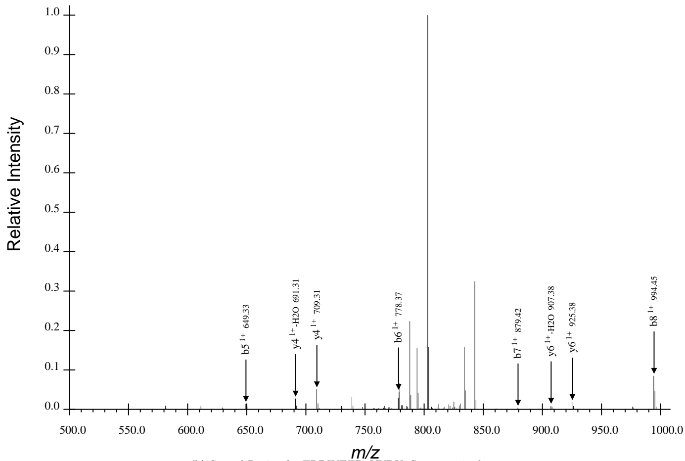
(b) Second Region for TRDIYETDpYYRK, Spectrum 35.dta
