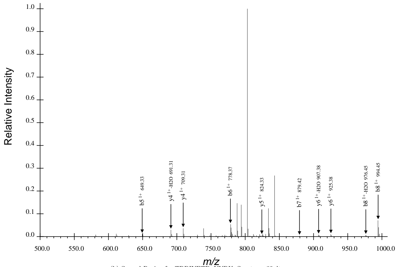
(b) Second Region for TRDIYETDpYYRK, Spectrum 32.dta
