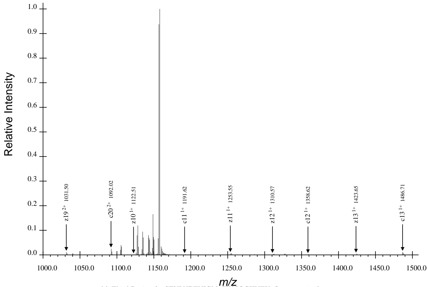
(c) Third Region for SFVLNPTNIGMpSKSSQGHVTK, Spectrum 25.dta
