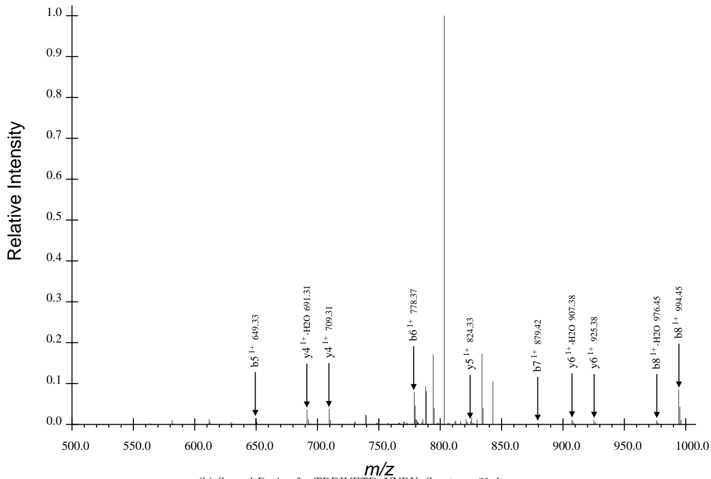
(b) Second Region for TRDIYETDpYYRK, Spectrum 31.dta
