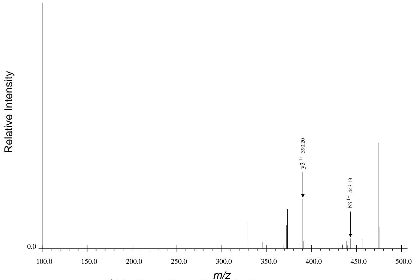
(a) First Region for FQpSEEQQQTEDELQDK, Spectrum 4.dta
