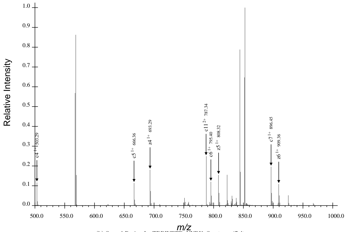
(b) Second Region for TRDIYETDpYYRK, Spectrum 47.dta
