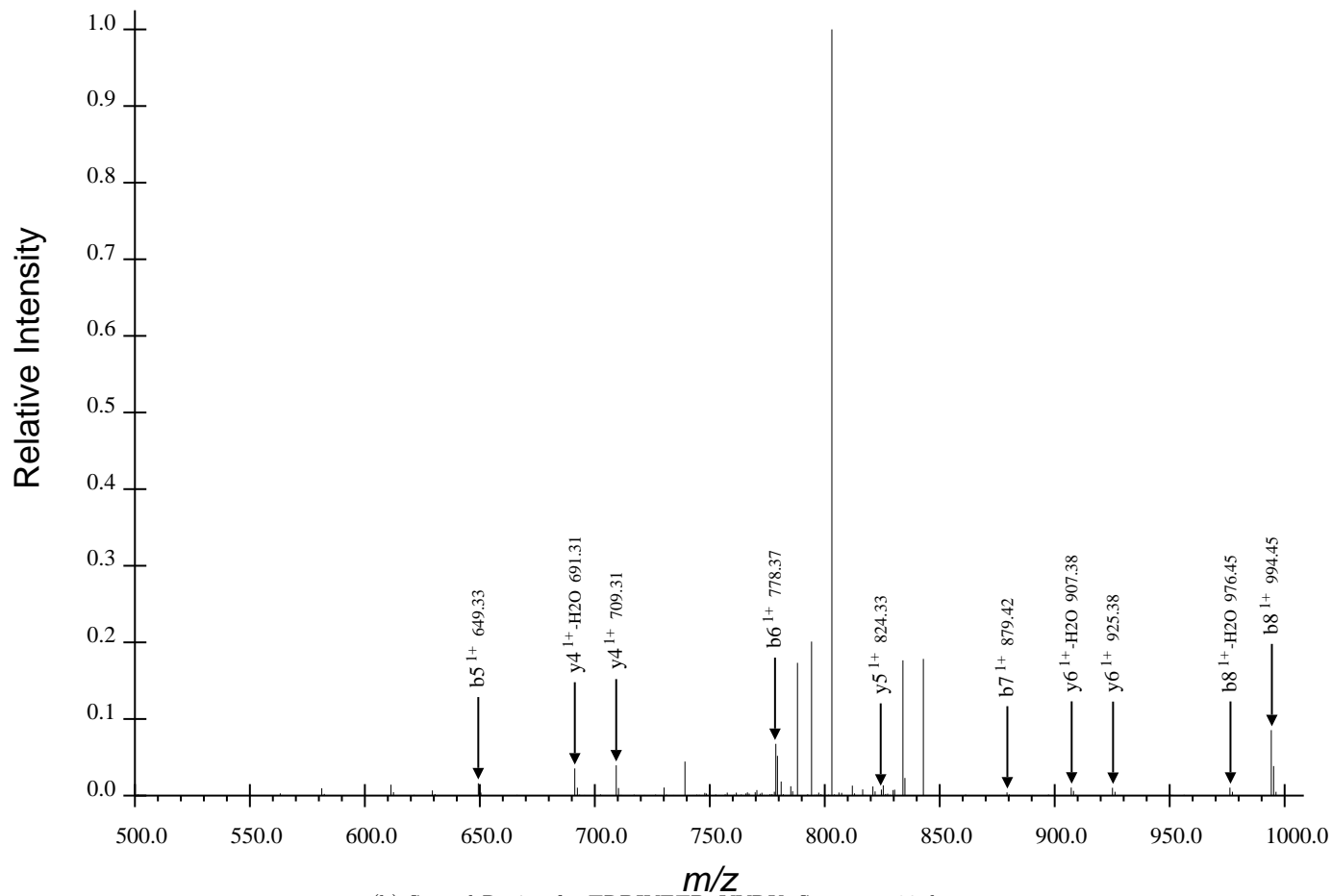
(b) Second Region for TRDIYETDpYYRK, Spectrum 30.dta
