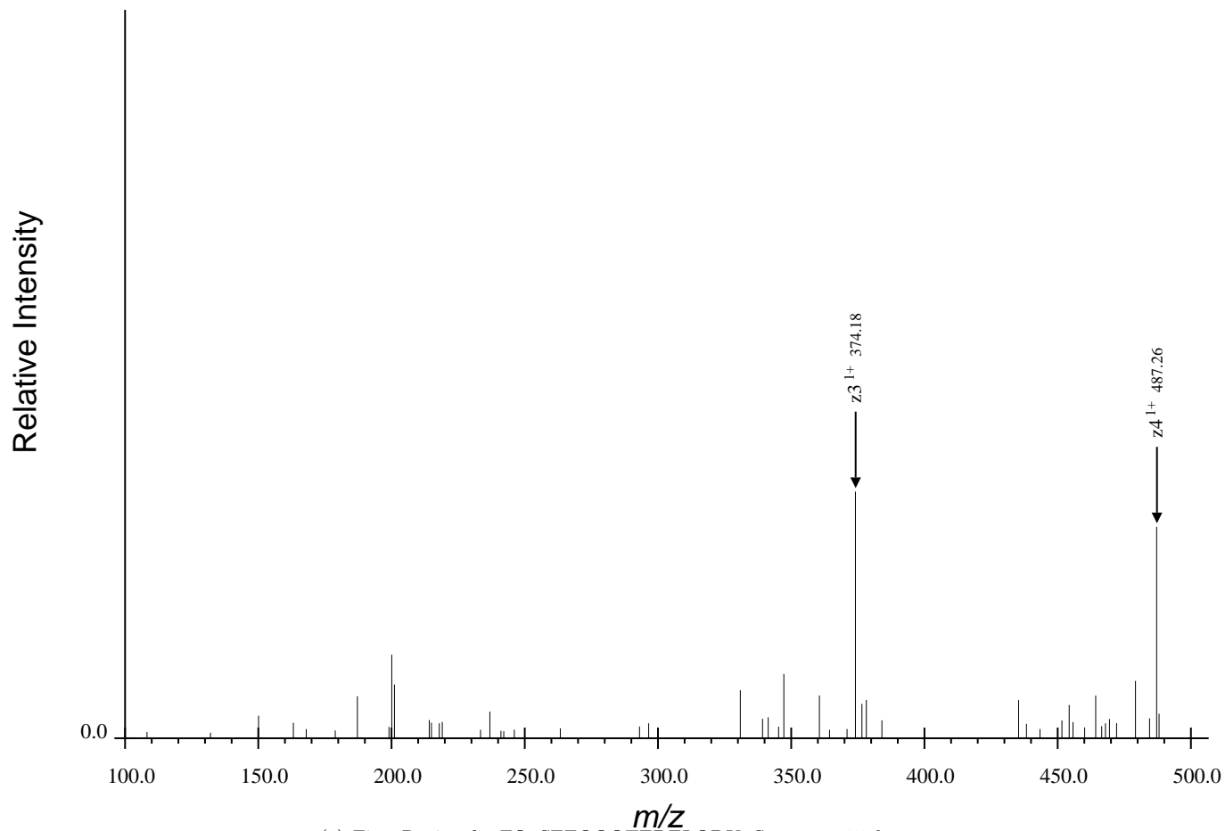
(a) First Region for FQpSEEQQQTEDELQDK, Spectrum 15.dta
