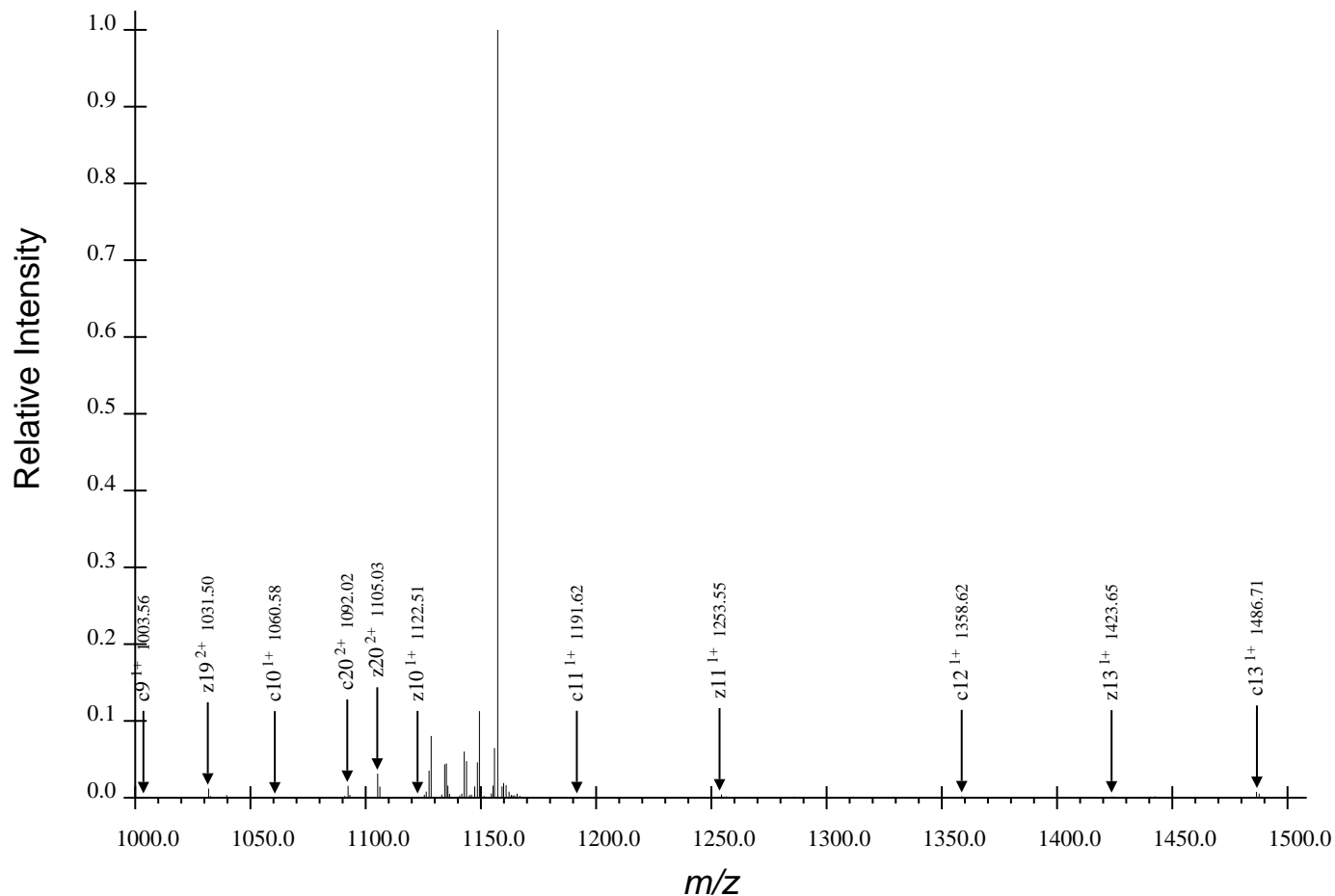
(c) Third Region for SFVLNPTNIGMpSKSSQGHVTK, Spectrum 24.dta
