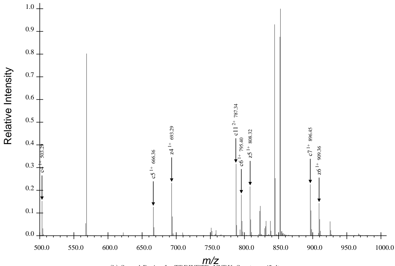
(b) Second Region for TRDIYETDpYYRK, Spectrum 45.dta
