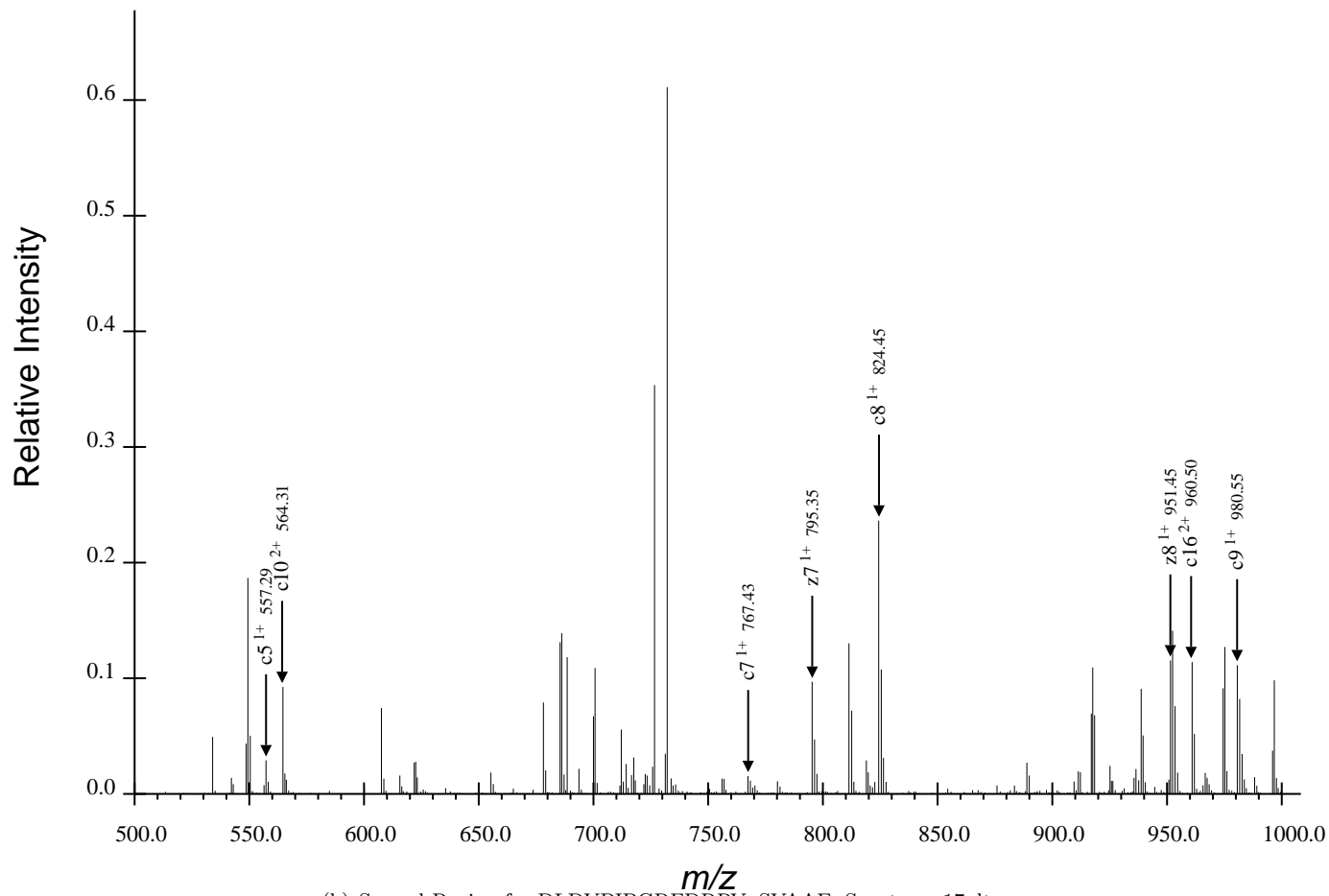
(b) Second Region for DLDVPIPGRFDRRVpSVA AE, Spectrum 17.dta
