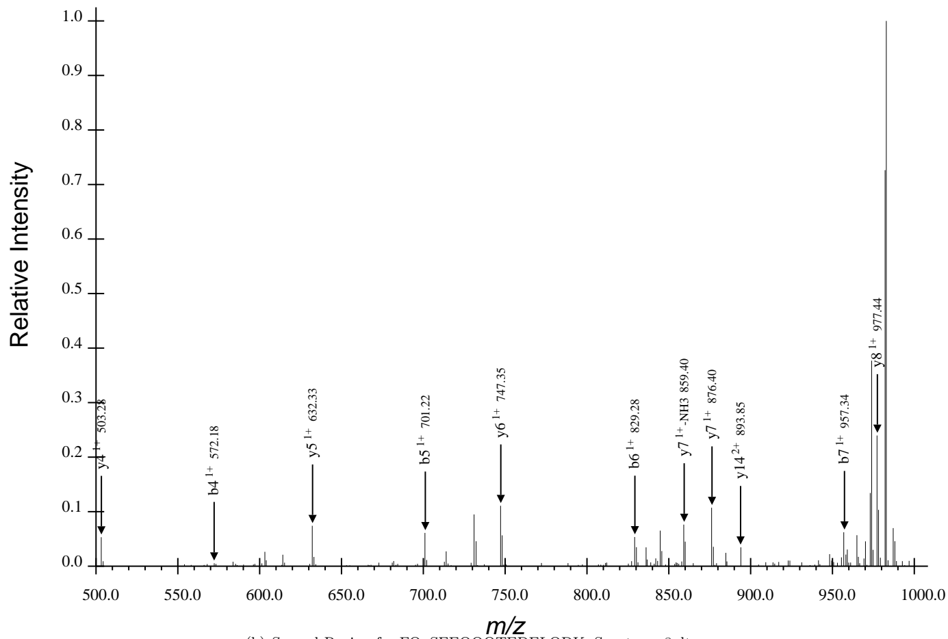
(b) Second Region for FQpSEEQQQTEDELQDK, Spectrum 8.dta
