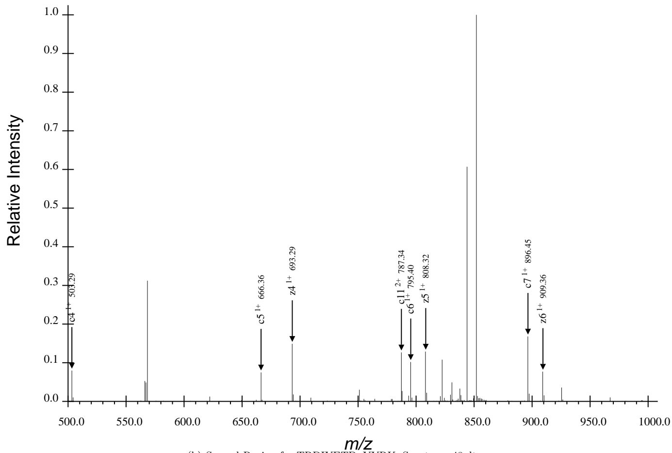
(b) Second Region for TRDIYETDpYYRK, Spectrum 48.dta
