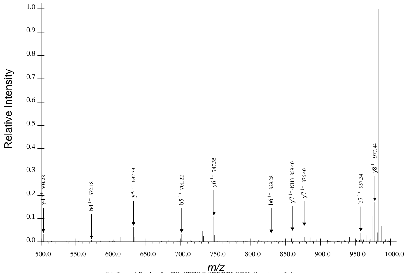
(b) Second Region for FQpSEEQQQTEDELQDK, Spectrum 3.dta
