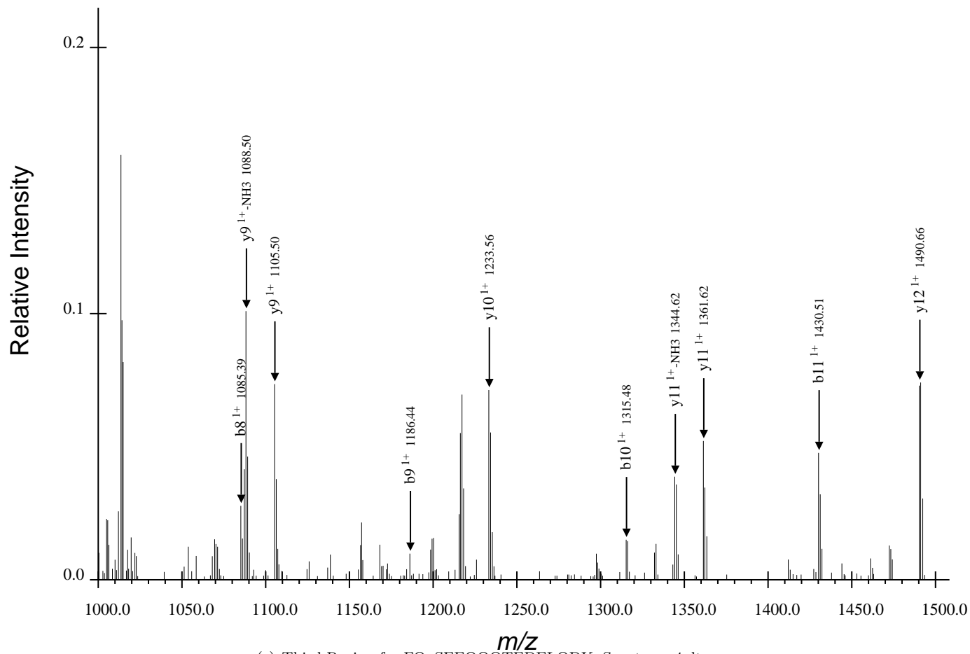
(c) Third Region for FQpSEEQQQTEDELQDK, Spectrum 4.dta
