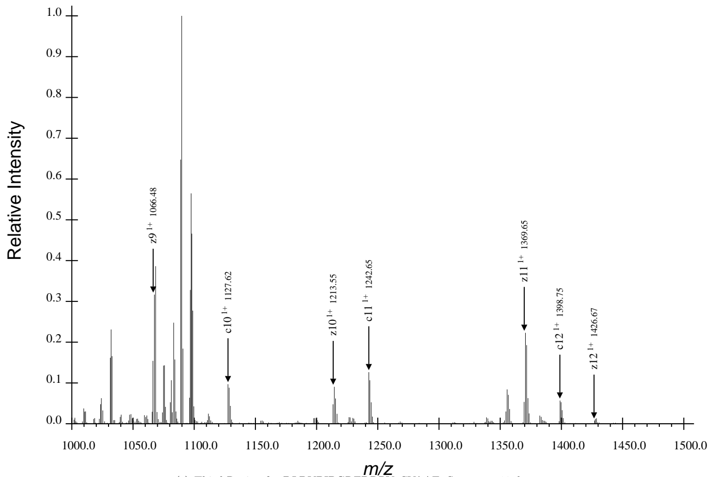
(c) Third Region for DLDVPIPGRFDRRVpSVA AE, Spectrum 18.dta
