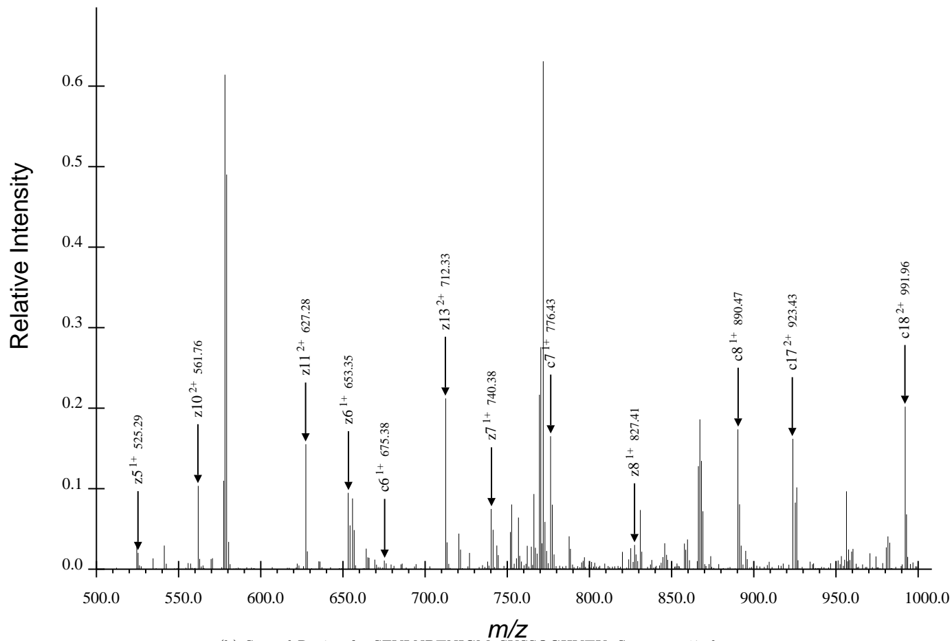
(b) Second Region for SFVLNPTNIGMpSKSSQGHVTK, Spectrum 27.dta
