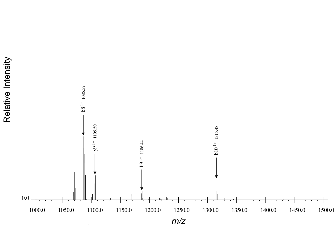
(c) Third Region for FQpSEEQQQTEDELQDK, Spectrum 14.dta
