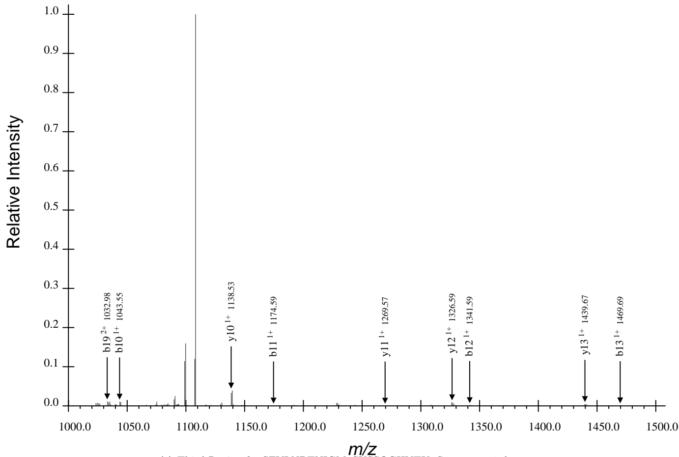
(c) Third Region for SFVLNPTNIGMpSKSSQGHVTK, Spectrum 19.dta
