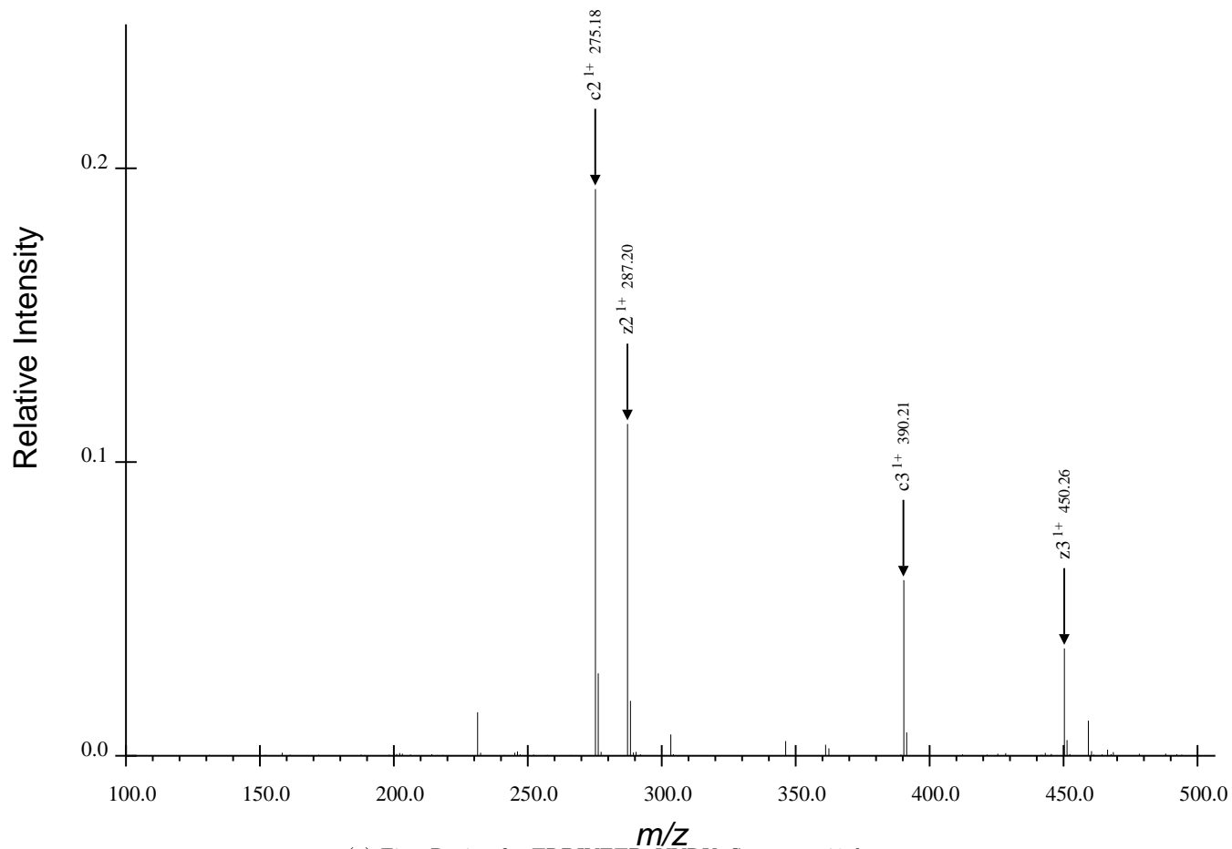
(a) First Region for TRDIYETDpYYRK, Spectrum 46.dta
