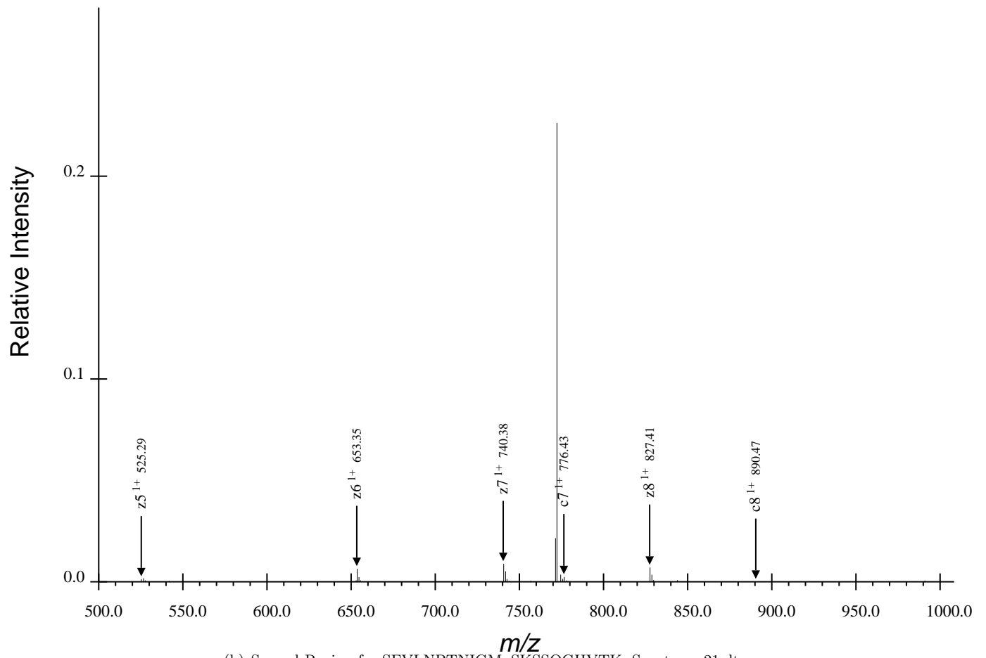
(b) Second Region for SFVLNPTNIGMpSKSSQGHVTK, Spectrum 21.dta
