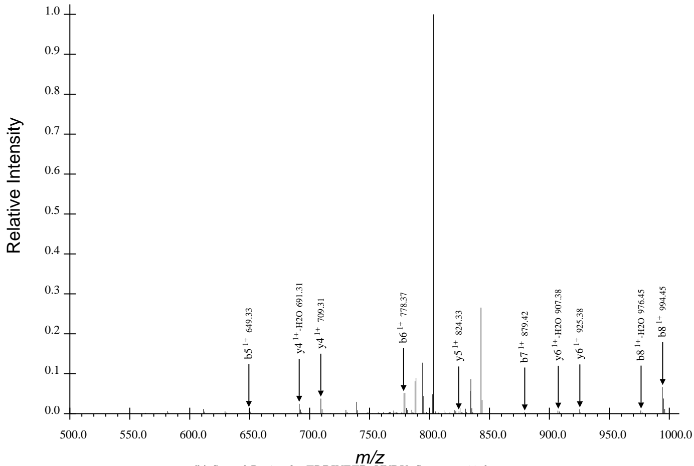
(b) Second Region for TRDIYETDpYYRK, Spectrum 33.dta
