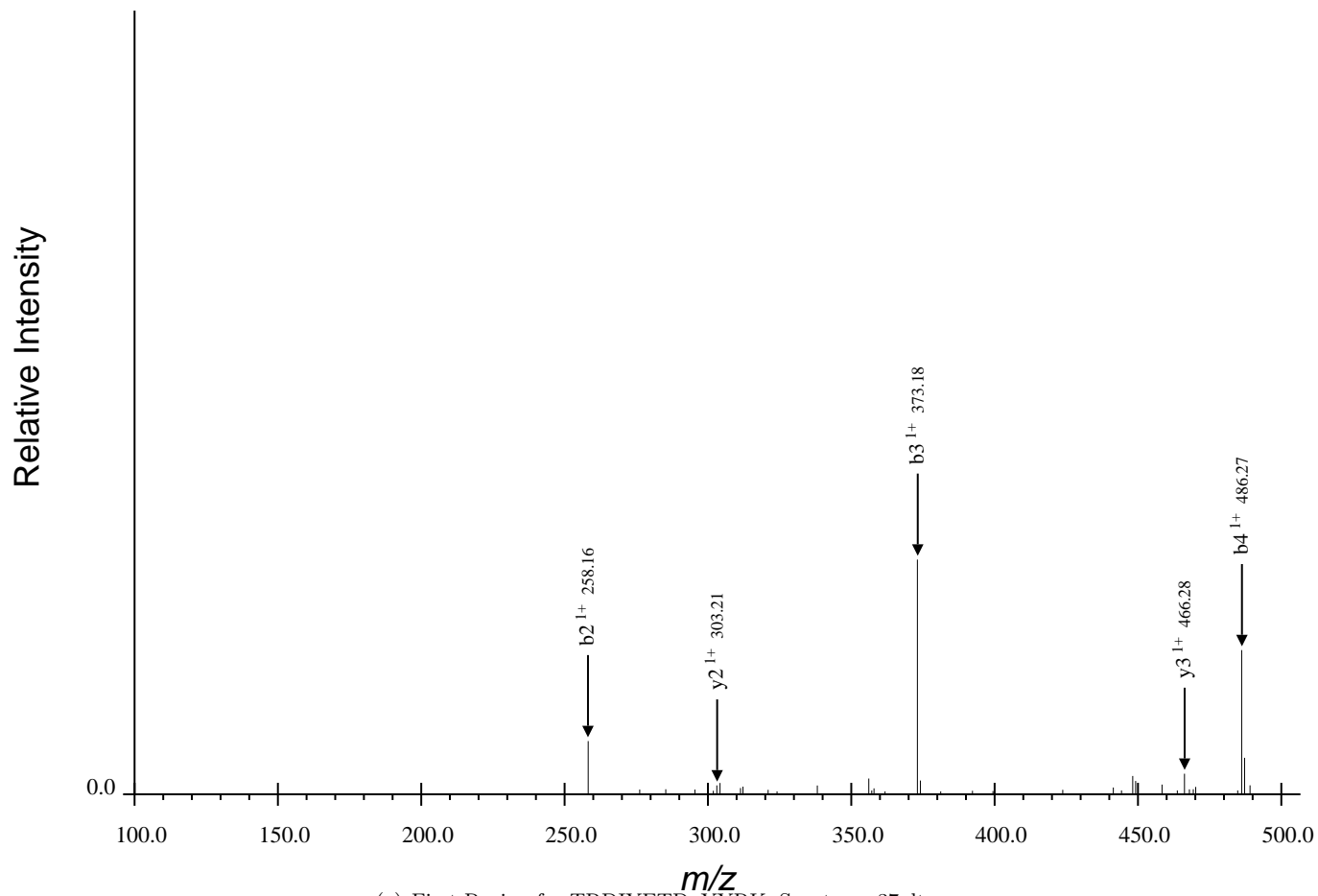
(a) First Region for TRDIYETDpYYRK, Spectrum 37.dta
