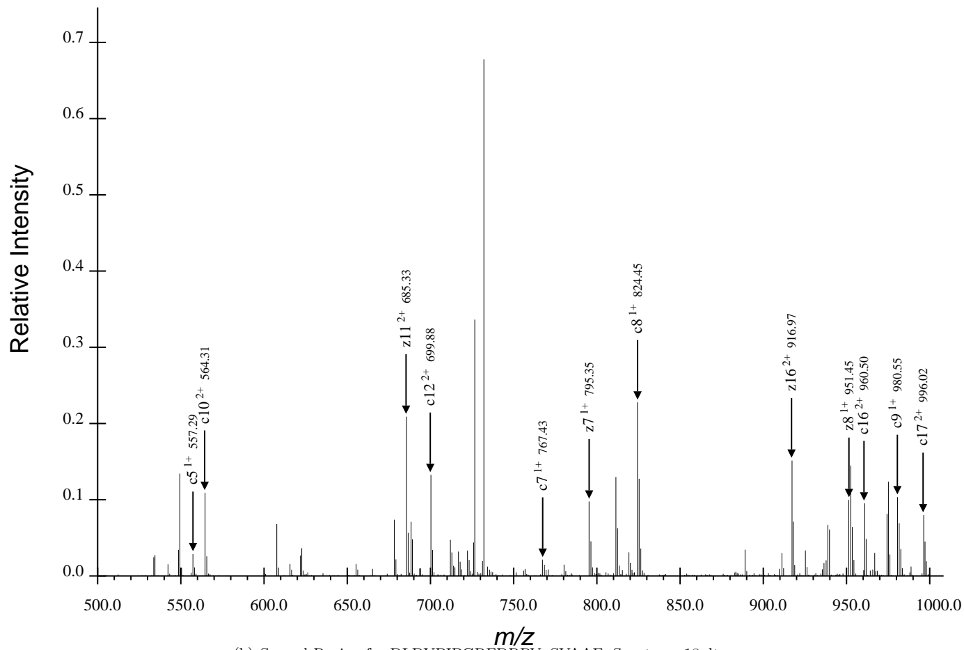
(b) Second Region for DLDVPIPGRFDRRVpSVAAE, Spectrum 18.dta
