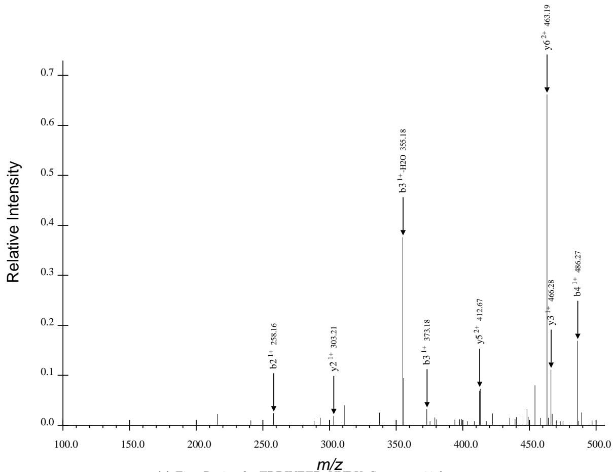
(a) First Region for TRDIYETDpYYRK, Spectrum 44.dta
