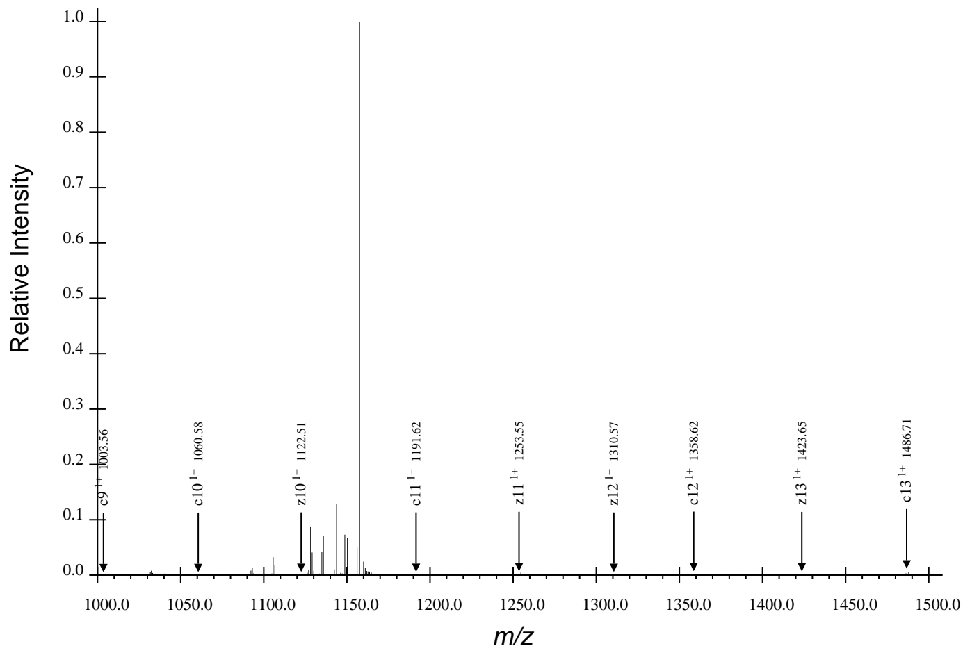
(c) Third Region for SFVLNPTNIGMpSKSSQGHVTK, Spectrum 21.dta
