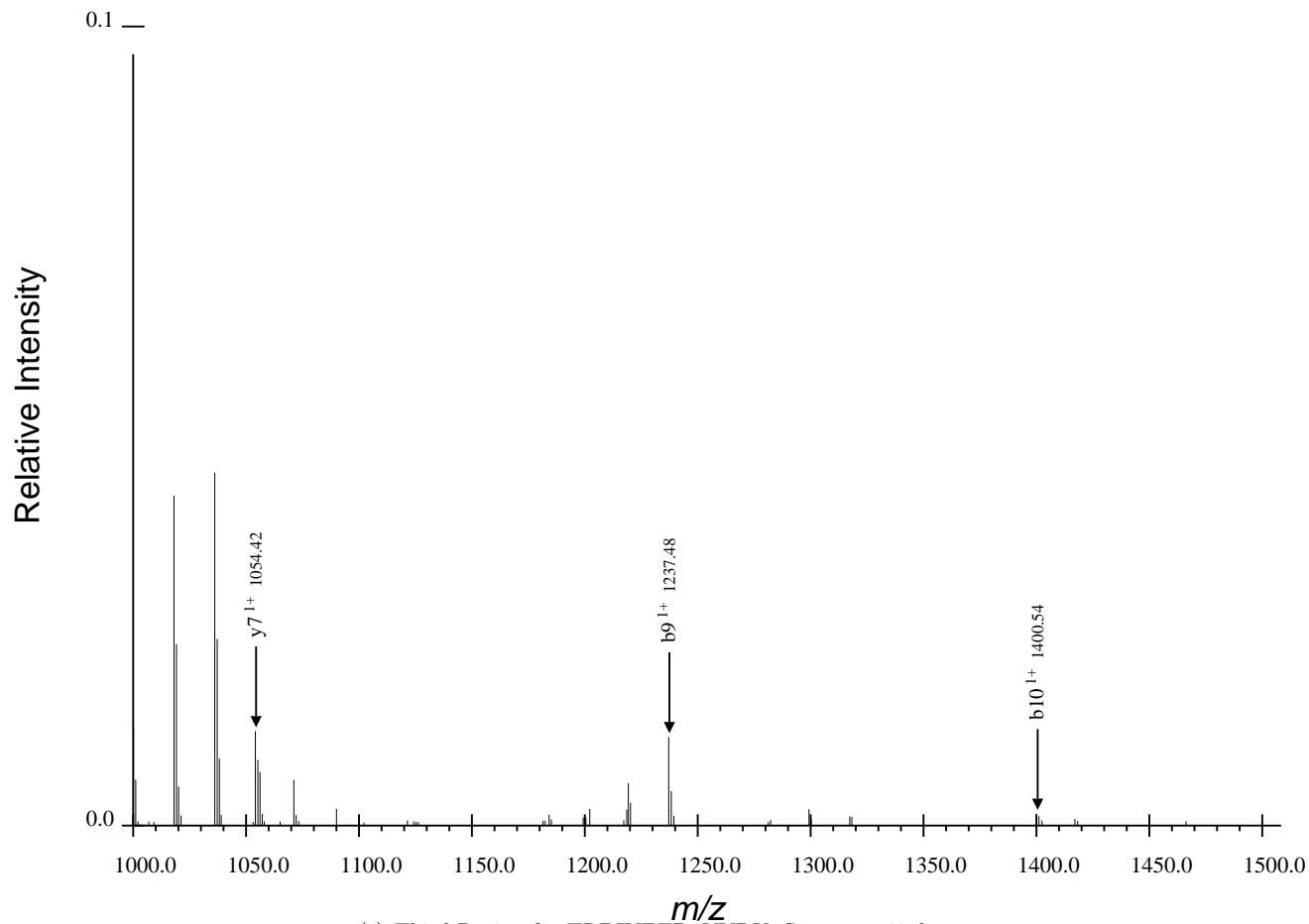
(c) Third Region for TRDIYETDpYYRK, Spectrum 40.dta
