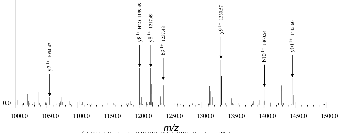
(c) Third Region for TRDIYETDpYYRK, Spectrum 37.dta
