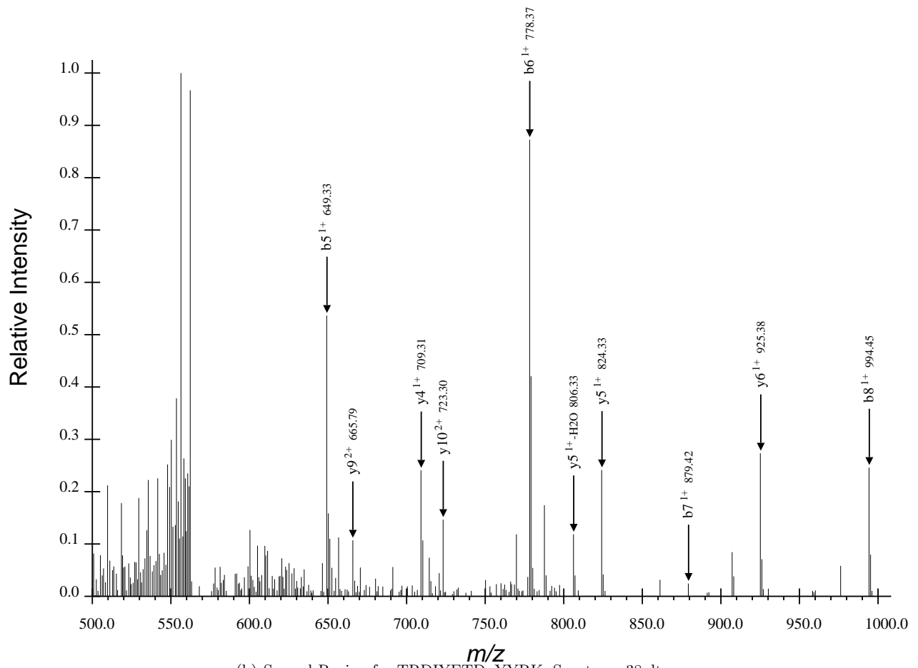
(b) Second Region for TRDIYETDpYYRK, Spectrum 38.dta
