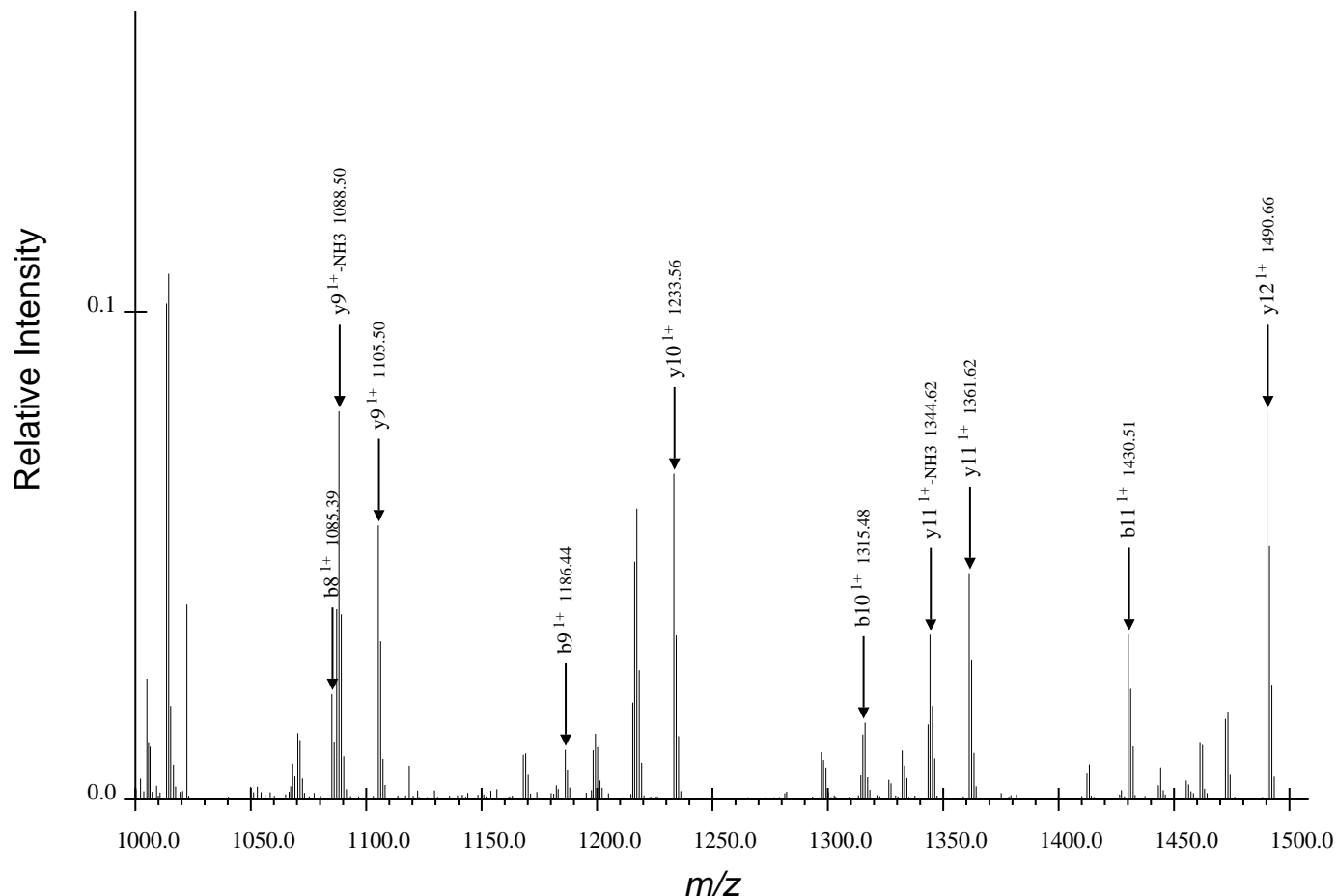
(c) Third Region for FQpSEEQQQTEDELQDK, Spectrum 1.dta
