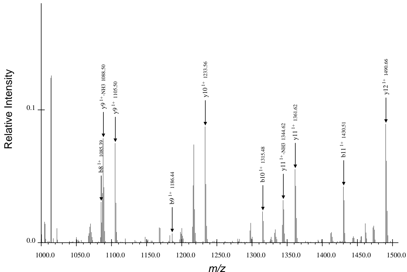
(c) Third Region for FQpSEEQQQTEDELQDK, Spectrum 9.dta
