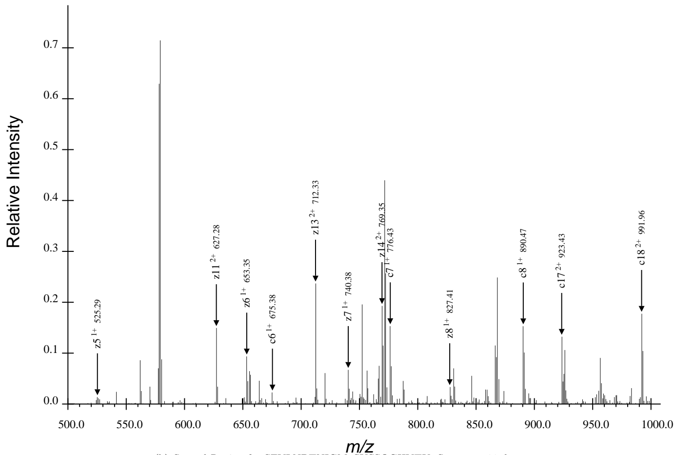
(b) Second Region for SFVLNPTNIGMpSKSSQGHVTK, Spectrum 28.dta
