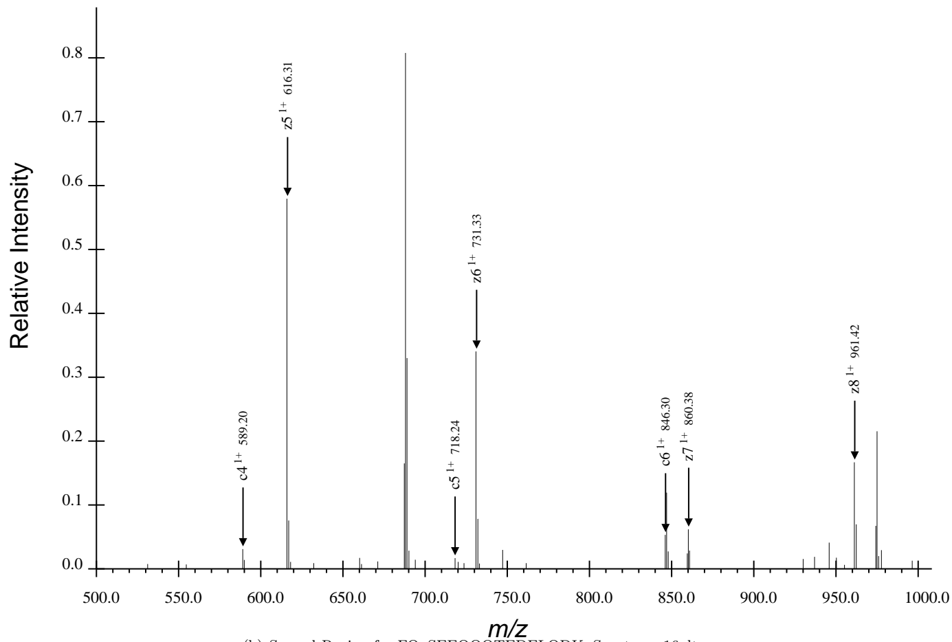
(b) Second Region for FQpSEEQQQTEDELQDK, Spectrum 16.dta
