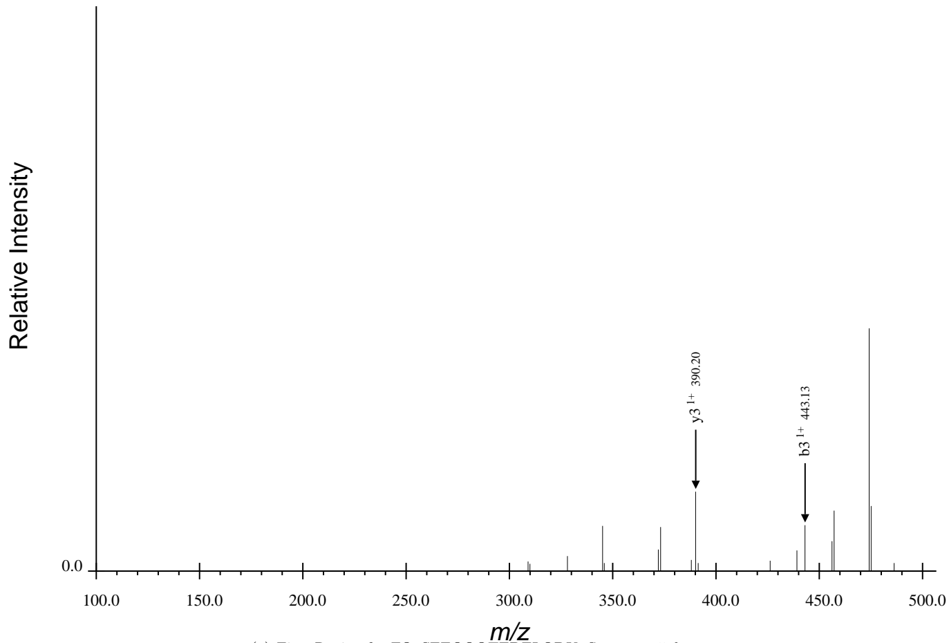
(a) First Region for FQpSEEQQQTEDELQDK, Spectrum 5.dta
