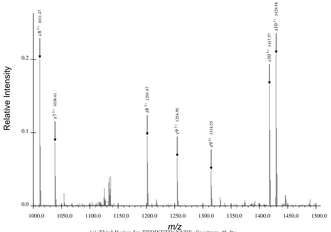
(c) Third Region for TRDIYETDpYYRK, Spectrum 46.dta
