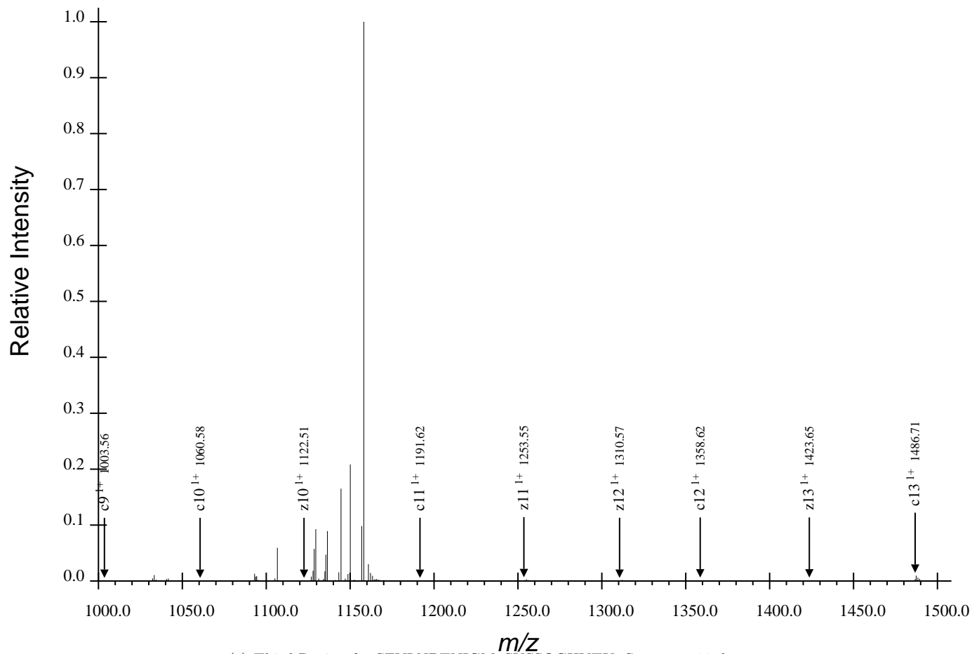
(c) Third Region for SFVLNPTNIGMpSKSSQGHVTK, Spectrum 22.dta
