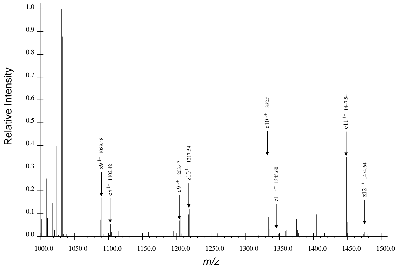
(c) Third Region for FQpSEEQQQTEDELQDK, Spectrum 16.dta
