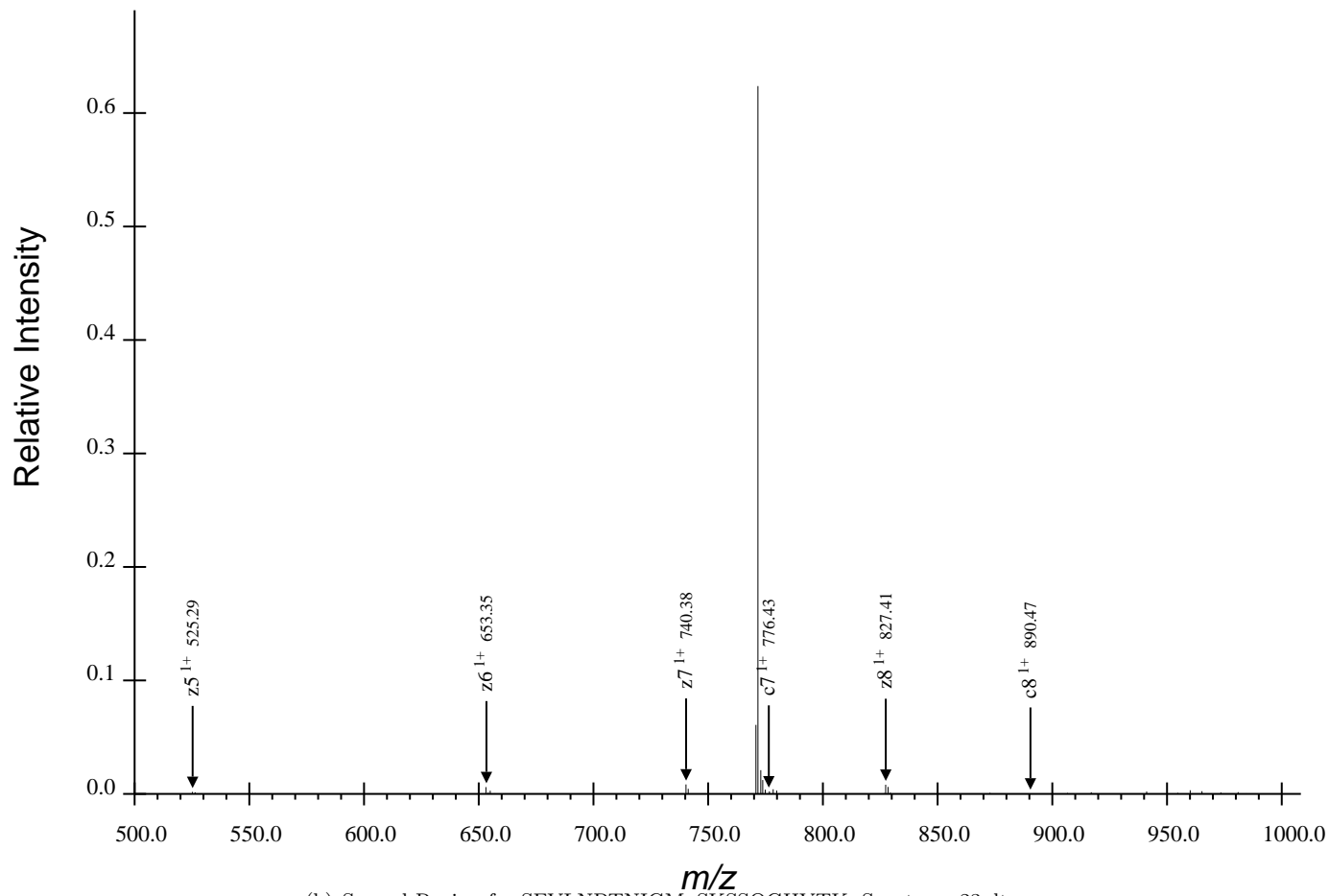
(b) Second Region for SFVLNPTNIGMpSKSSQGHVTK, Spectrum 23.dta
