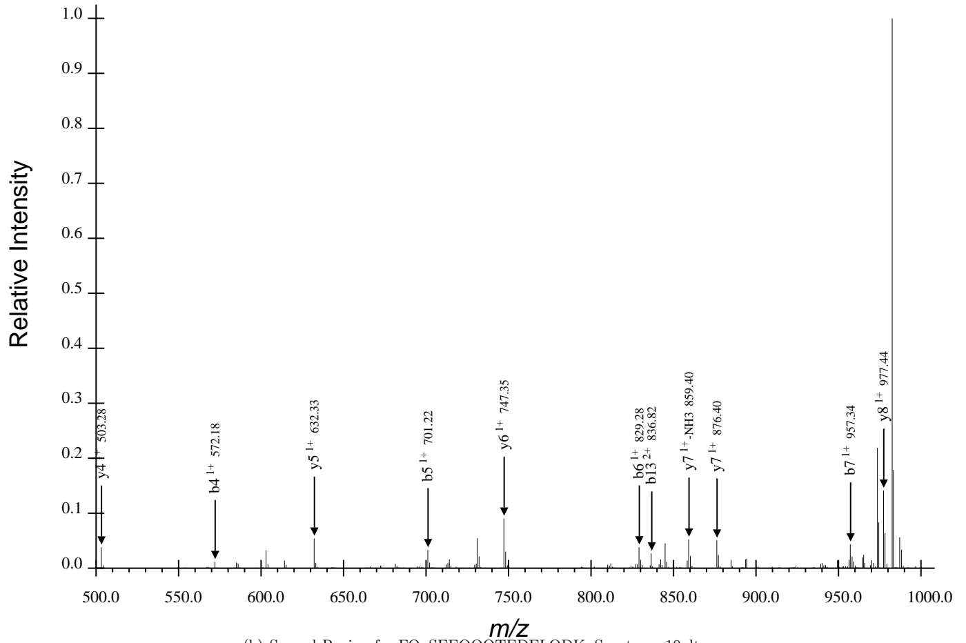
(b) Second Region for FQpSEEQQQTEDELQDK, Spectrum 10.dta
