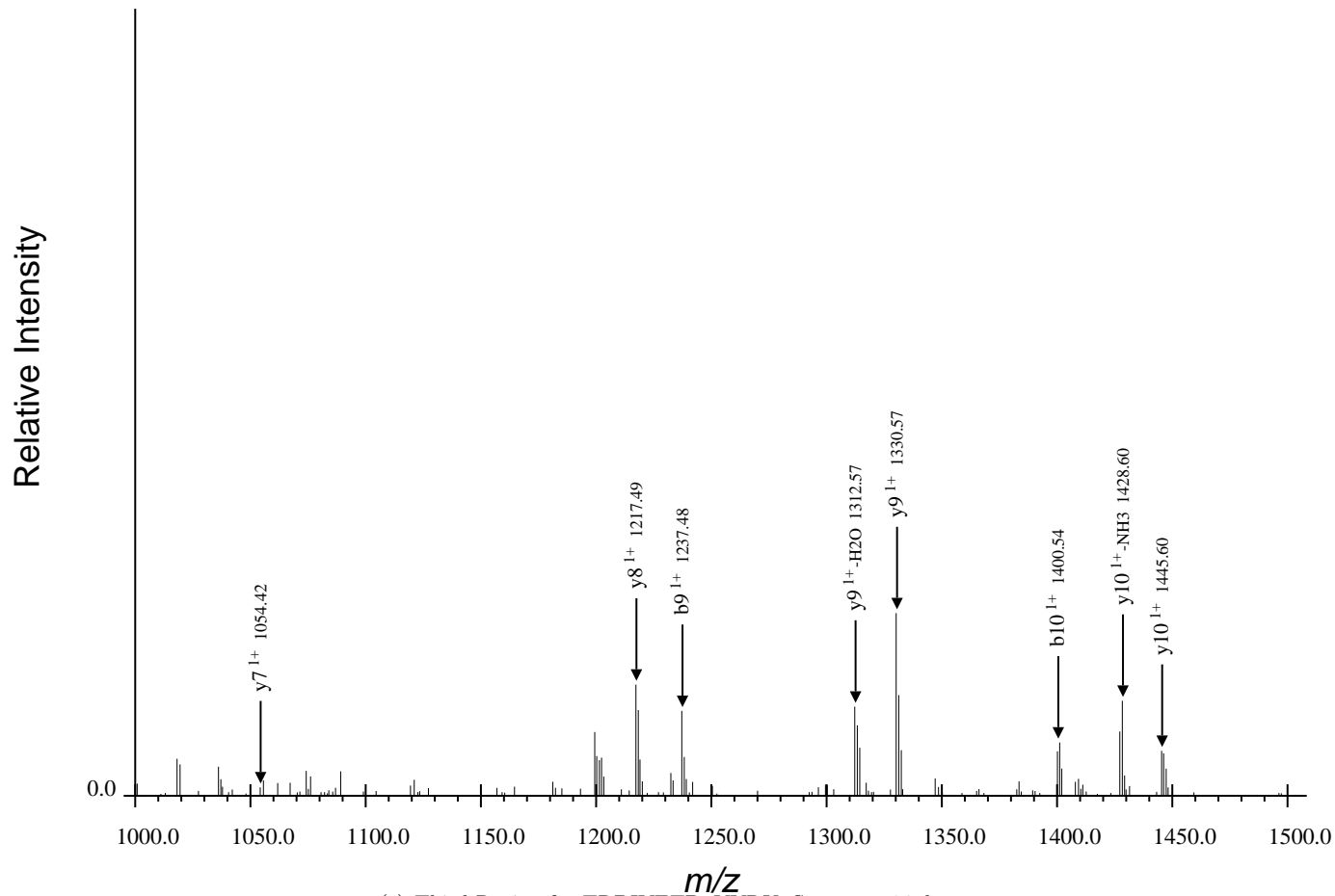
(c) Third Region for TRDIYETDpYYRK, Spectrum 36.dta
