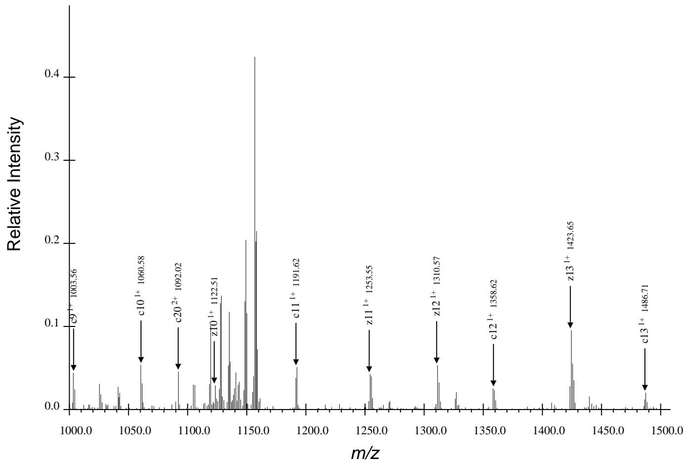
(c) Third Region for SFVLNPTNIGMpSKSSQGHVTK, Spectrum 29.dta
