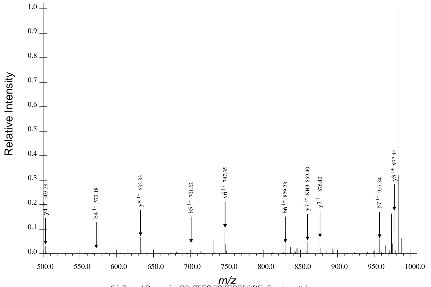
(b) Second Region for FQpSEEQQQTEDELQDK, Spectrum 9.dta
