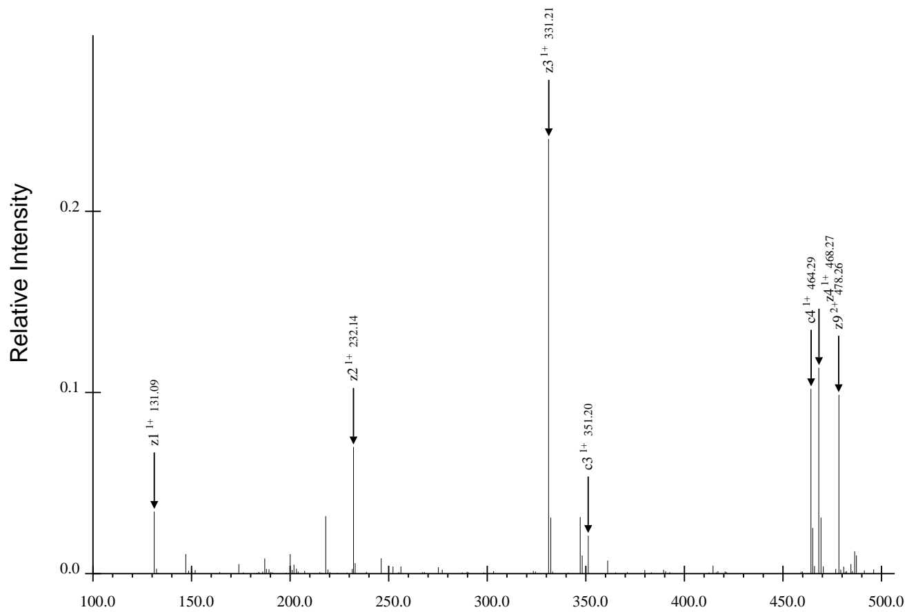
(a) First Region for SFVLNPTNIGMpSKSSQGHVTK, Spectrum 27.dta
