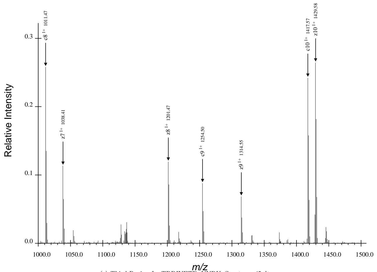
(c) Third Region for TRDIYETDpYYRK, Spectrum 45.dta
