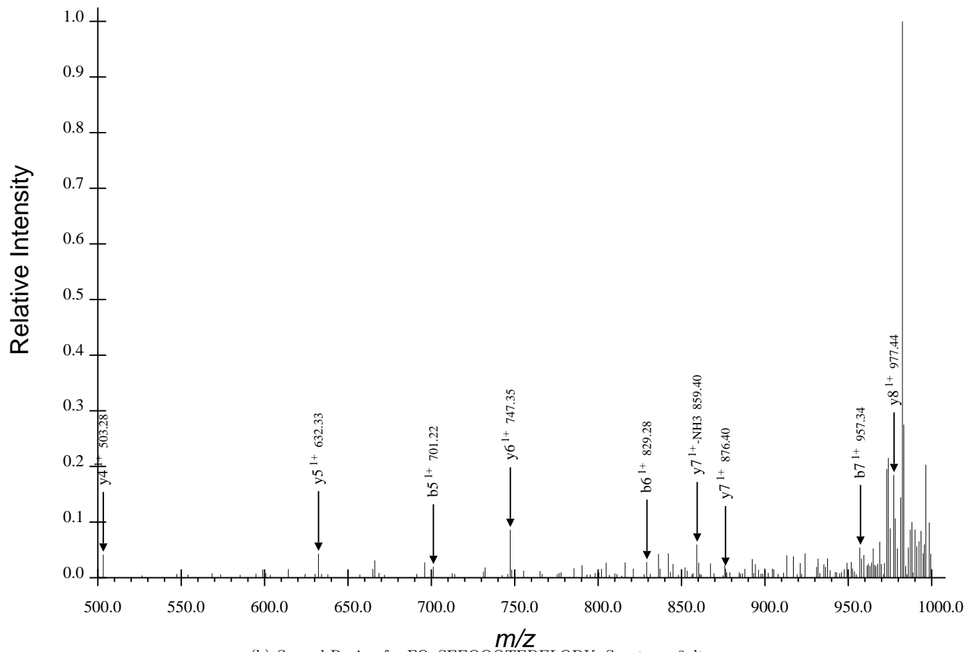
(b) Second Region for FQpSEEQQQTEDELQDK, Spectrum 6.dta
