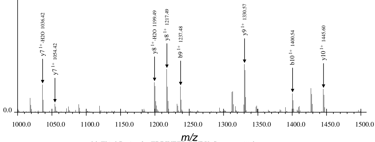
(c) Third Region for TRDIYETDpYYRK, Spectrum 35.dta
