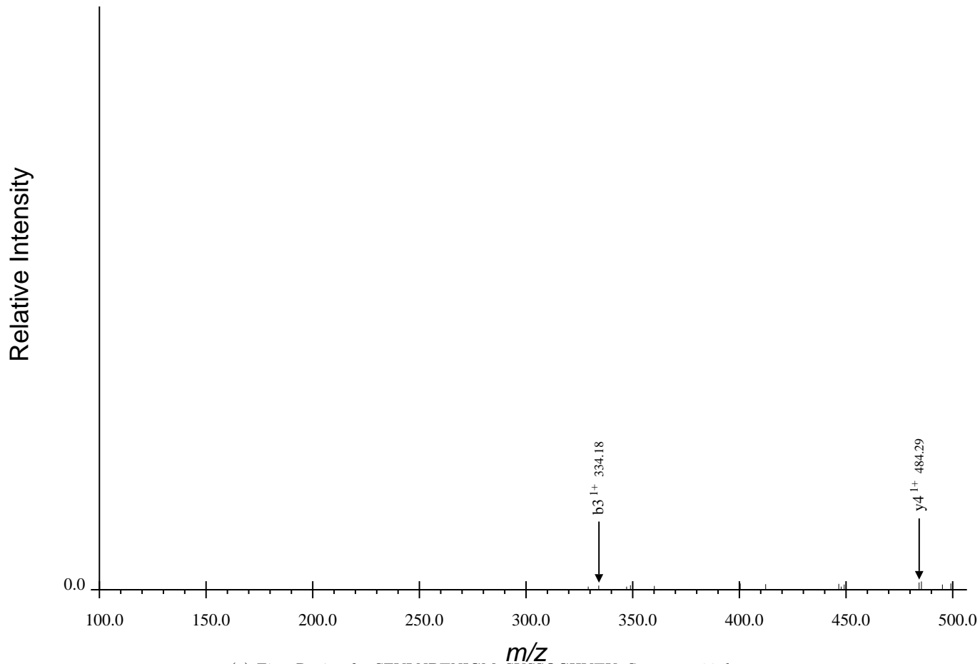
(a) First Region for SFVLNPTNIGMpSKSSQGHVTK, Spectrum 20.dta
