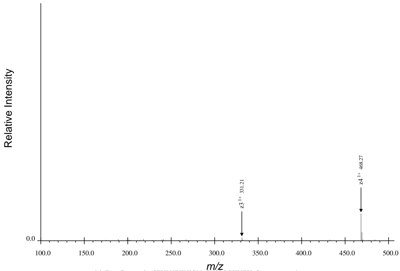
(a) First Region for SFVLNPTNIGMpSKSSQGHVTK, Spectrum 26.dta
