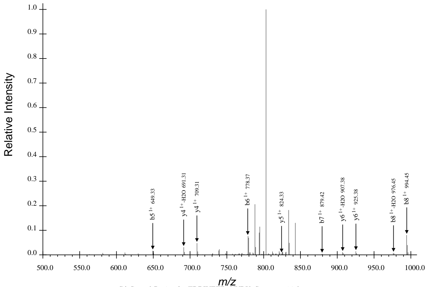
(b) Second Region for TRDIYETDpYYRK, Spectrum 34.dta
