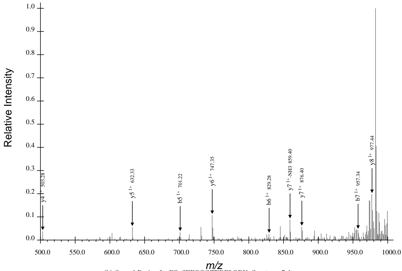
(b) Second Region for FQpSEEQQQTEDELQDK, Spectrum 7.dta
