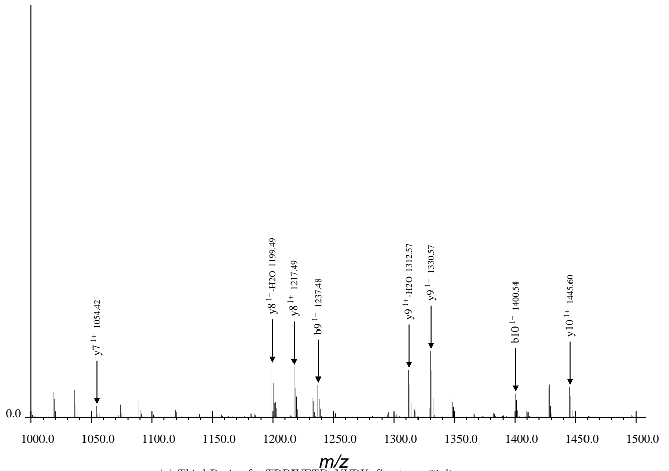
(c) Third Region for TRDIYETDpYYRK, Spectrum 32.dta
