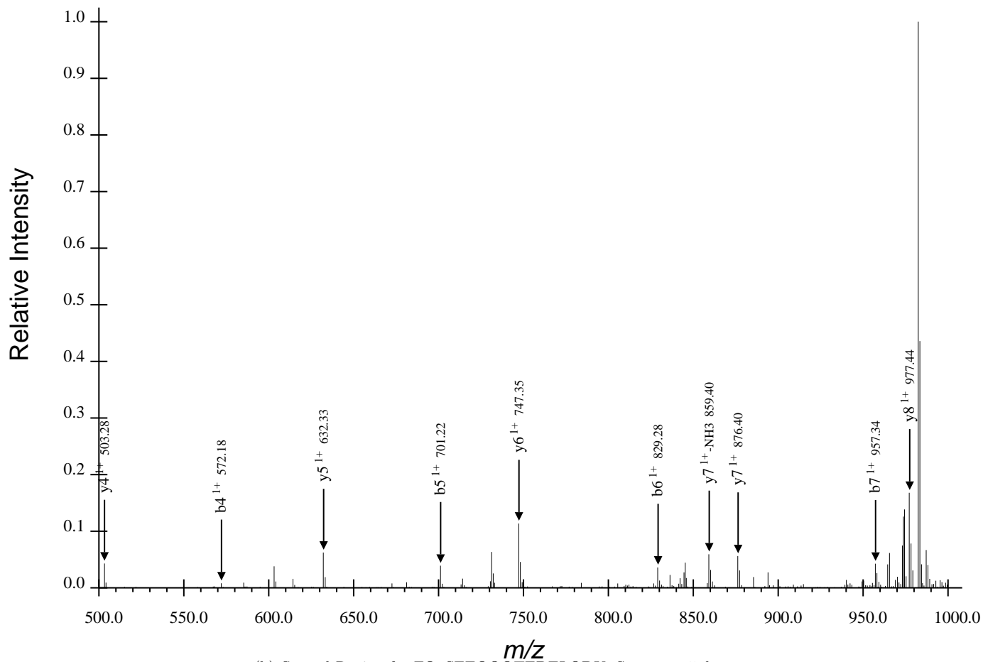
(b) Second Region for FQpSEEQQQTEDELQDK, Spectrum 5.dta
