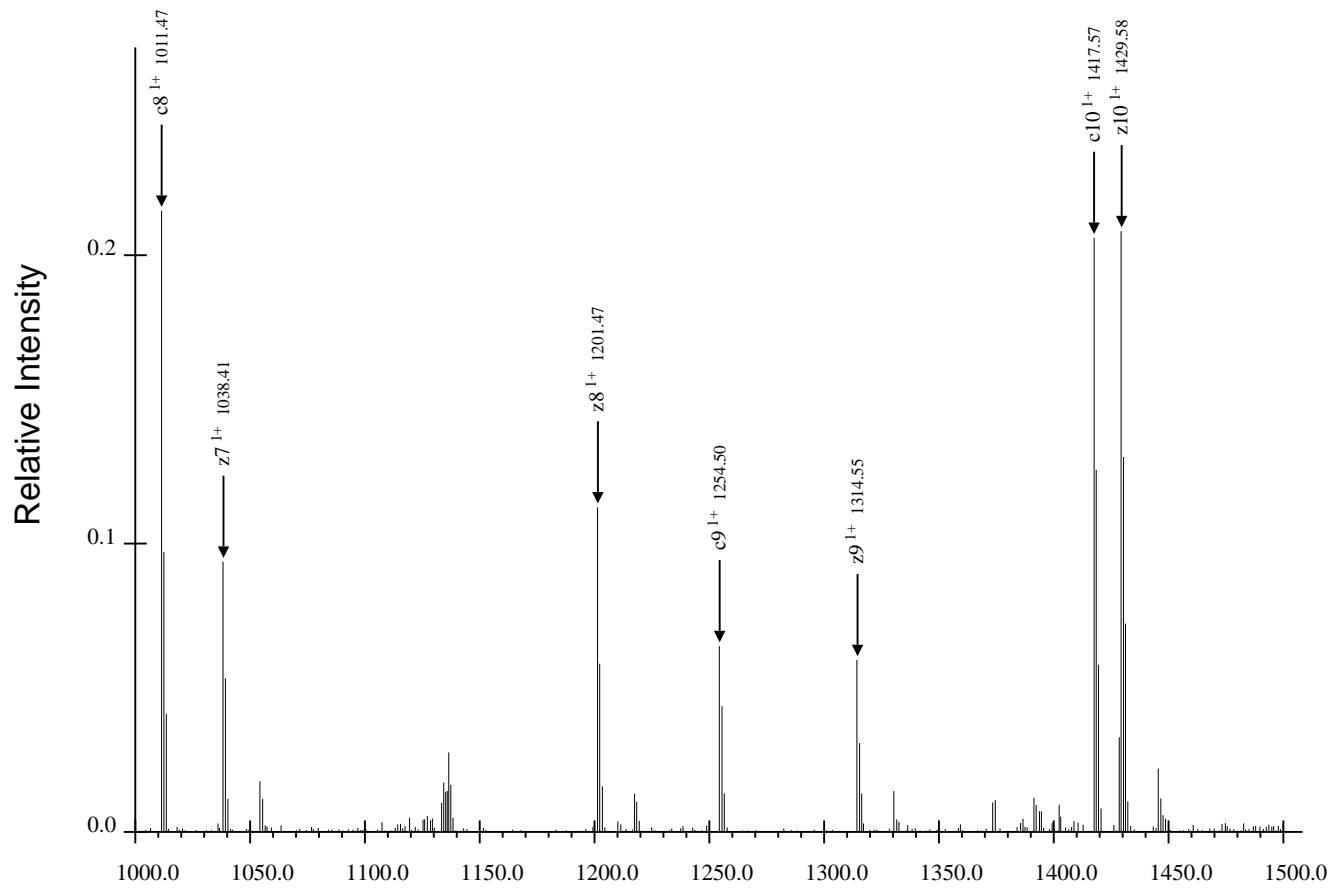
(c) Third Region for TRDIYETDpYYRK, Spectrum 47.dta
