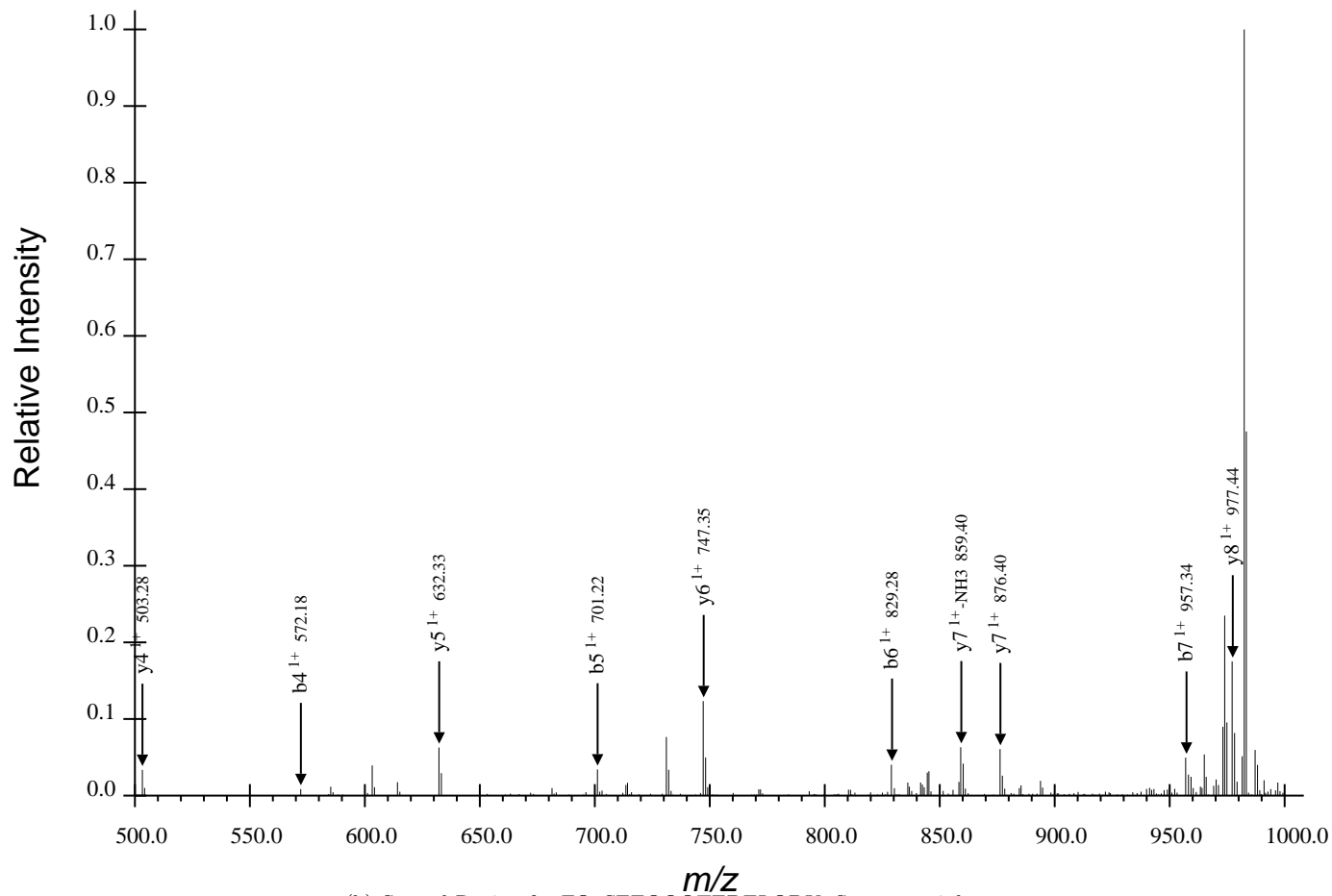
(b) Second Region for FQpSEEQQQTEDELQDK, Spectrum 4.dta
