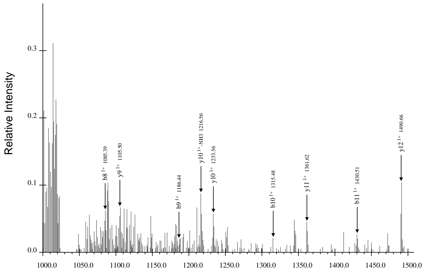
(c) Third Region for FQpSEEQQQTEDELQDK, Spectrum 7.dta
