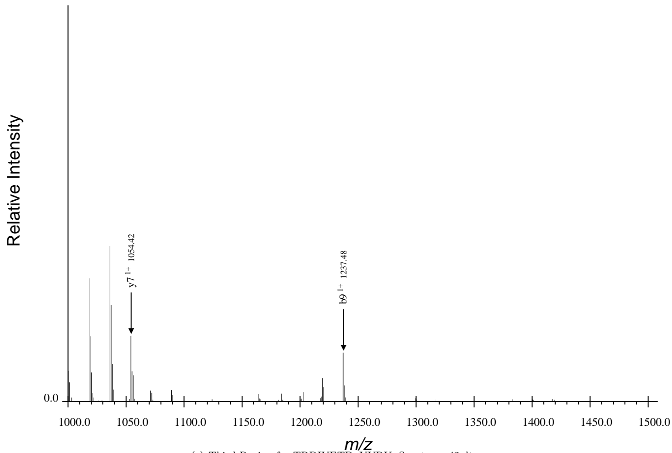
(c) Third Region for TRDIYETDpYYRK, Spectrum 42.dta
