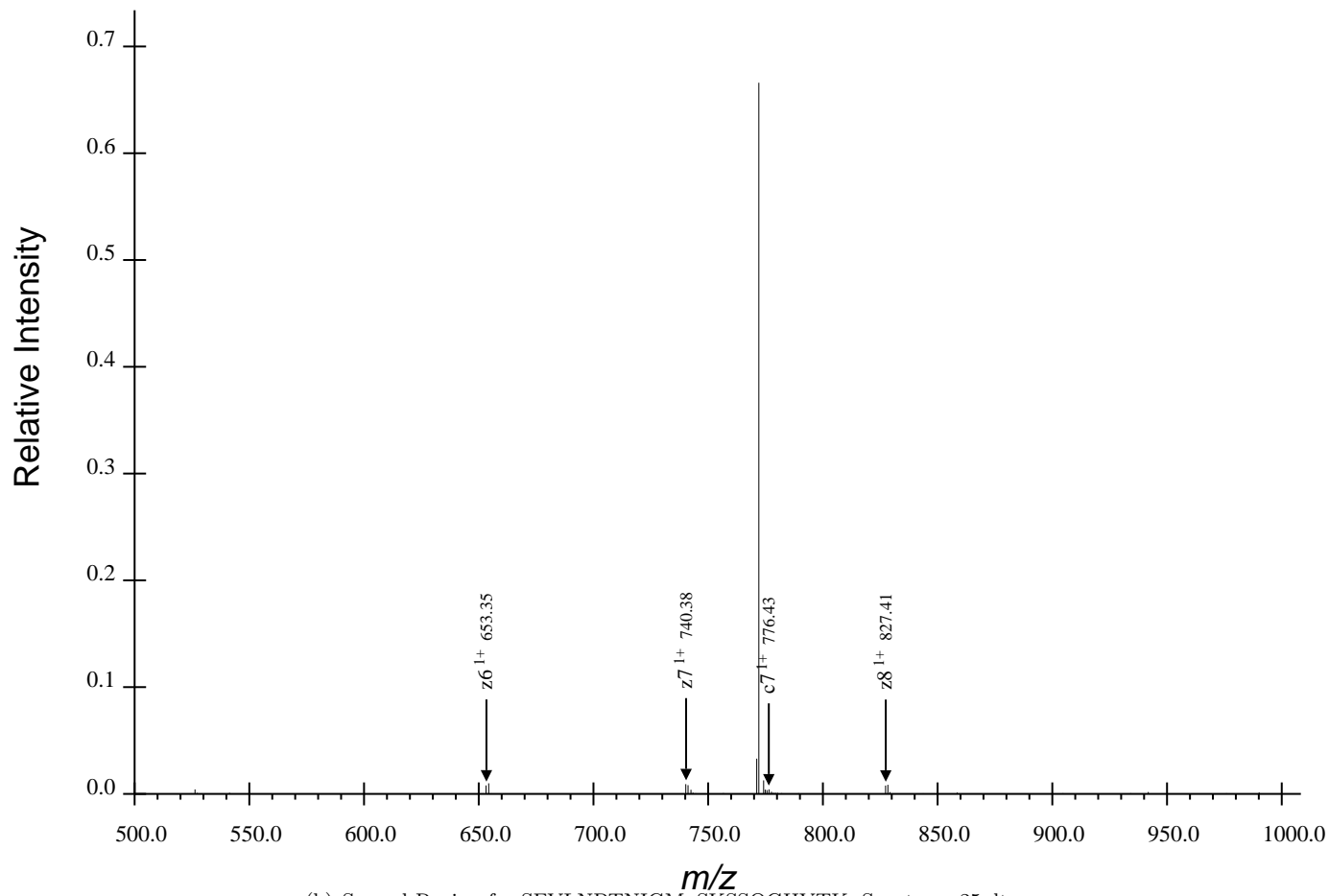
(b) Second Region for SFVLNPTNIGMpSKSSQGHVTK, Spectrum 25.dta
