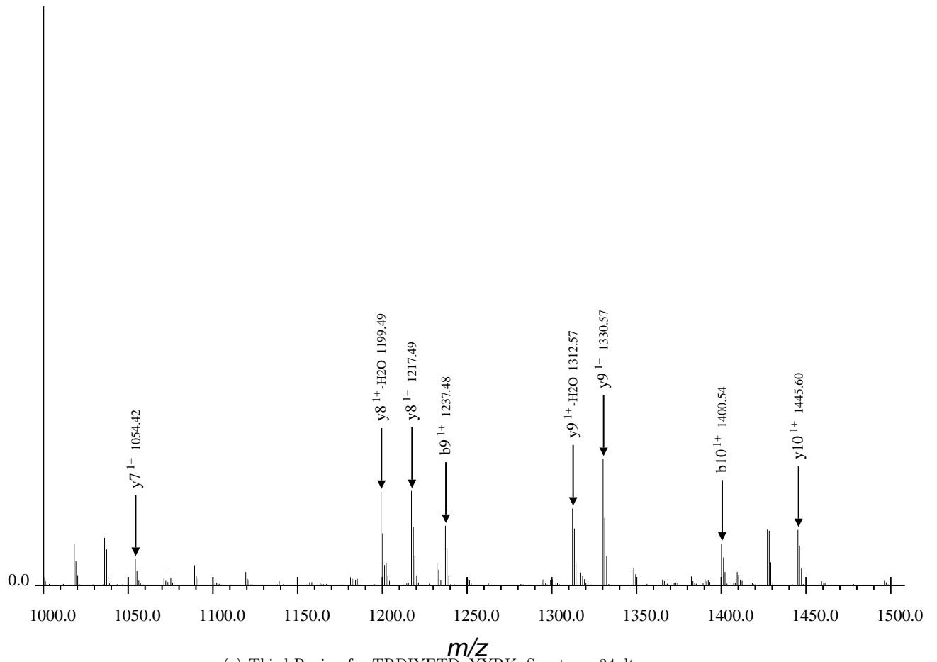
(c) Third Region for TRDIYETDpYYRK, Spectrum 34.dta
