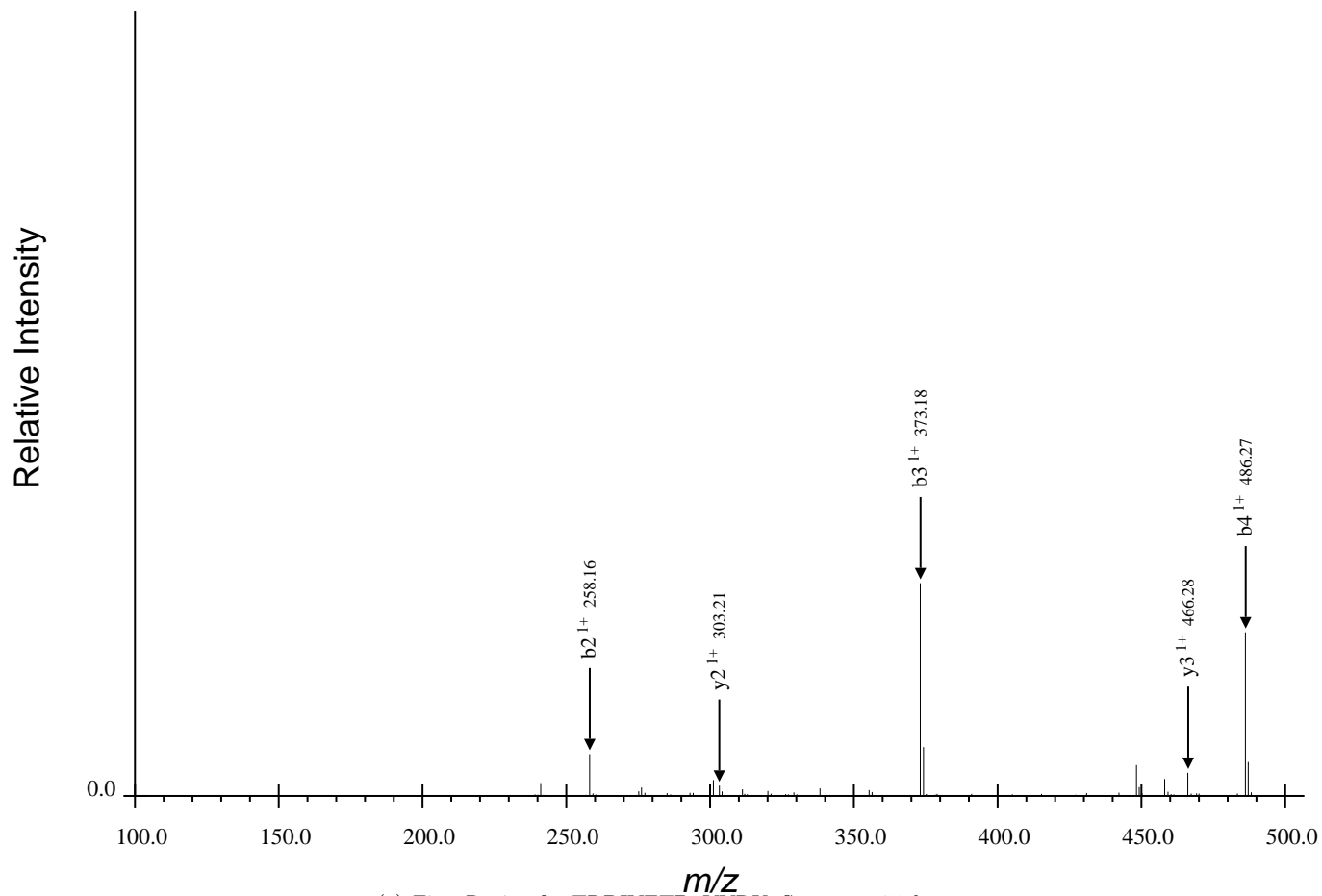
(a) First Region for TRDIYETDpYYRK, Spectrum 35.dta
