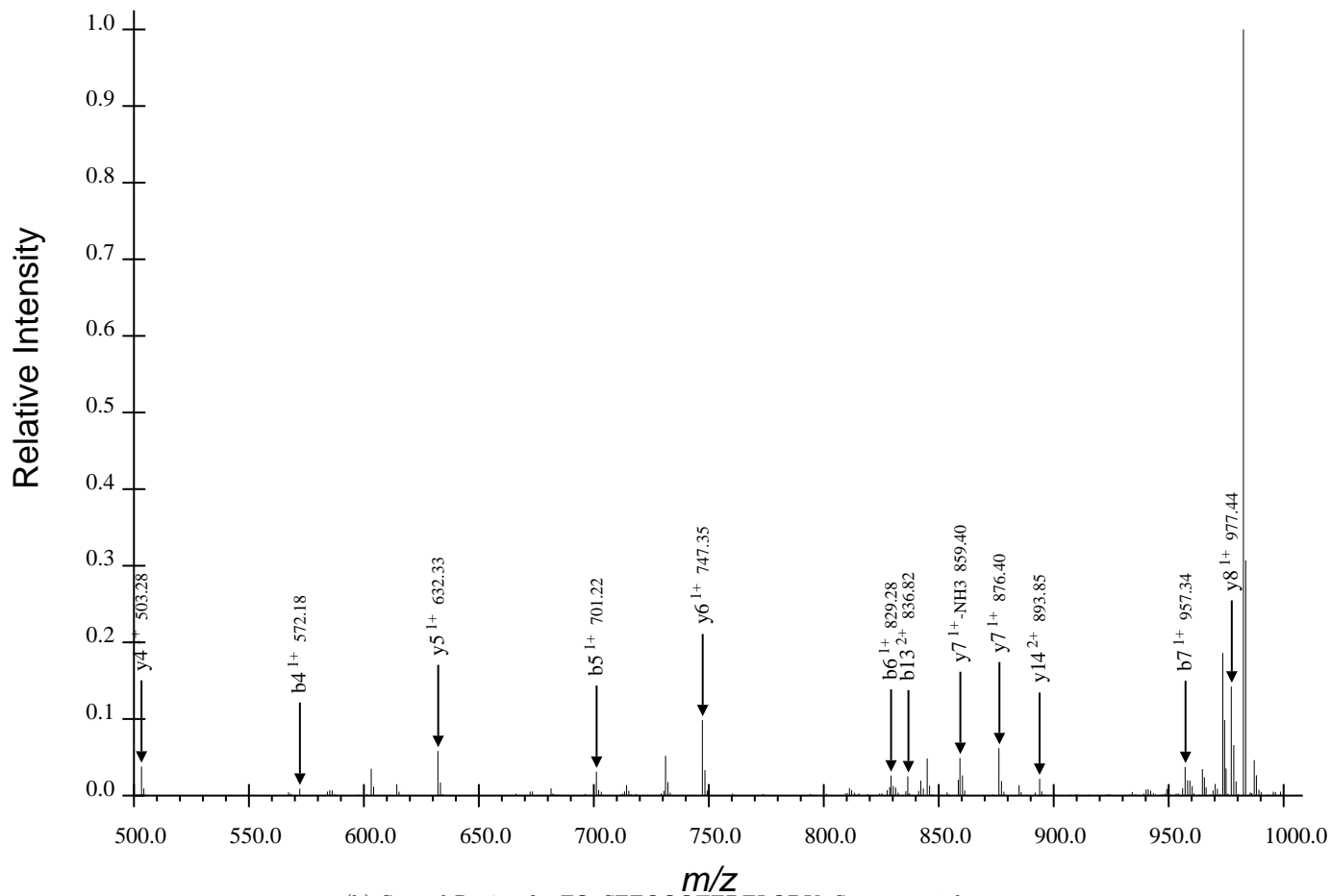
(b) Second Region for FQpSEEQQQTEDELQDK, Spectrum 1.dta
