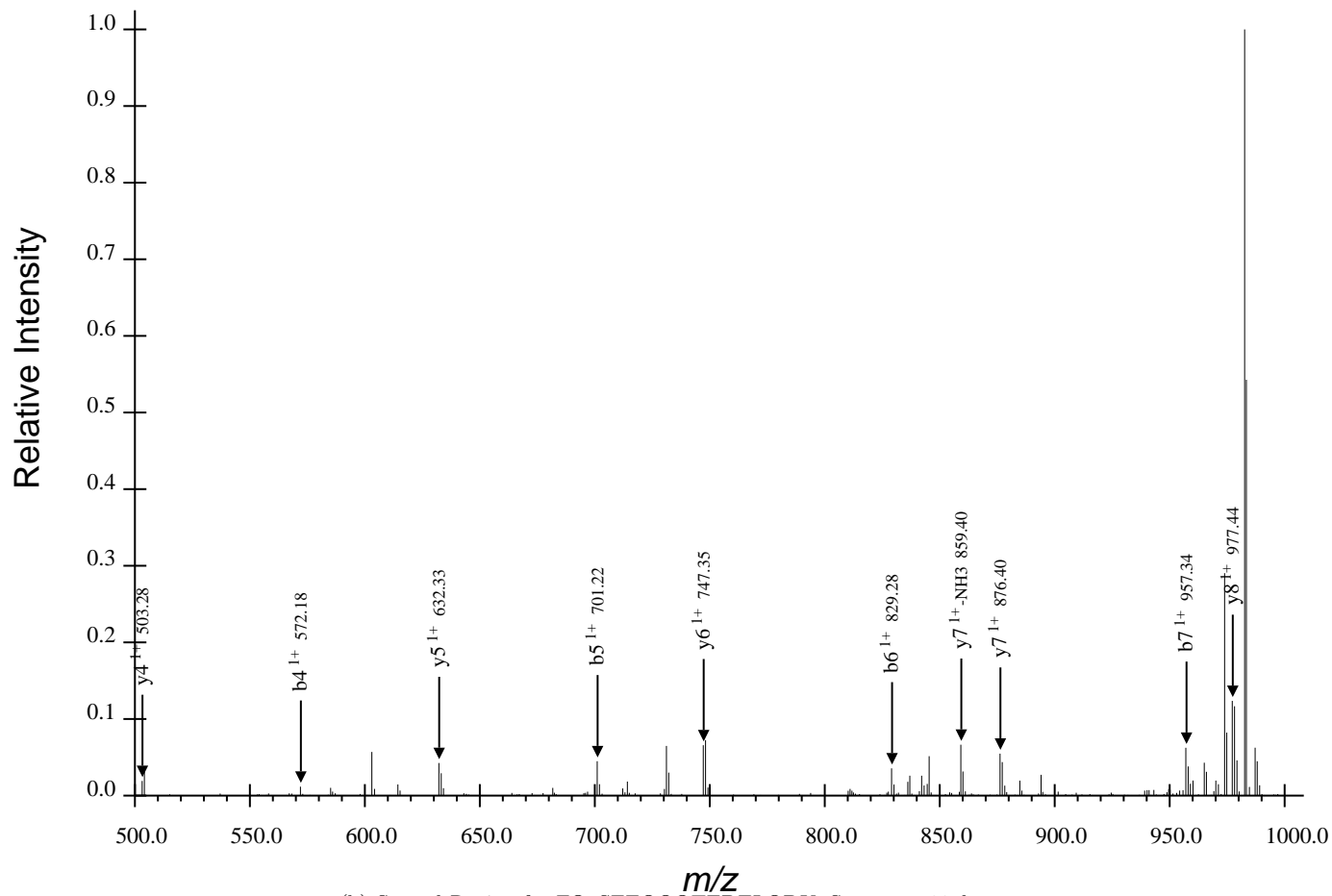
(b) Second Region for FQpSEEQQQTEDELQDK, Spectrum 11.dta
