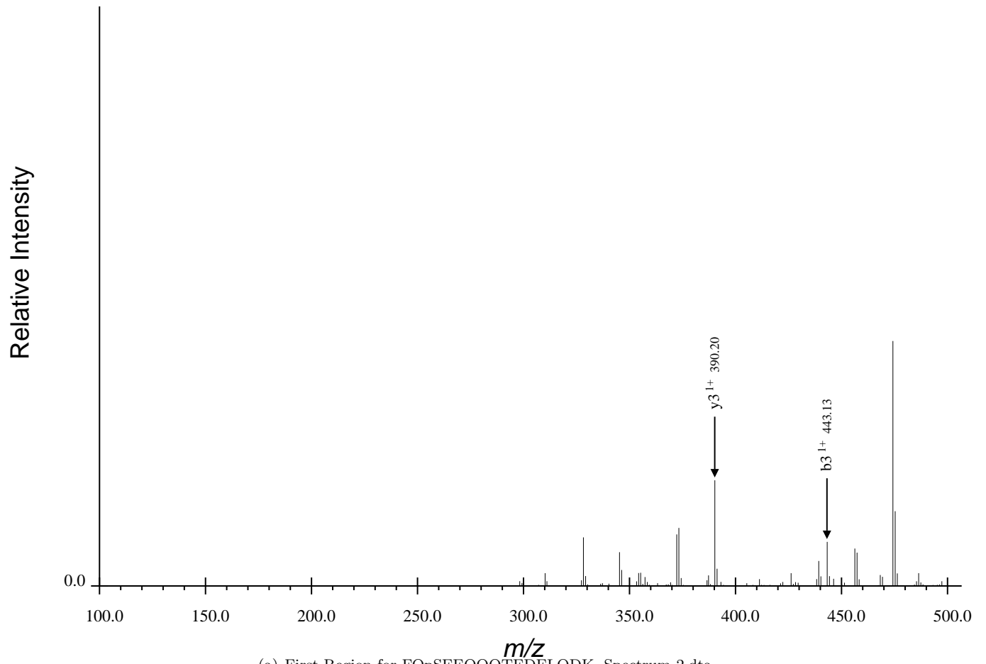
(a) First Region for FQpSEEQQQTEDELQDK, Spectrum 2.dta
