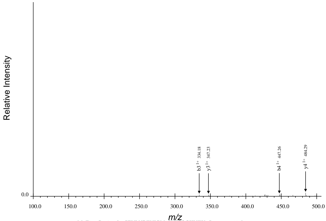
(a) First Region for SFVLNPTNIGMpSKSSQGHVTK, Spectrum 19.dta
