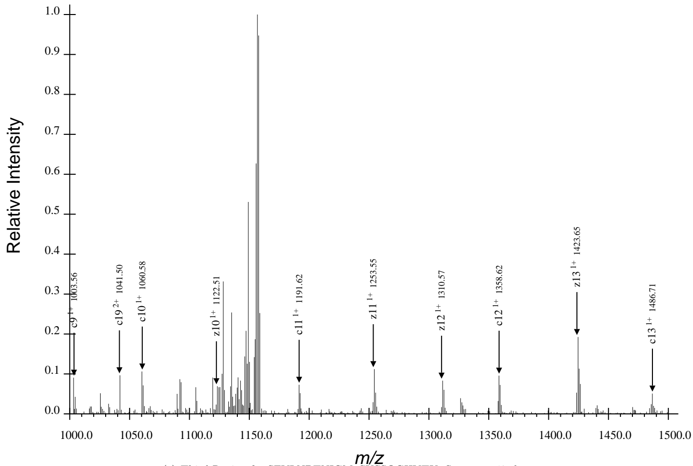
(c) Third Region for SFVLNPTNIGMpSKSSQGHVTK, Spectrum 27.dta
