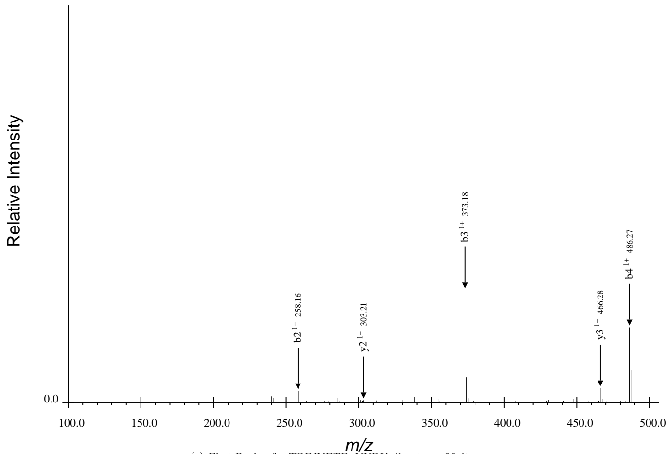
(a) First Region for TRDIYETDpYYRK, Spectrum 36.dta
