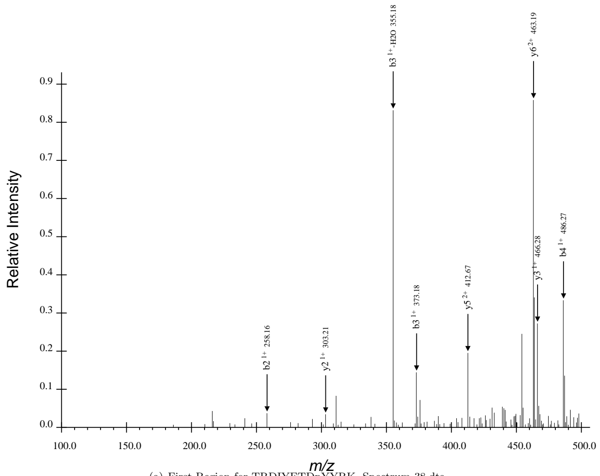
(a) First Region for TRDIYETDpYYRK, Spectrum 38.dta
