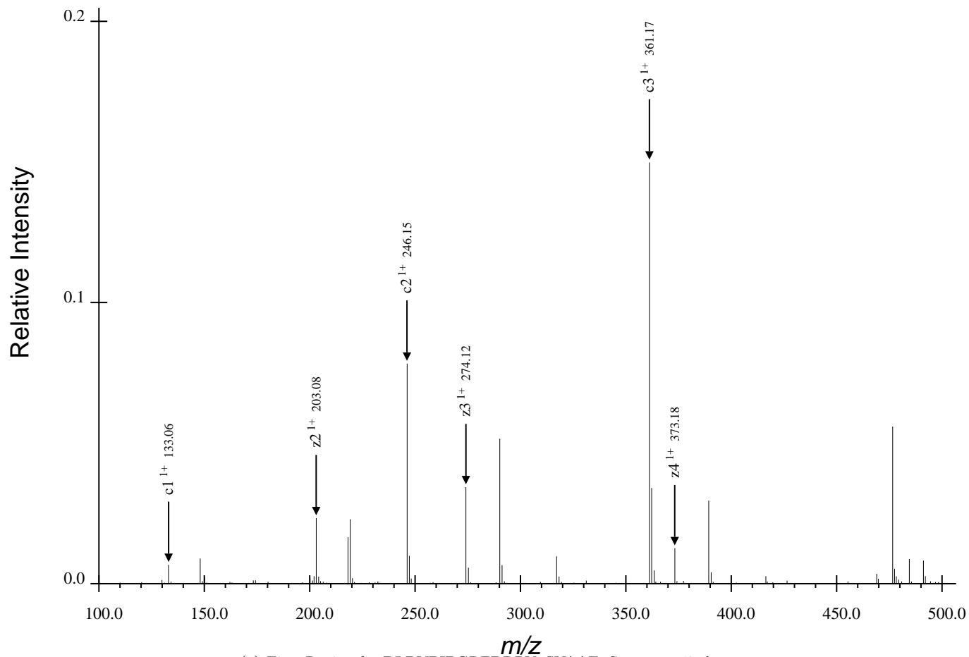
(a) First Region for DLDVPIPGRFDRRVpSVA AE, Spectrum 17.dta
