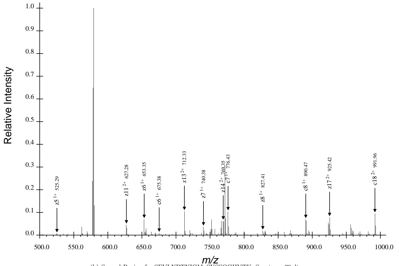
(b) Second Region for SFVLNPTNIGMpSKSSQGHVTK, Spectrum 29.dta
