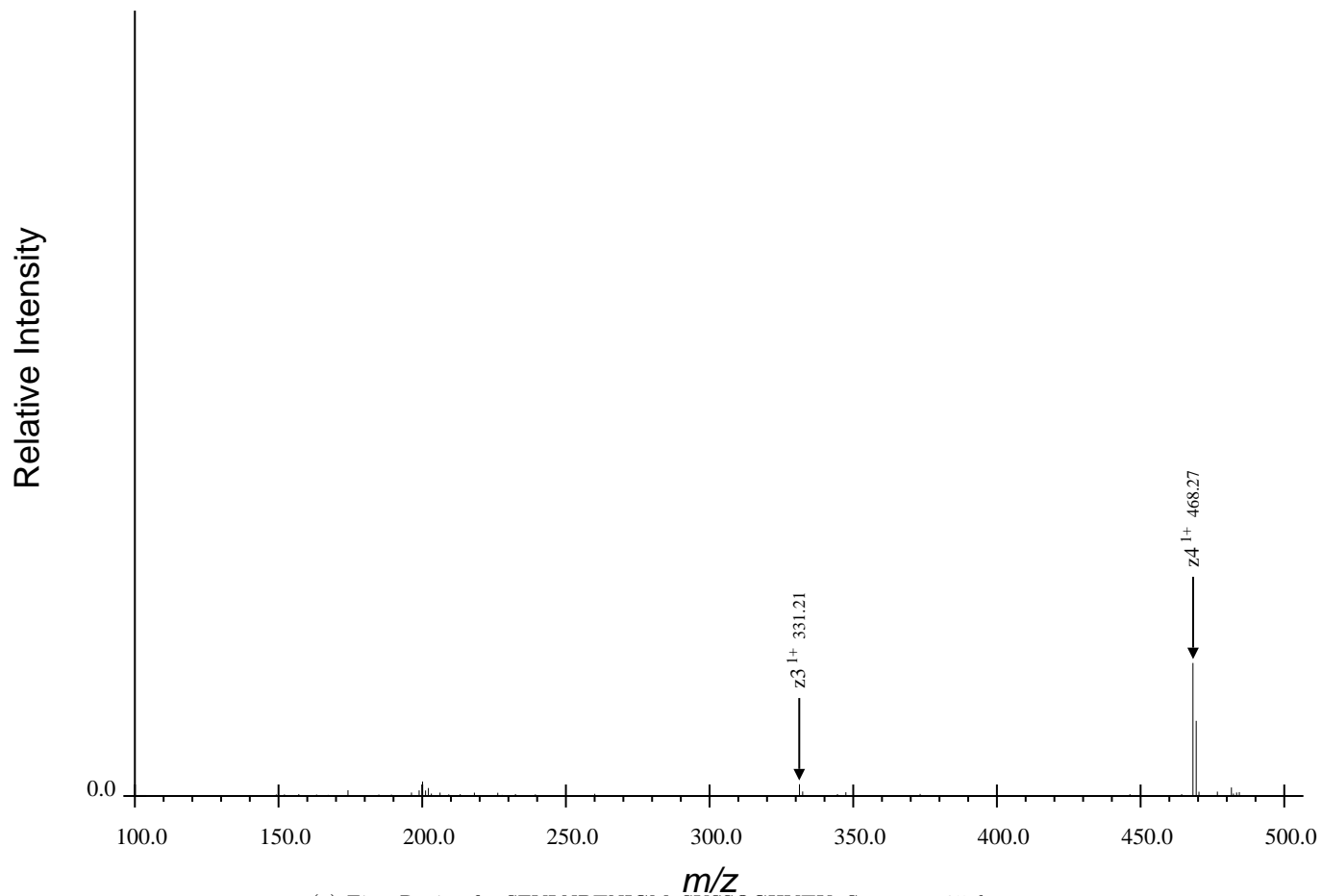
(a) First Region for SFVLNPTNIGMpSKSSQGHVTK, Spectrum 25.dta
