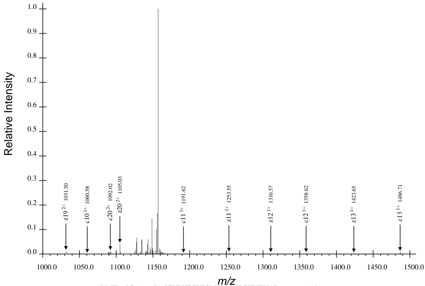
(c) Third Region for SFVLNPTNIGMpSKSSQGHVTK, Spectrum 26.dta
