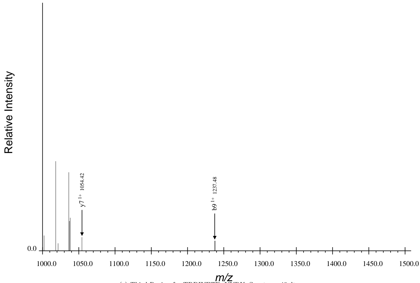
(c) Third Region for TRDIYETDpYYRK, Spectrum 43.dta
