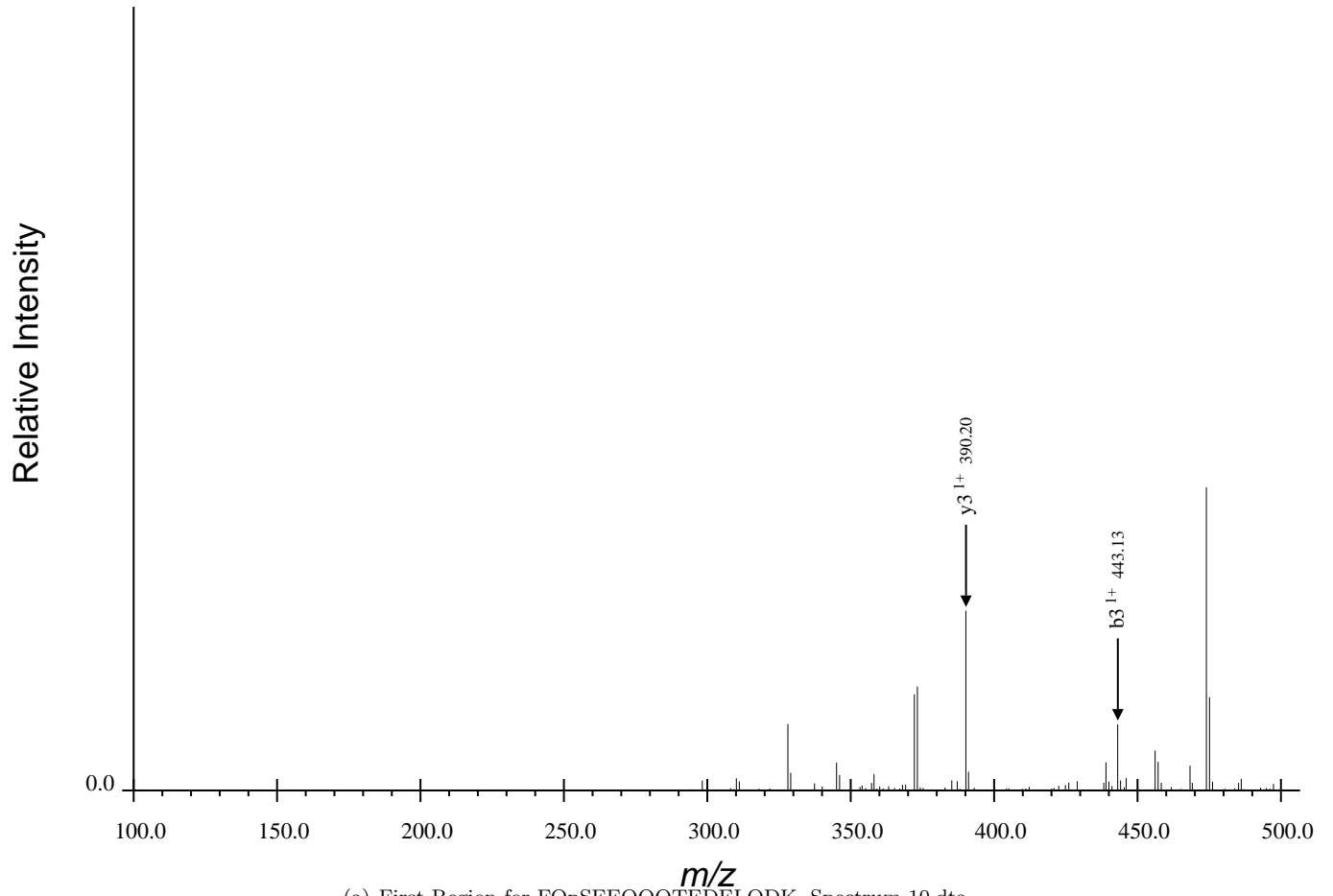
(a) First Region for FQpSEEQQQTEDELQDK, Spectrum 10.dta
