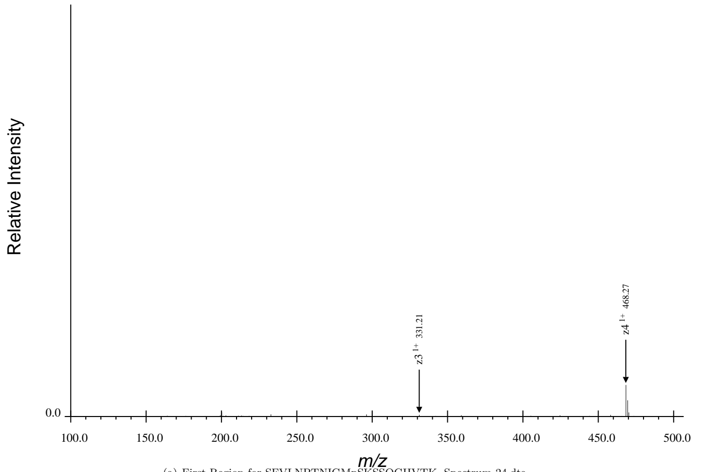
(a) First Region for SFVLNPTNIGMpSKSSQGHVTK, Spectrum 24.dta
