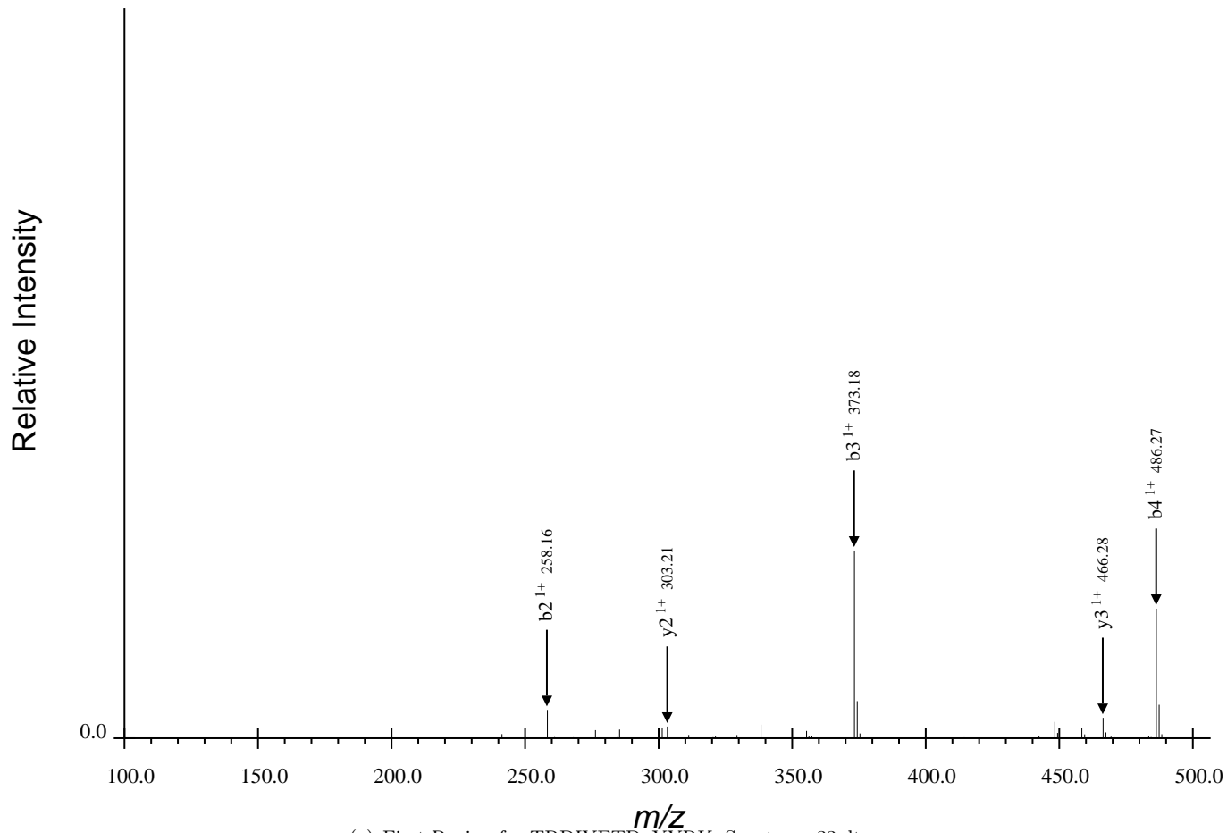
(a) First Region for TRDIYETDpYYRK, Spectrum 33.dta
