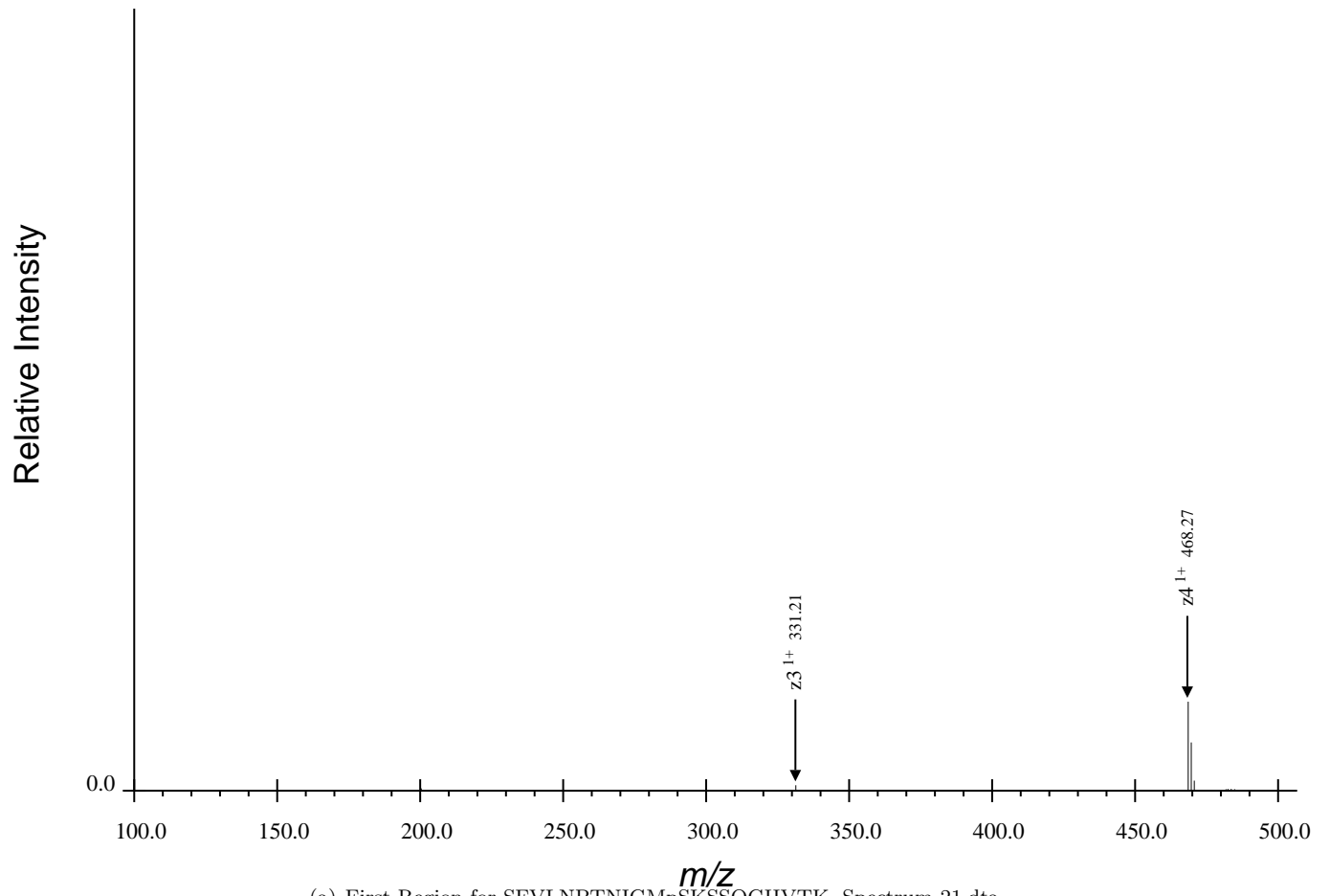
(a) First Region for SFVLNPTNIGMpSKSSQGHVTK, Spectrum 21.dta
