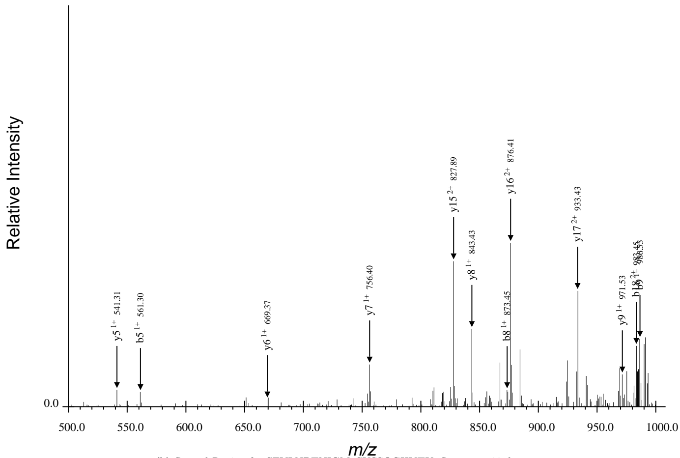
(b) Second Region for SFVLNPTNIGMpSKSSQGHVTK, Spectrum 20.dta
