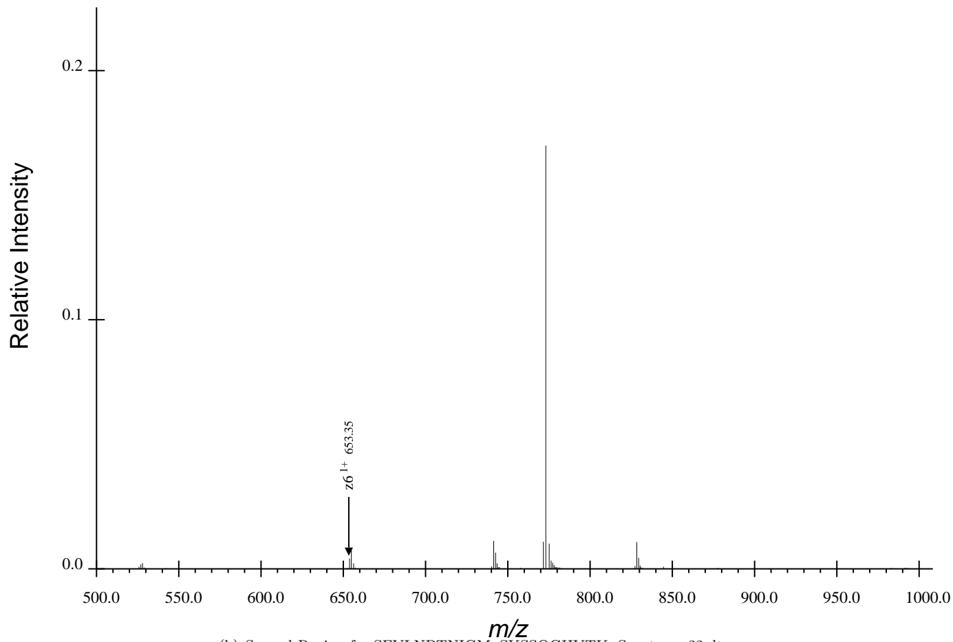
(b) Second Region for SFVLNPTNIGMpSKSSQGHVTK, Spectrum 22.dta
