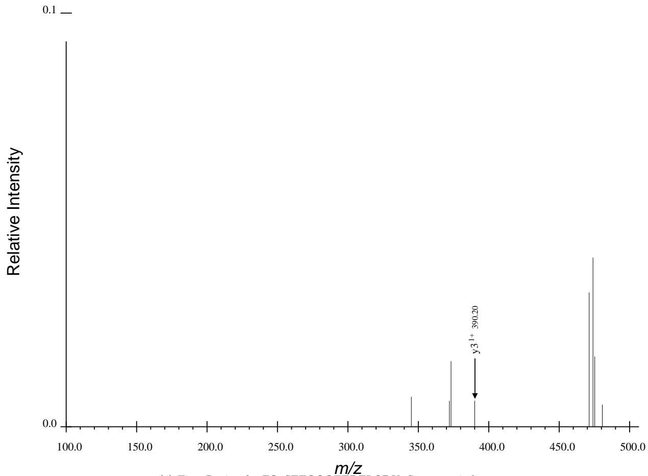
(a) First Region for FQpSEEQQQTEDELQDK, Spectrum 7.dta
