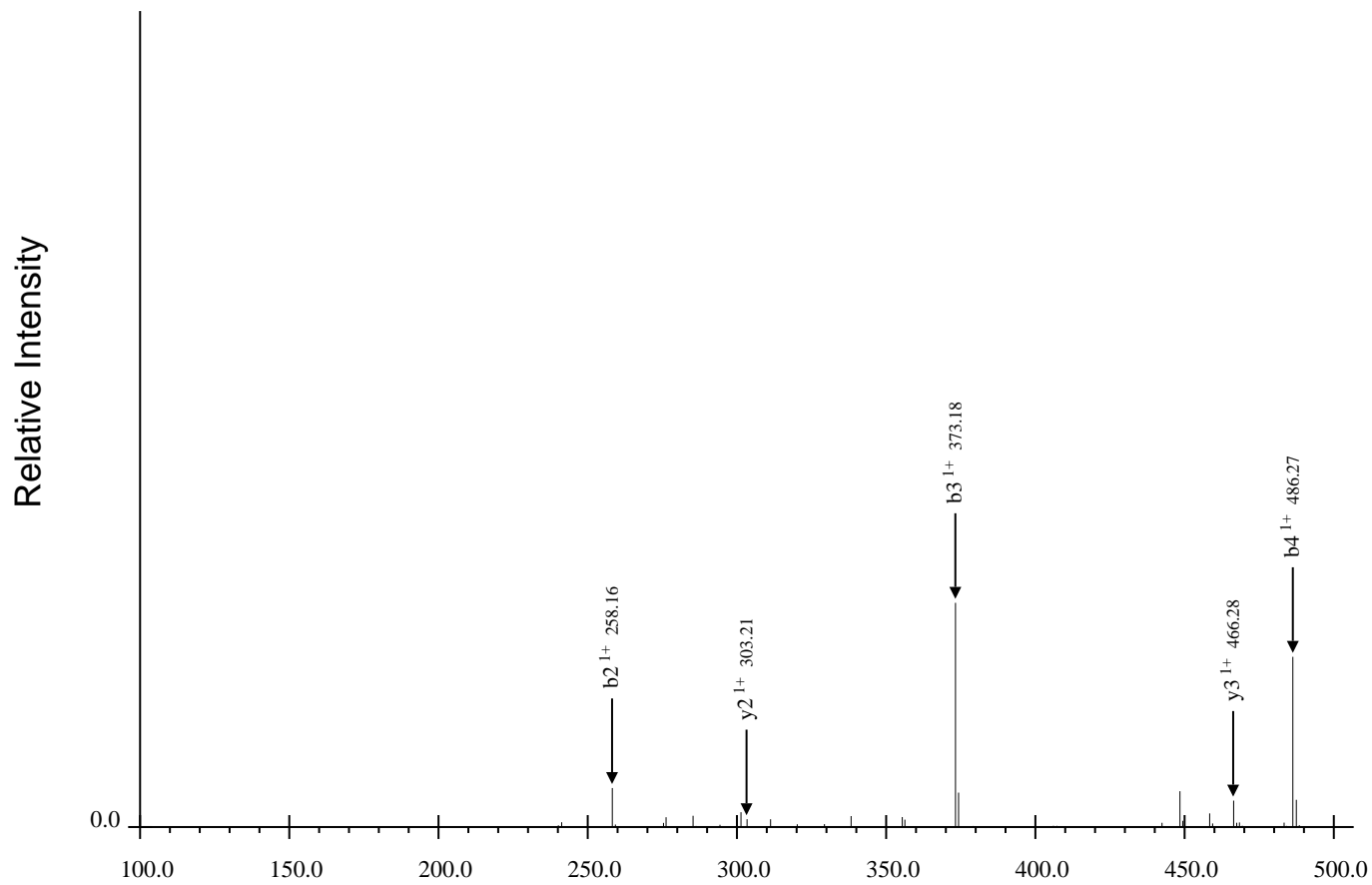
(a) First Region for TRDIYETDpYYRK, Spectrum 30.dta
