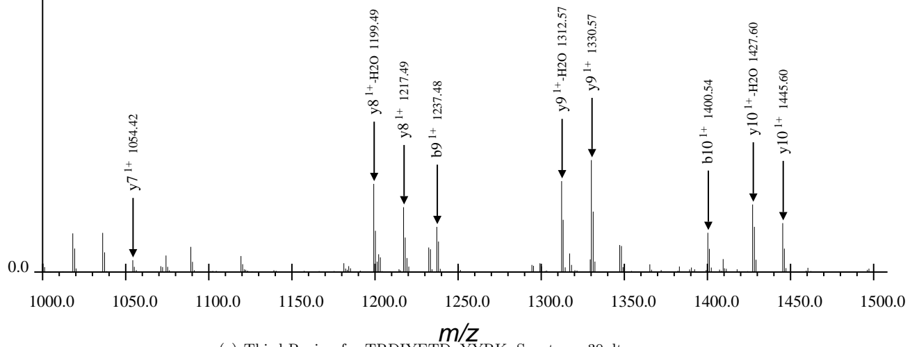
(c) Third Region for TRDIYETDpYYRK, Spectrum 30.dta
