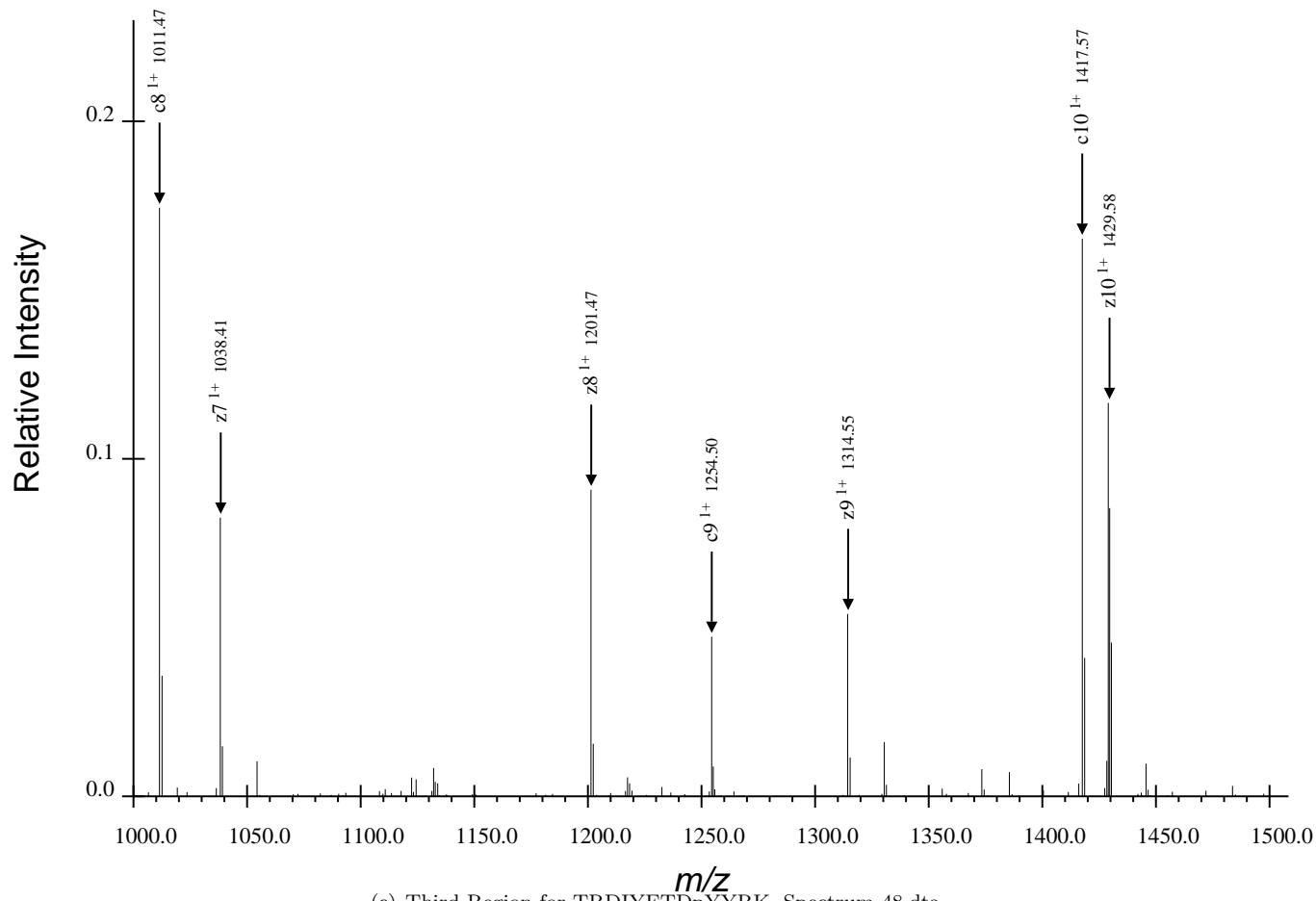
(c) Third Region for TRDIYETDpYYRK, Spectrum 48.dta
