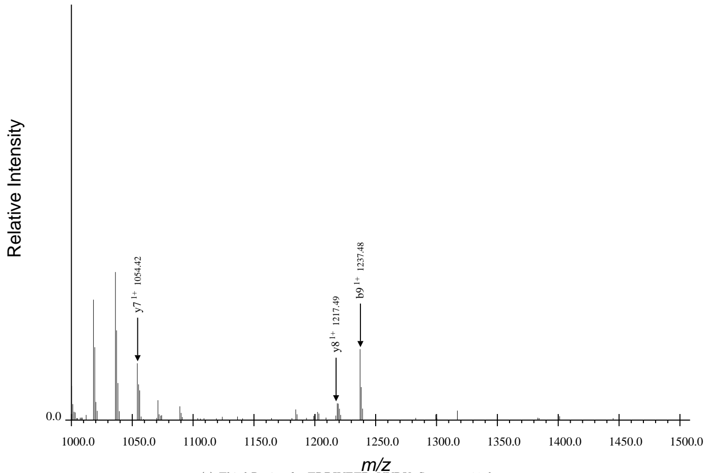
(c) Third Region for TRDIYETDpYYRK, Spectrum 39.dta
