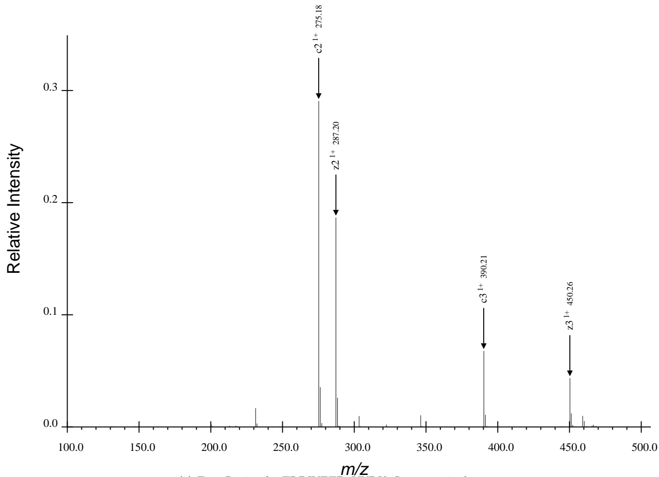
(a) First Region for TRDIYETDpYYRK, Spectrum 45.dta
