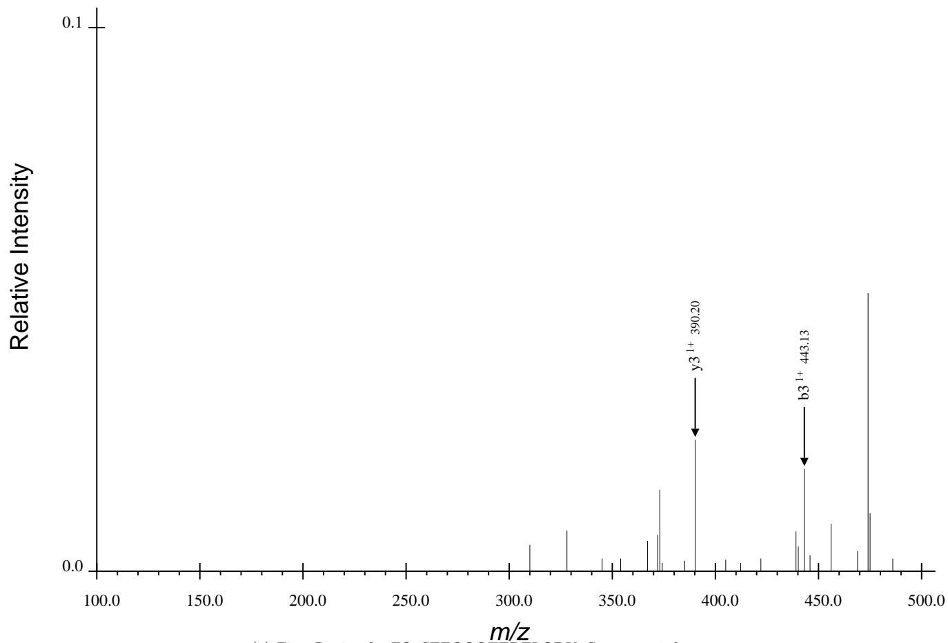
(a) First Region for FQpSEEQQQTEDELQDK, Spectrum 8.dta
