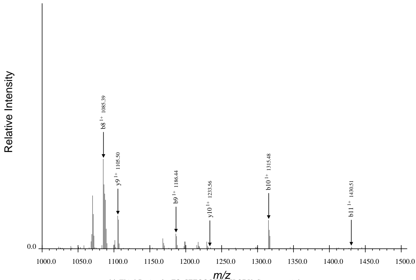
(c) Third Region for FQpSEEQQQTEDELQDK, Spectrum 13.dta
