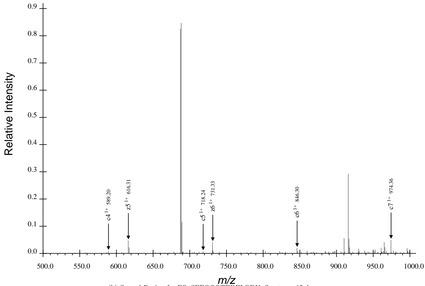
(b) Second Region for FQpSEEQQQTEDELQDK, Spectrum 15.dta
