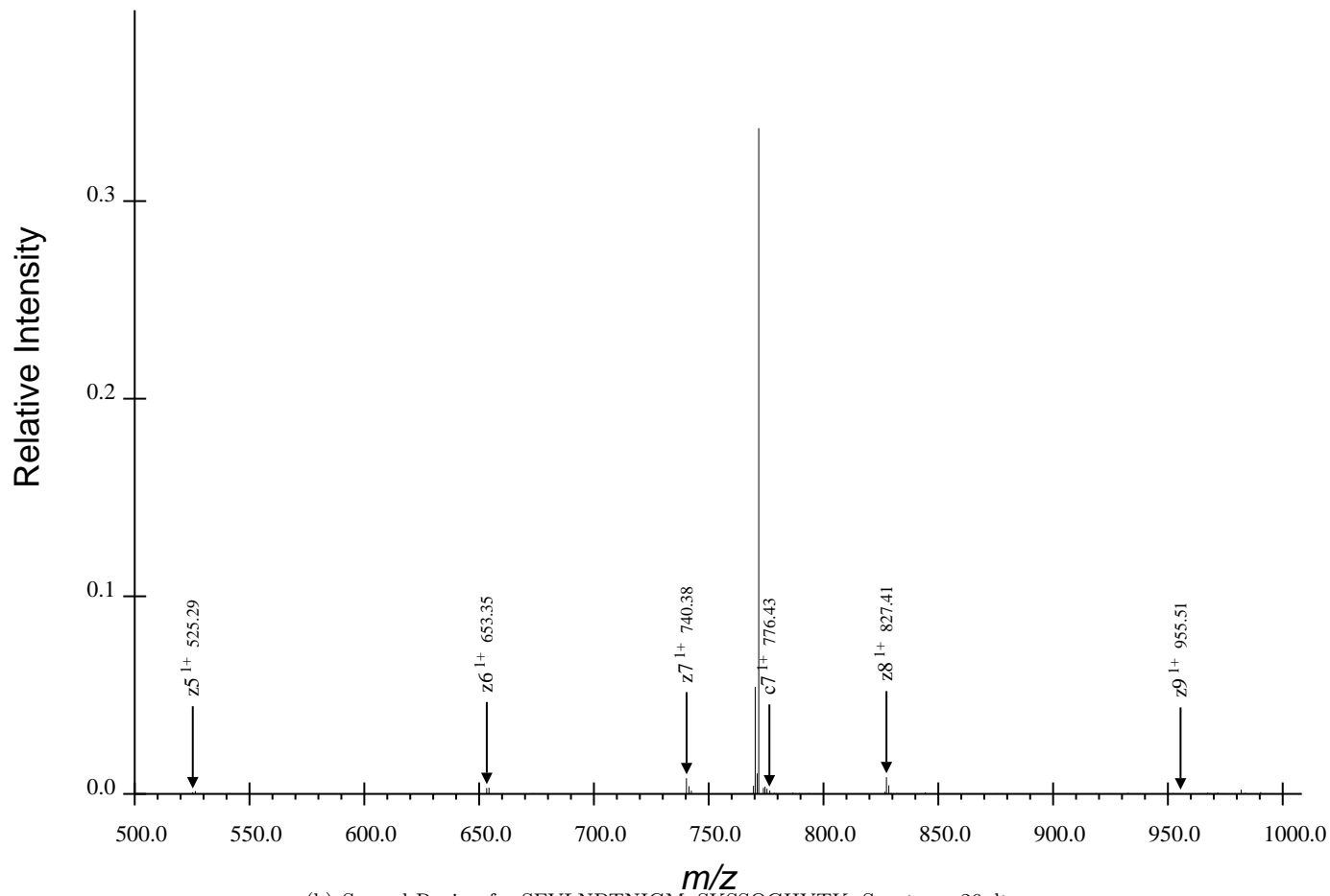
(b) Second Region for SFVLNPTNIGMpSKSSQGHVTK, Spectrum 26.dta
