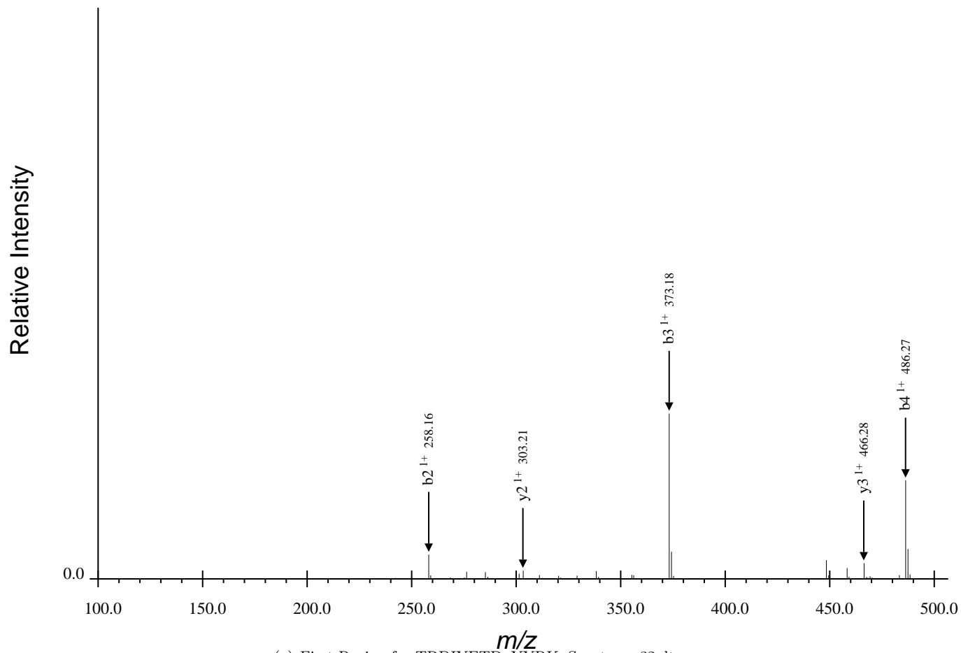
(a) First Region for TRDIYETDpYYRK, Spectrum 32.dta
