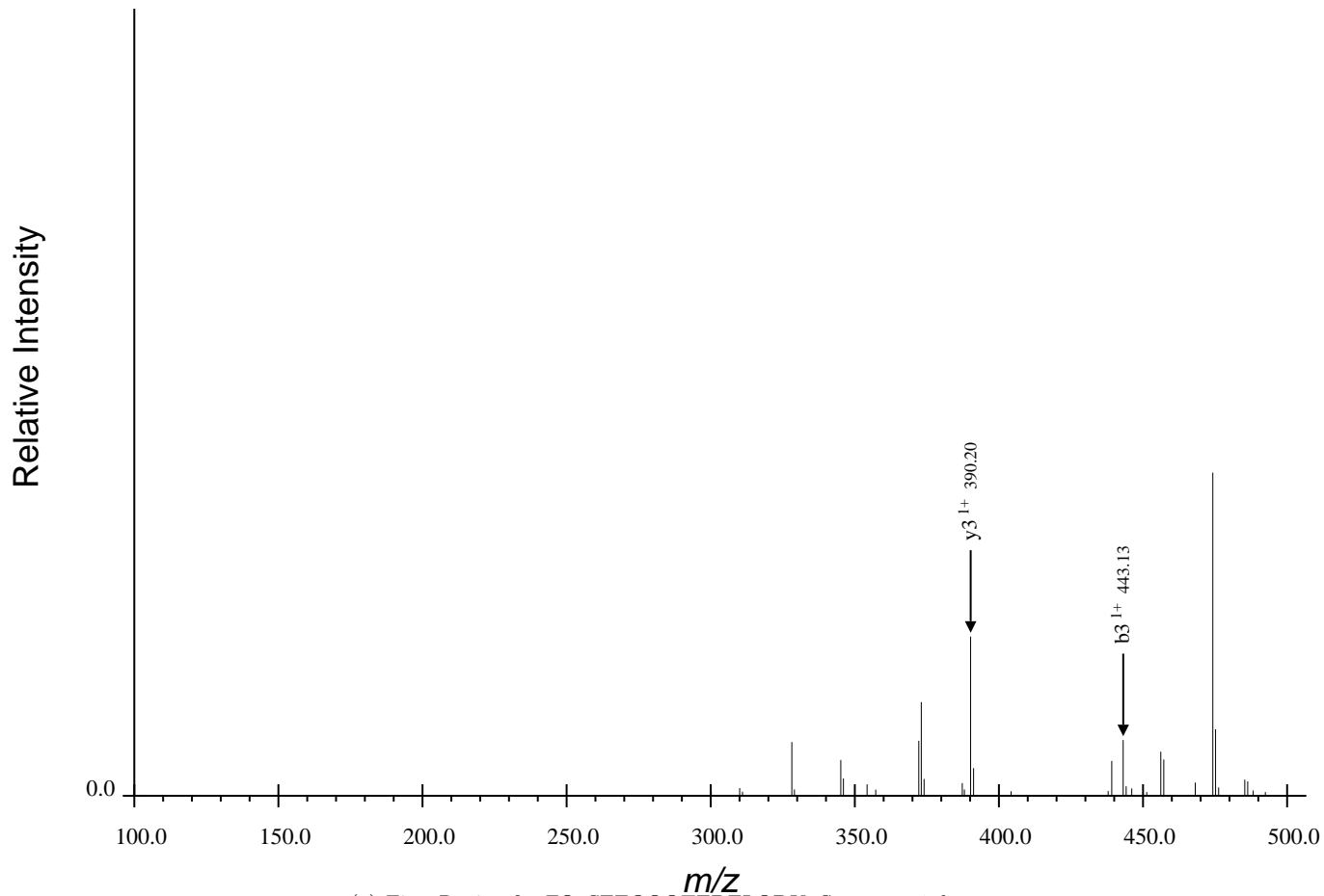
(a) First Region for FQpSEEQQQTEDELQDK, Spectrum 1.dta
