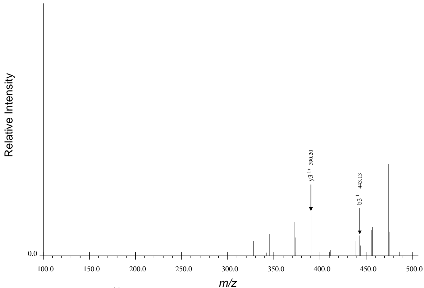
(a) First Region for FQpSEEQQQTEDELQDK, Spectrum 3.dta
