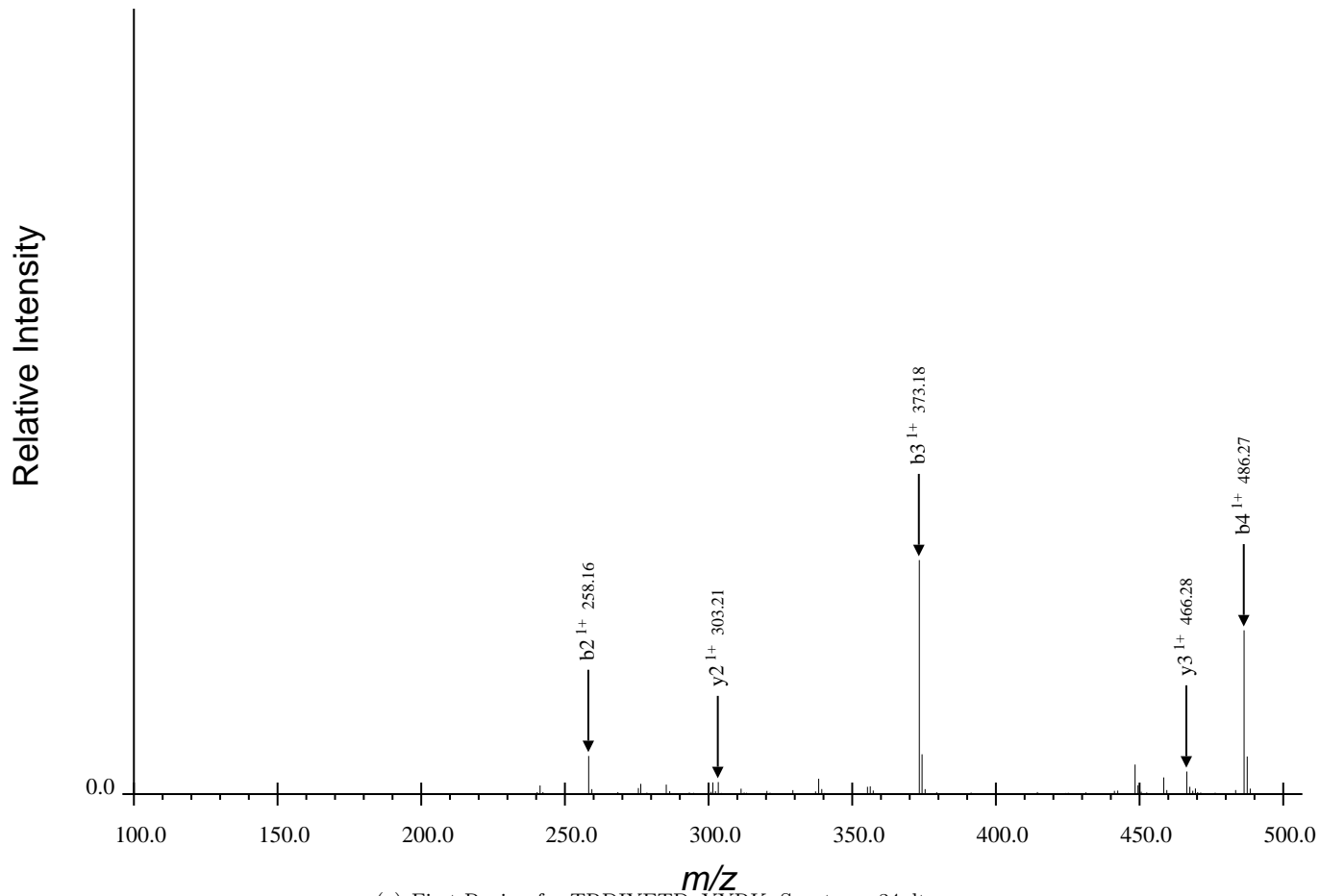
(a) First Region for TRDIYETDpYYRK, Spectrum 34.dta
