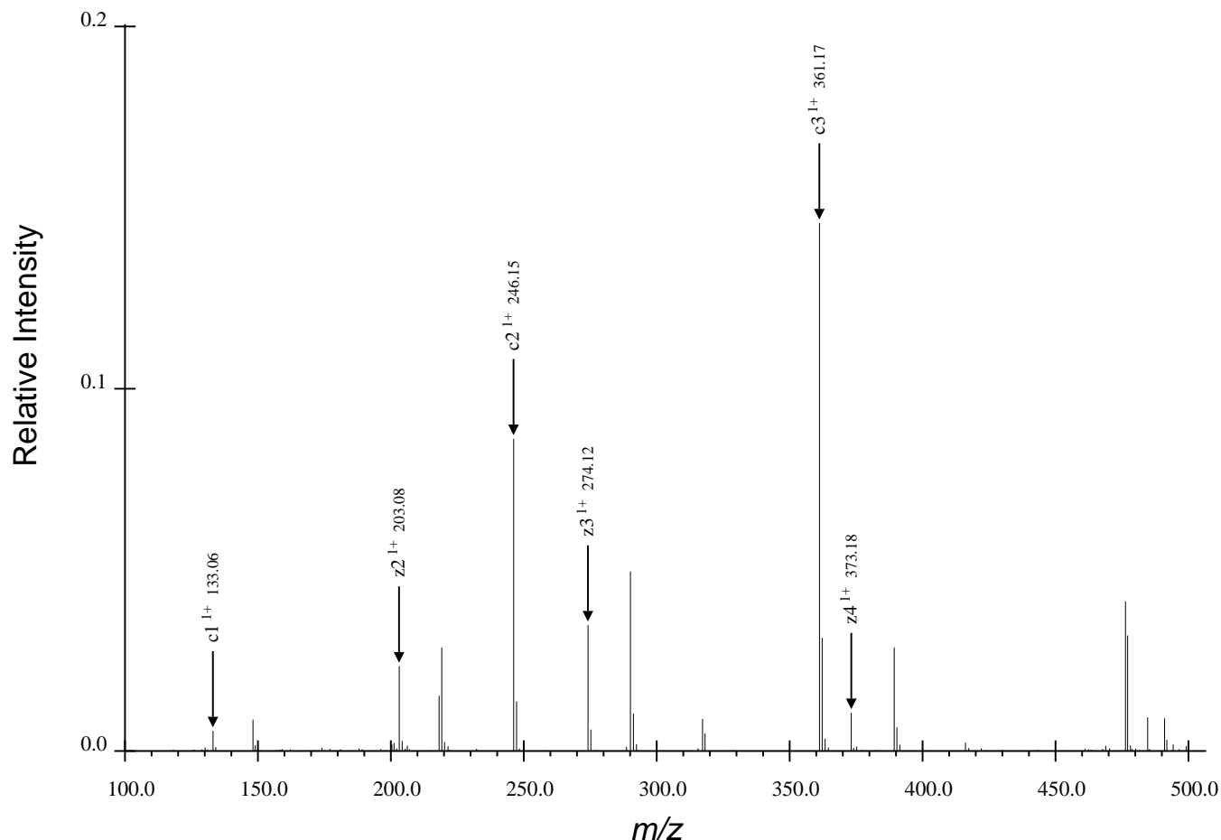
(a) First Region for DLDVPIPGRFDRRVpSVAAE, Spectrum 18.dta
