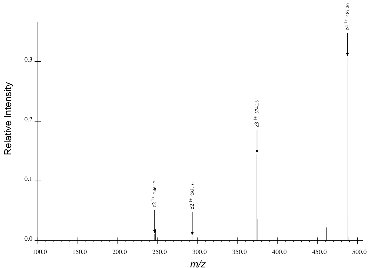
(a) First Region for FQpSEEQQQTEDELQDK, Spectrum 16.dta
