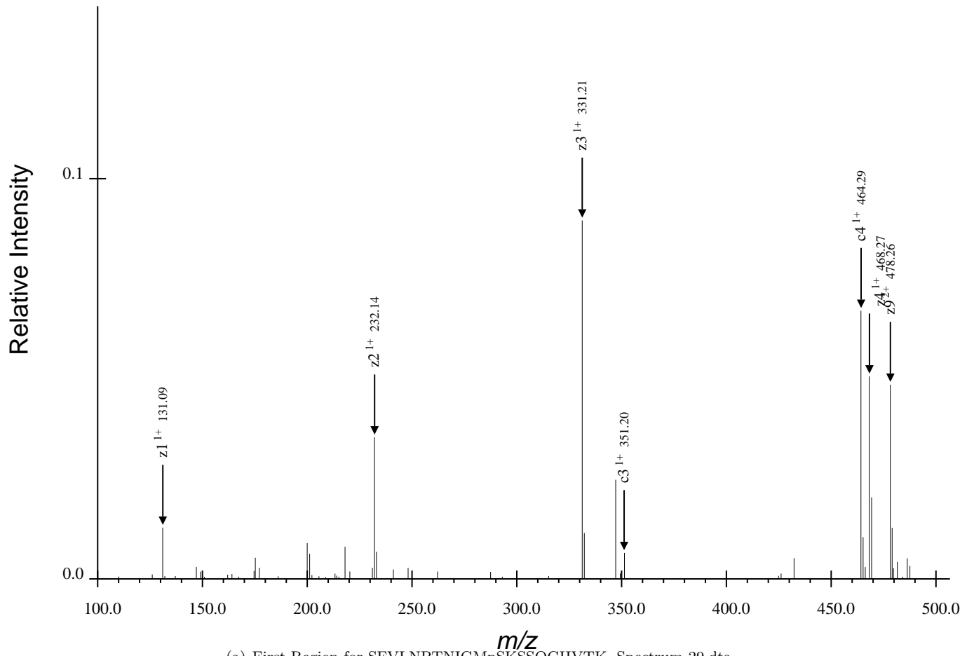
(a) First Region for SFVLNPTNIGMpSKSSQGHVTK, Spectrum 29.dta
