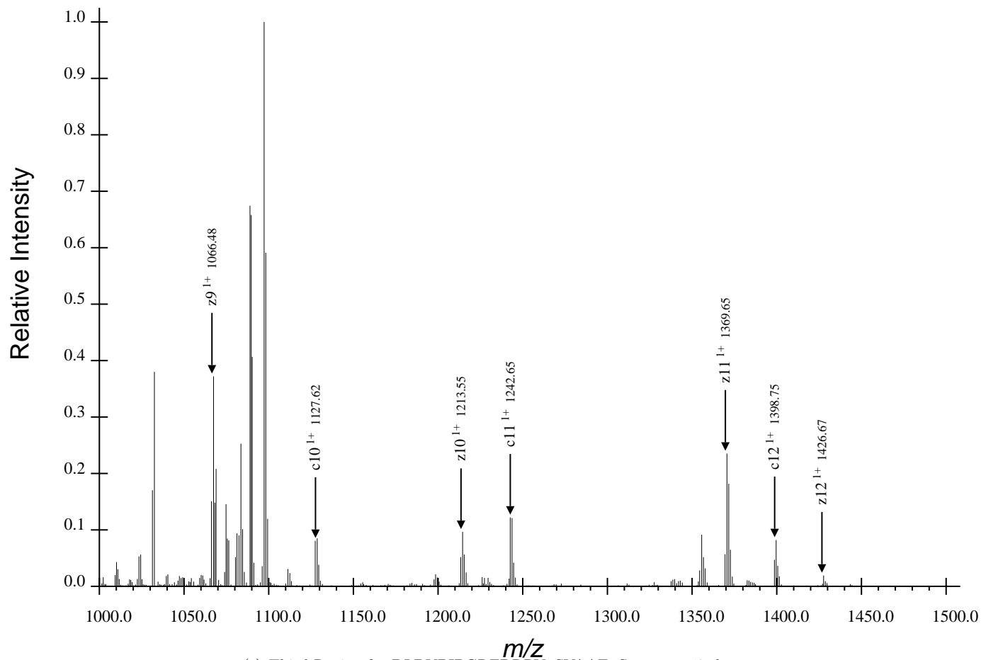
(c) Third Region for DLDVPIPGRFDRRVpSVAEE, Spectrum 17.dta
