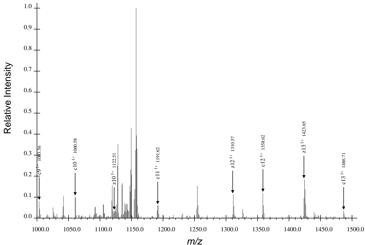
(c) Third Region for SFVLNPTNIGMpSKSSQGHVTK, Spectrum 28.dta
