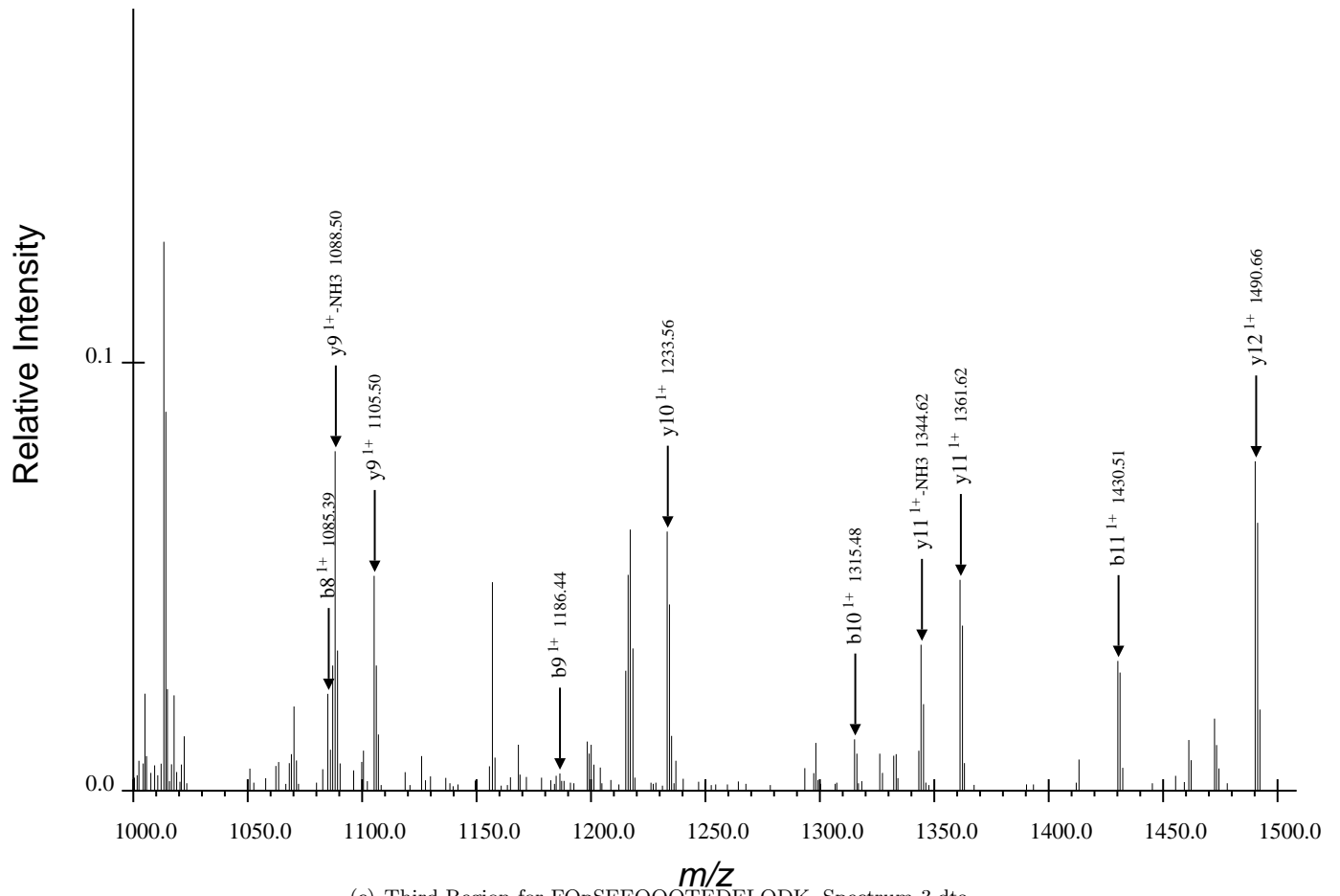
(c) Third Region for FQpSEEQQQTEDELQDK, Spectrum 3.dta
