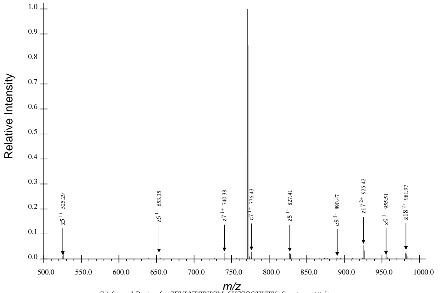
(b) Second Region for SFVLNPTNIGMpSKSSQGHVTK, Spectrum 19.dta
