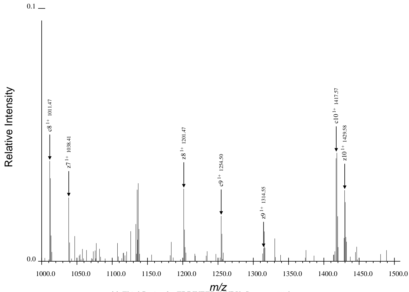
(c) Third Region for TRDIYETDpYYRK, Spectrum 55.dta
