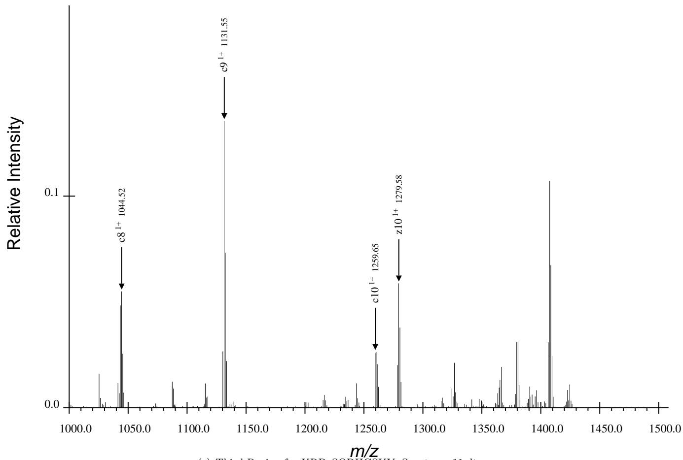
(c) Third Region for KRPpSQRHGSKY, Spectrum 11.dta
