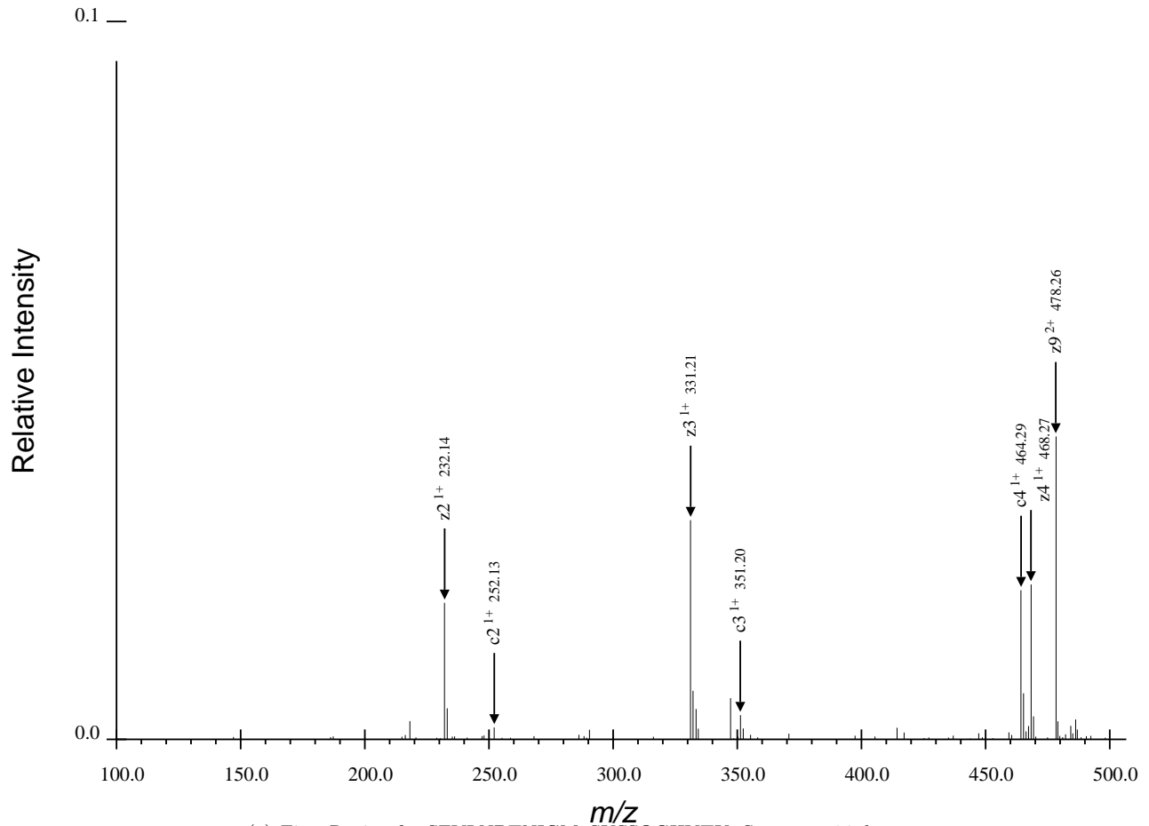
(a) First Region for SFVLNPTNIGMpSKSSQGHVTK, Spectrum 26.dta
