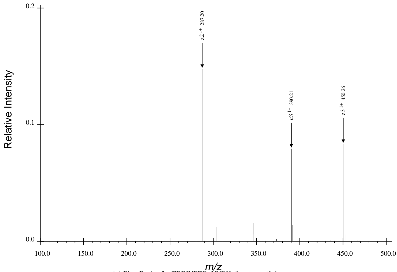
(a) First Region for TRDIYETDpYYRK, Spectrum 40.dta
