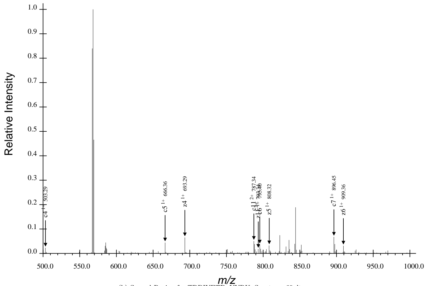
(b) Second Region for TRDIYETDpYYRK, Spectrum 60.dta
