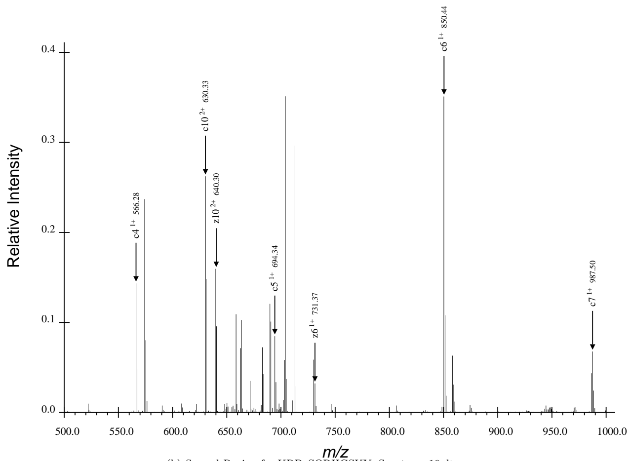
(b) Second Region for KRPpSQRHGSKY, Spectrum 10.dta
