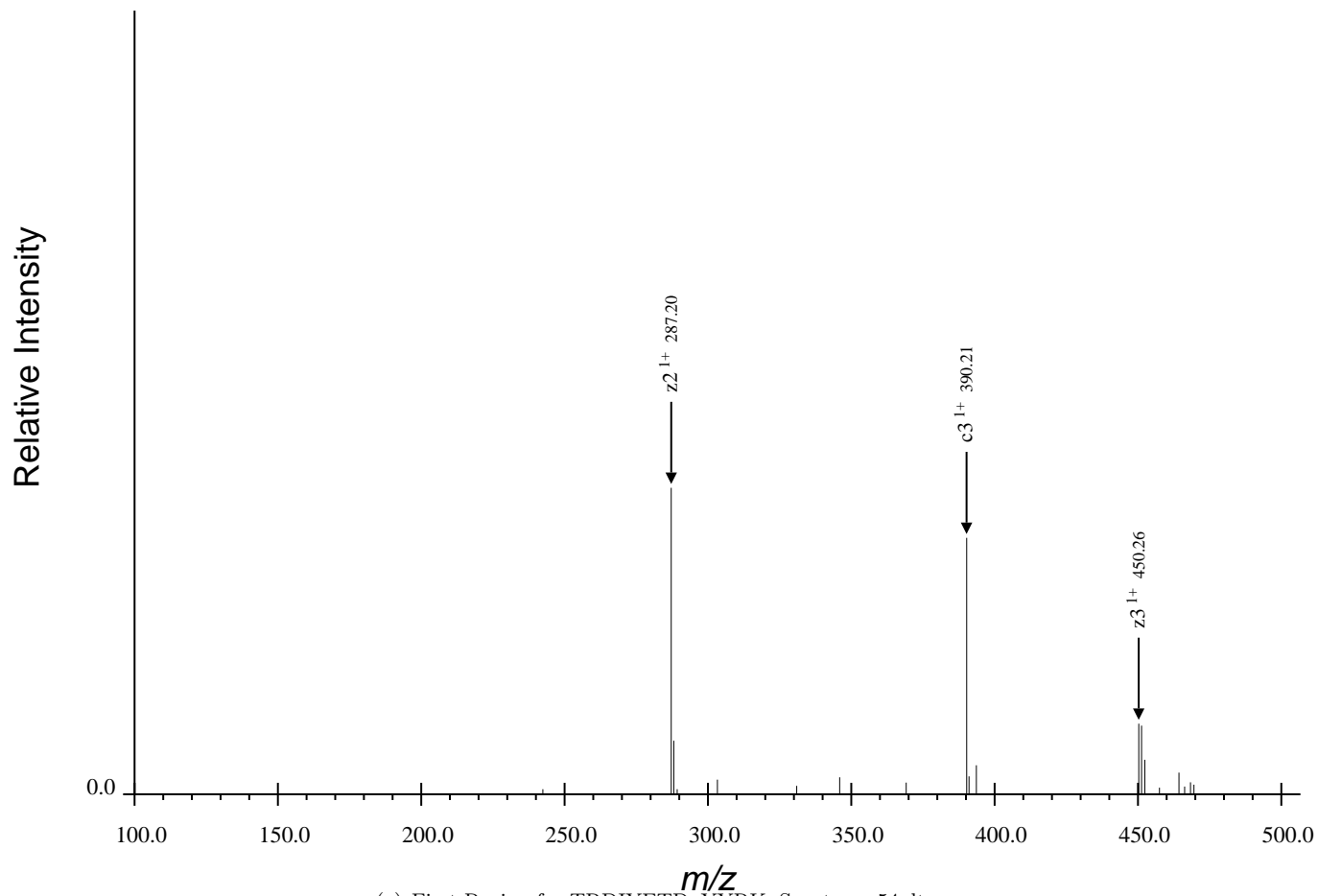
(a) First Region for TRDIYETDpYYRK, Spectrum 54.dta
