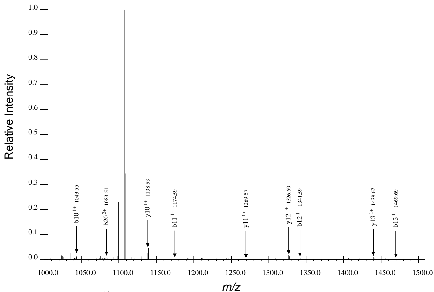
(c) Third Region for SFVLNPTNIGMpSKSSQGHVTK, Spectrum 17.dta
