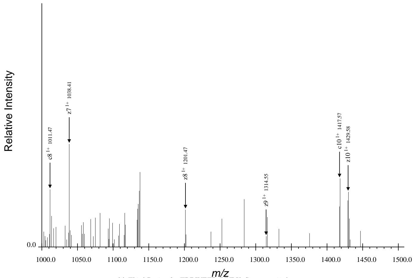
(c) Third Region for TRDIYETDpYYRK, Spectrum 68.dta
