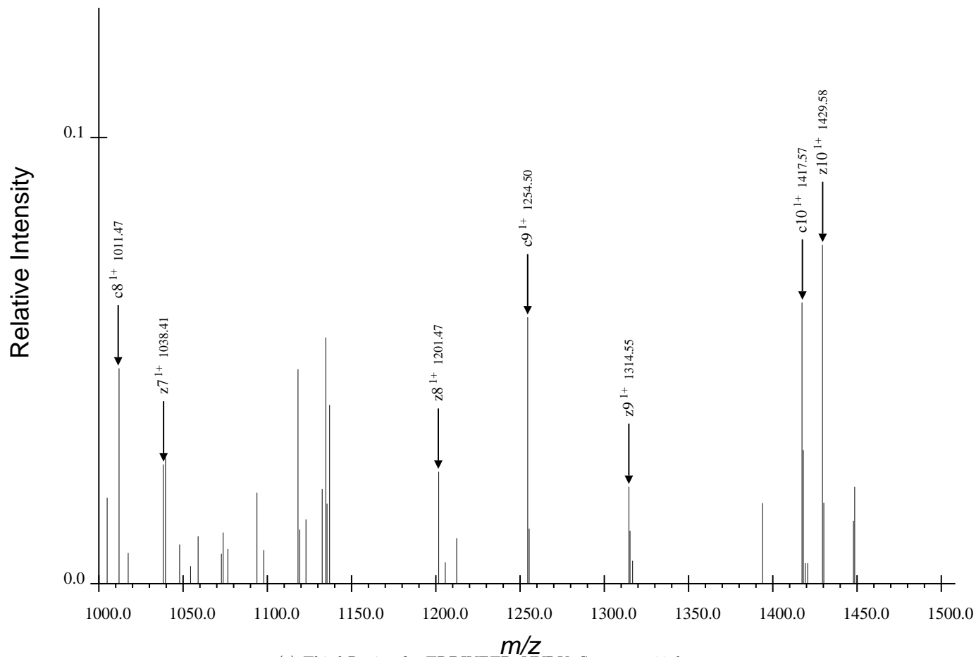
(c) Third Region for TRDIYETDpYYRK, Spectrum 66.dta
