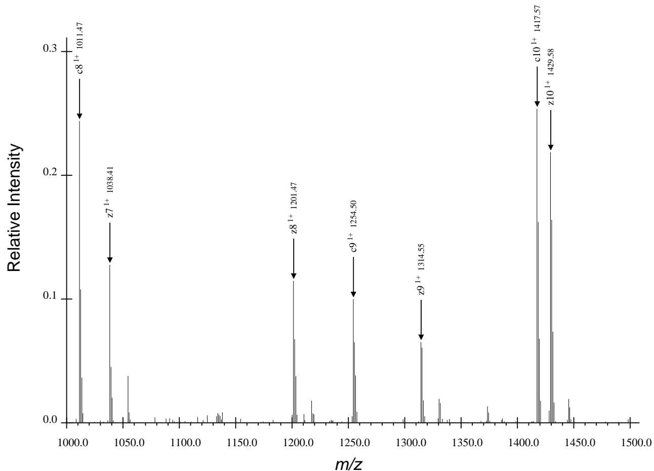
(c) Third Region for TRDIYETDpYYRK, Spectrum 40.dta
