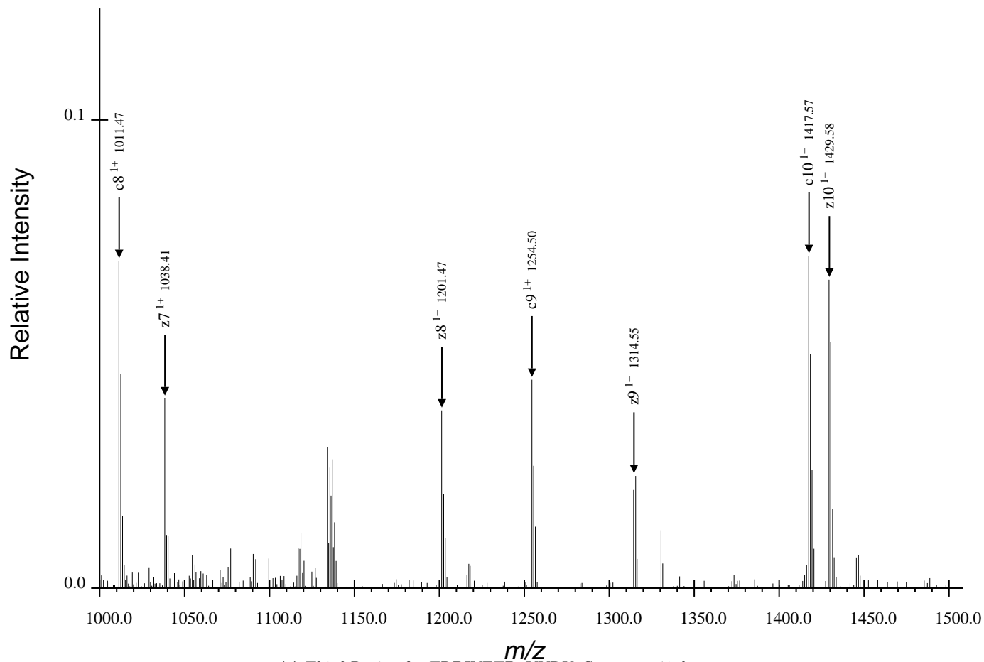
(c) Third Region for TRDIYETDpYYRK, Spectrum 41.dta
