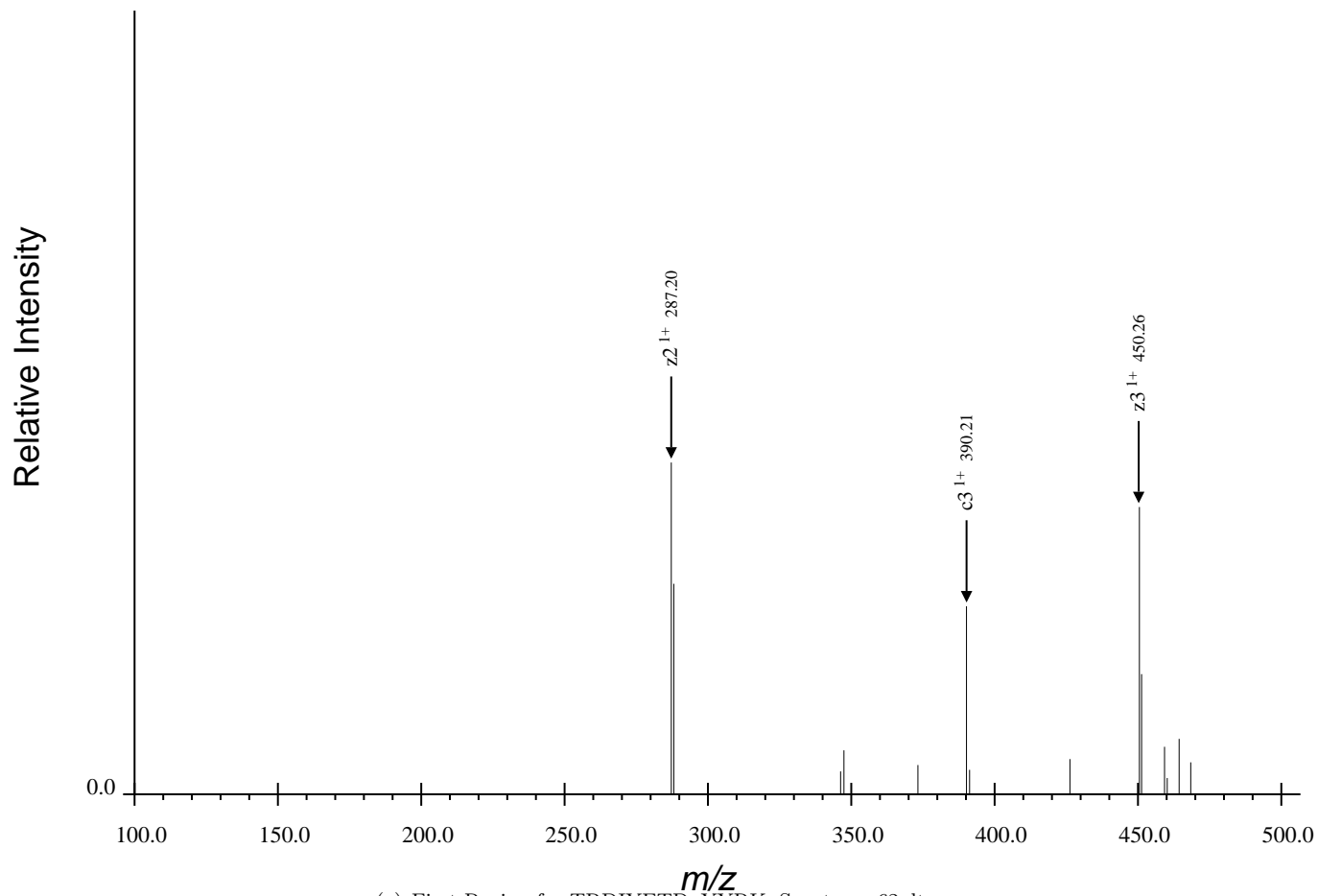
(a) First Region for TRDIYETDpYYRK, Spectrum 62.dta
