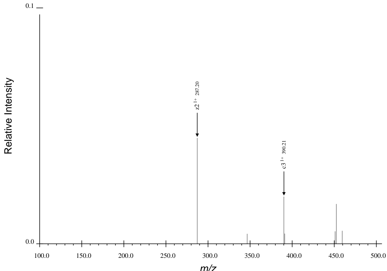
(a) First Region for TRDIYETDpYYRK, Spectrum 67.dta
