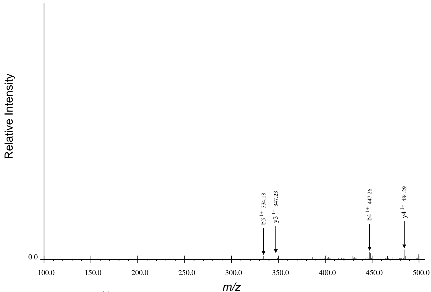
(a) First Region for SFVLNPTNIGMpSKSSQGHVTK, Spectrum 18.dta
