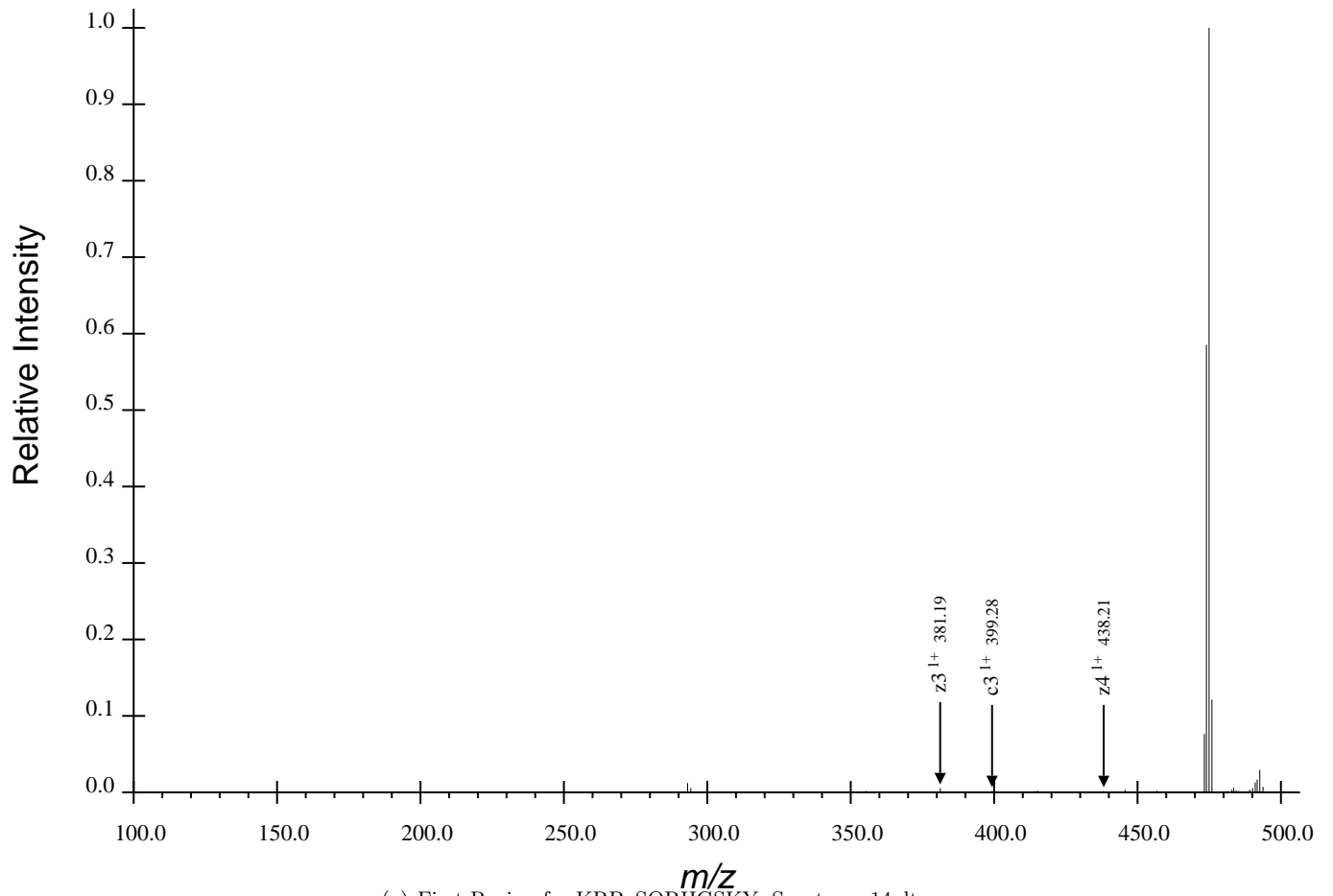
(a) First Region for KRPpSQRHGSKY, Spectrum 14.dta
