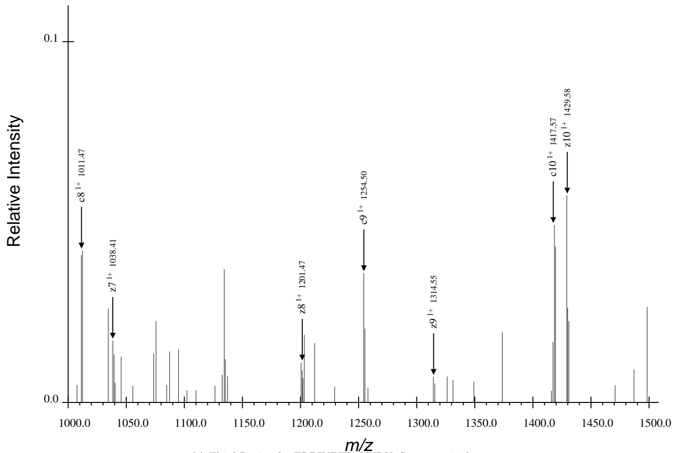
(c) Third Region for TRDIYETDpYYRK, Spectrum 65.dta
