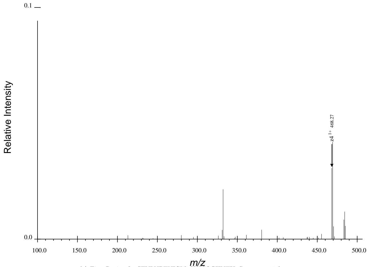
(a) First Region for SFVLNPTNIGMpSKSSQGHVTK, Spectrum 19.dta
