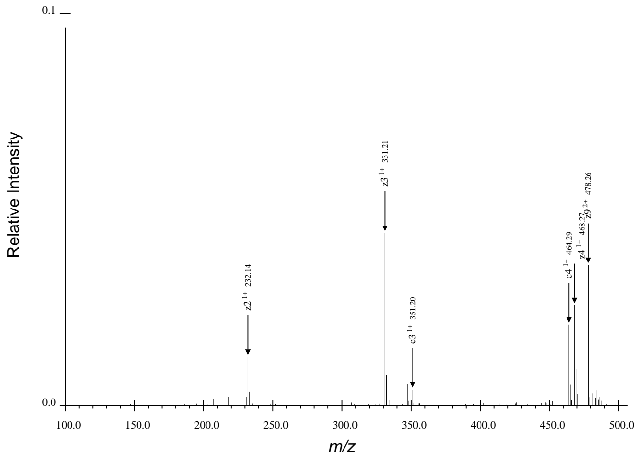
(a) First Region for SFVLNPTNIGMpSKSSQGHVTK, Spectrum 25.dta
