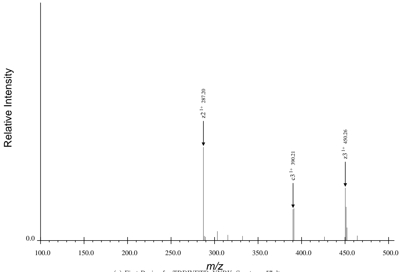
(a) First Region for TRDIYETDpYYRK, Spectrum 57.dta
