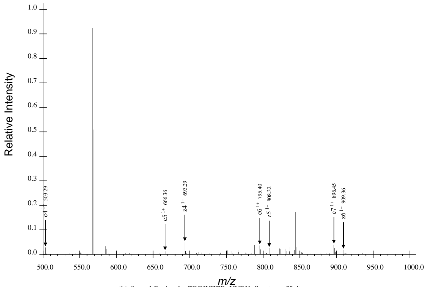
(b) Second Region for TRDIYETDpYYRK, Spectrum 55.dta
