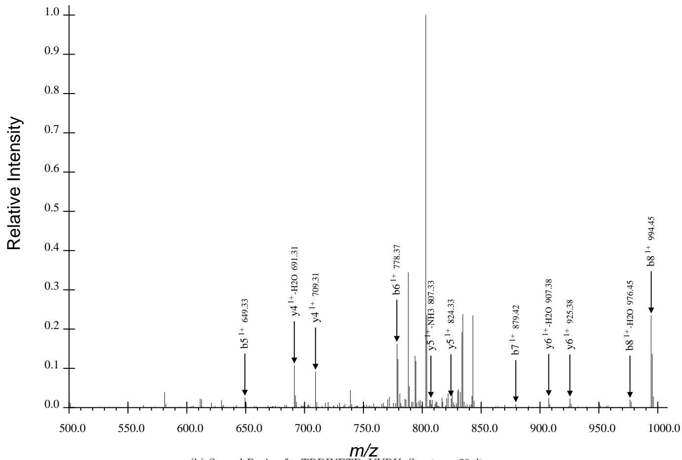
(b) Second Region for TRDIYETDpYYRK, Spectrum 29.dta
