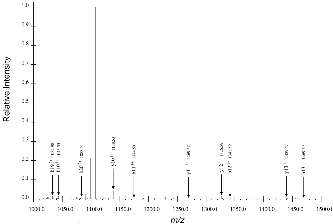
(c) Third Region for SFVLNPTNIGMpSKSSQGHVTK, Spectrum 18.dta
