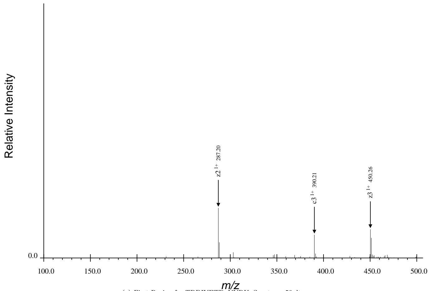
(a) First Region for TRDIYETDpYYRK, Spectrum 50.dta
