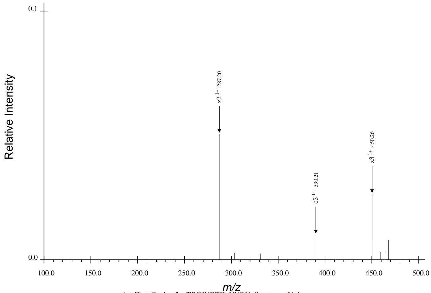
(a) First Region for TRDIYETDpYYRK, Spectrum 64.dta
