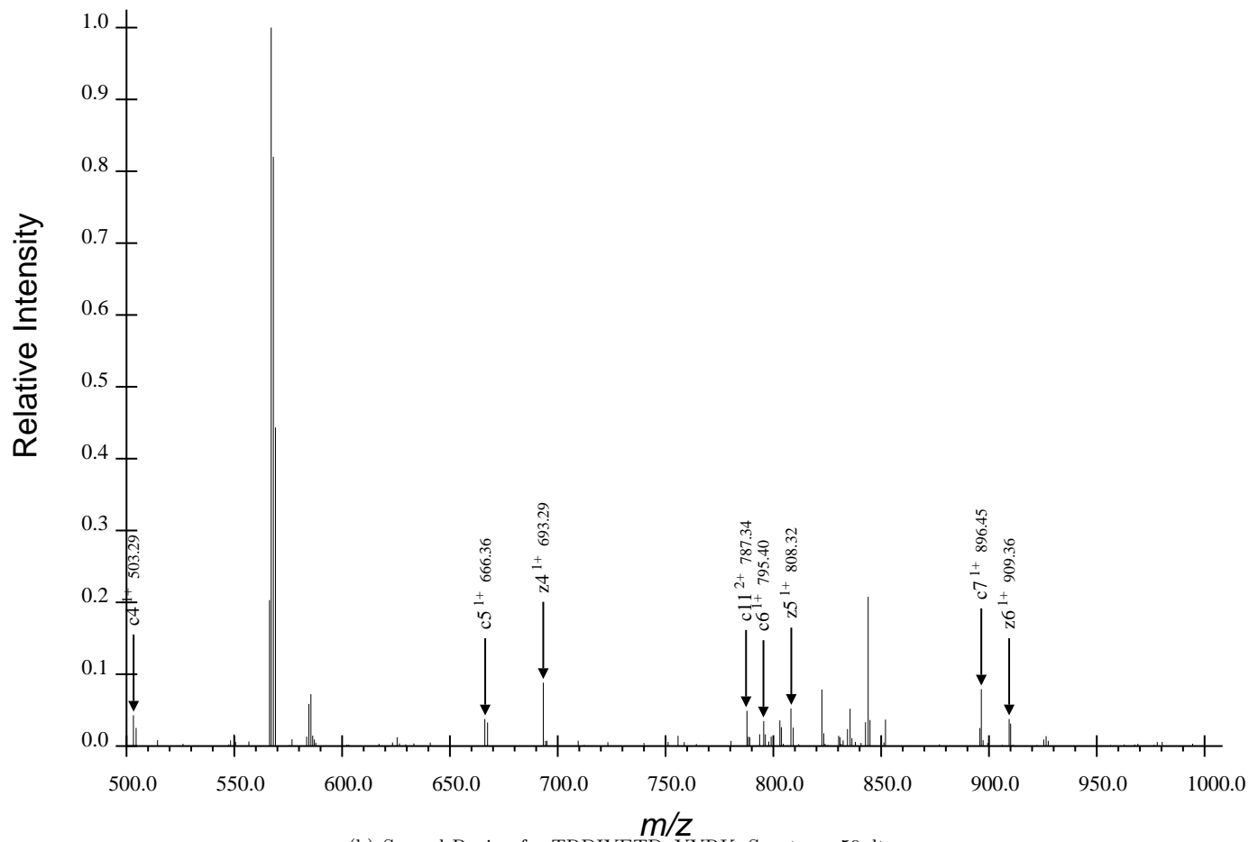
(b) Second Region for TRDIYETDpYYRK, Spectrum 59.dta
