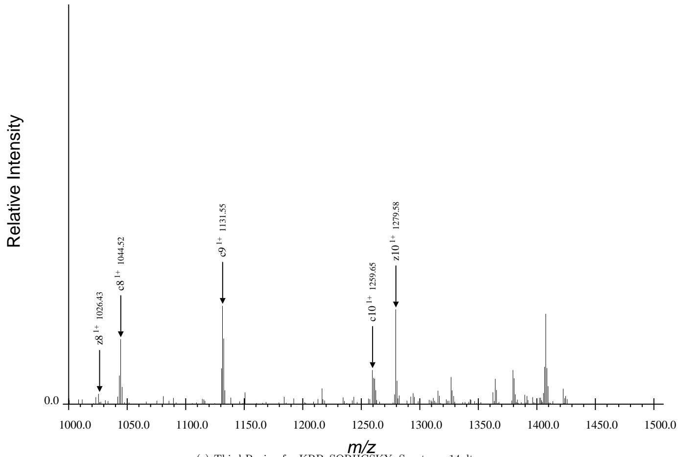
(c) Third Region for KRPpSQRHGSKY, Spectrum 14.dta
