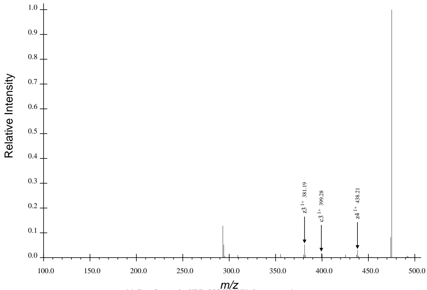
(a) First Region for KRPPSQRHGSKY, Spectrum 5.dta
