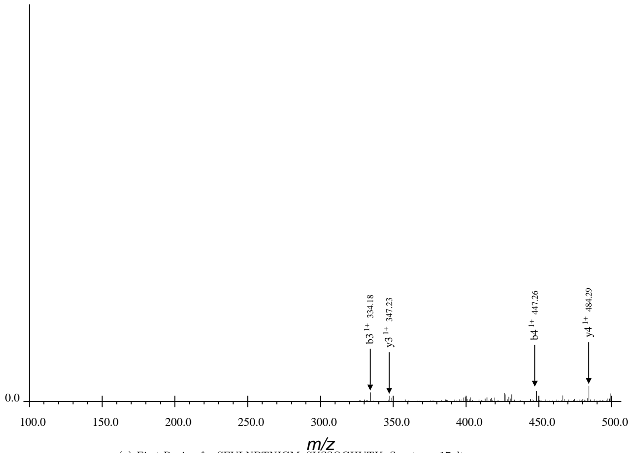
(a) First Region for SFVLNPTNIGMpSKSSQGHVTK, Spectrum 17.dta
