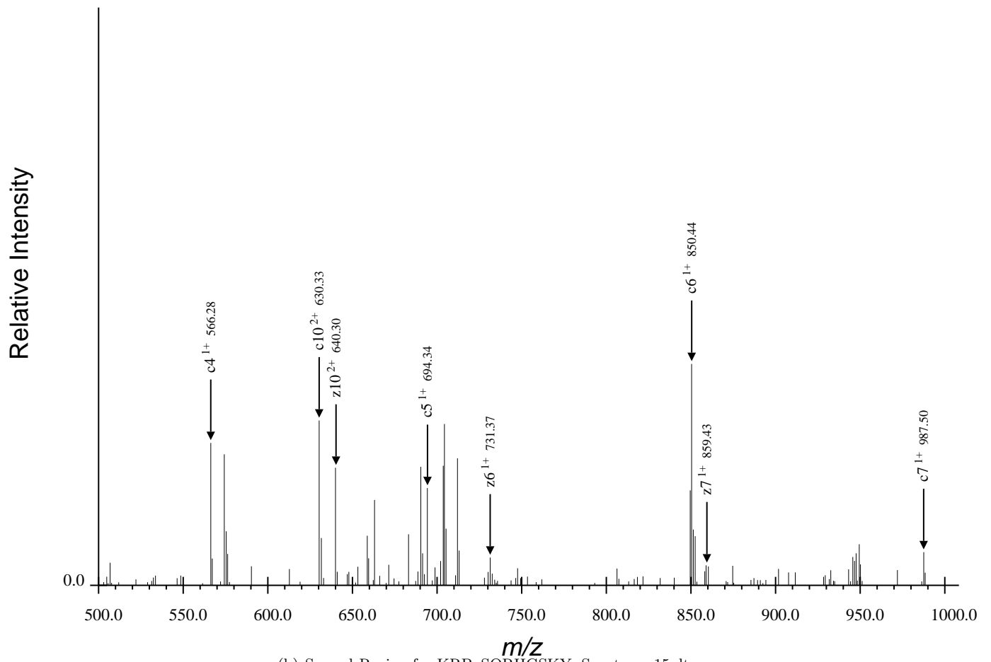
(b) Second Region for KRPpSQRHGSKY, Spectrum 15.dta
