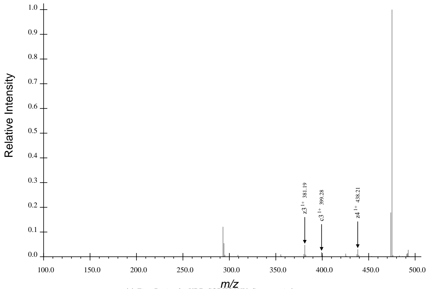
(a) First Region for KRPpSQRHGSKY, Spectrum 7.dta
