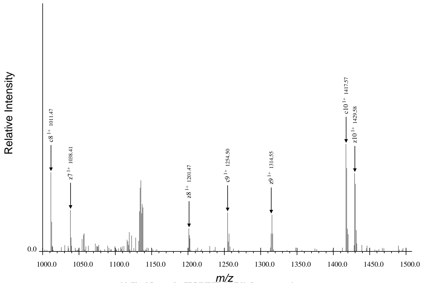
(c) Third Region for TRDIYETDpYYRK, Spectrum 52.dta
