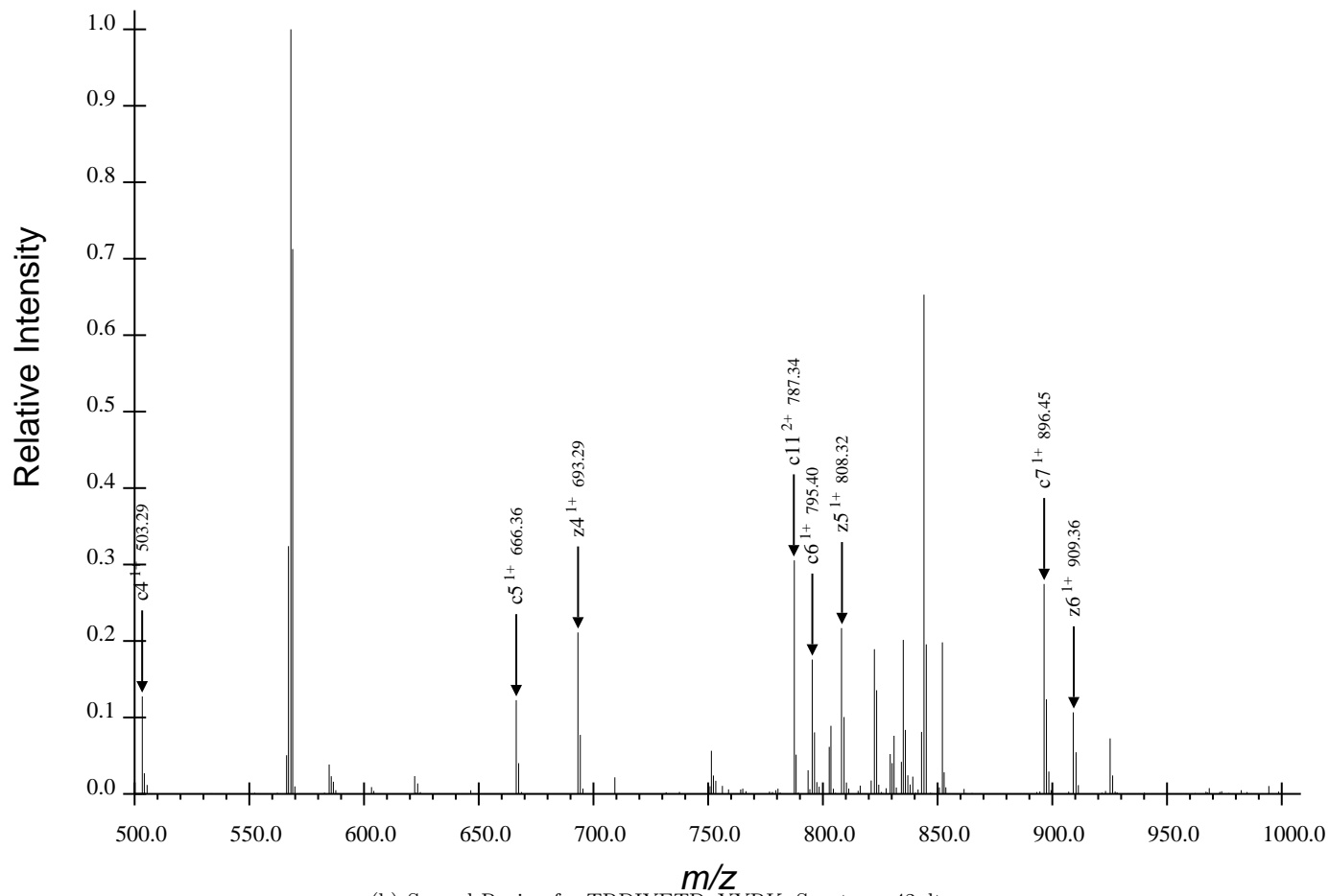
(b) Second Region for TRDIYETDpYYRK, Spectrum 42.dta
