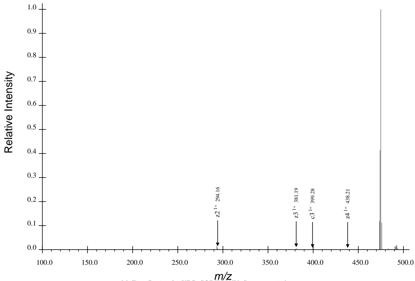
(a) First Region for KRPpSQRHGSKY, Spectrum 13.dta
