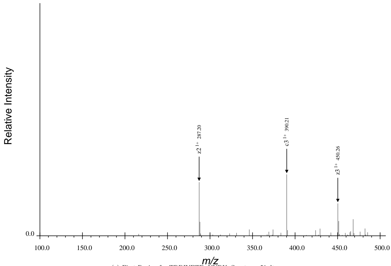
(a) First Region for TRDIYETDpYYRK, Spectrum 51.dta
