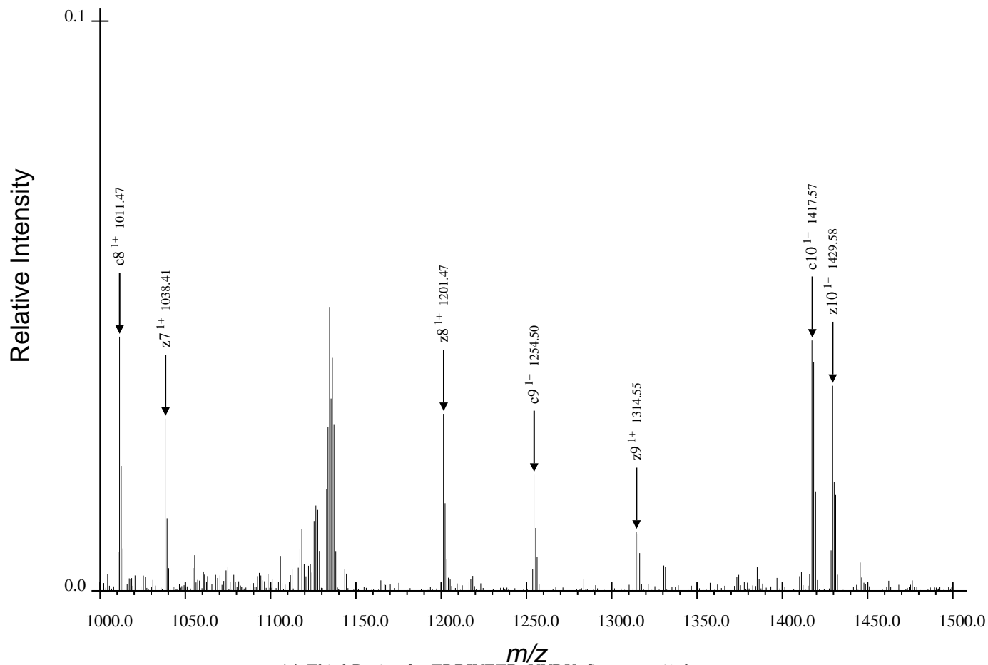
(c) Third Region for TRDIYETDpYYRK, Spectrum 48.dta
