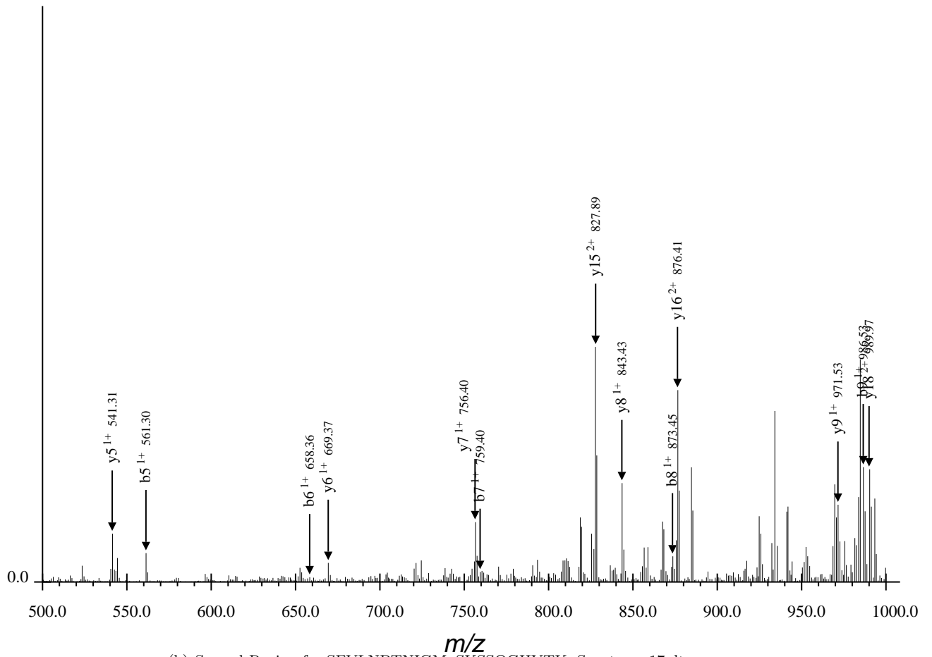
(b) Second Region for SFVLNPTNIGMpSKSSQGHVTK, Spectrum 17.dta
