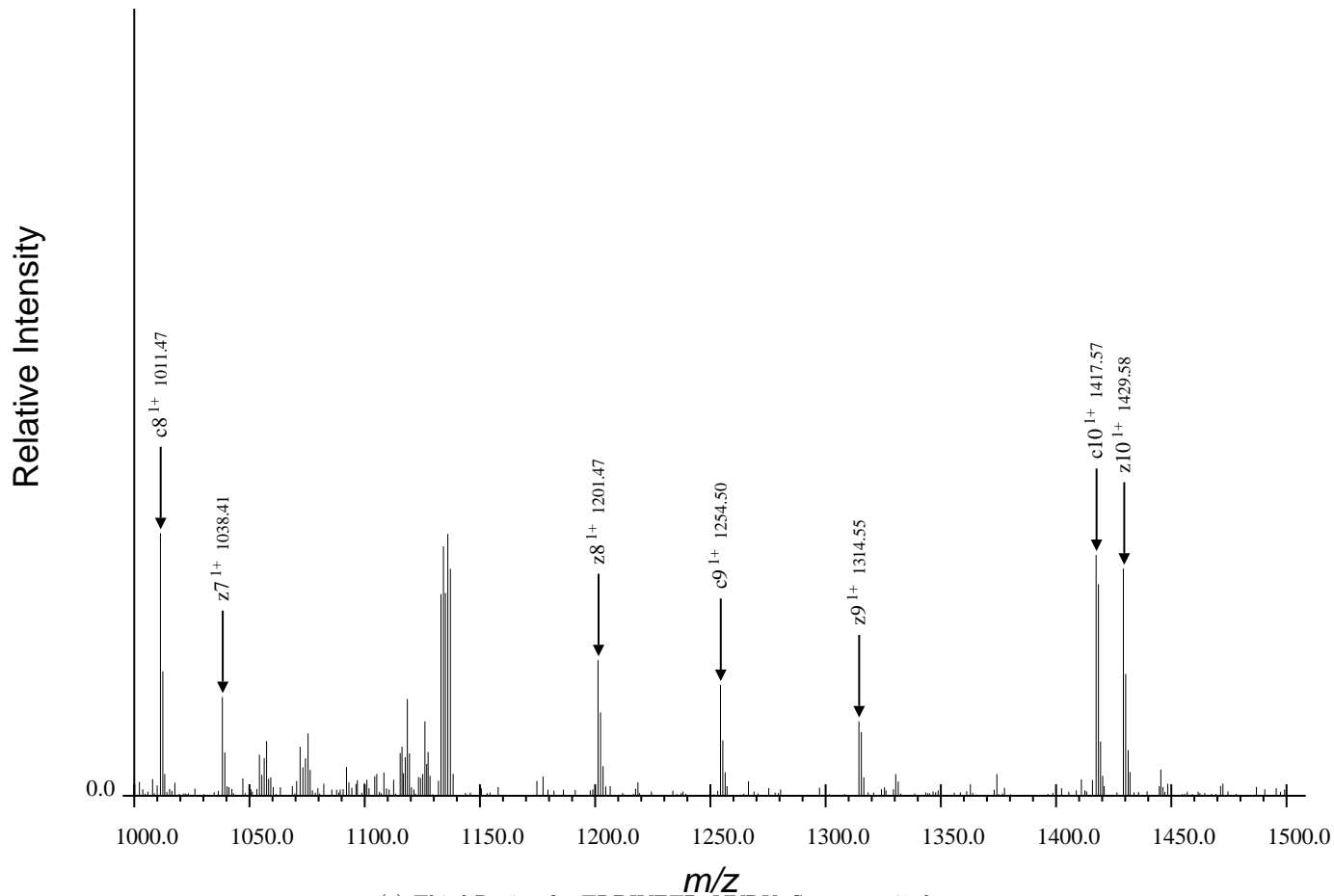
(c) Third Region for TRDIYETDpYYRK, Spectrum 49.dta
