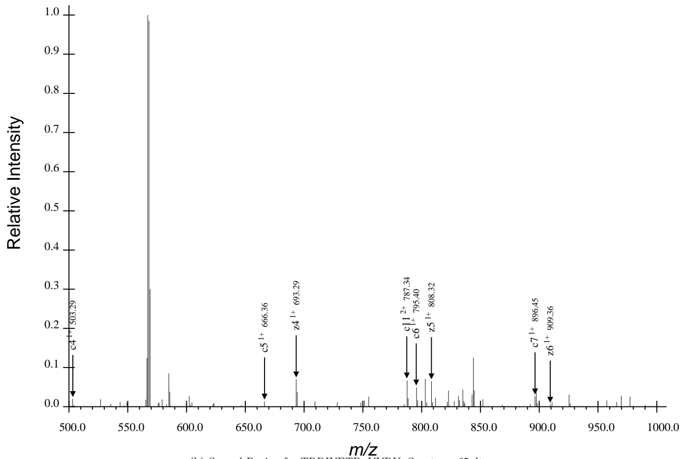
(b) Second Region for TRDIYETDpYYRK, Spectrum 65.dta
