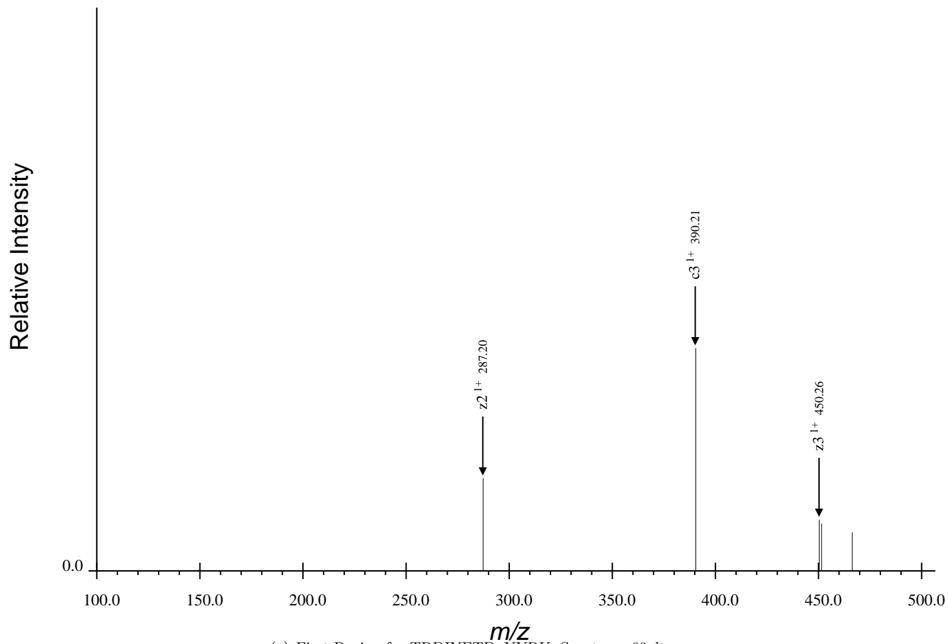
(a) First Region for TRDIYETDpYYRK, Spectrum 66.dta
