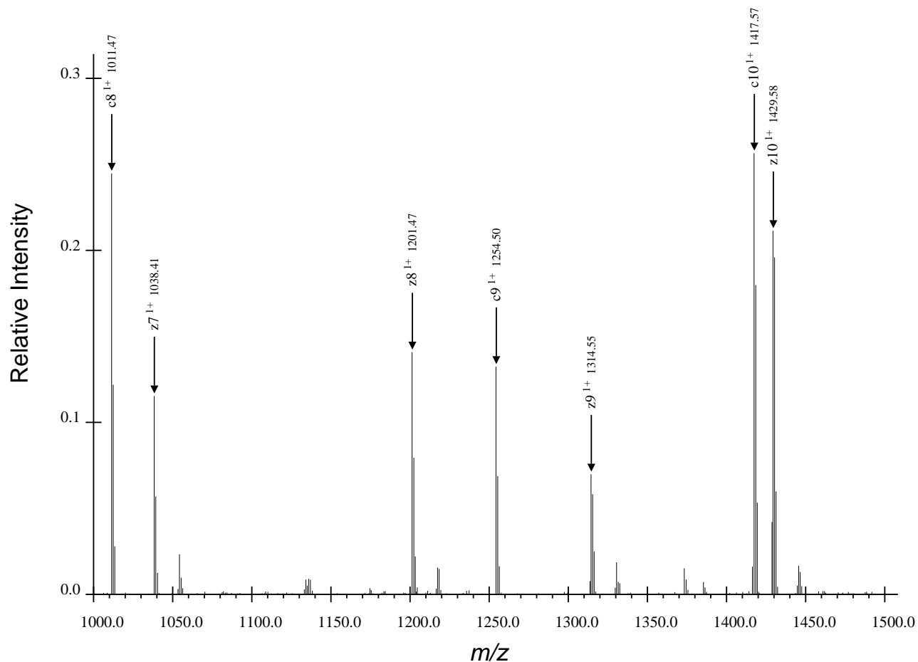
(c) Third Region for TRDIYETDpYYRK, Spectrum 44.dta
