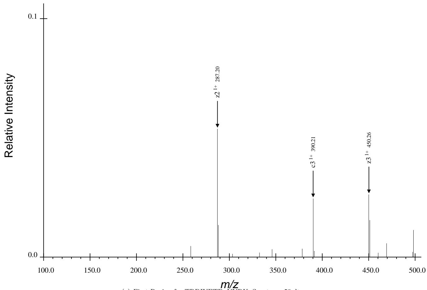
(a) First Region for TRDIYETDpYYRK, Spectrum 59.dta
