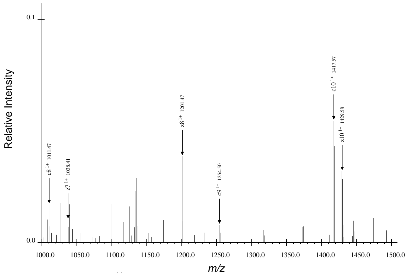
(c) Third Region for TRDIYETDpYYRK, Spectrum 64.dta
