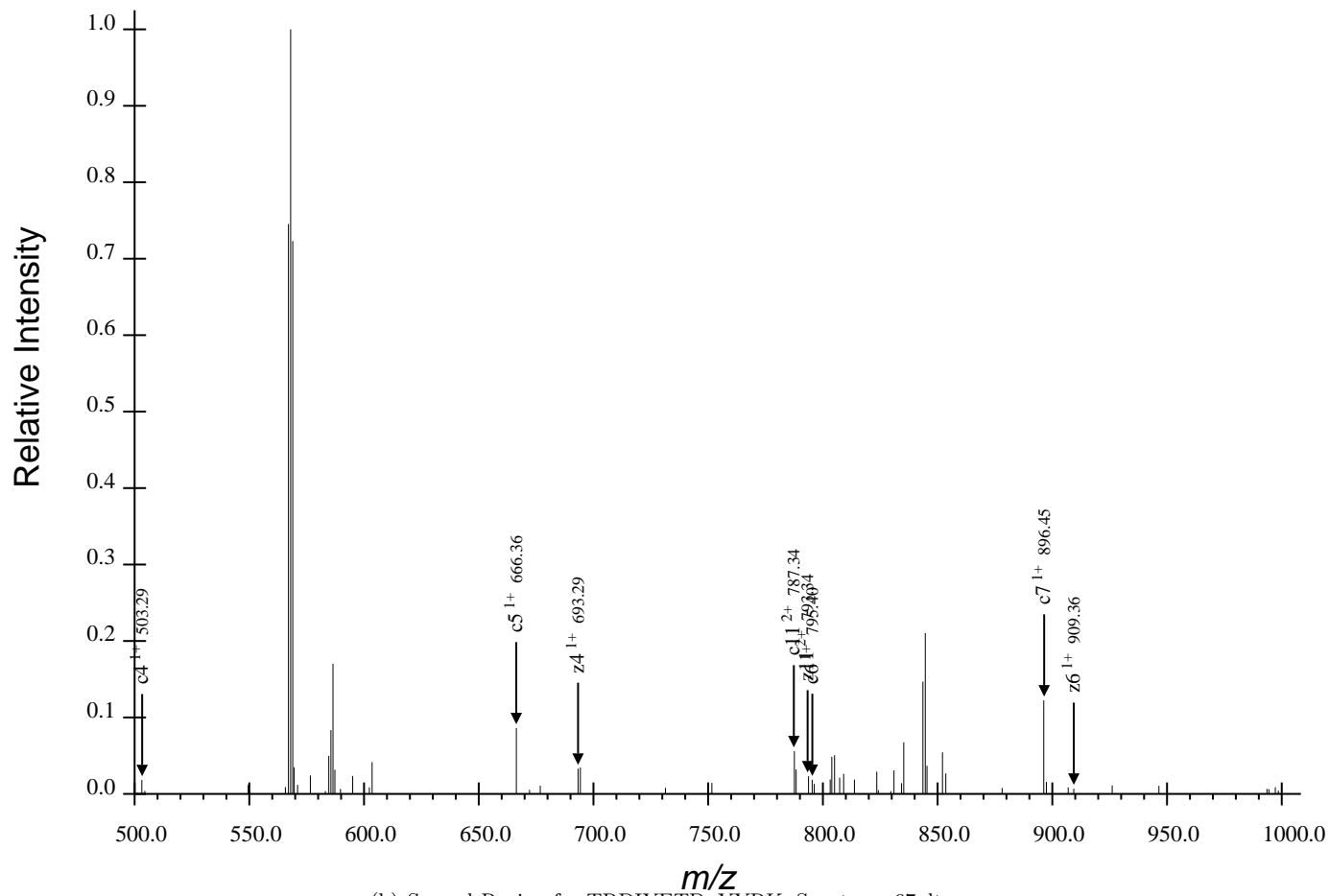
(b) Second Region for TRDIYETDpYYRK, Spectrum 67.dta
