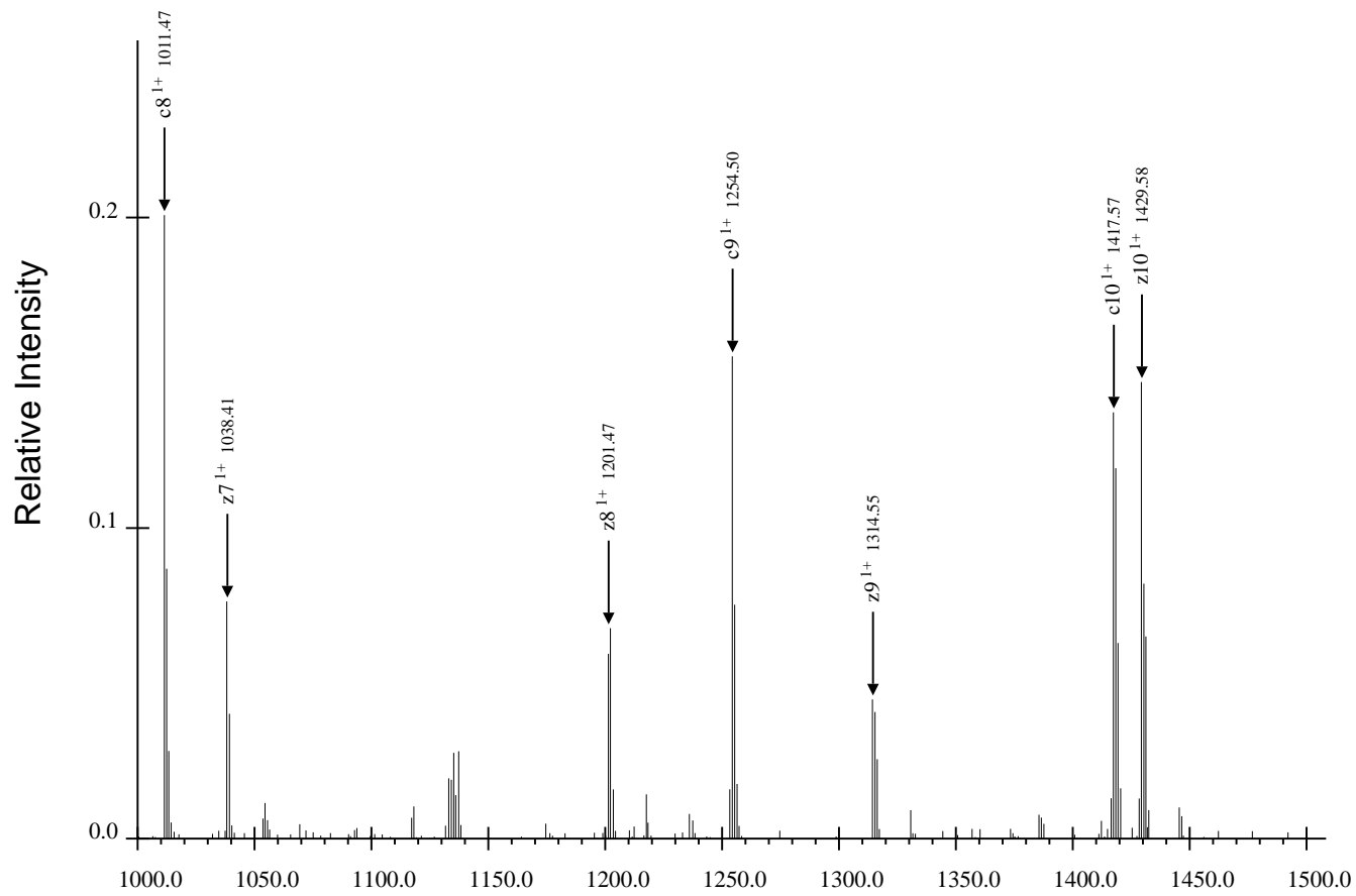
(c) Third Region for TRDIYETDpYYRK, Spectrum 38.dta
