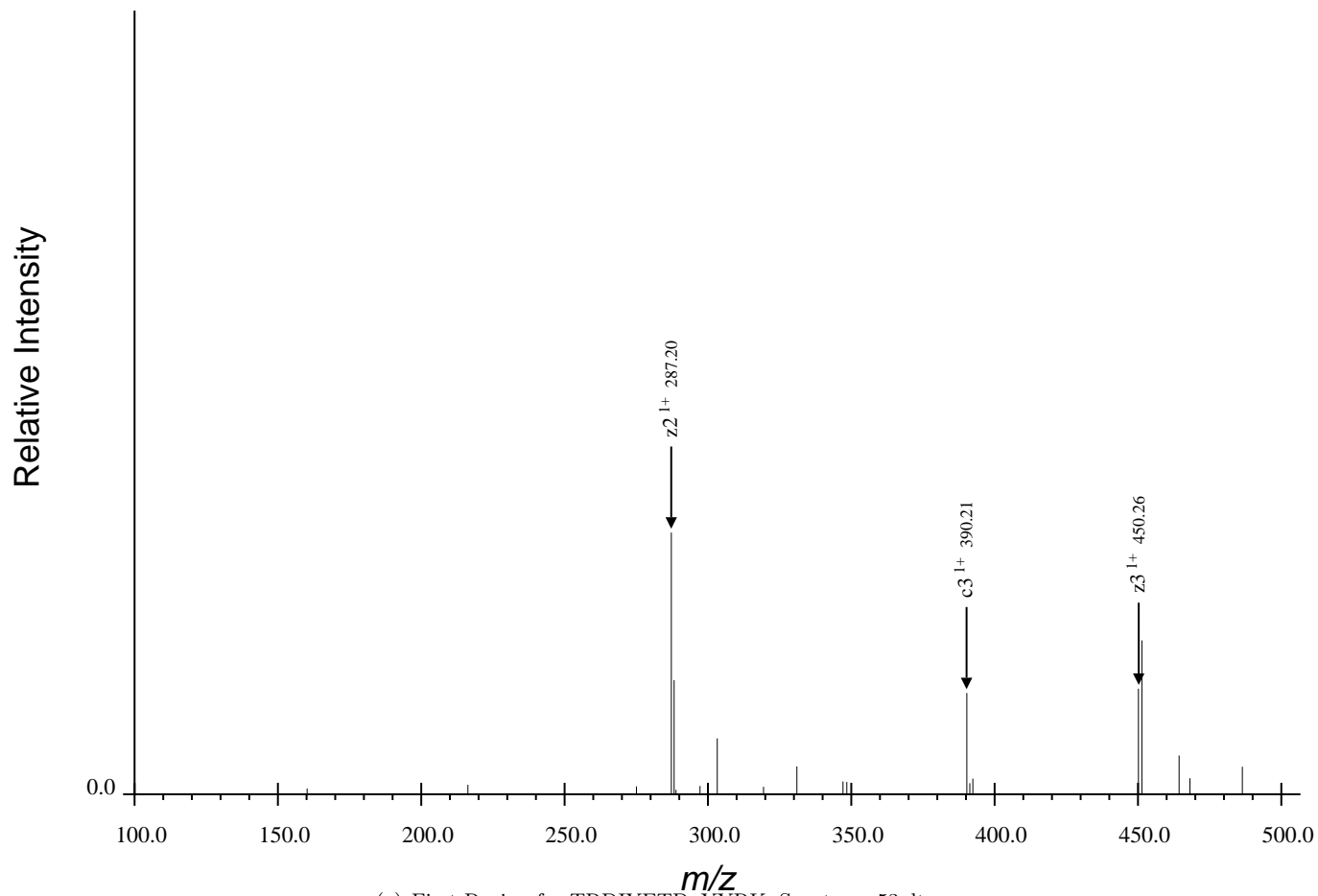
(a) First Region for TRDIYETDpYYRK, Spectrum 53.dta
