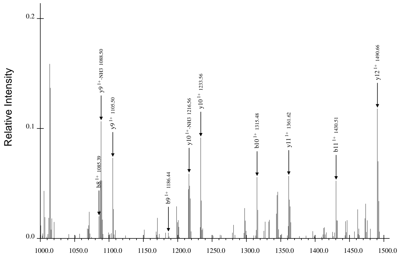
(c) Third Region for FQpSEEQQQTEDELQDK, Spectrum 2.dta
