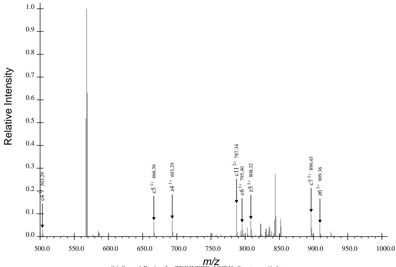
(b) Second Region for TRDIYETDpYYRK, Spectrum 41.dta
