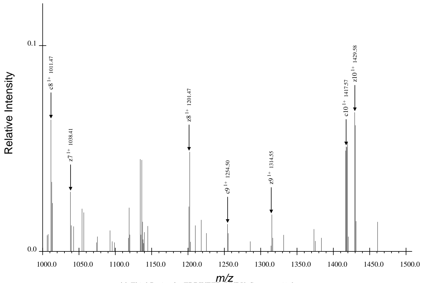
(c) Third Region for TRDIYETDpYYRK, Spectrum 63.dta
