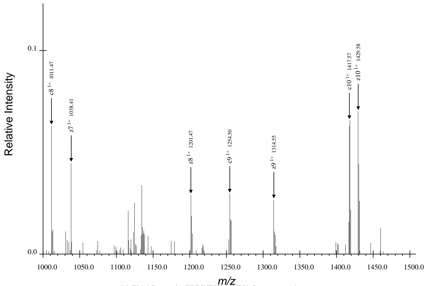
(c) Third Region for TRDIYETDpYYRK, Spectrum 59.dta
