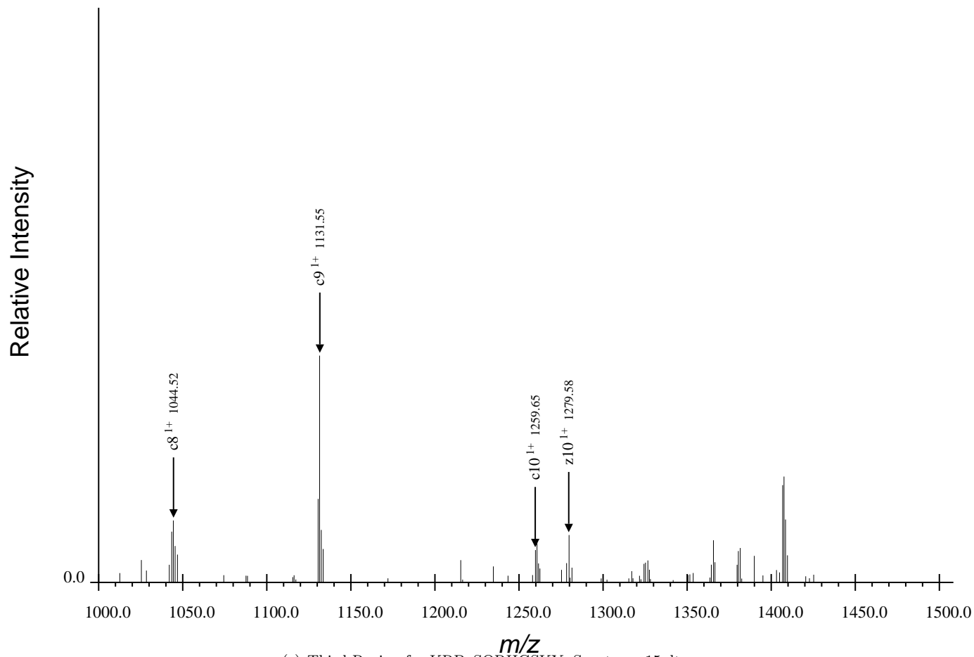
(c) Third Region for KRPPSQRHGSKY, Spectrum 15.dta
