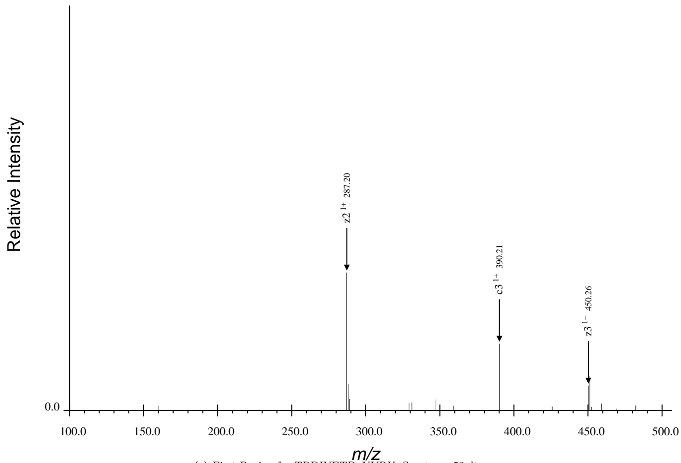
(a) First Region for TRDIYETDpYYRK, Spectrum 52.dta
