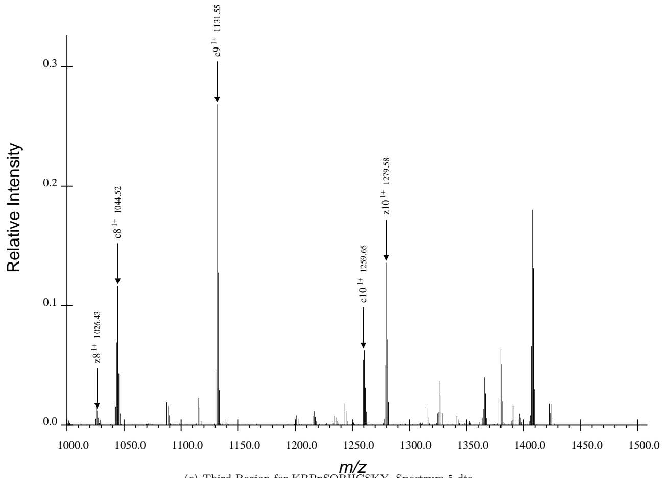
(c) Third Region for KRPPSQRHGSKY, Spectrum 5.dta
