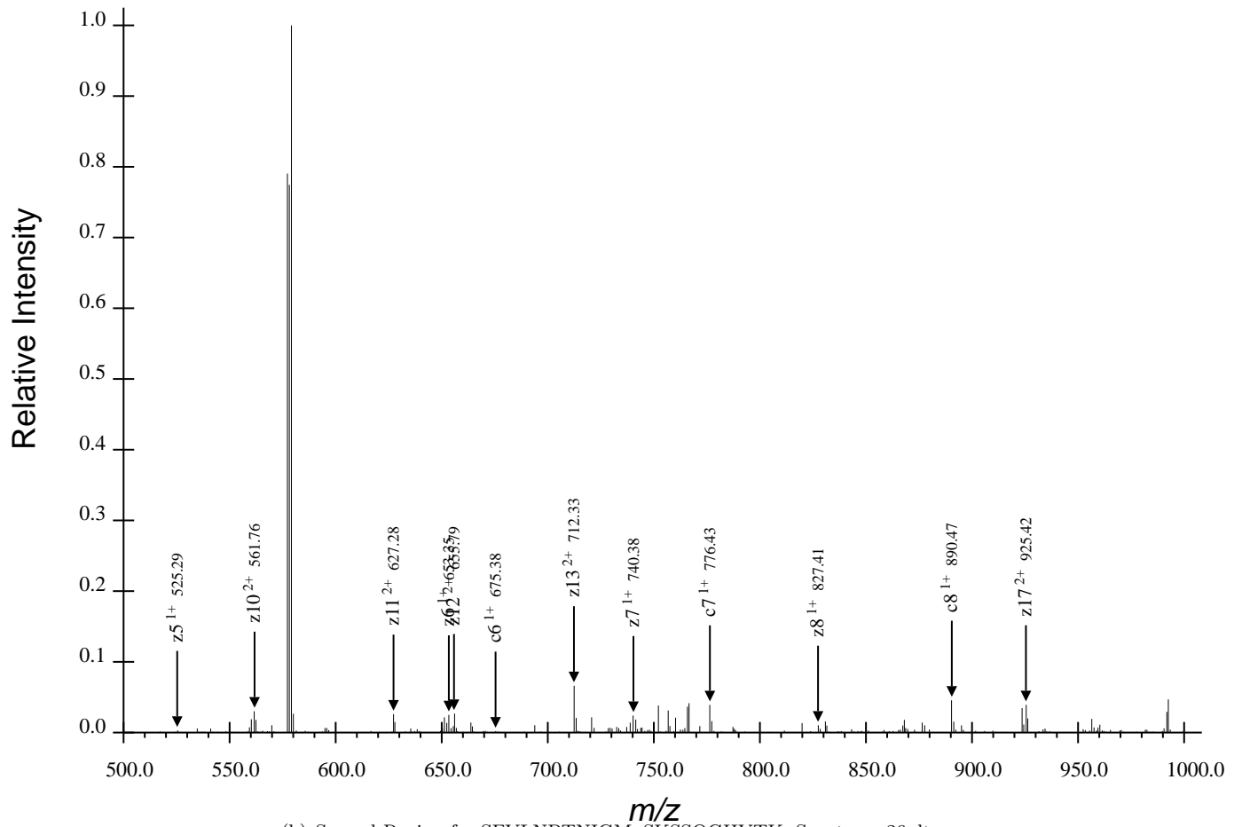
(b) Second Region for SFVLNPTNIGMpSKSSQGHVTK, Spectrum 26.dta
