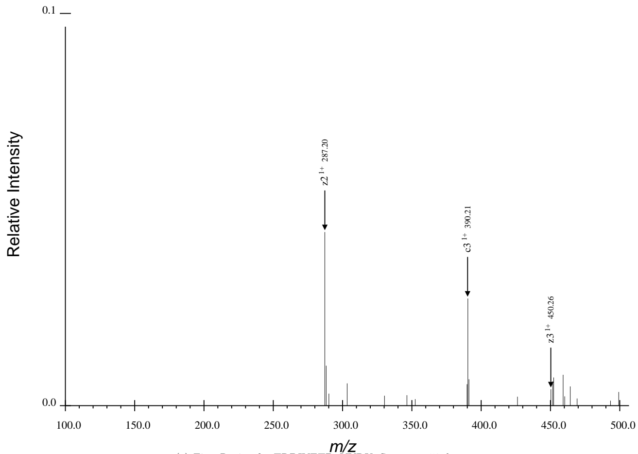
(a) First Region for TRDIYETDpYYRK, Spectrum 58.dta
