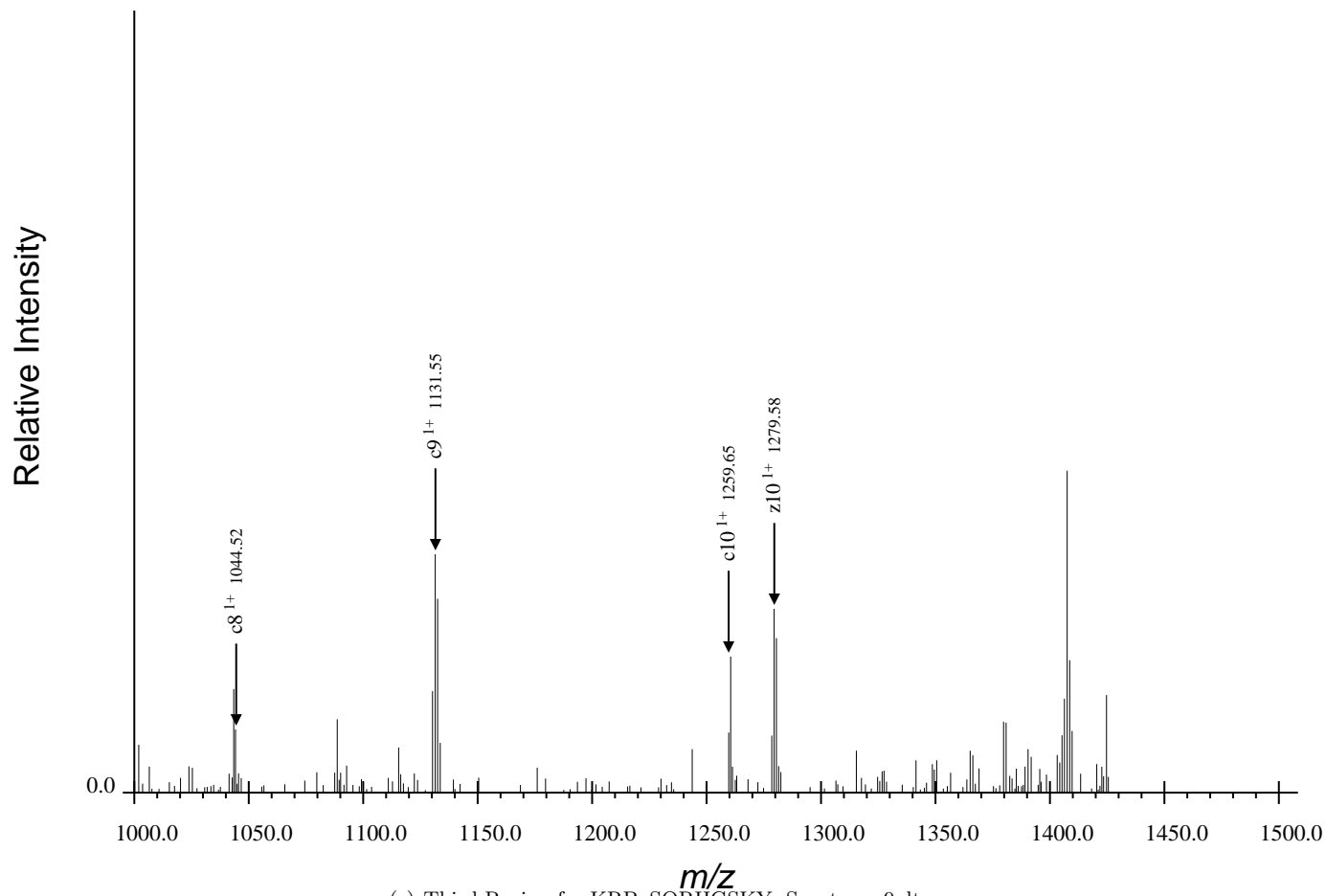
(c) Third Region for KRPpSQRHGSKY, Spectrum 9.dta
