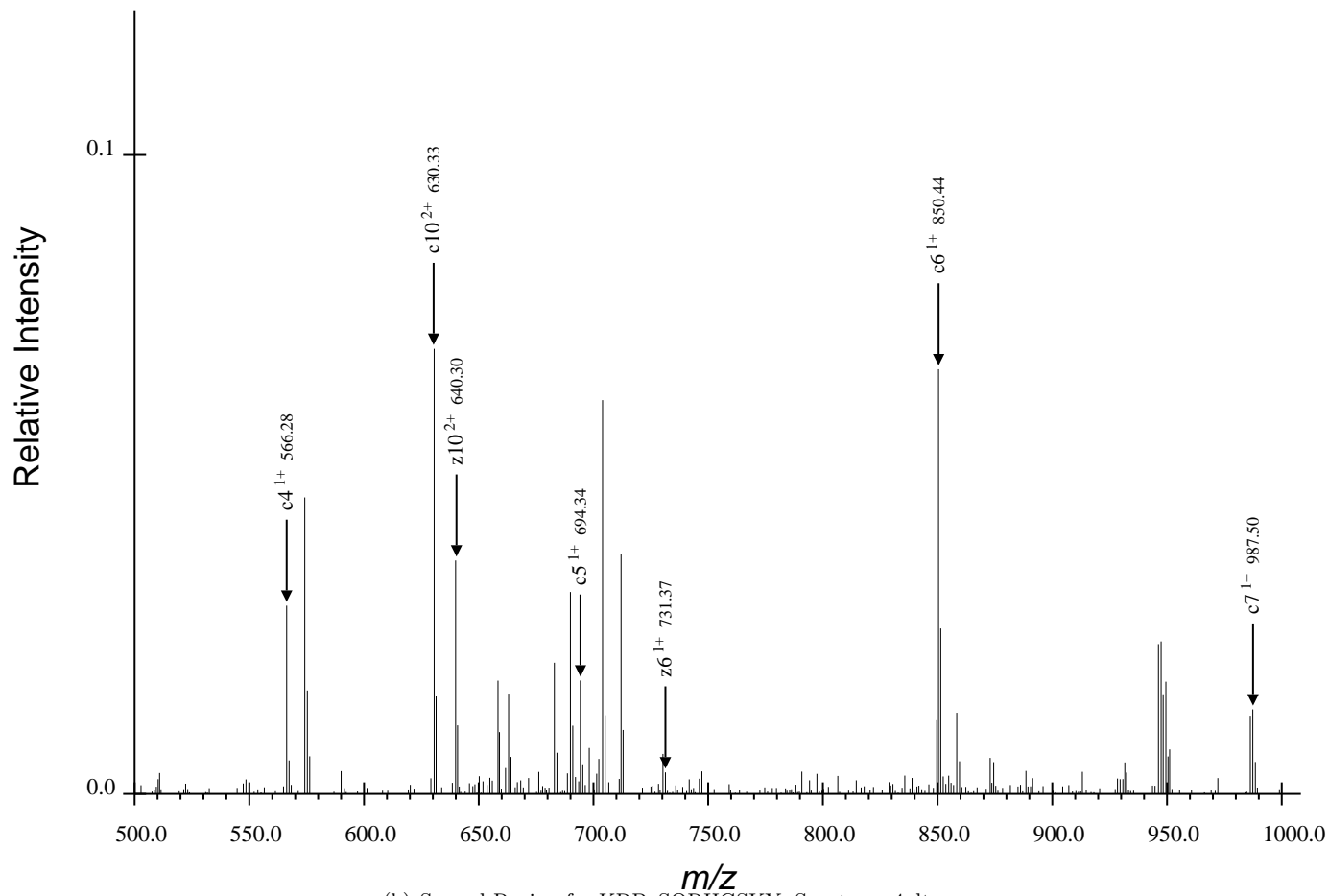
(b) Second Region for KRPPSQRHGSKY, Spectrum 4.dta
