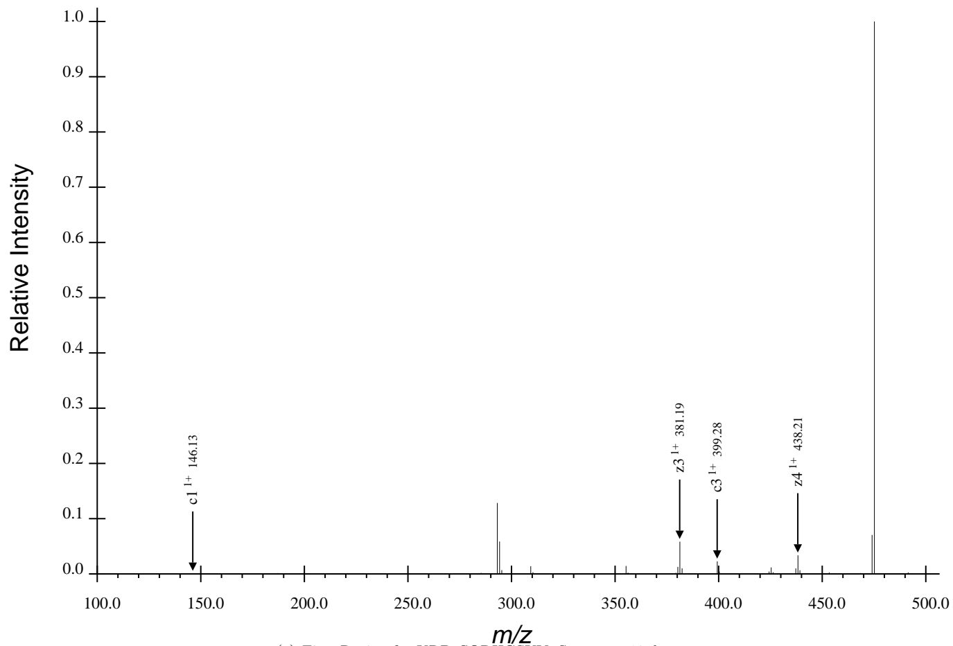
(a) First Region for KRPpSQRHGSKY, Spectrum 10.dta
