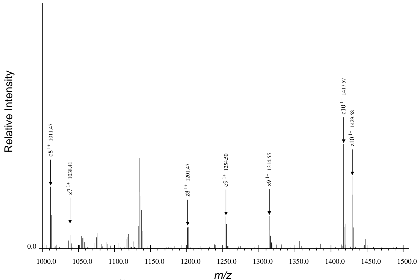
(c) Third Region for TRDIYETDpYYRK, Spectrum 51.dta
