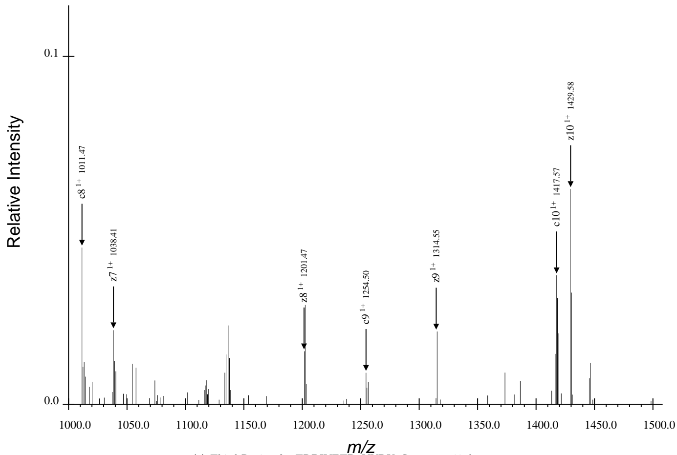
(c) Third Region for TRDIYETDpYYRK, Spectrum 60.dta
