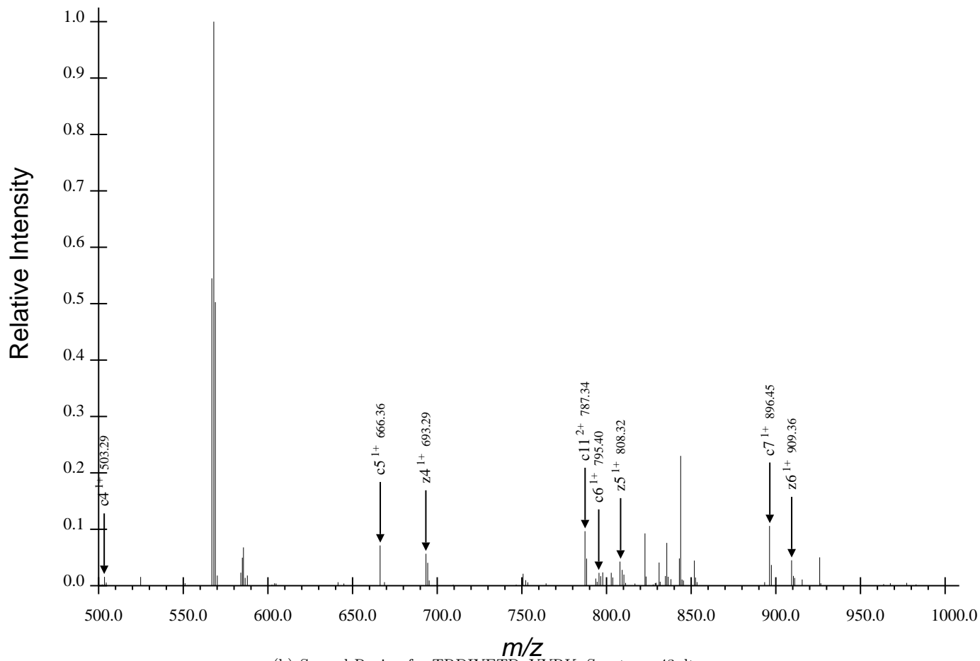
(b) Second Region for TRDIYETDpYYRK, Spectrum 43.dta
