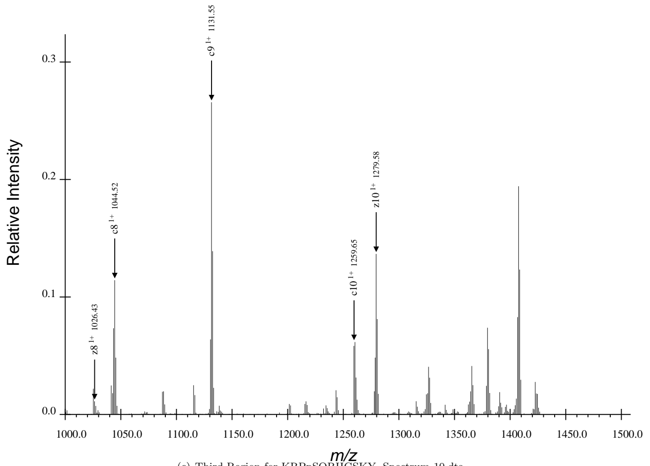
(c) Third Region for KRPpSQRHGSKY, Spectrum 10.dta
