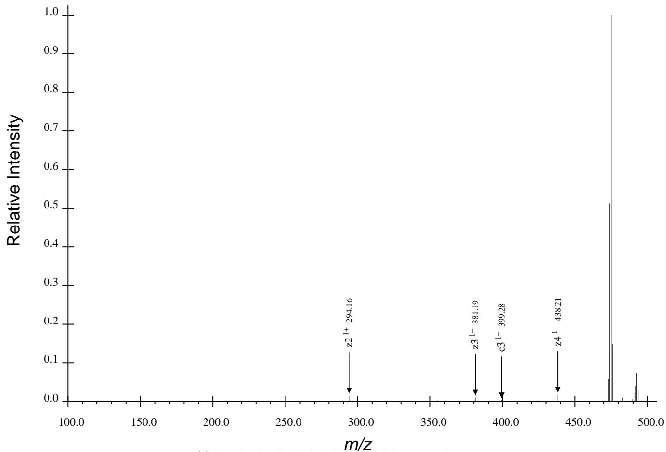
(a) First Region for KRPPSQRHGSKY, Spectrum 4.dta
