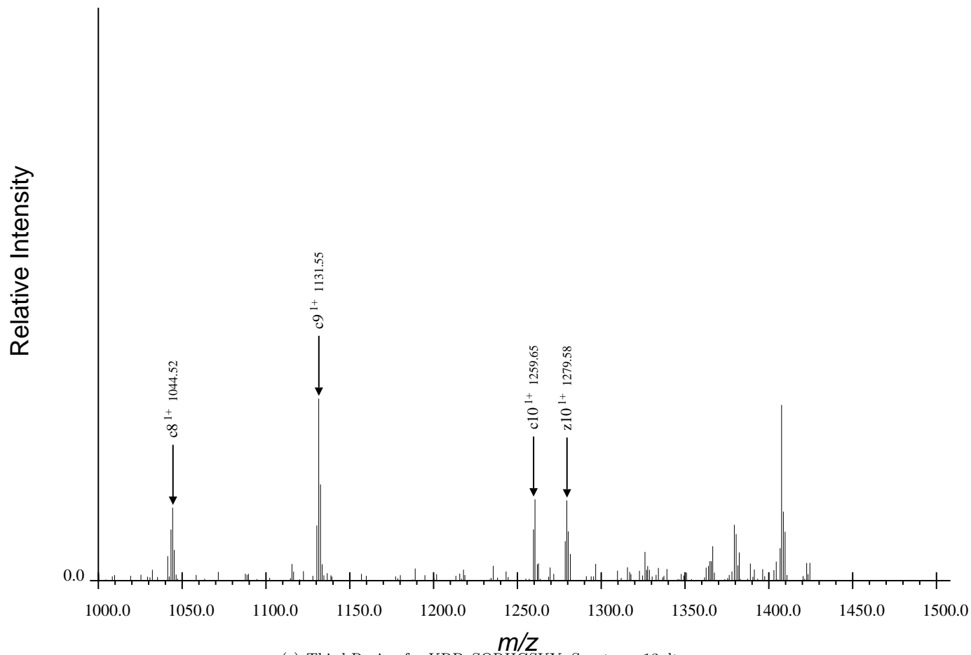
(c) Third Region for KRPPSQRHGSKY, Spectrum 13.dta
