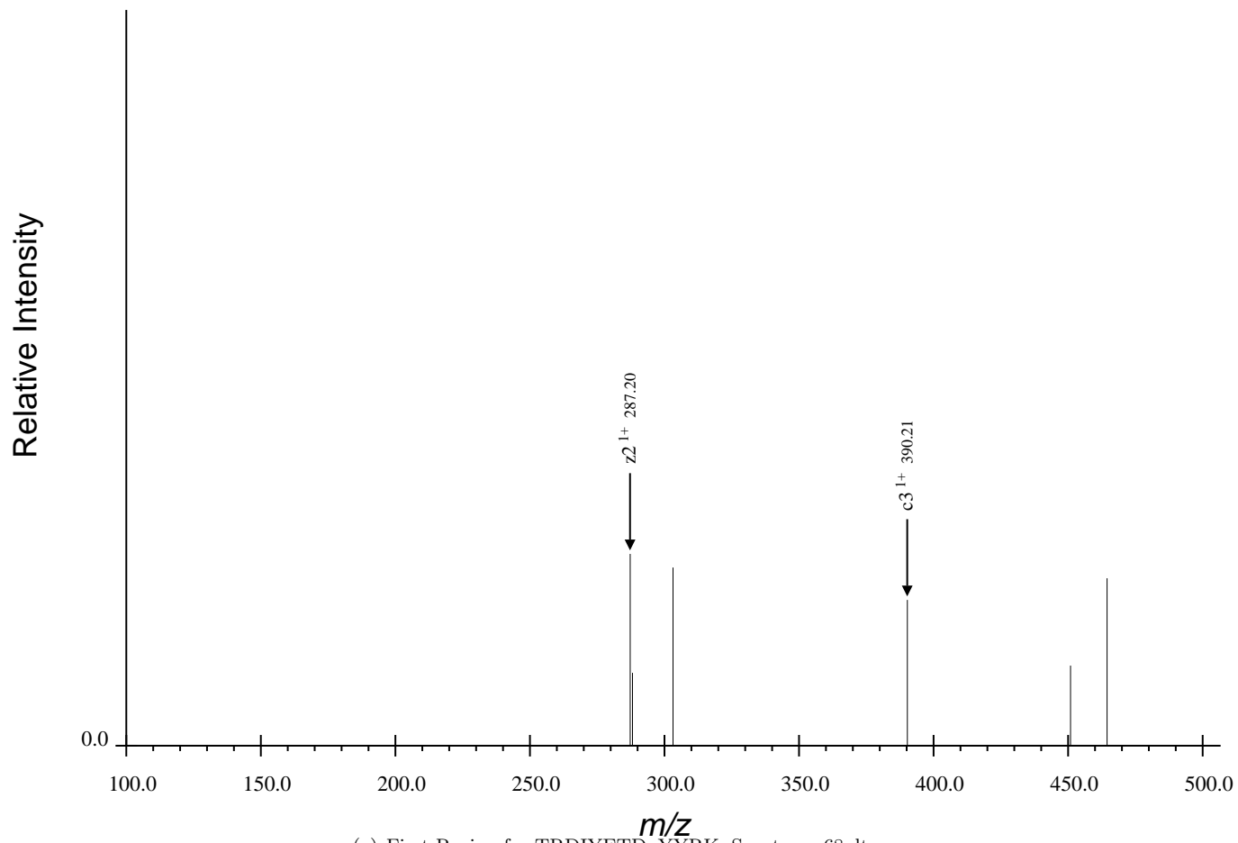
(a) First Region for TRDIYETDpYYRK, Spectrum 68.dta
