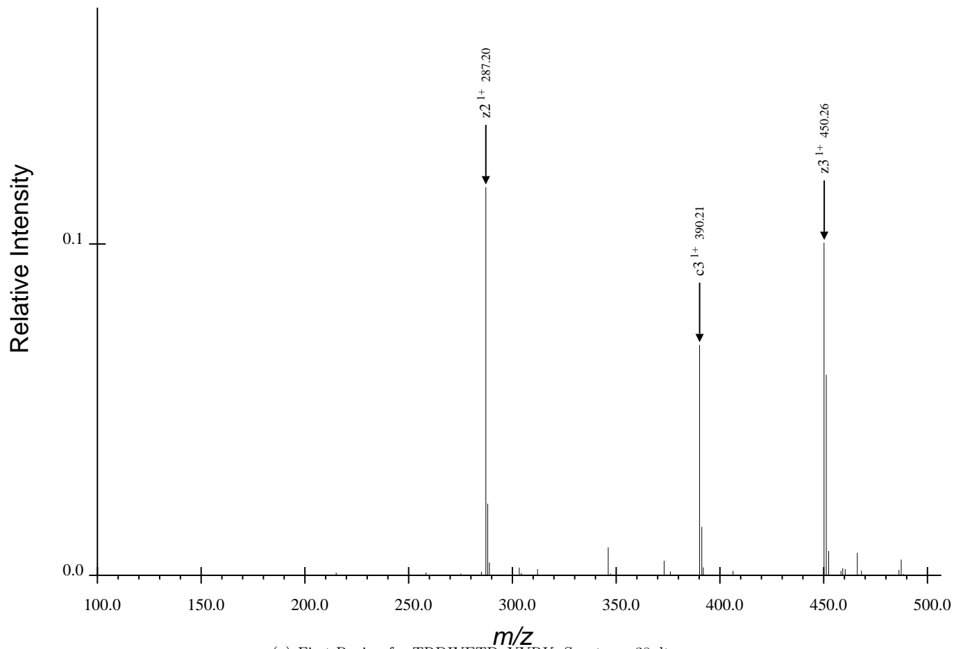
(a) First Region for TRDIYETDpYYRK, Spectrum 38.dta
