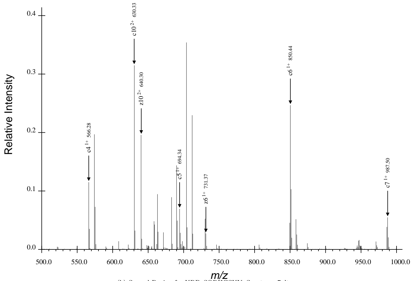
(b) Second Region for KRPpSQRHGSKY, Spectrum 7.dta
