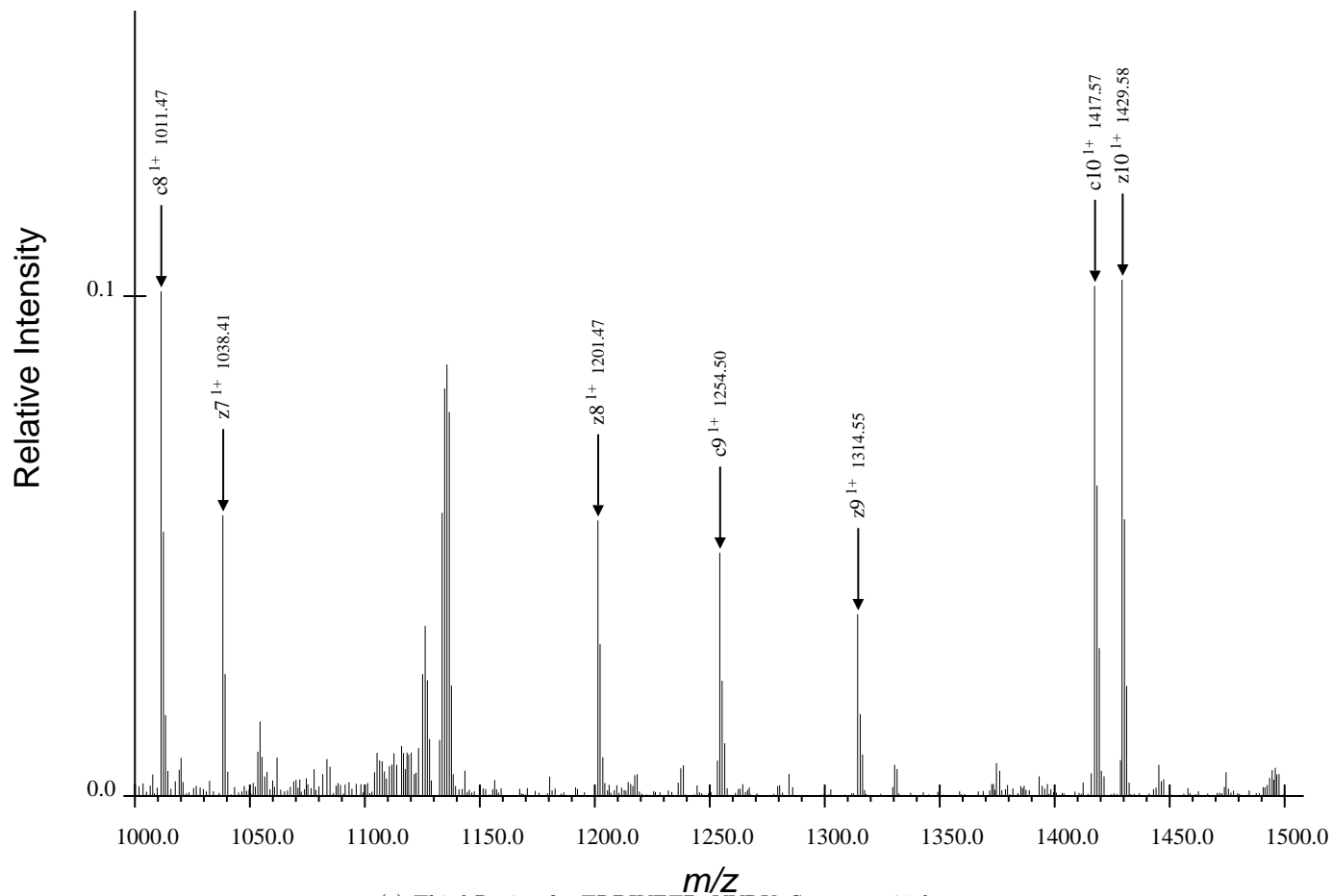
(c) Third Region for TRDIYETDpYYRK, Spectrum 46.dta
