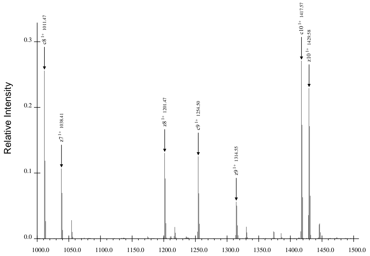
(c) Third Region for TRDIYETDpYYRK, Spectrum 39.dta
