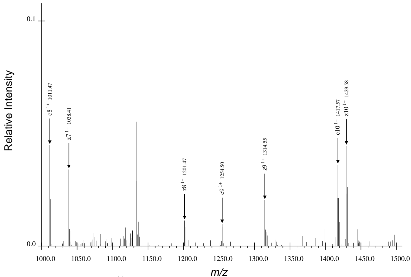
(c) Third Region for TRDIYETDpYYRK, Spectrum 53.dta
