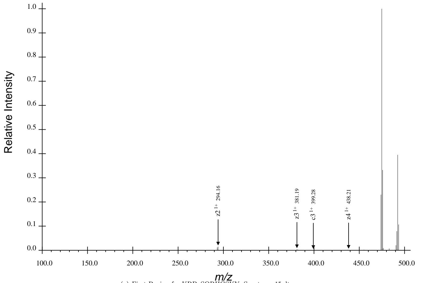
(a) First Region for KRPpSQRHGSKY, Spectrum 15.dta
