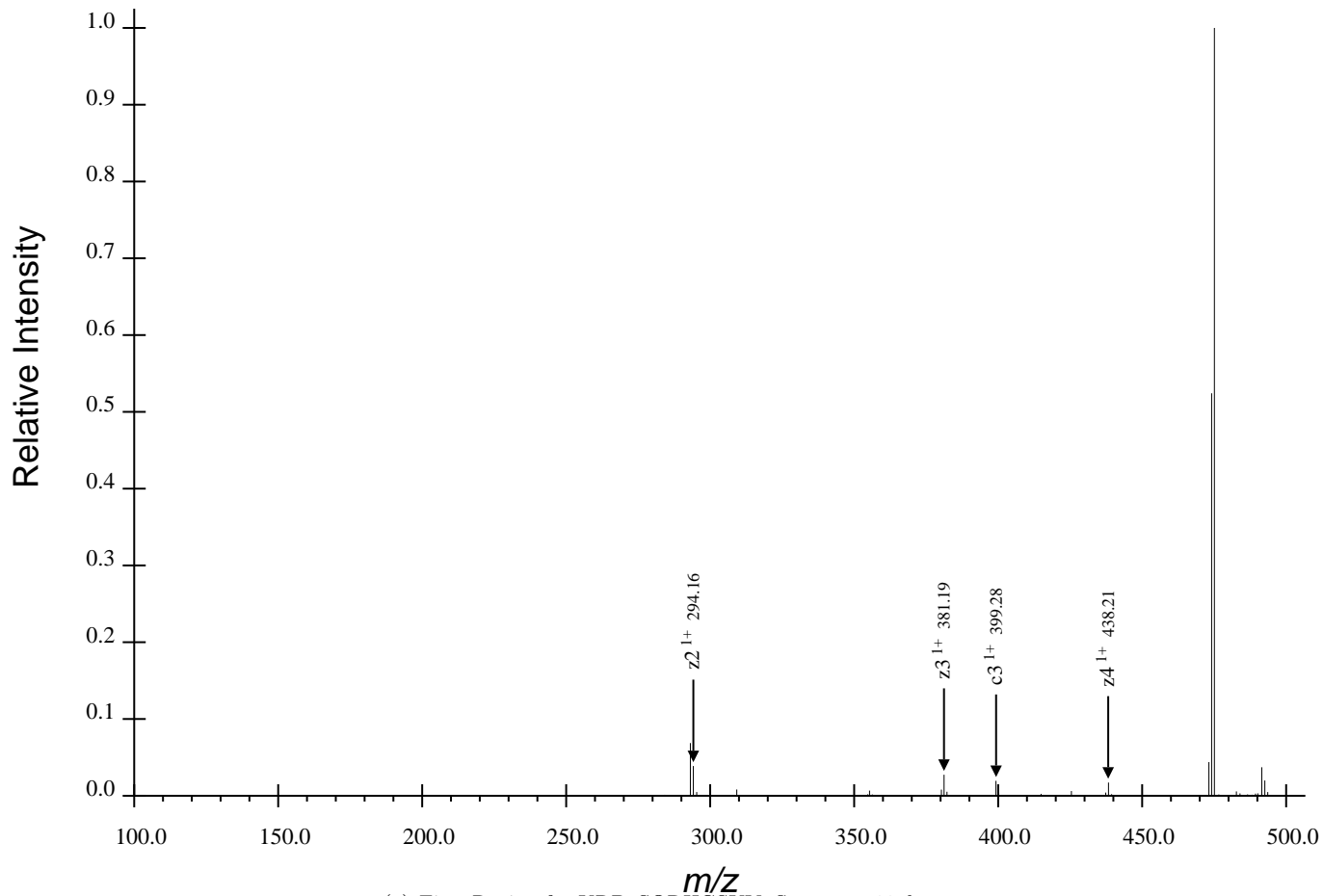
(a) First Region for KRPpSQRHGSKY, Spectrum 11.dta
