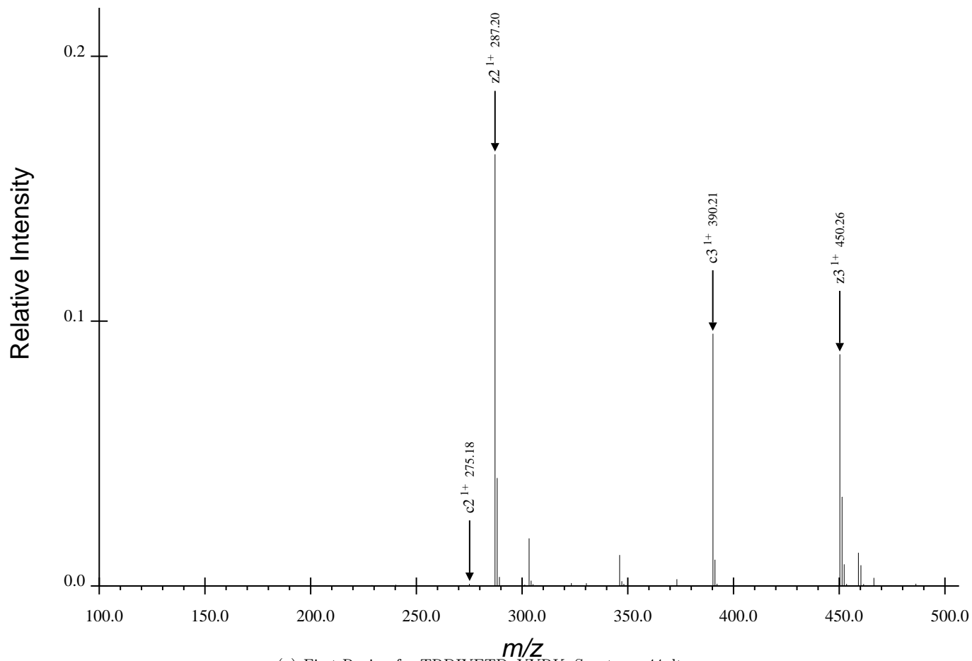
(a) First Region for TRDIYETDpYYRK, Spectrum 44.dta
