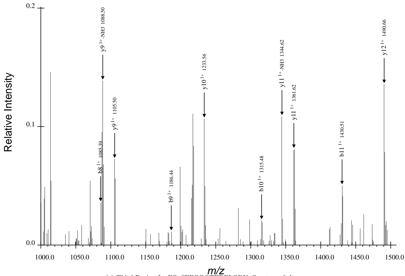
(c) Third Region for FQpSEEQQQTEDELQDK, Spectrum 3.dta
