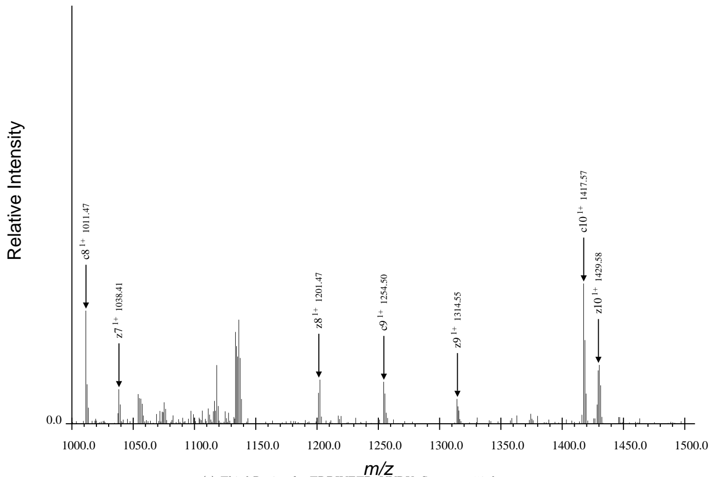
(c) Third Region for TRDIYETDpYYRK, Spectrum 50.dta
