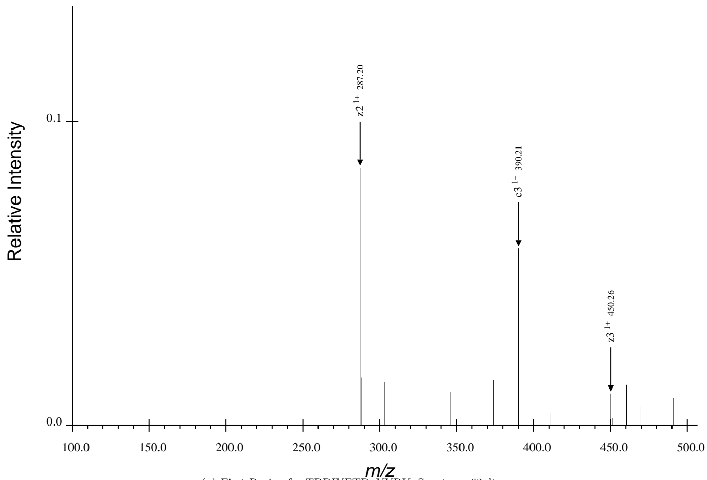
(a) First Region for TRDIYETDpYYRK, Spectrum 63.dta
