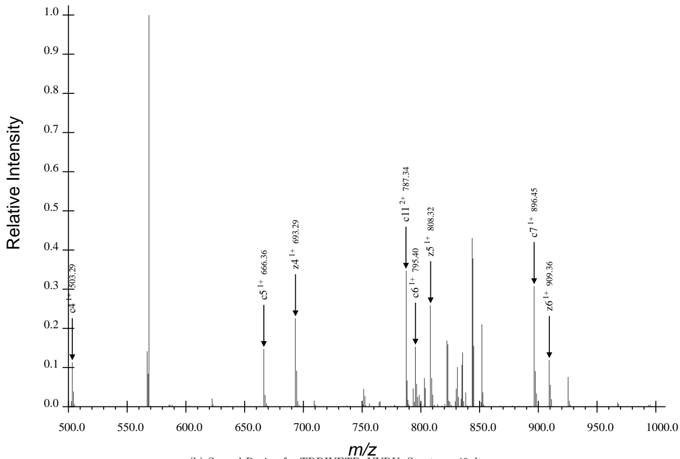
(b) Second Region for TRDIYETDpYYRK, Spectrum 40.dta
