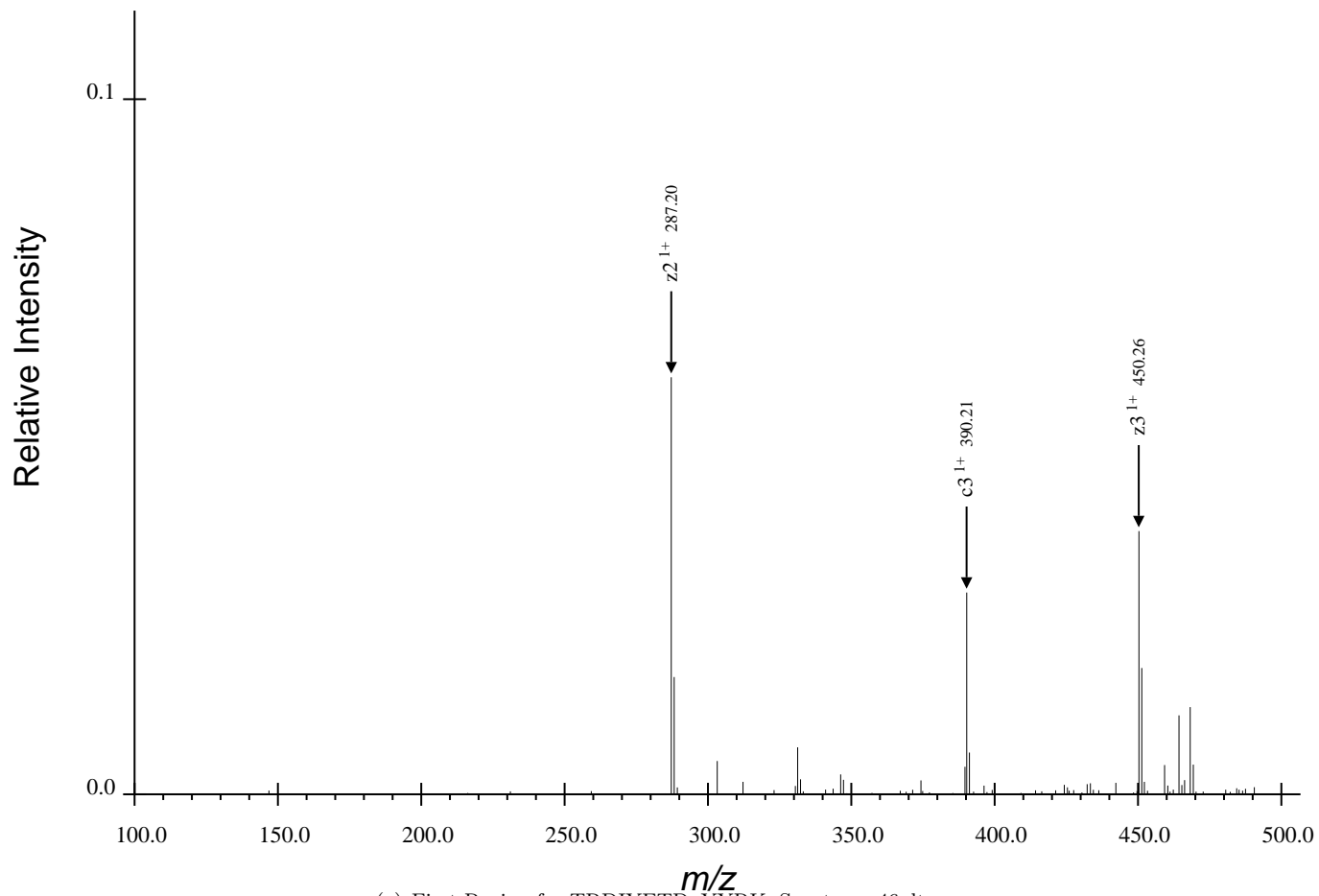
(a) First Region for TRDIYETDpYYRK, Spectrum 46.dta
