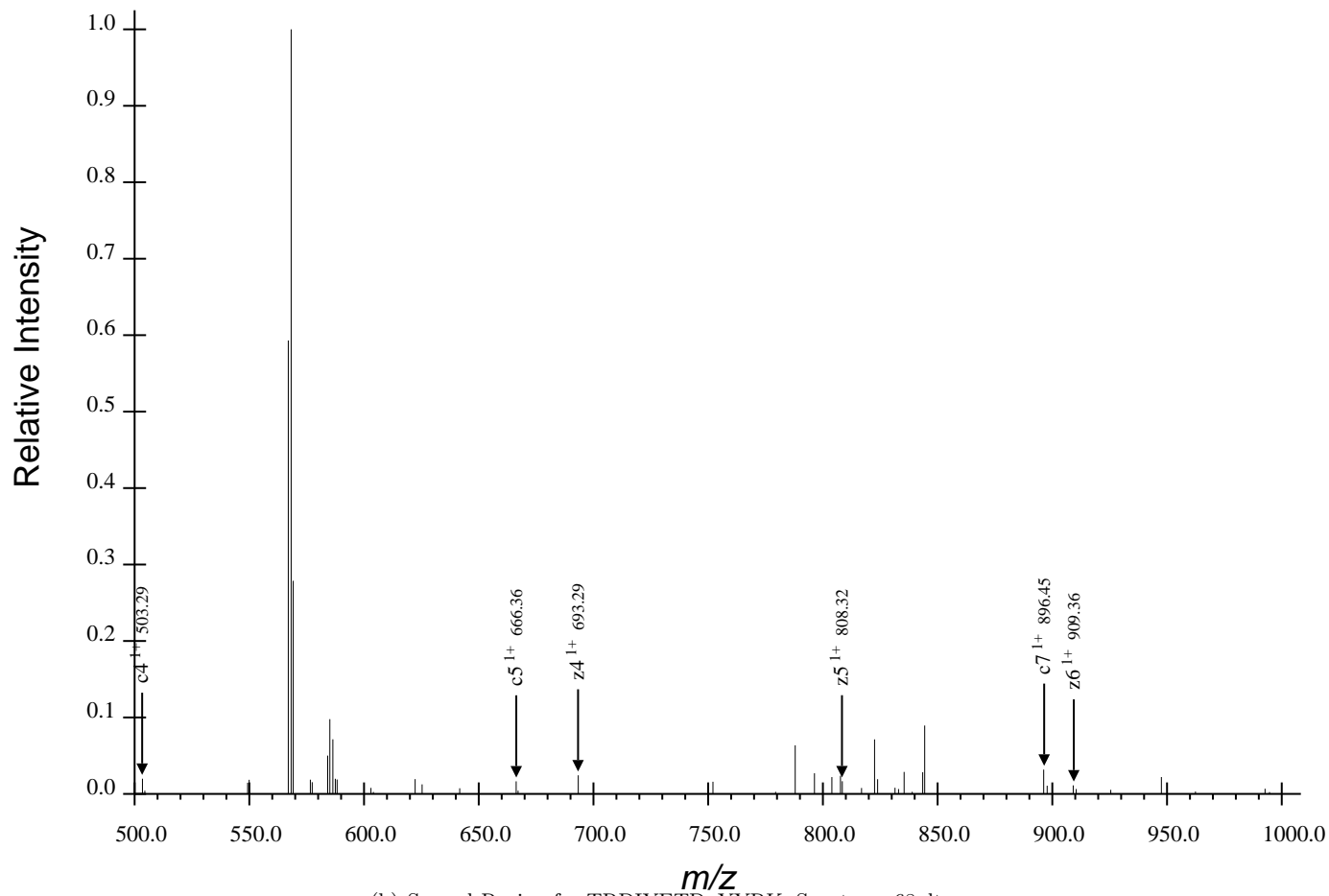
(b) Second Region for TRDIYETDpYYRK, Spectrum 68.dta
