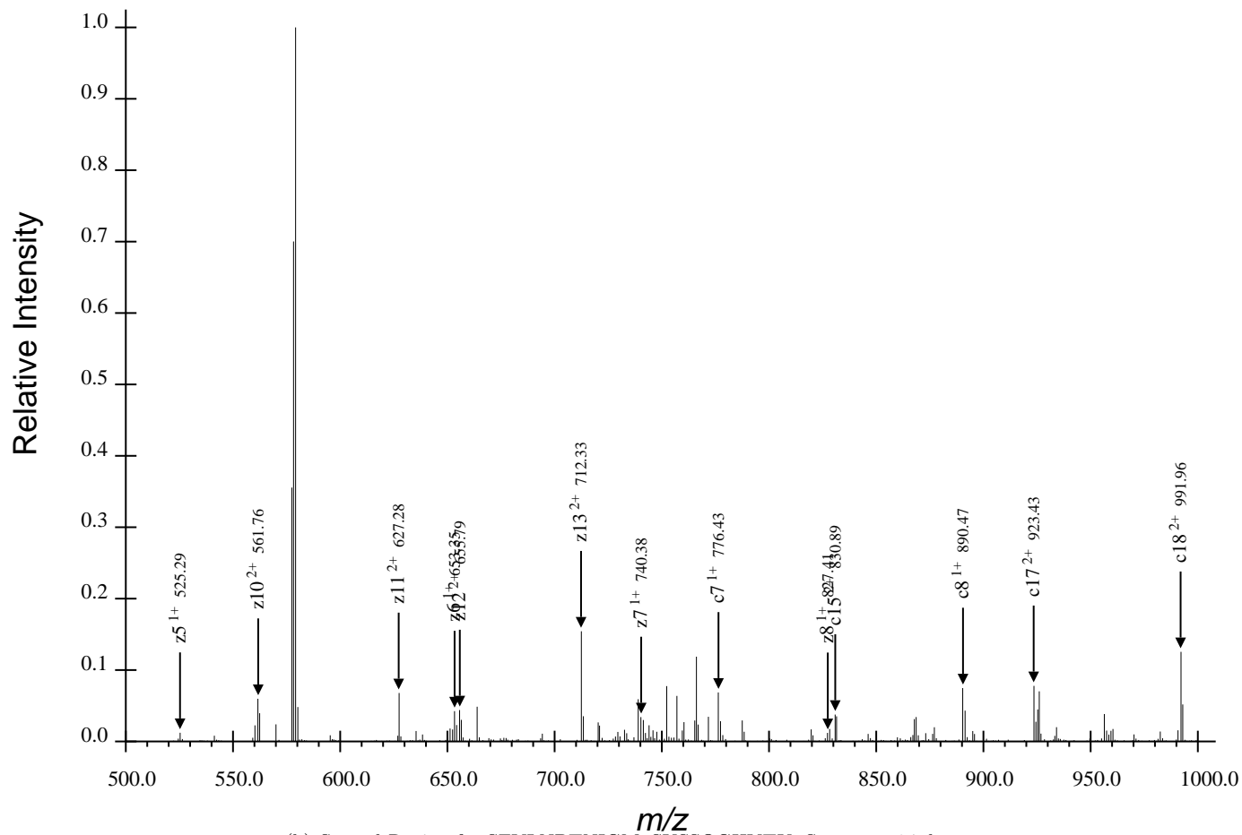
(b) Second Region for SFVLNPTNIGMpSKSSQGHVTK, Spectrum 24.dta
