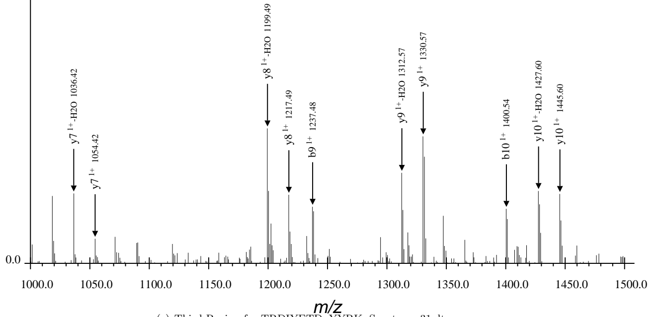
(c) Third Region for TRDIYETDpYYRK, Spectrum 31.dta
