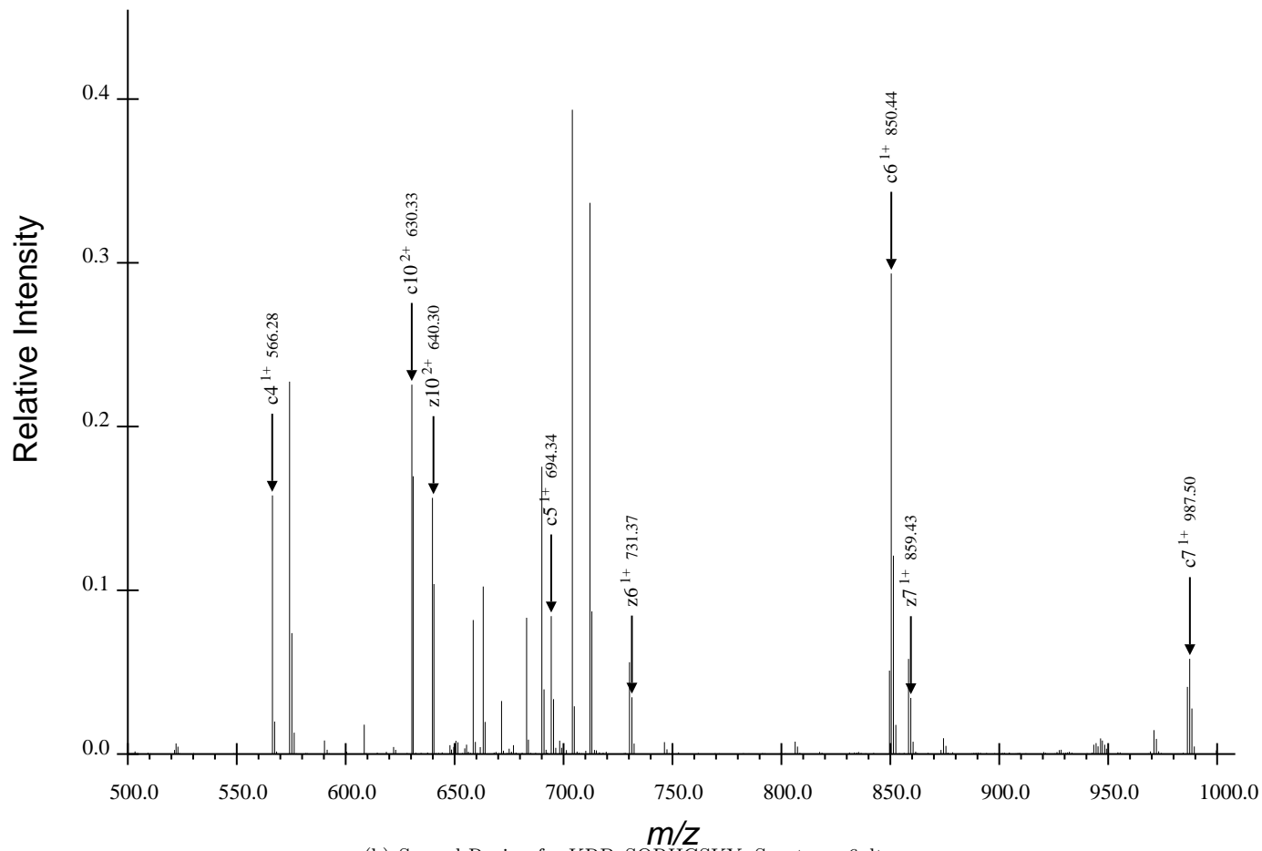
(b) Second Region for KRPPSQRHGSKY, Spectrum 6.dta
