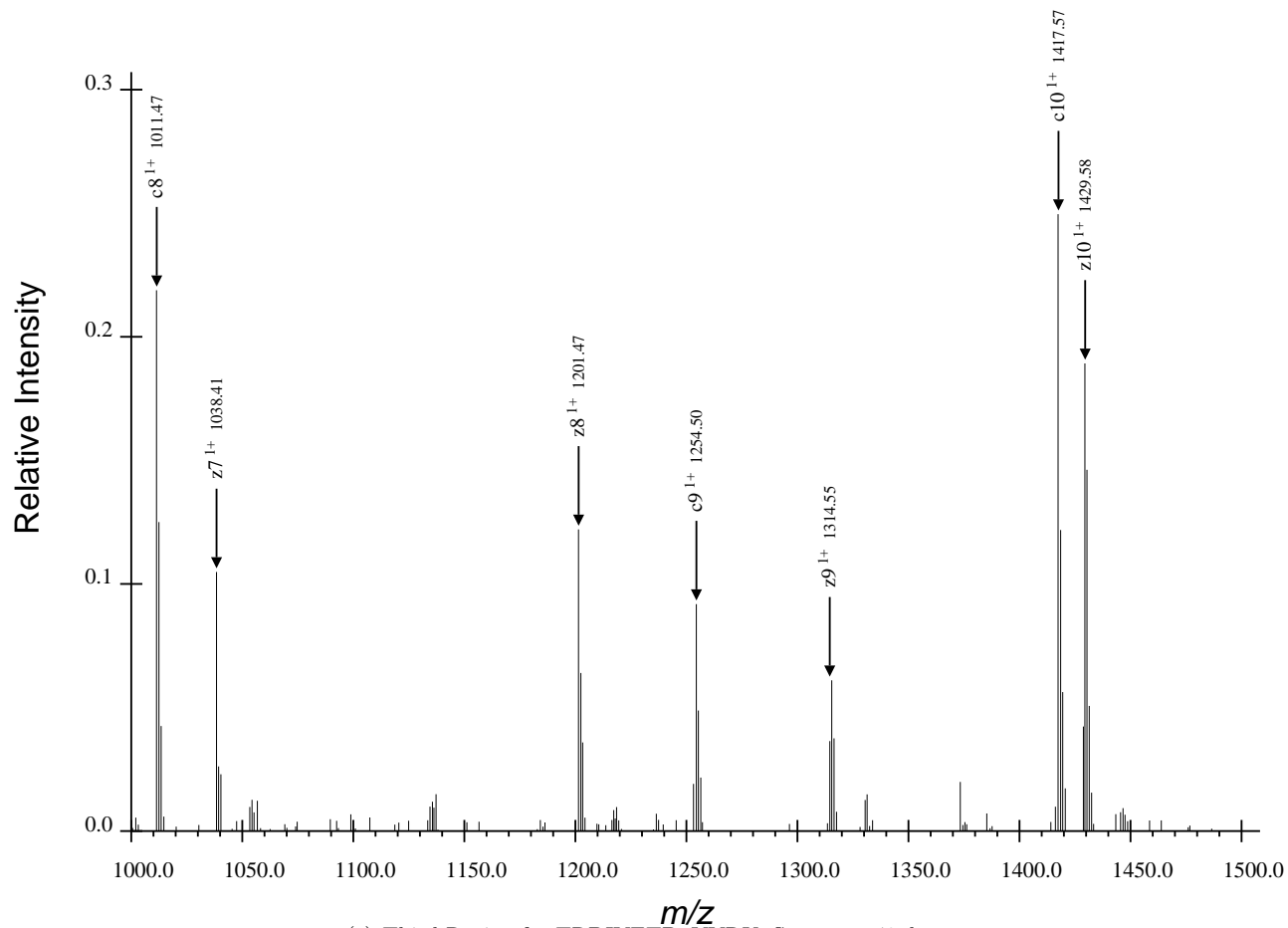
(c) Third Region for TRDIYETDpYYRK, Spectrum 42.dta
