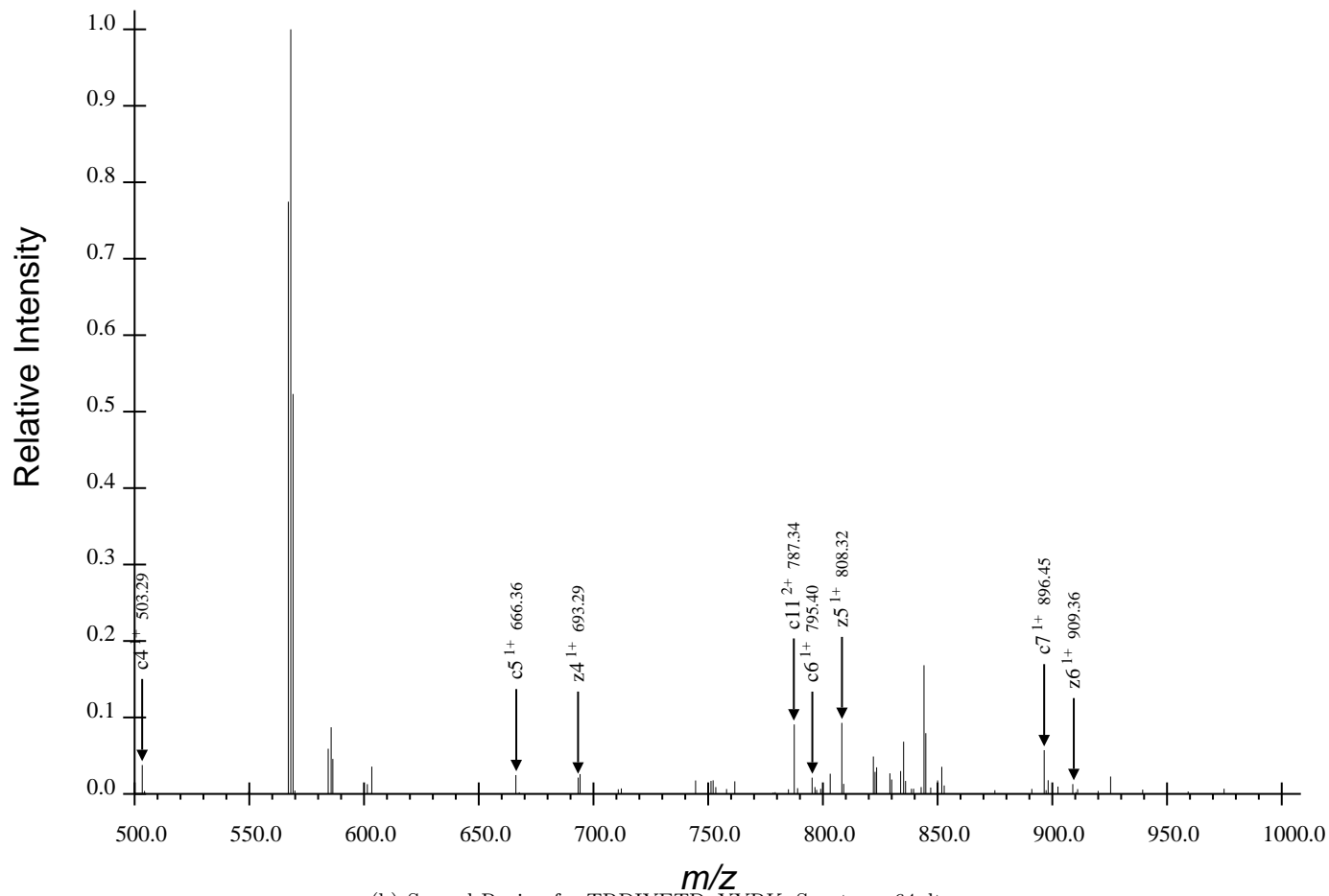
(b) Second Region for TRDIYETDpYYRK, Spectrum 64.dta
