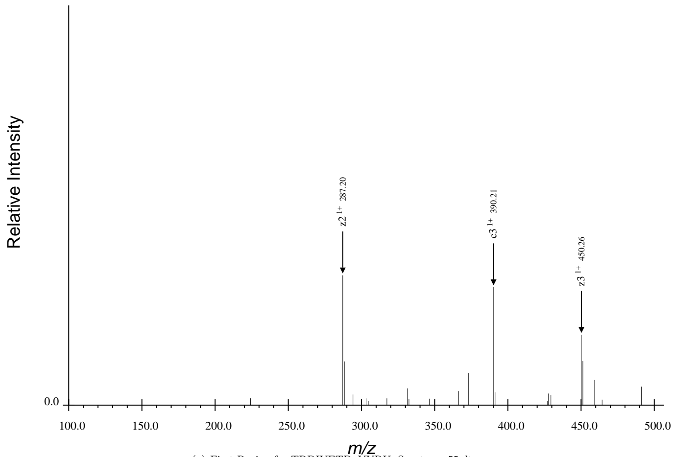
(a) First Region for TRDIYETDpYYRK, Spectrum 55.dta
