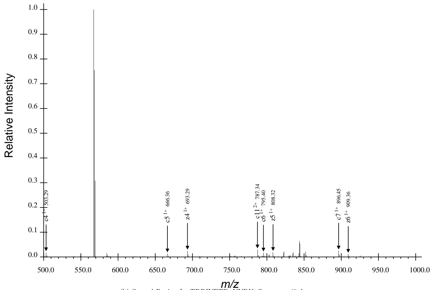
(b) Second Region for TRDIYETDpYYRK, Spectrum 49.dta
