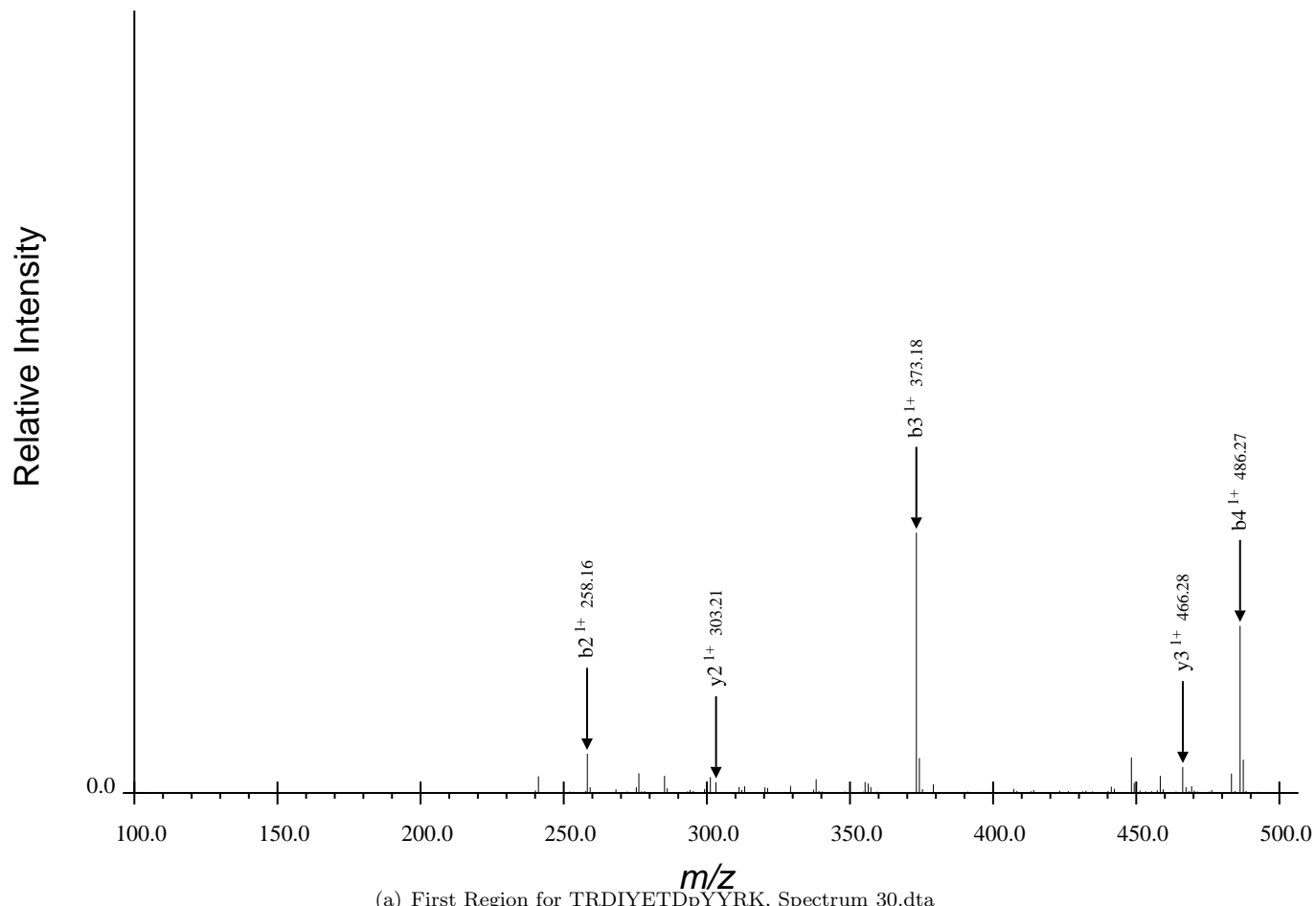
(a) First Region for TRDIYETDpYYRK, Spectrum 30.dta
