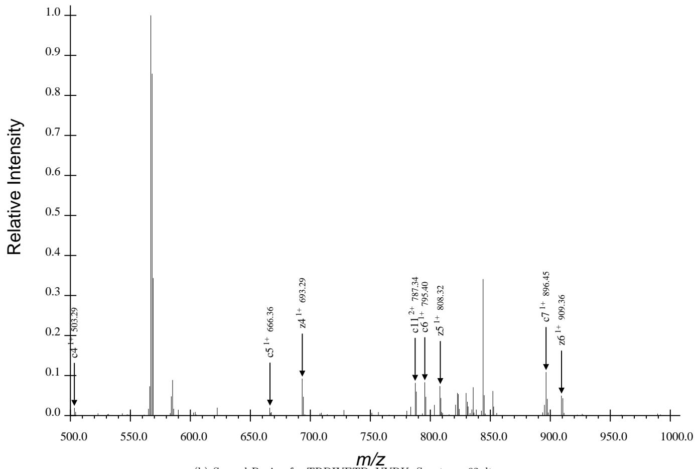
(b) Second Region for TRDIYETDpYYRK, Spectrum 62.dta
