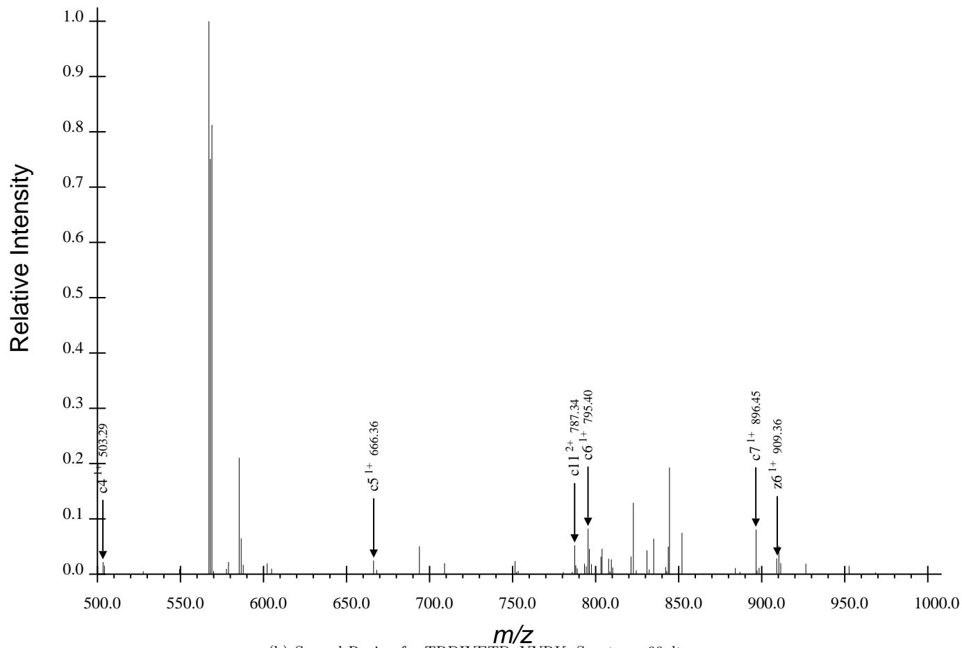
(b) Second Region for TRDIYETDpYYRK, Spectrum 66.dta
