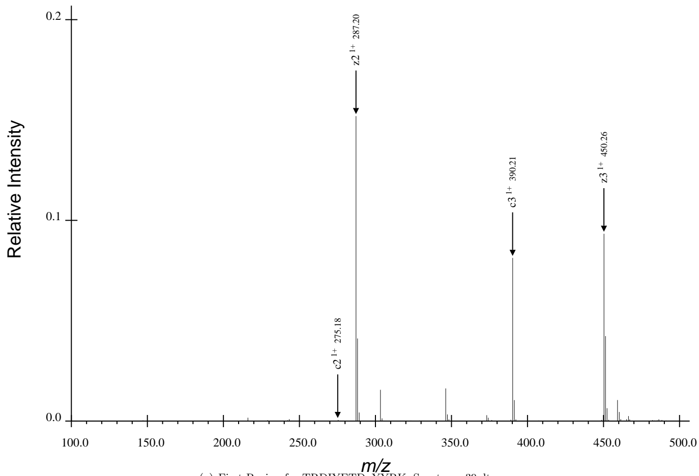
(a) First Region for TRDIYETDpYYRK, Spectrum 39.dta
