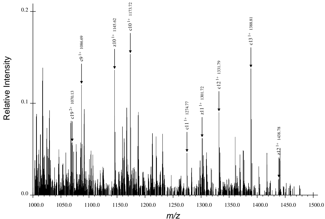
(c) Third Region for ARTKQTARdKSTGGaKAPRKQLATaKAARdKSAPATGGVdKKPHRYRPGTVALRE, Spectrum 40.dta
