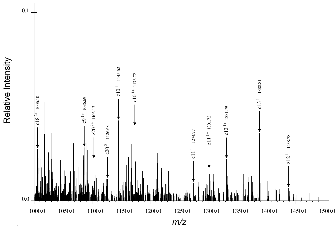
(c) Third Region for ARTKQTARdKSTGGaKAPRKQLATaKAARdKSAPATGGVdKKPHRYRPGTVALRE, Spectrum 1.dta
