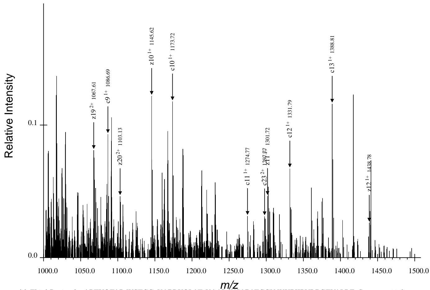
(c) Third Region for ARTKQTARdKSTGGaKAPRKQLATaKAARdKSAPATGGVdKKPHRYRPGTVALRE, Spectrum 20.dta
