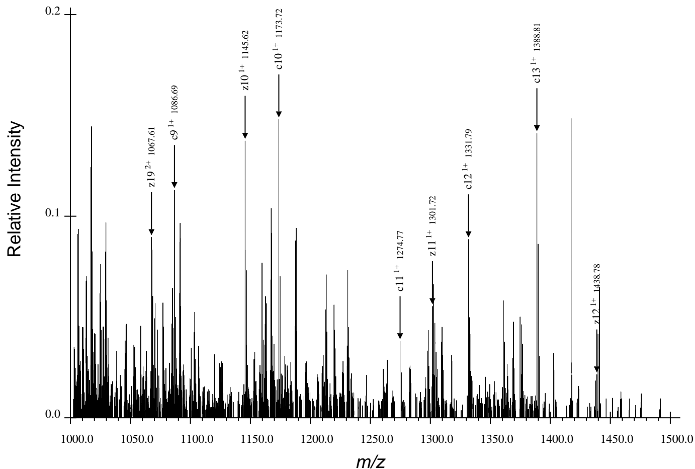
(c) Third Region for ARTKQTARdKSTGGaKAPRKQLATaKAARdKSAPATGGVdKKPHRYRPGTVALRE, Spectrum 35.dta
