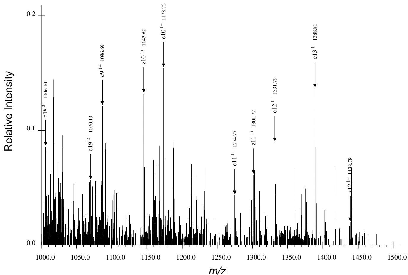
(c) Third Region for ARTKQTARdKSTGGaKAPRKQLATaKAARdKSAPATGGVdKKPHRYRPGTVALRE, Spectrum 41.dta
