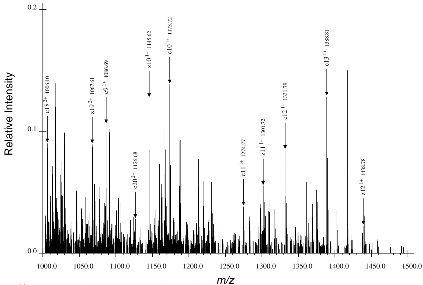
(c) Third Region for ARTKQTARdKSTGGaKAPRKQLATaKAARdKSAPATGGVdKKPHRYRPGTVALRE, Spectrum 29.dta
