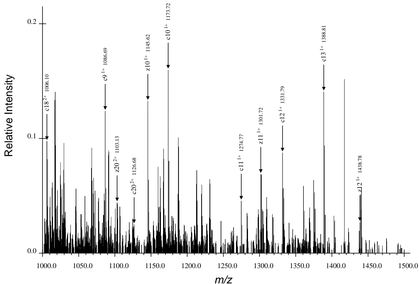
(c) Third Region for ARTKQTARdKSTGGaKAPRKQLATaKAARdKSAPATGGVdKKPHRYRPGTVALRE, Spectrum 52.dta
