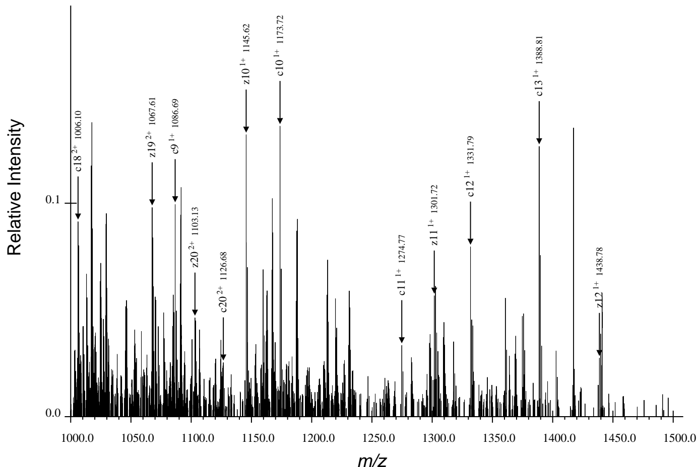
(c) Third Region for ARTKQTARdKSTGGaKAPRKQLATaKAARdKSAPATGGVdKKPHRYRPGTVALRE, Spectrum 25.dta
