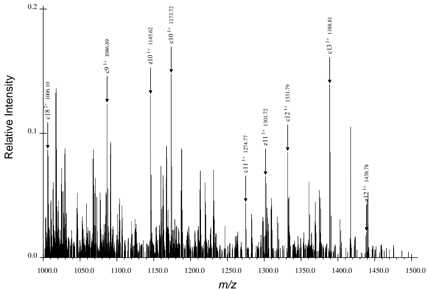
(c) Third Region for ARTKQTARdKSTGGaKAPRKQLATaKAARdKSAPATGGVdKKPHRYRPGTVALRE, Spectrum 45.dta
