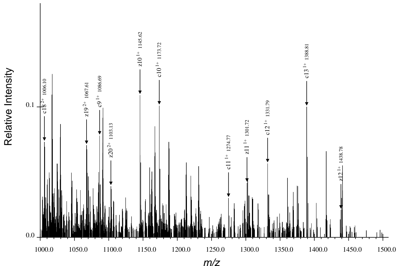
(c) Third Region for ARTKQTARdKSTGGaKAPRKQLATaKAARdKSAPATGGVdKKPHRYRPGTVALRE, Spectrum 18.dta
