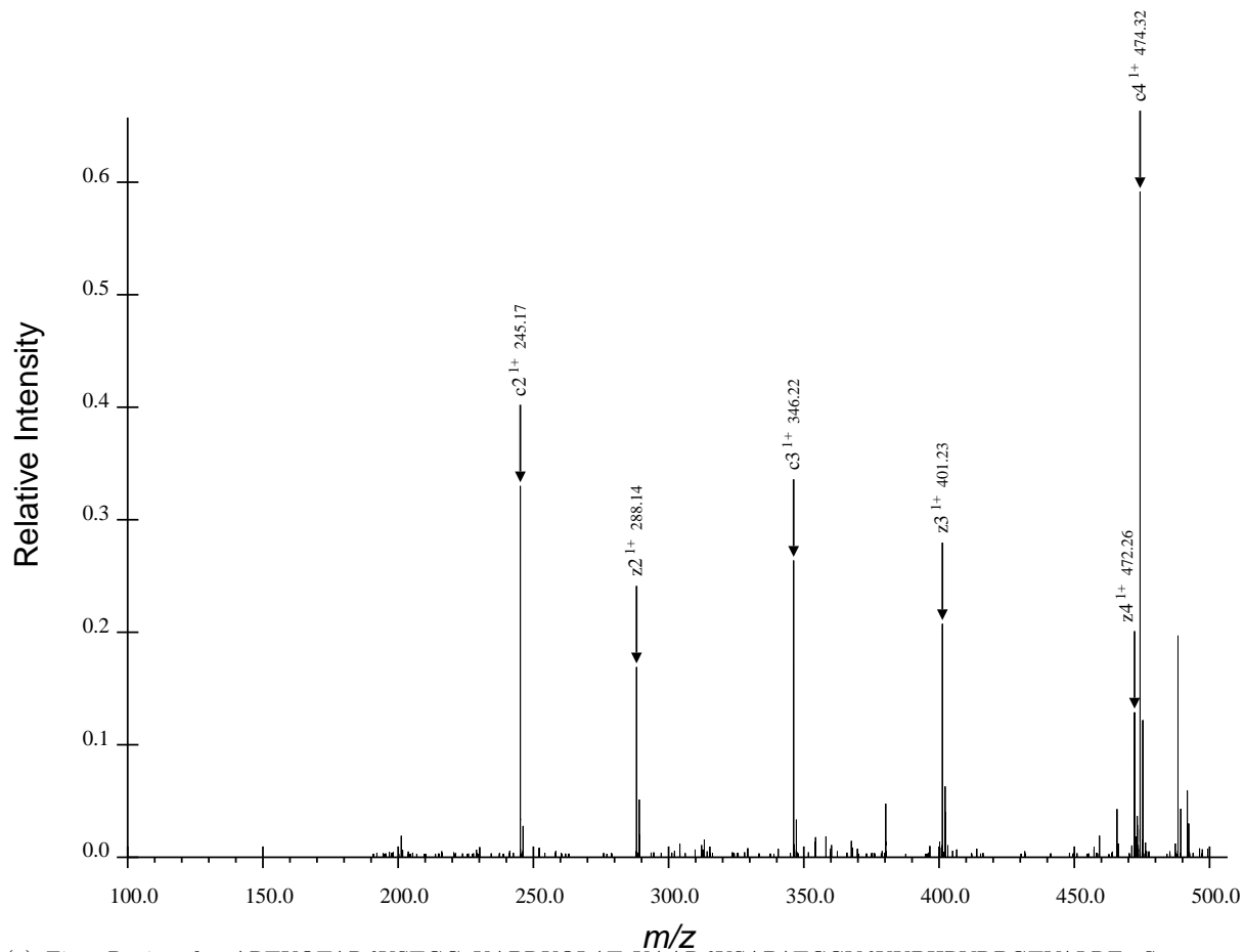
(a) First Region for ARTKQTARdKSTGGaKAPRKQLATaKAARdKSAPATGGVdKKPHRYRPGTVALRE, Spectrum 51.dta
