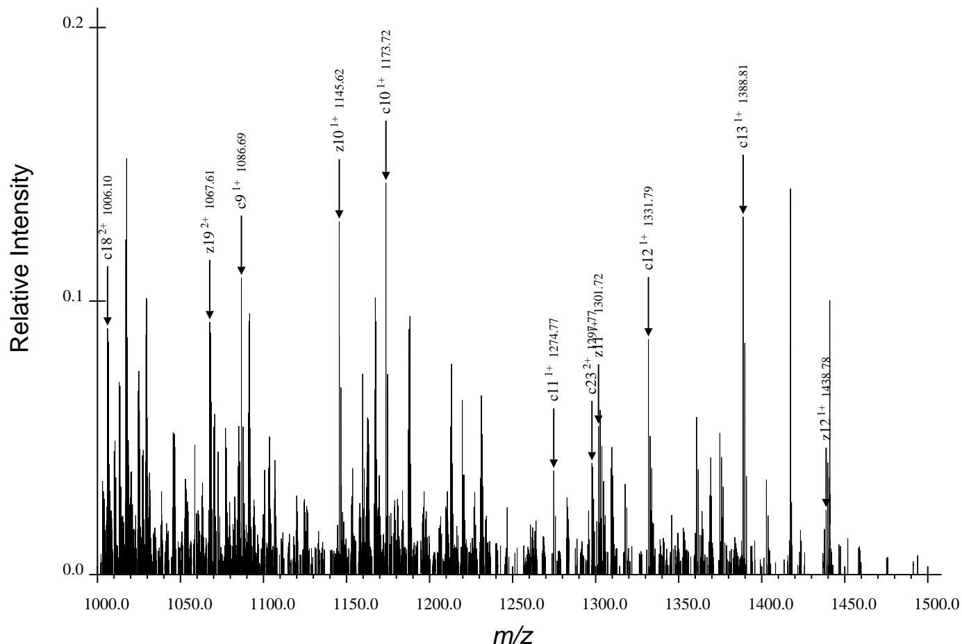
(c) Third Region for ARTKQTARdKSTGGaKAPRKQLATaKAARdKSAPATGGVdKKPHRYRPGTVALRE, Spectrum 31.dta
