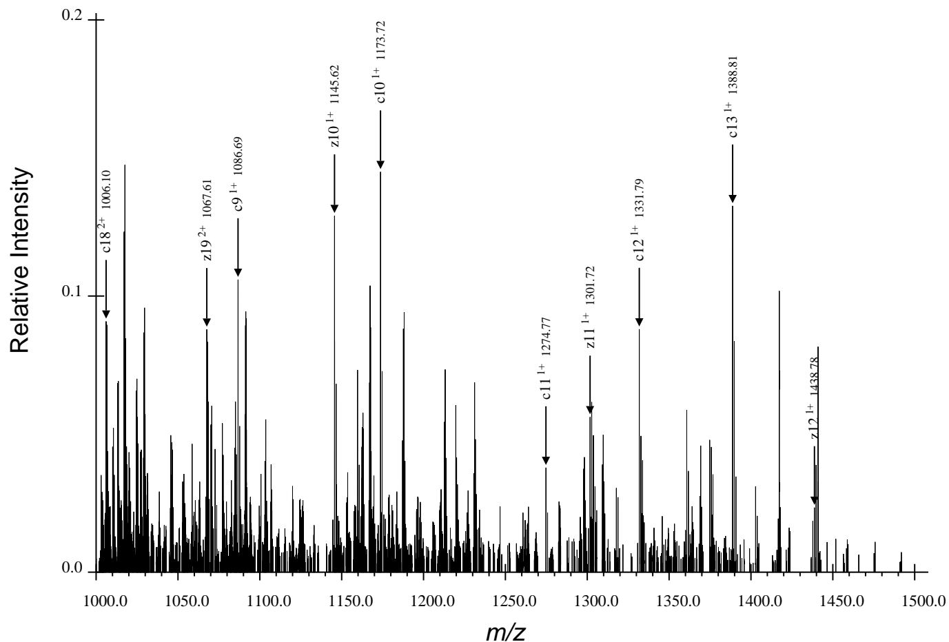
(c) Third Region for ARTKQTARdKSTGGaKAPRKQLATaKAARdKSAPATGGVdKKPHRYRPGTVALRE, Spectrum 33.dta
