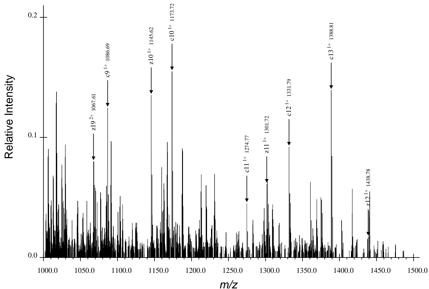
(c) Third Region for ARTKQTARdKSTGGaKAPRKQLATaKAARdKSAPATGGVdKKPHRYRPGTVALRE, Spectrum 39.dta
