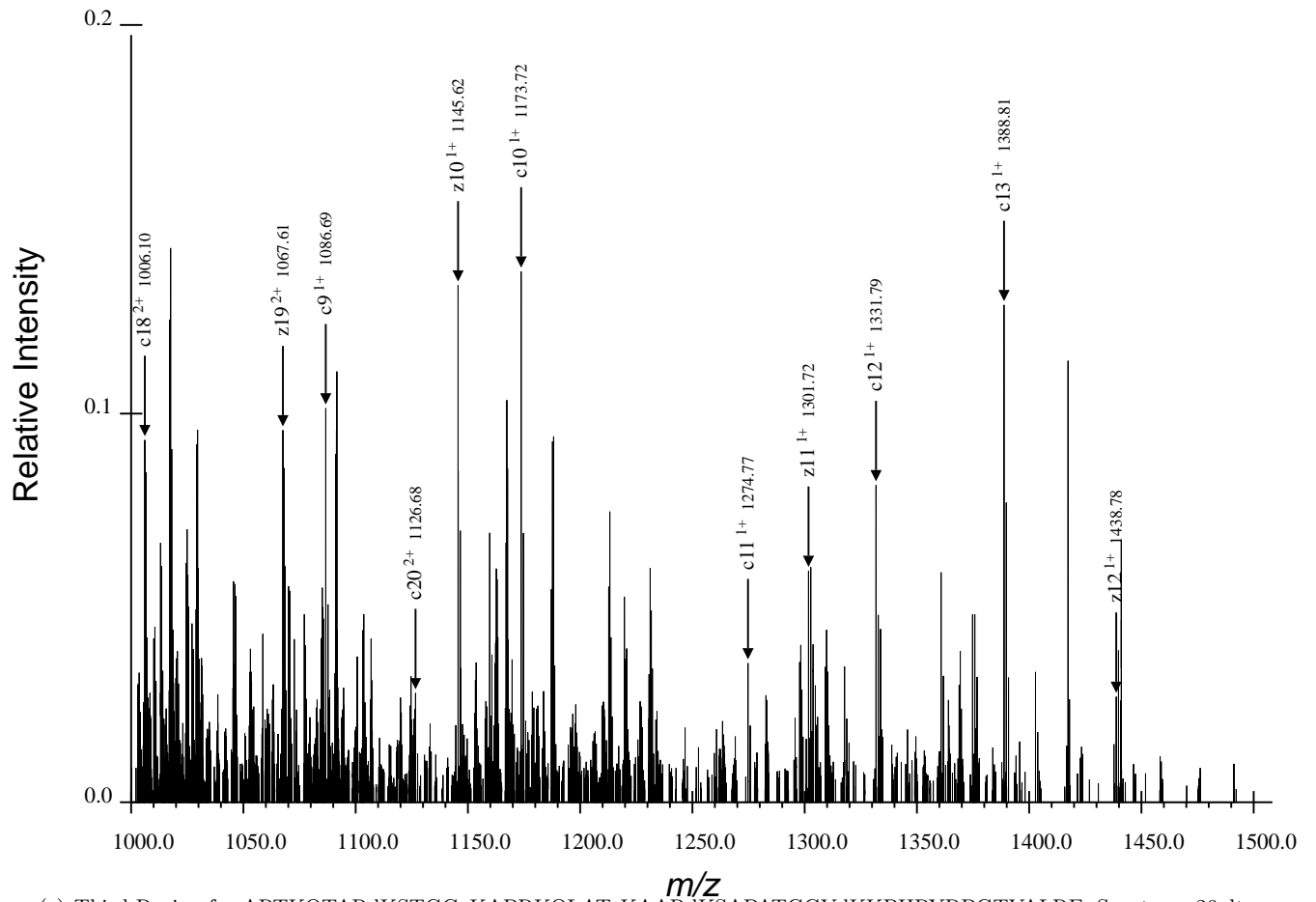
(c) Third Region for ARTKQTARdKSTGGaKAPRKQLATaKAARdKSAPATGGVdKKPHRYRPGTVALRE, Spectrum 26.dta
