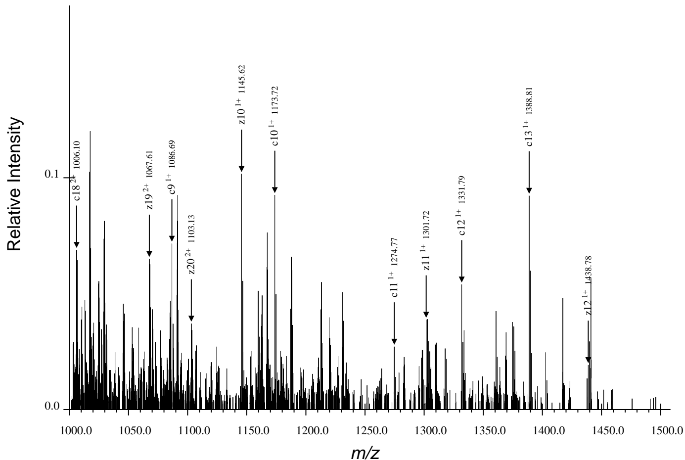
(c) Third Region for ARTKQTARdKSTGGaKAPRKQLATaKAARdKSAPATGGVdKKPHRYRPGTVALRE, Spectrum 17.dta
