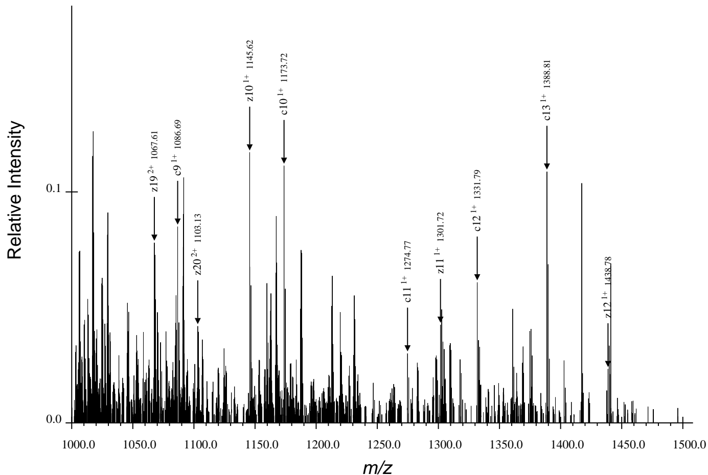
(c) Third Region for ARTKQTARdKSTGGaKAPRKQLATaKAARdKSAPATGGVdKKPHRYRPGTVALRE, Spectrum 19.dta
