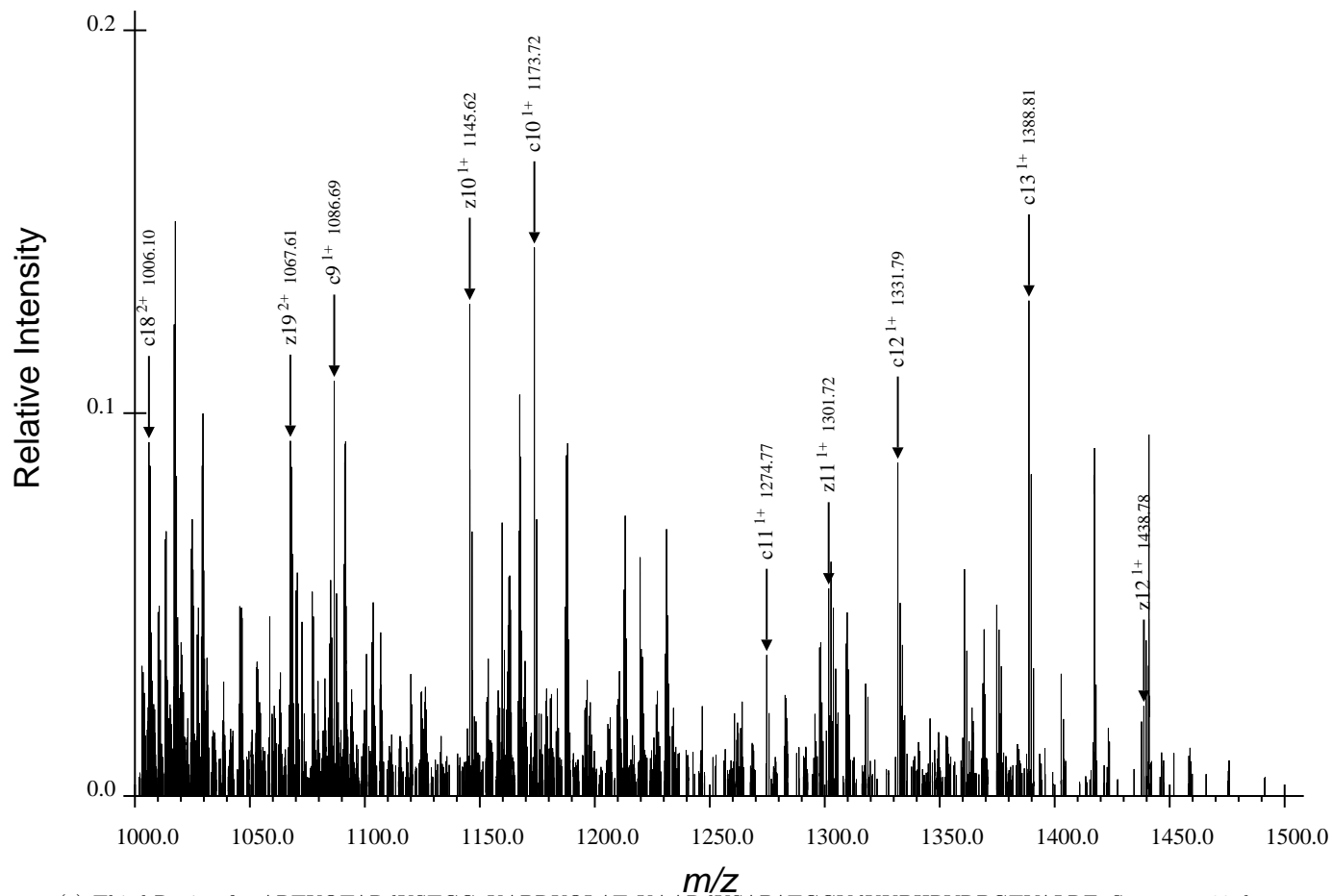
(c) Third Region for ARTKQTARdKSTGGaKAPRKQLATaKAARdKSAPATGGVdKKPHRYRPGTVALRE, Spectrum 32.dta
