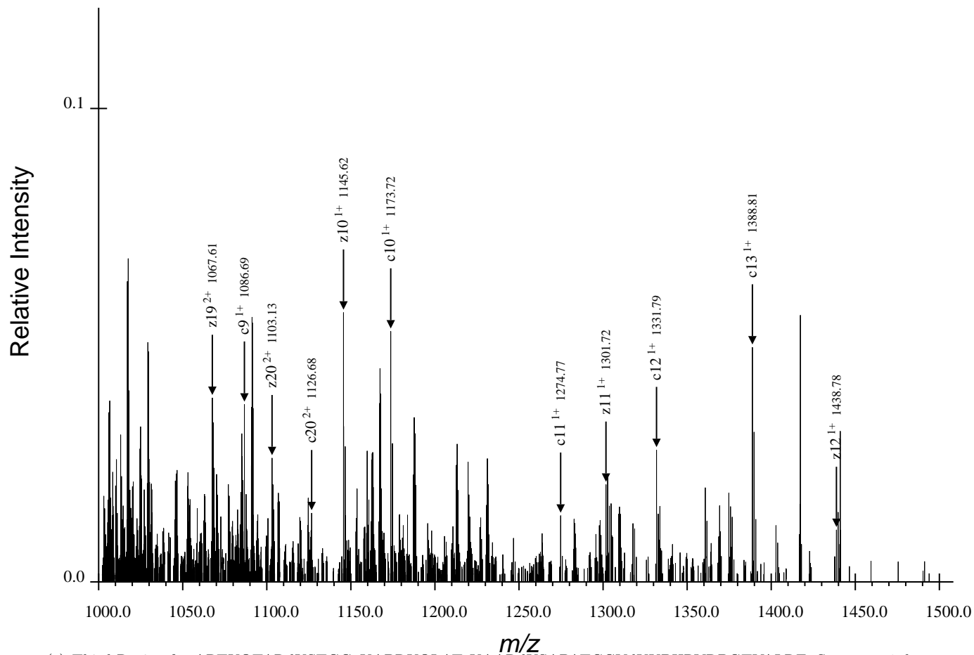
(c) Third Region for ARTKQTARdKSTGGaKAPRKQLATaKAARdKSAPATGGVdKKPHRYRPGTVALRE, Spectrum 8.dta
