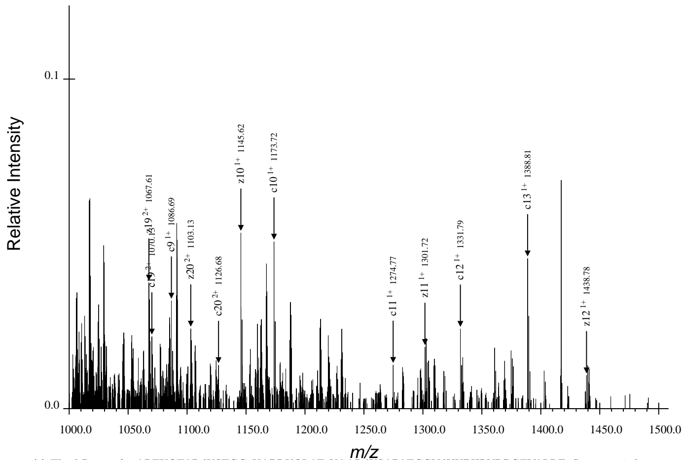
(c) Third Region for ARTKQTARdKSTGGaKAPRKQLATaKAARdKSAPATGGVdKKPHRYRPGTVALRE, Spectrum 7.dta
