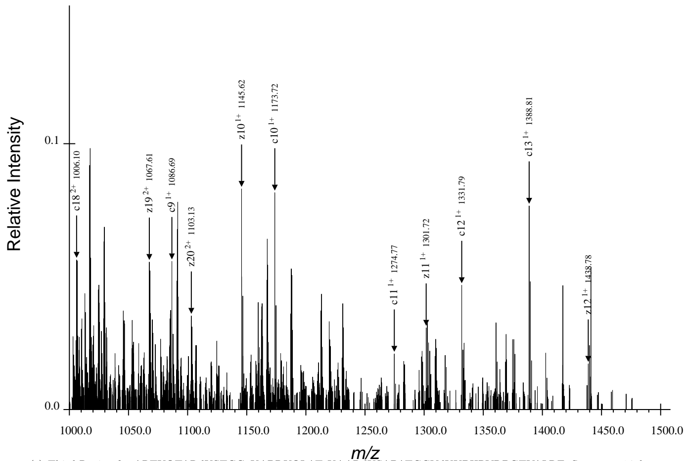
(c) Third Region for ARTKQTARdKSTGGaKAPRQLATaKAARdKSAPATGGVdKKPHRYRPGTVALRE, Spectrum 14.dta
