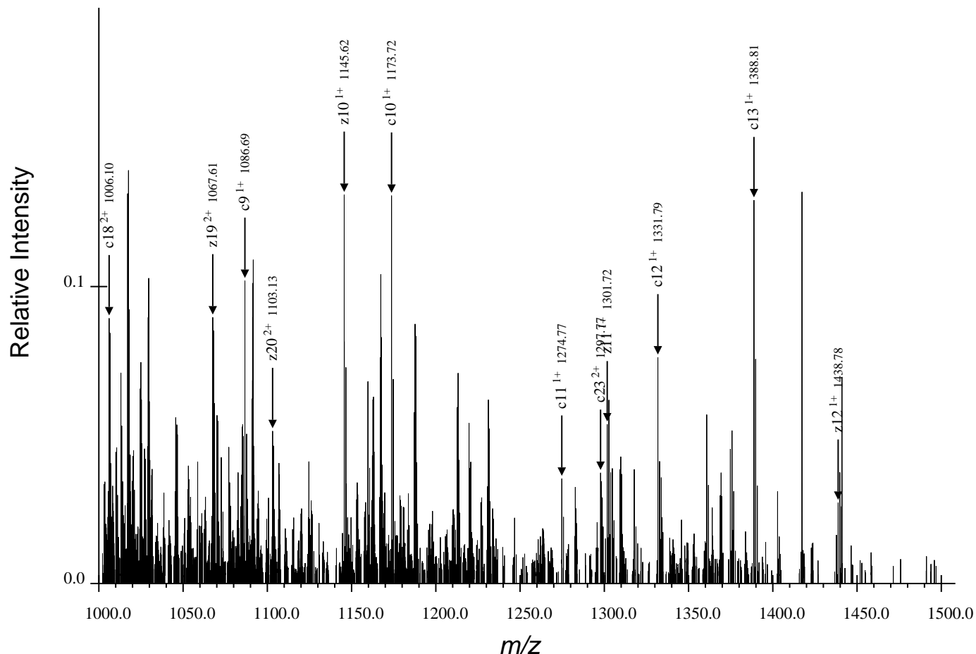
(c) Third Region for ARTKQTARdKSTGGaKAPRKQLATaKAARdKSAPATGGVdKKPHRYRPGTVALRE, Spectrum 22.dta
