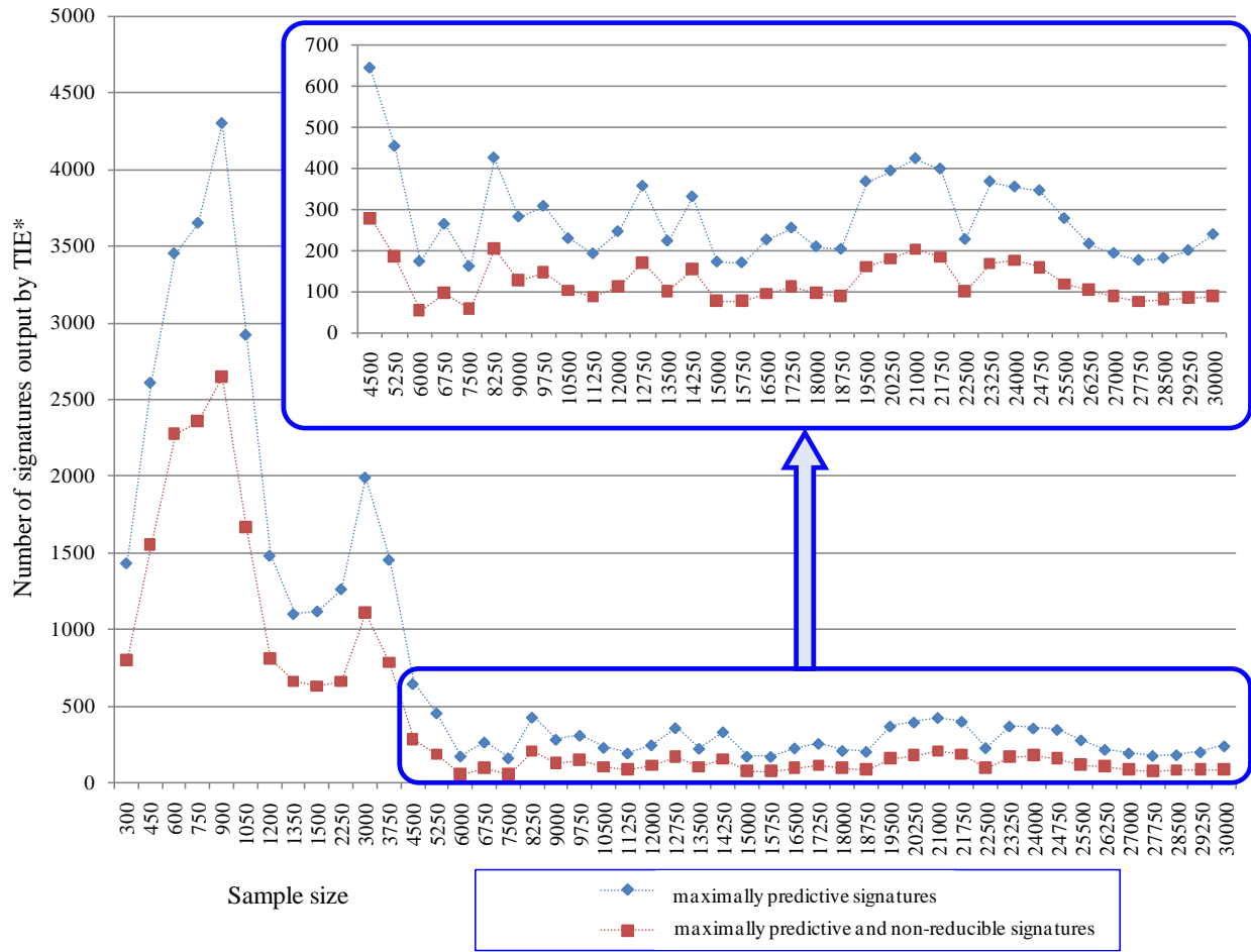
Figure S3: Number of signatures output by TIE* as sample size grows. The inner figure is a magnified region of the main figure.
