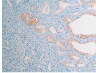
Figure S2. Immunohistochemical analysis of ATDC expression. A representative sample of anti-ATDC immunostaining of pancreatic cancer versus adjacent normal tissue.
