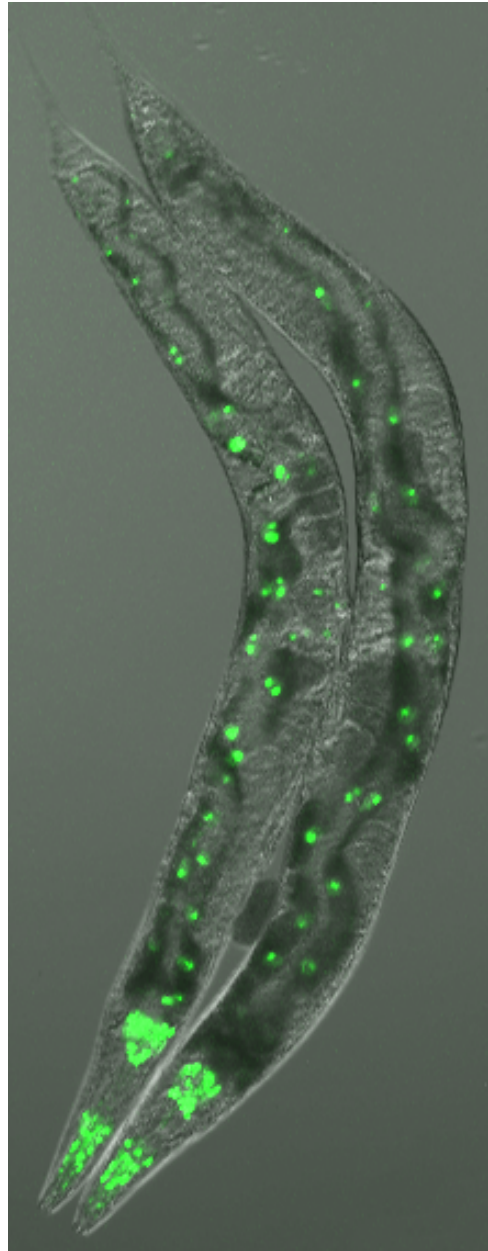
JF88( mtEx63 ) 400 \mu M zinc 24 hour exposure
