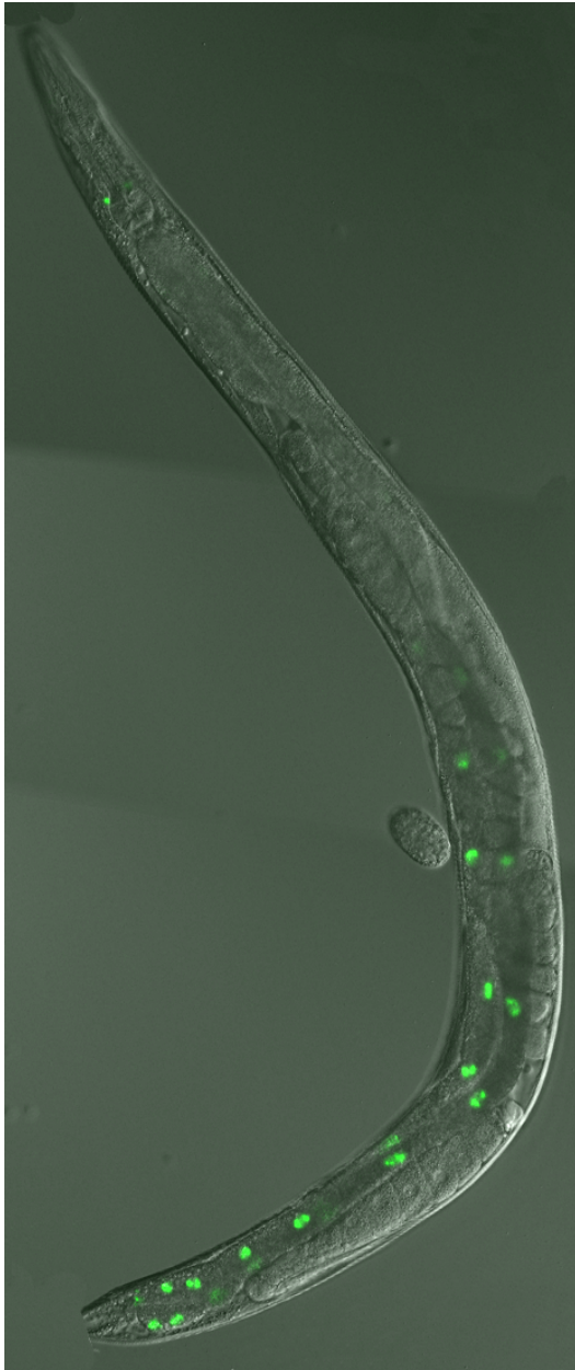
JF88( mtEx63 ) 2 \mu M silver 24 hour exposure
