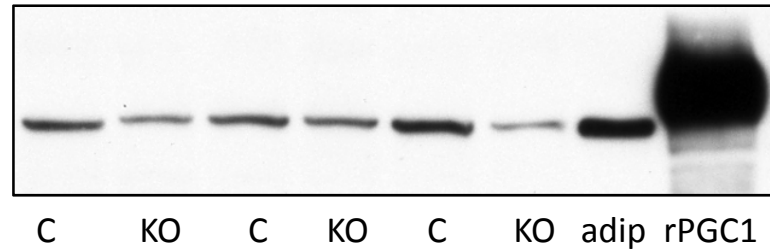
Supplemental Figure 1: PGC1 \alpha content as detected with the Calbiochem antibody (Cat#516557). C = control mouse gastrocnemius. KO = mLKB1-KO gastrocnemius. Adip = brown adipose tissue. rPGC1 = recombinant flag-tagged mouse PGC1 \alpha .
