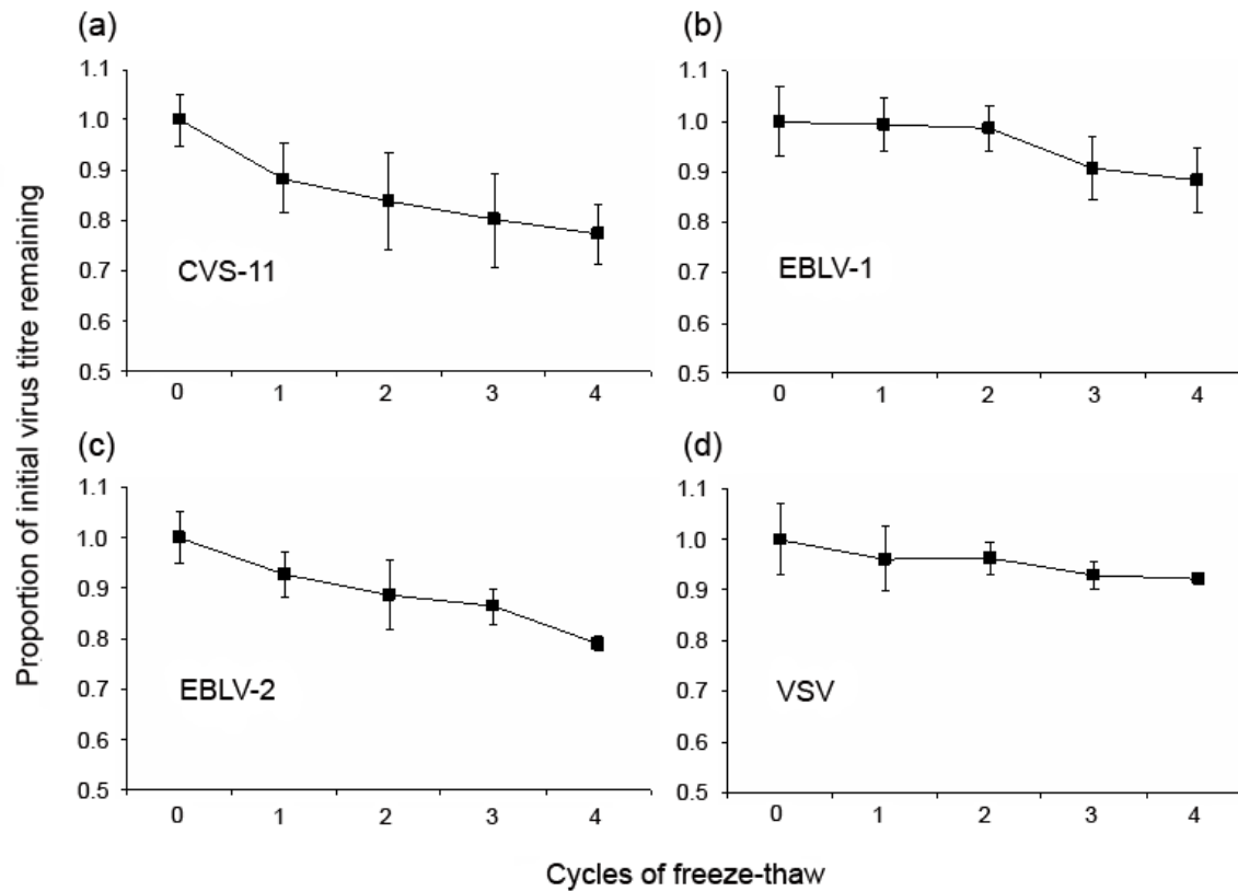
Fig. S1. Stability of lyssavirus pseudotypes. Lentiviral pseudotypes packaging the luciferase reporter and expressing (a) CVS-11, (b) EBLV-1, (c) EBLV-2 and (d) VSV G-proteins were subjected to four cycles of freeze–thaw. A 5 \mu l aliquot of each sample was then incubated with 1 \times 10^4 BHK cells for 48 h, after which the level of viral infection was determined; this is reported as the proportion of virus remaining compared to the sample that underwent no (0) freeze–thaw cycles. The mean \pm SD of four experiments is shown.
