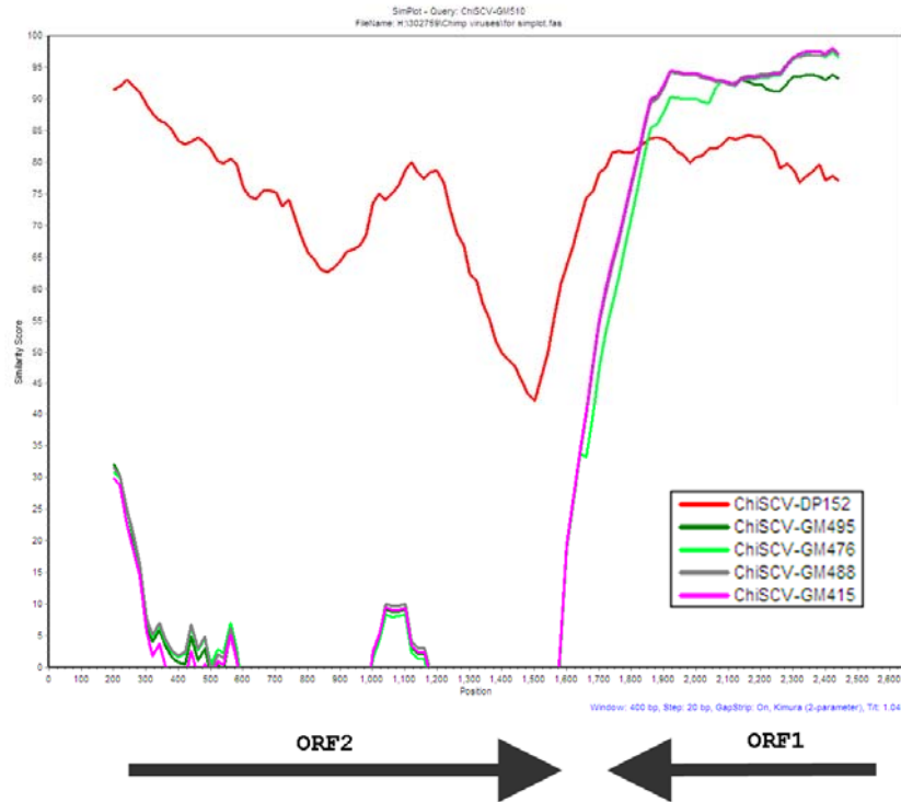
Supplementary Fig. S1. Recombination analyses. (a) Sliding window SimPlot of ChiSCV-GM510 against other ChiSCVs (except for the shorter ChiSCV-GT306 sequence). The nucleotide position is shown on the x -axis, the per cent nucleotide sequence similarity is shown on the y -axis. The positions of the major ORFs are indicated by arrows.
