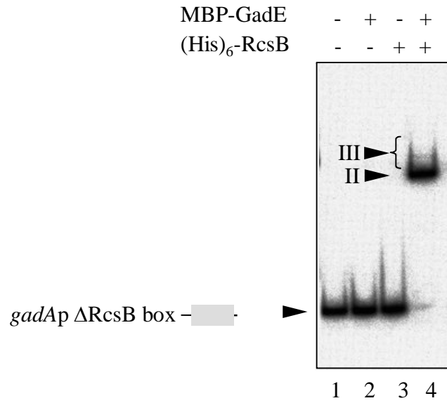
Figure S1 : EMSA of gadA promoter region template containing only the GAD box ( gadAp ΔRcsB box region from -101 to -22) in the presence of (His) 6 -RcsB (5 μM) and/or MBP-GadE (4 μM).
