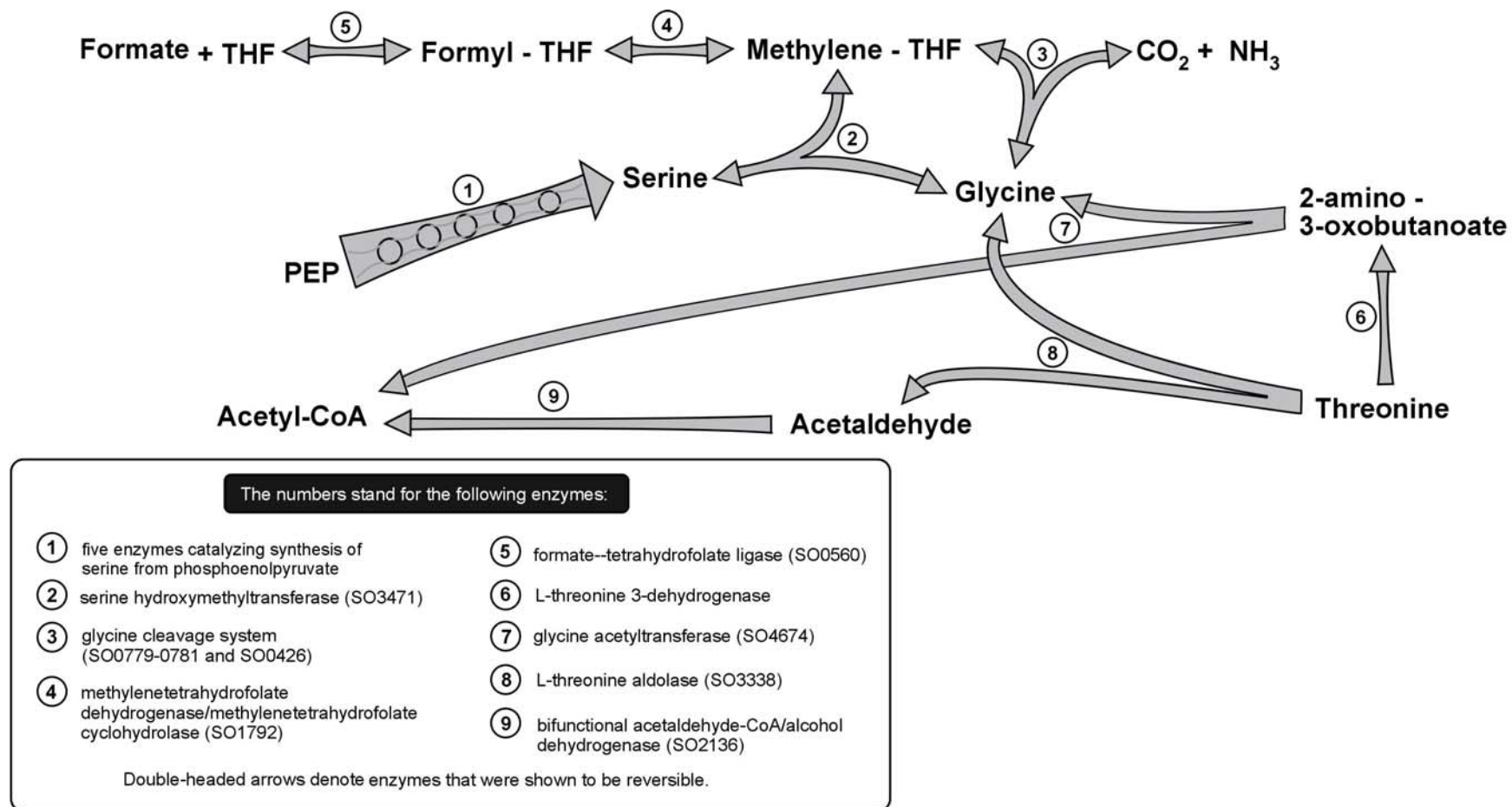
Figure S5. Metabolic network for interconversion of C1-compounds and biosynthesis/degradation of relevant amino acids in S. oneidensis MR-1. The network was constructed based on genome annotation.
