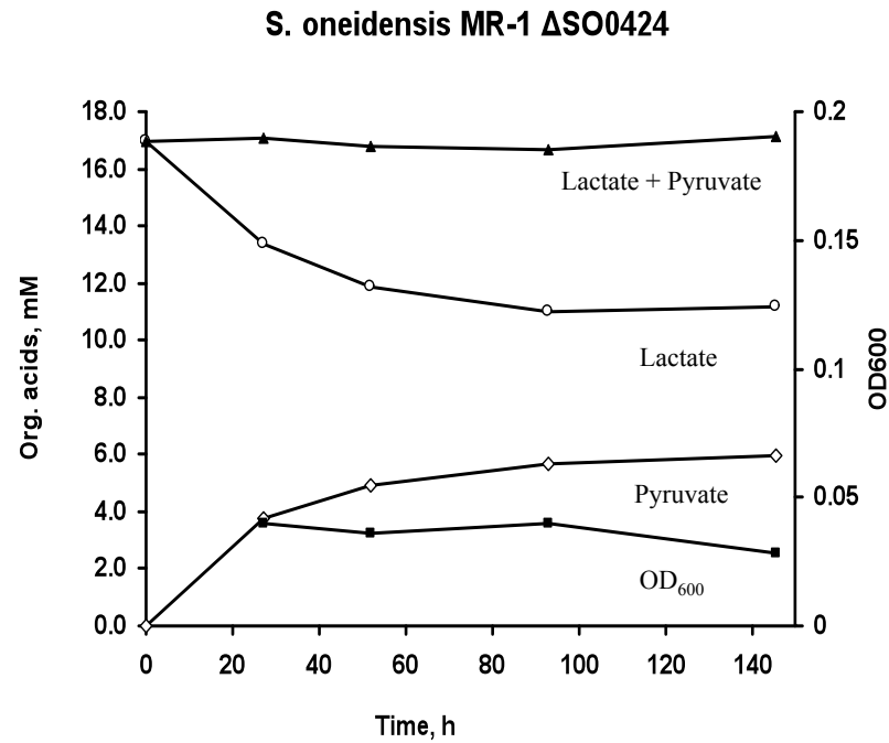
Figure S7. Aerobic growth of S. oneidensis \Delta SO0424 cells in M1 medium supplemented with 18 mM D,L-lactate. 70 ml serum bottles containing 15 ml of medium were used. Periodically 0.7-0.8 ml samples were withdrawn to measure OD 600 and organic acids in 0.22 \mu m filtrates of culture.
