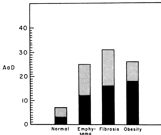
FIG. 1. MEAN ALVEOLAR-ARTERIAL OXYGEN TENSION DIFFERENCE (AaD) IN NORMAL SUBJECTS AND IN PATIENTS WITH EMPHYSEMA, DIFFUSE PULMONARY FIBROSIS, OR OBESITY. Height of bars represents total AaD during air breathing, and blackened segment, portion due to venous admixture after oxygen was breathed.
