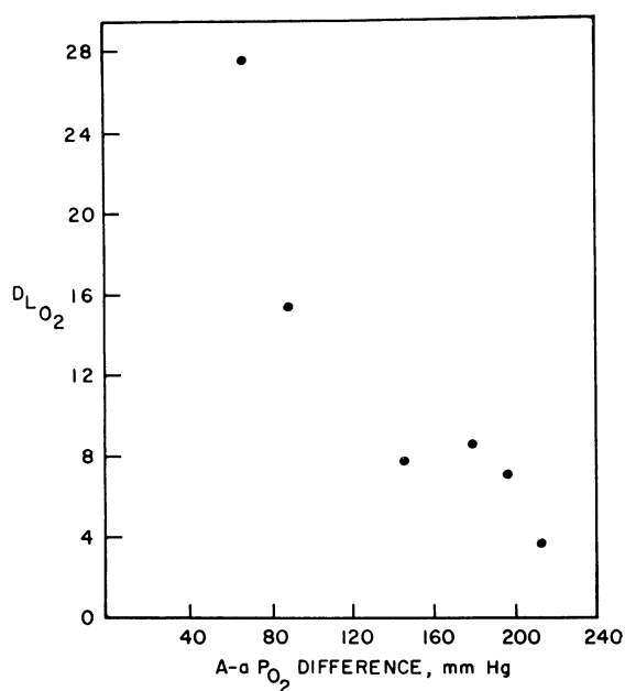
FIG. 2. PLOT OF PULMONARY DIFFUSING CAPACITY FOR OXYGEN ( D_{L_{O_2}} ) AGAINST ALVEOLAR-ARTERIAL OXYGEN PARTIAL PRESSURE DIFFERENCE, MEASURED DURING OXYGEN BREATHING, IN SIX PATIENTS WITH DIFFUSE DISEASES OF THE ALVEOLAR-CAPILLARY BED. Values shown for D_{L_{O_2}} represent direct measurements in four patients (K.B., S.J., R.G., and G.J.), and calculations in two (C.K. and V.A.S.) of 1.23 \times measured diffusing capacity for carbon monoxide (data from Table III).
