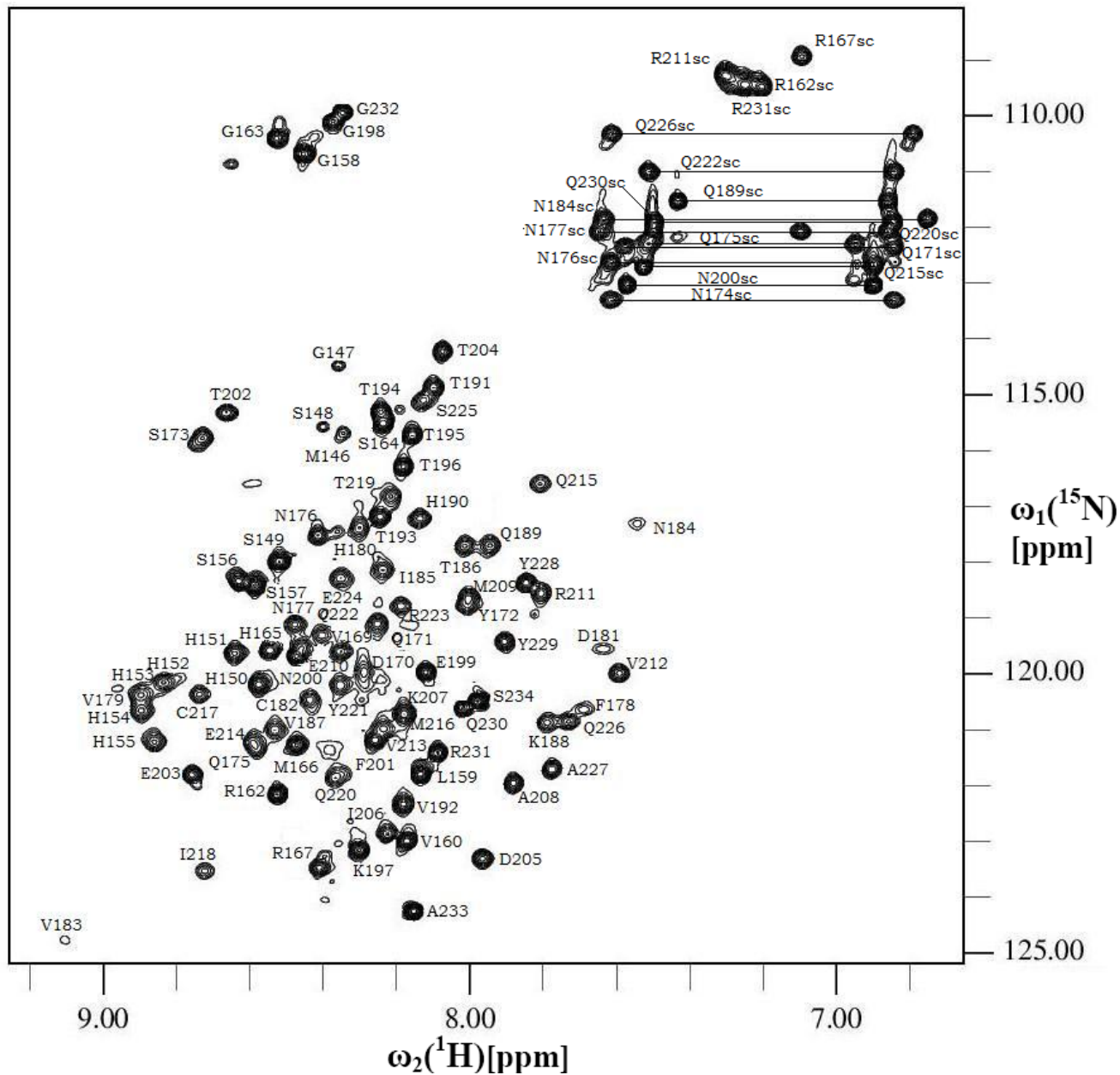
FIGURE S1 – HSQC spectrum of ^{15}\text{N} labelled ovH2H3_I208A recorded at 25°C and 600 MHz.
