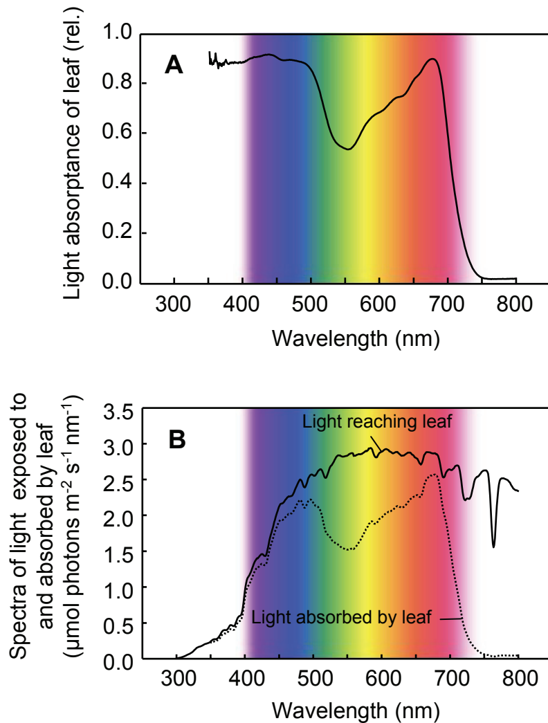
Supplemental Figure 2. A, The spectrum of light absorbance of a leaf. B, The spectra of light reaching the leaf and absorbed by the leaf during the photodamage experiment to the leaf in Figure 2. Spectrum of light absorbed by the leaf was calculated from multiplying the light absorbance at each wavelength by light reaching the leaf.
