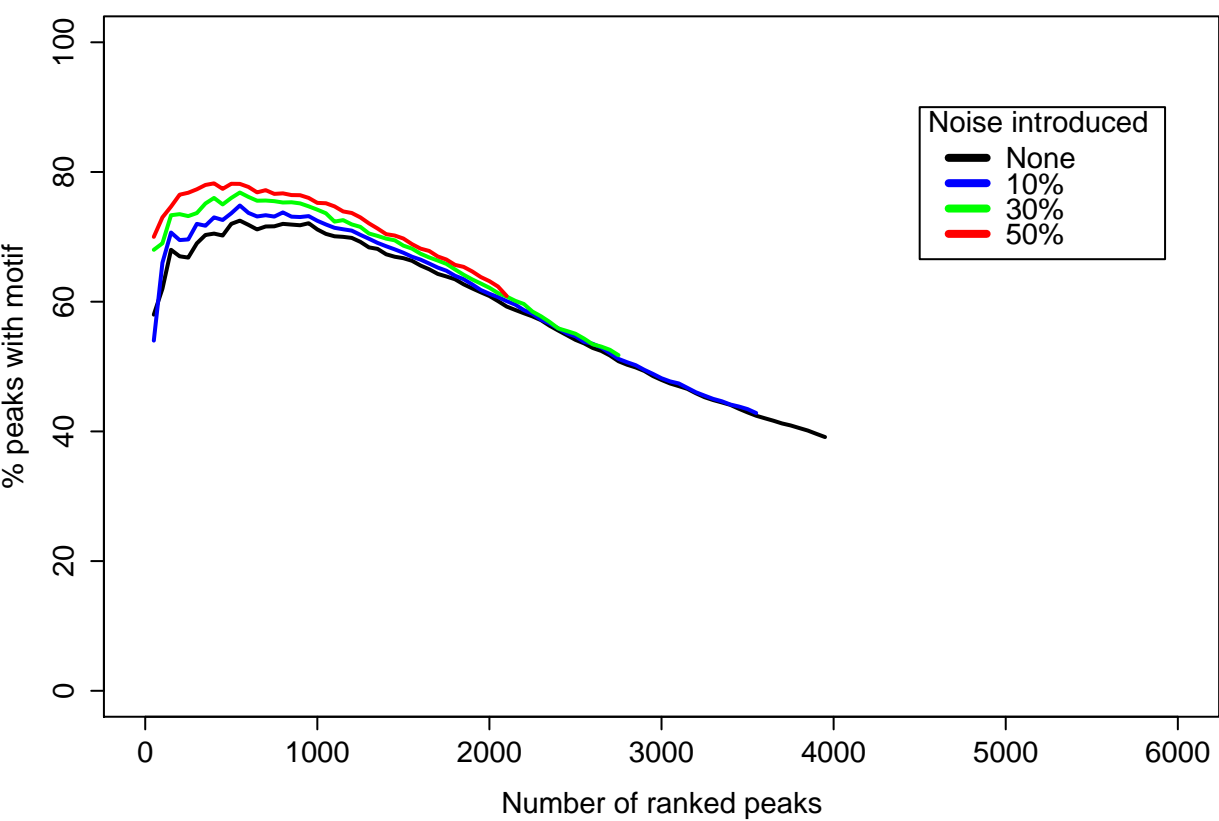
PeakSeq
