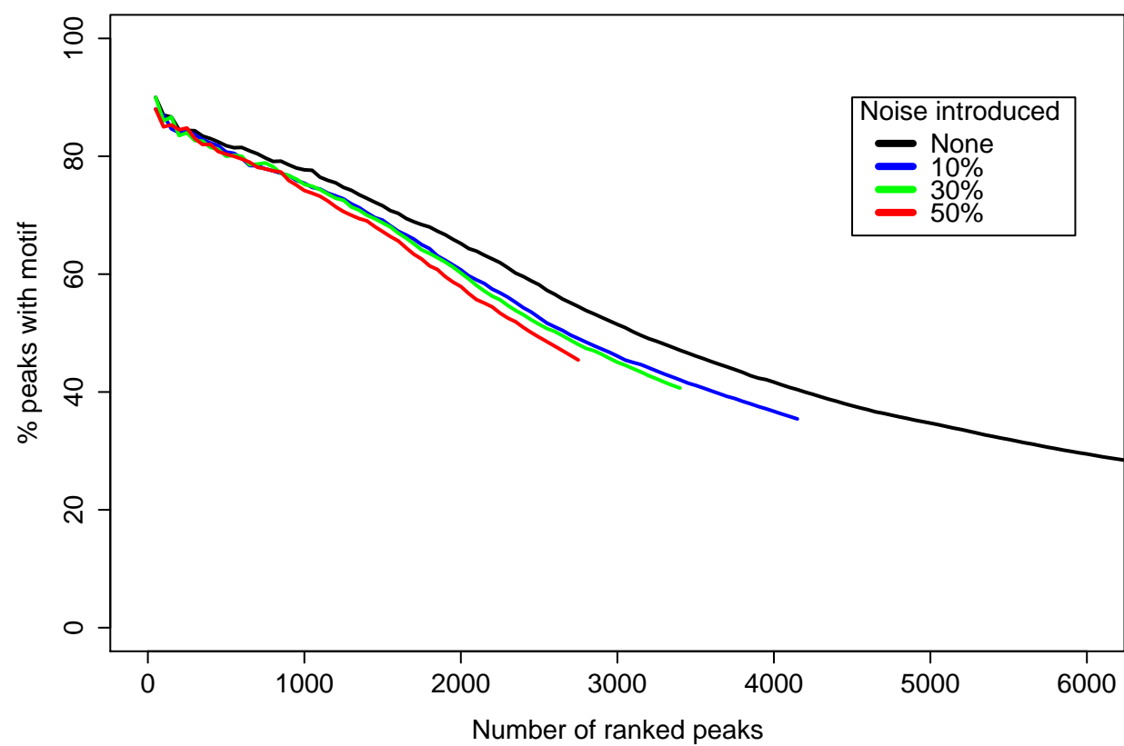
QuEST
