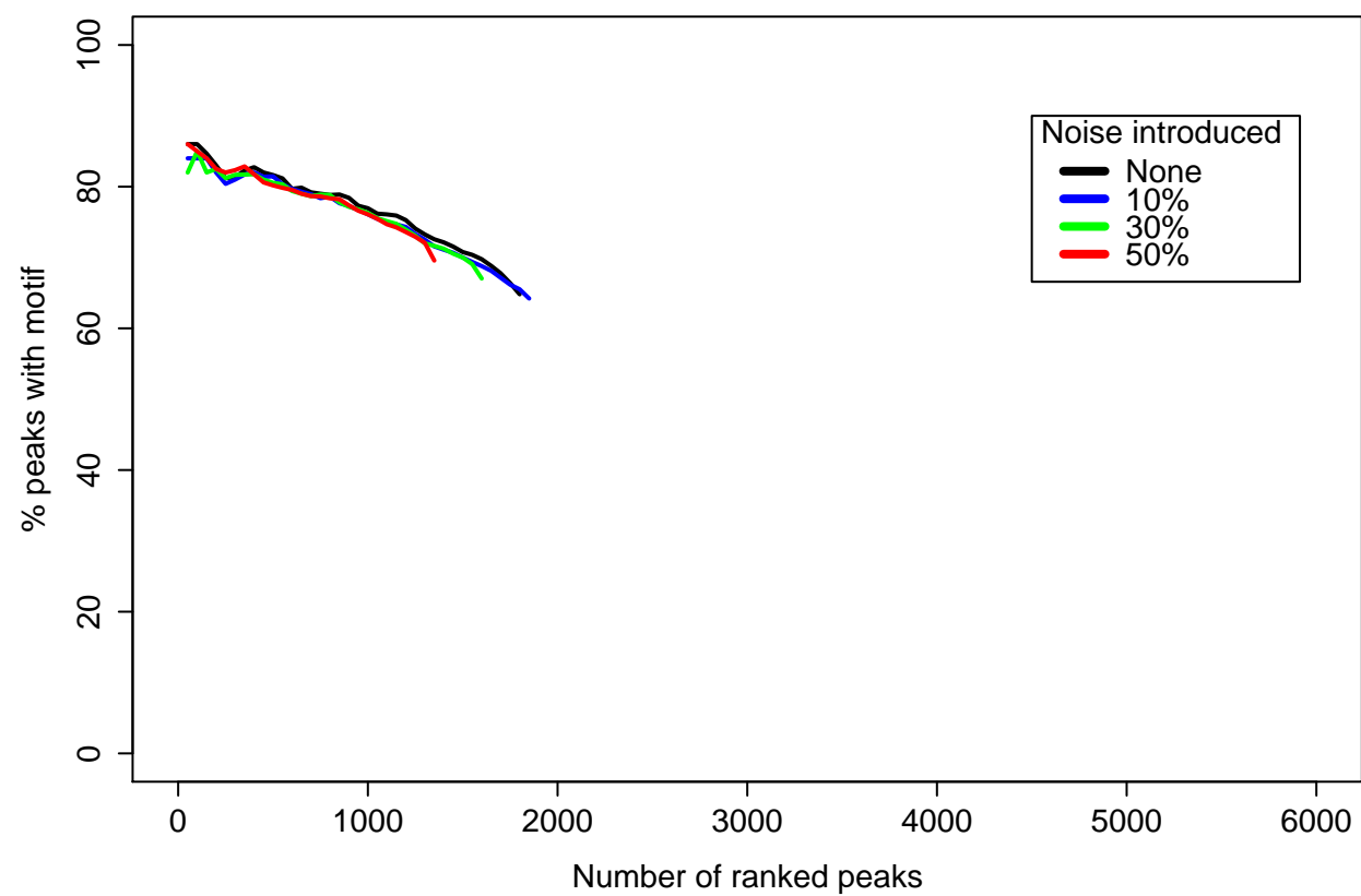
Sole-Search
