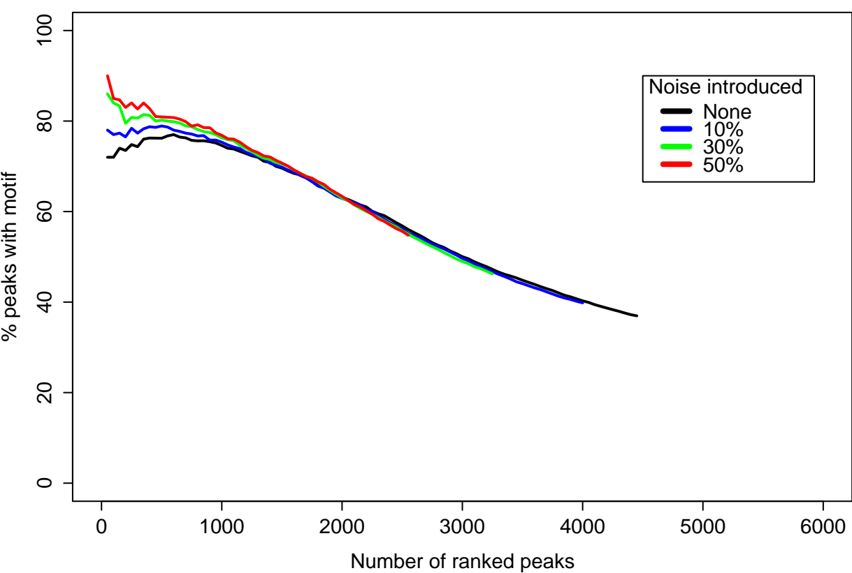
HPeak
