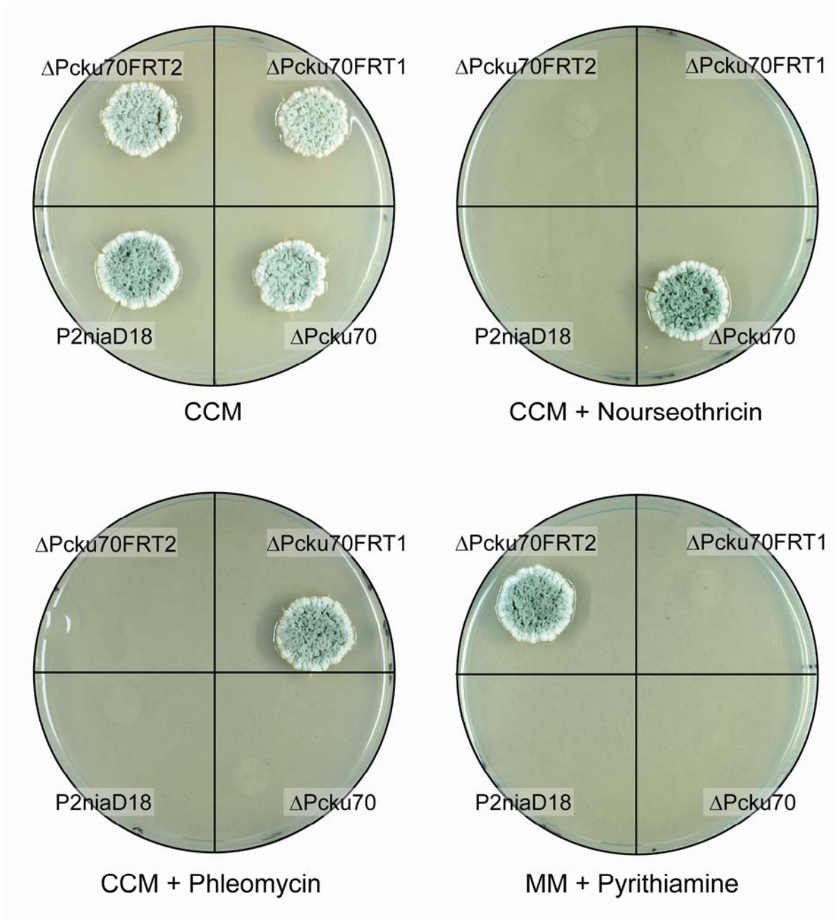
Supplementary Fig. 3: Growth tests on selective media of recombinant strains carrying the optimized FLP/FRT recombination system as a first step to constructing a marker-free \Delta Pcku70 strain. All strains are given in Table 1.
