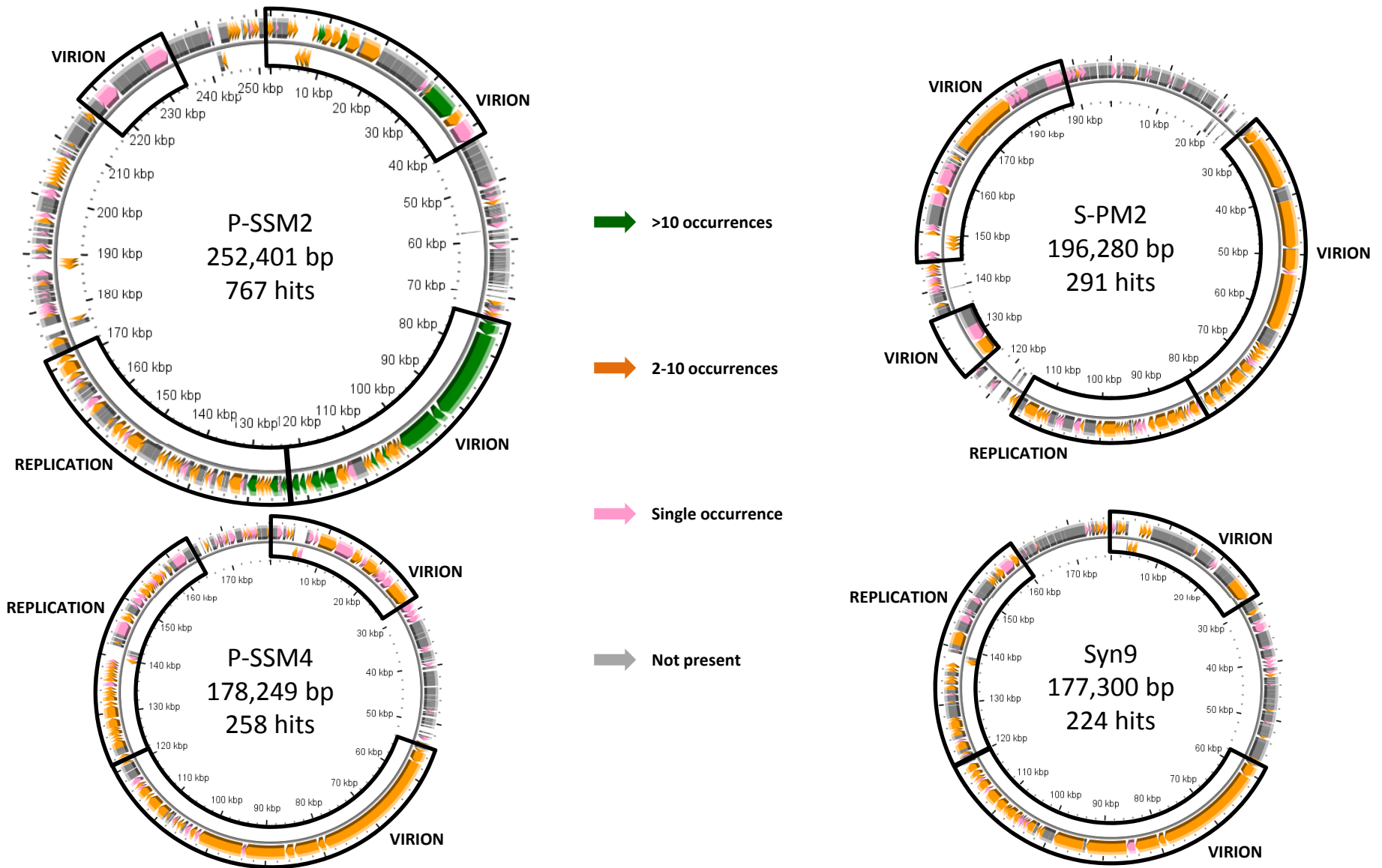
Figure S1. GOS scaffold coverage of the Cyano-T4 genomes. The genomes of the four Cyano-T4 phages with significant hits on the scaffolds are presented, along with the coverage of individual genes/ORFs (different colors) and the conserved virion and replication modules (curved black boxes) indicated. The genomes are drawn to scale.
