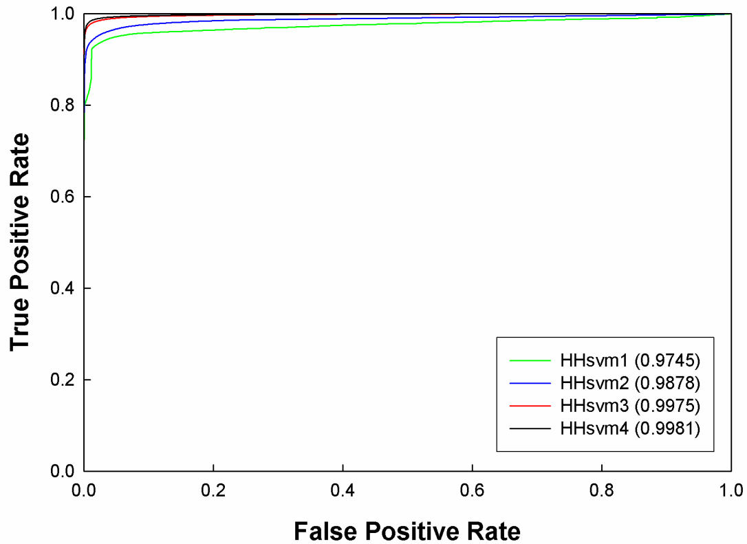
Supplementary Figure 1. Receiver operating characteristic (ROC) curves (Fawcett, 2006) of SVM classifiers described in the main text. The area under curve (AUC) for each classifier is shown in the box. The perfect classifier has AUC of 1.
