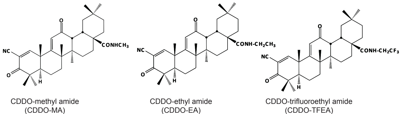
(A) Chemical structures of CDDO analogues
