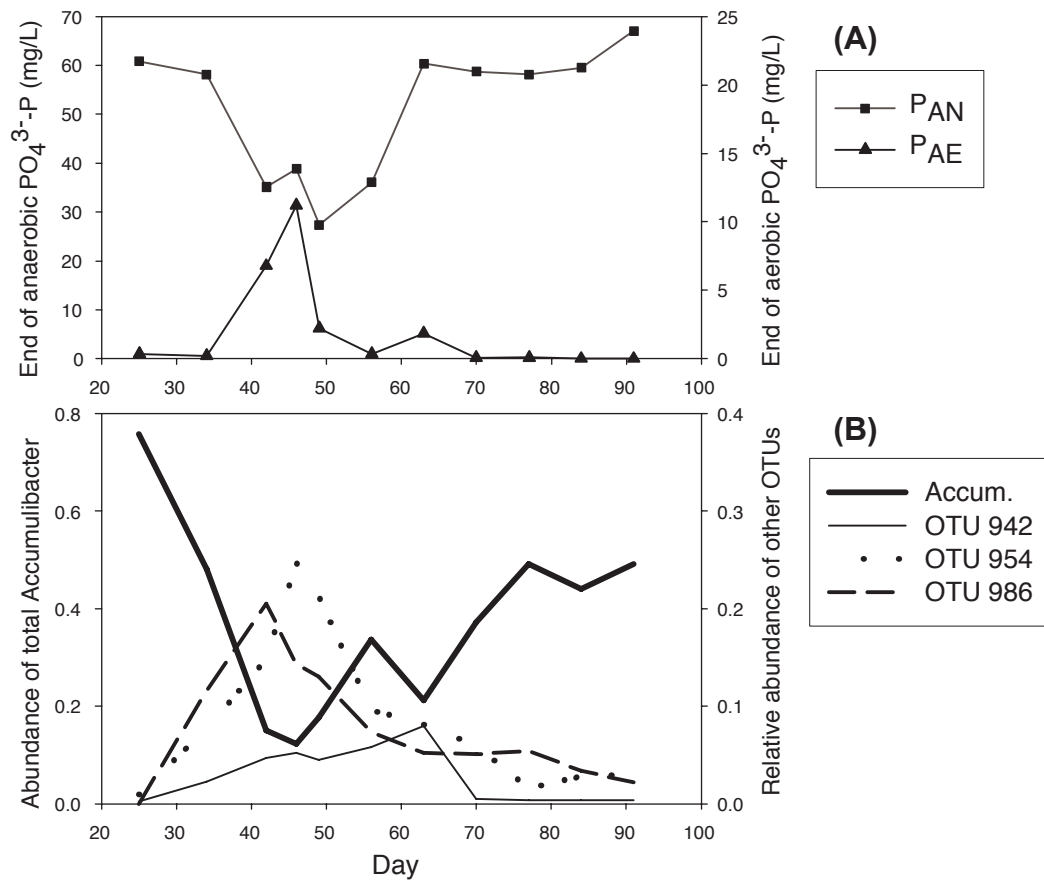
FIG. S1. Performance of R2 (panel A) and relative abundance of total Accumulibacter and OTUs correlated to the poor performance (panel B). Relative abundances were measured using semiquantitative ARISA.
