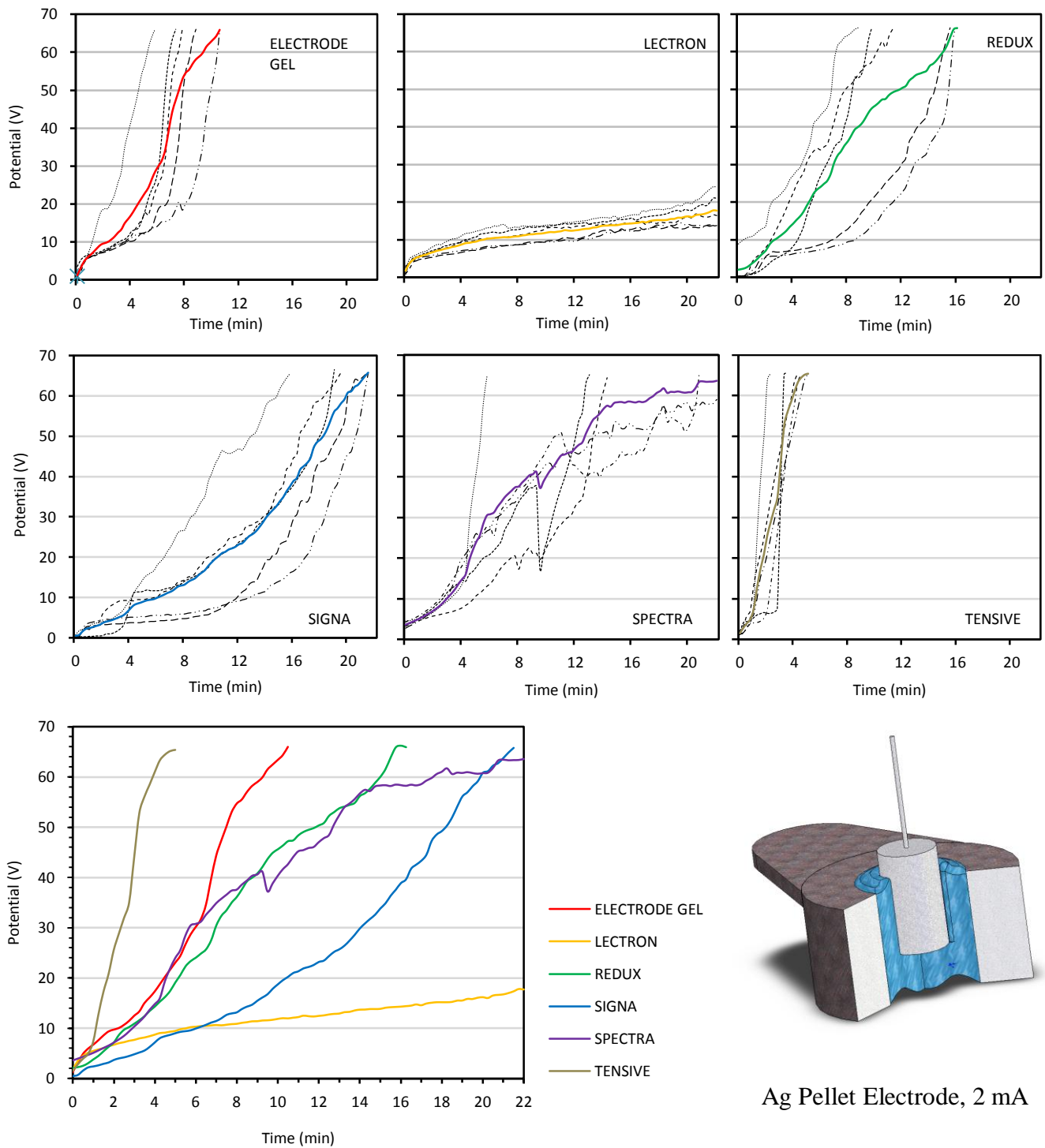
Supplementary Figure 1.A - Current induced polarization of conductive Ag Pellet electrode, shown as apparent voltage across anode against time. Voltage measured across pure Ag pellet anode is shown against time. 2mA DC current with commercially available gels was passed and change in voltage with time was measured. Black dotted curves shows five repeats while colored line shows average. The lower panel compares average voltage plots of all gels.
