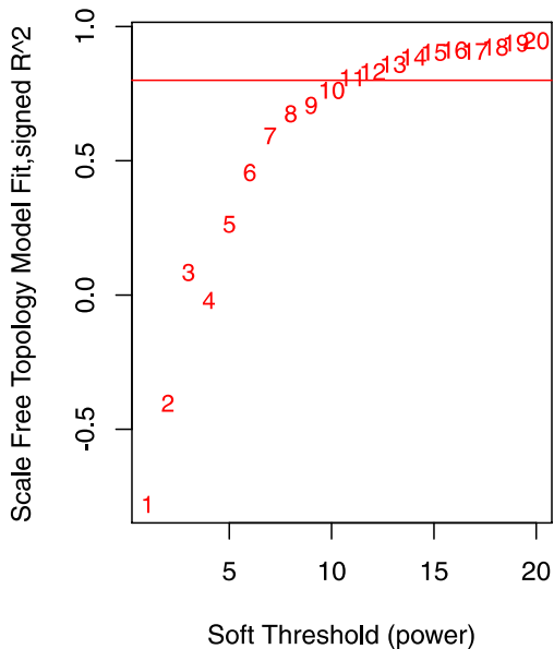
Scale independence
