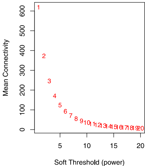
Mean connectivity
