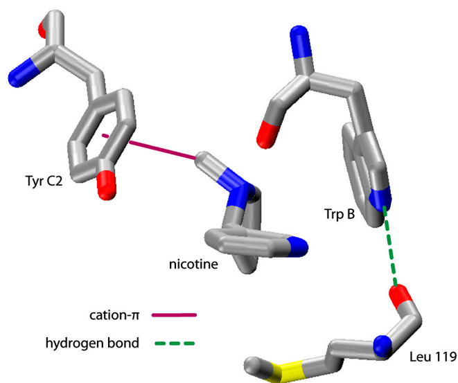
Fig. S1. Additional interactions seen in the crystal structure of nicotine bound to acetylcholine binding protein (PDB ID code 1UW6). Residue numbering is for the \alpha 4\beta 2 receptor.
