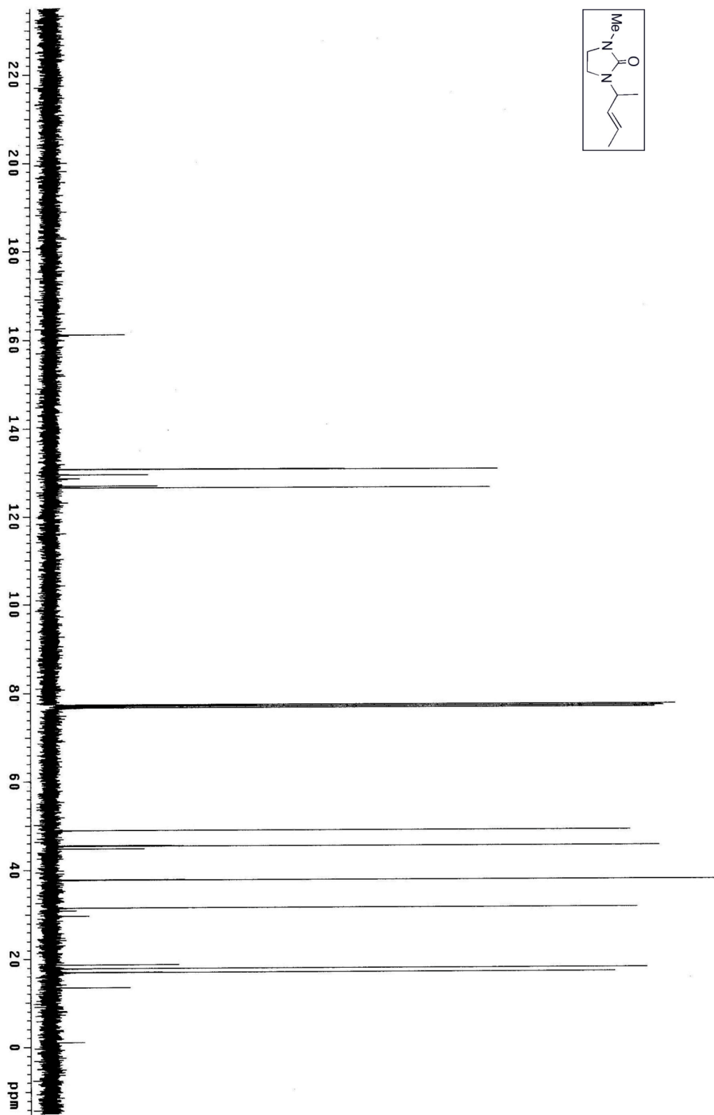
Figure S36. ^{13}\text{C}\{^1\text{H}\} NMR spectrum of 1-methyl-3-(pent-3-en-2-yl)imidazolidin-2-one (11).
