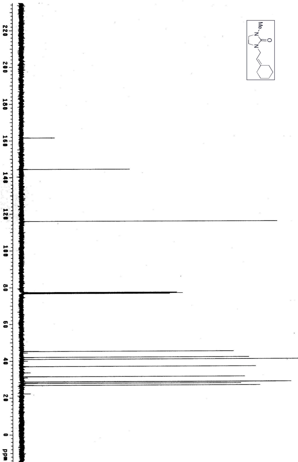
Figure S30. ^{13}\text{C}\{^1\text{H}\} NMR spectrum of 1-(2-cyclohexylideneethyl)-3-methylimidazolidin-2-one (7).
