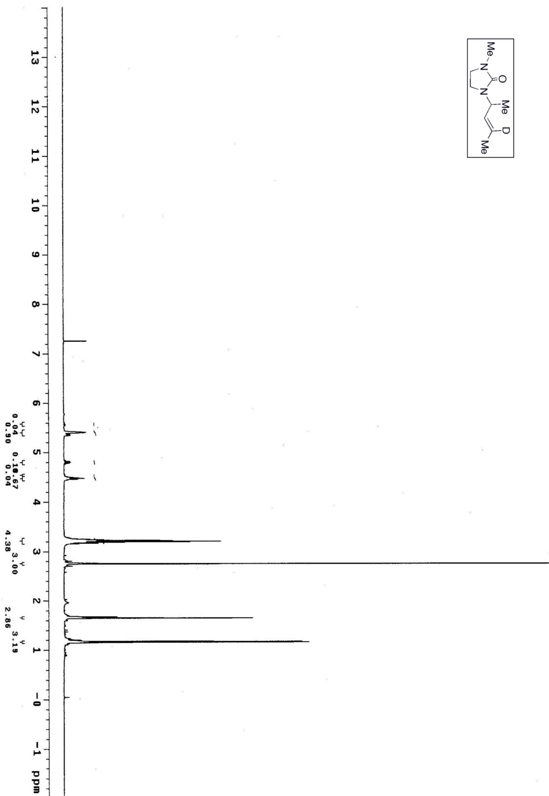
Figure S37. ^1\text{H} NMR spectrum of 1-(1-methyl-3-deuterio-2-butenyl)-3-methylimidazolidin-2-one ( 11- \gamma - d_1 ).
