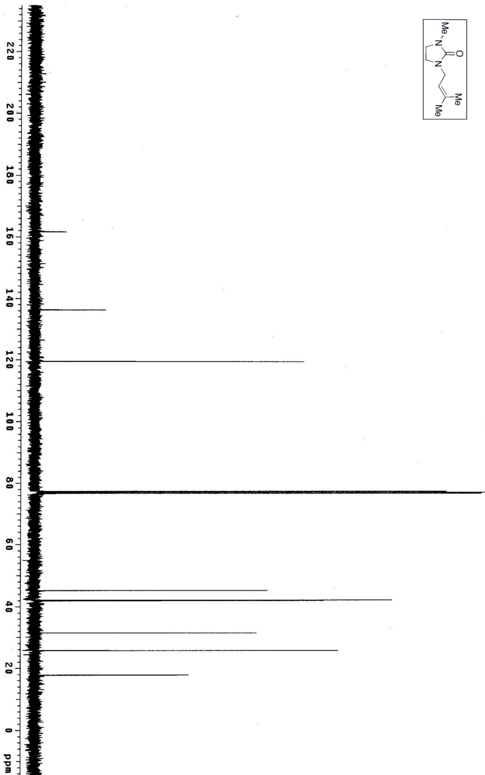
Figure S26. ^{13}\text{C}\{^1\text{H}\} NMR spectrum of 1-methyl-3-(3-methylbut-2-enyl)imidazolidin-2-one (6a).
