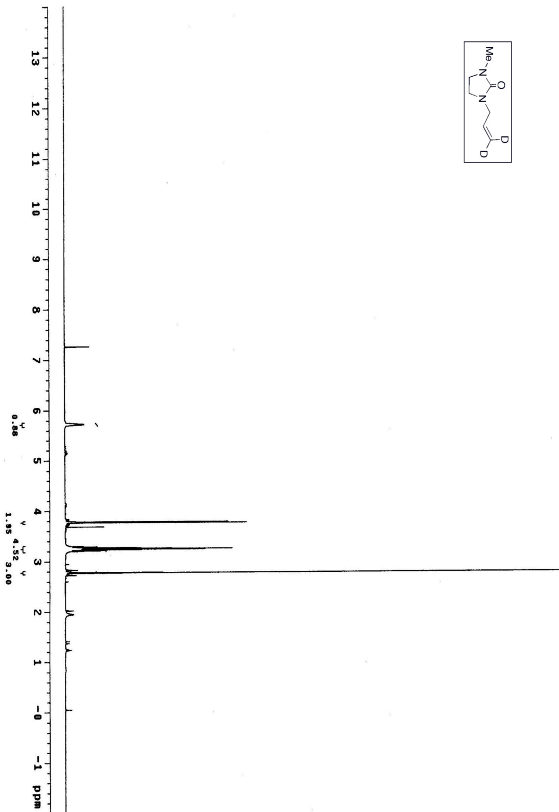
Figure S17. ^1\text{H} NMR spectrum of 1-(3,3-dideuterio-2-propenyl)-3-methyl-imidazolidin-2-one ( 3- \gamma,\gamma - d_2 ).
