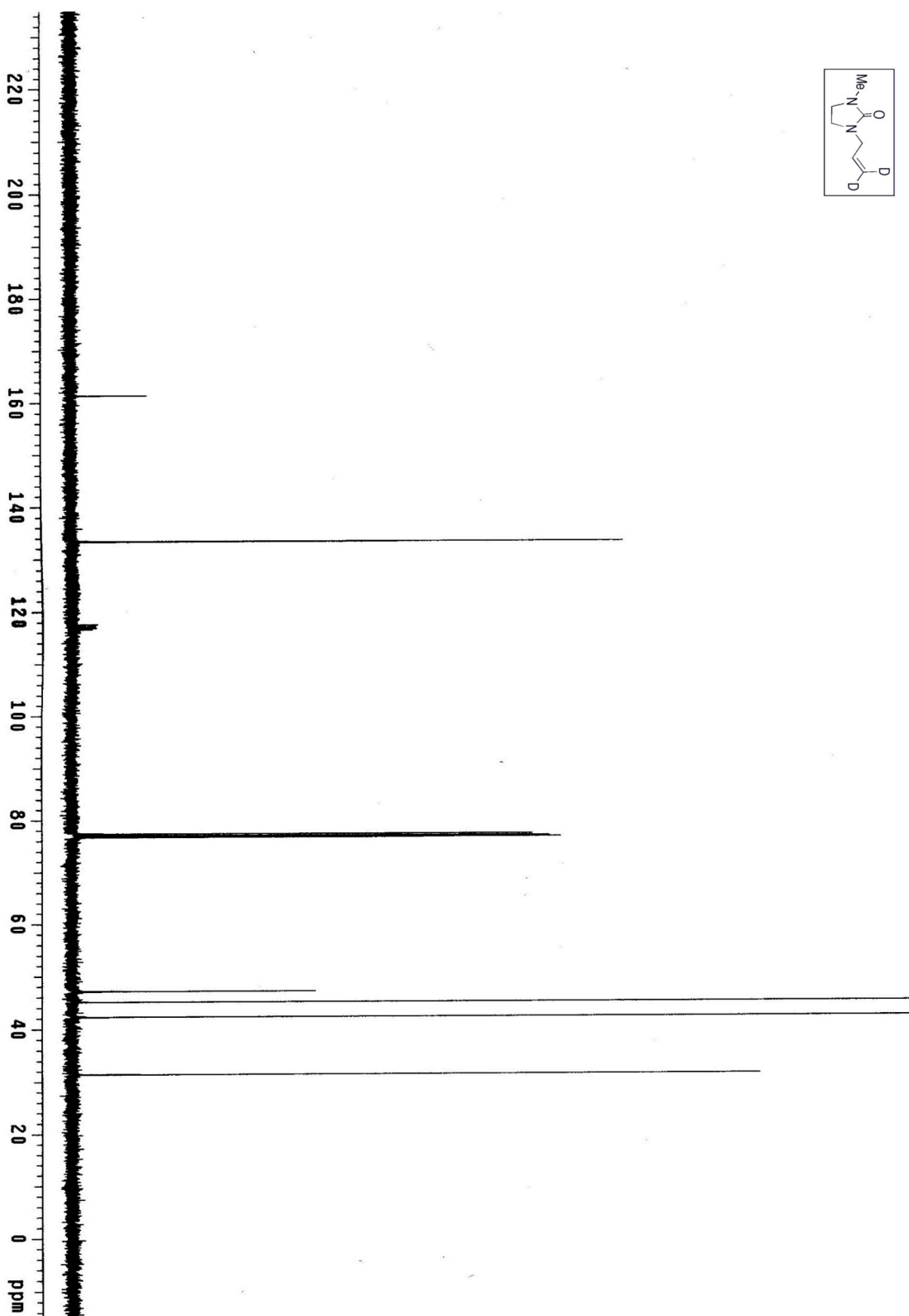
Figure S18. ^{13}\text{C}\{^1\text{H}\} NMR spectrum of 1-(3,3-dideuterio-2-propenyl)-3-methylimidazolidin-2-one ( 3- \gamma,\gamma - d_2 ).
