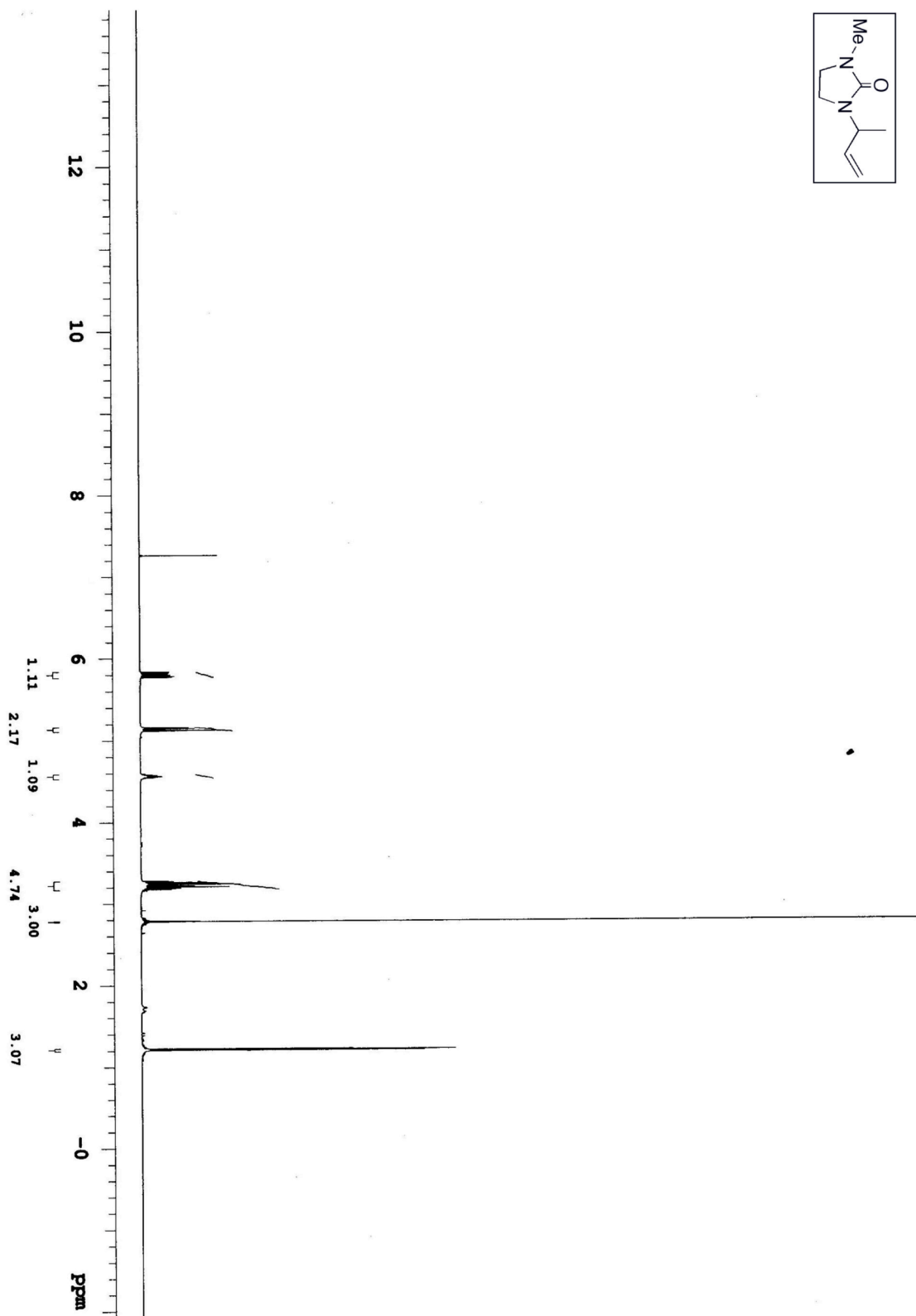
Figure S31. ^1\text{H} NMR spectrum of 1-(but-3-en-2-yl)-3-methylimidazolidin-2-one ( 8 ).
