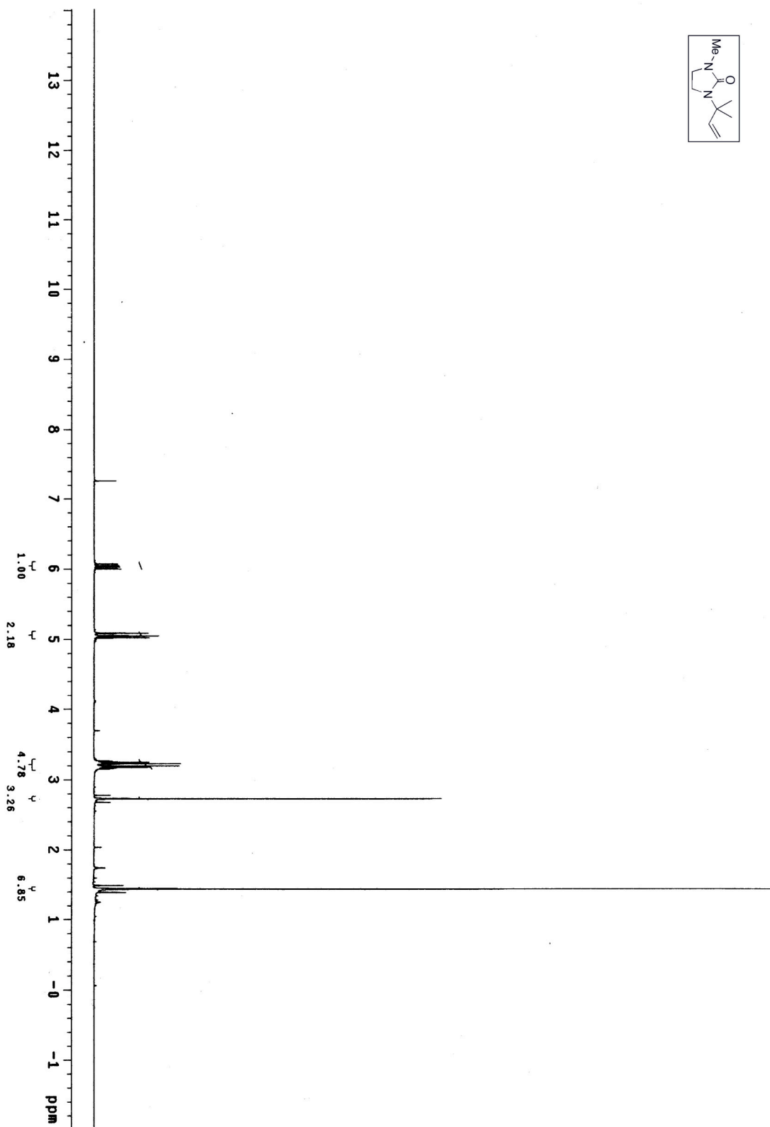
Figure S27. ^1\text{H} NMR spectrum of 1-methyl-3-(2-methylbut-3-en-2-yl)imidazolidin-2-one ( 6b ).
