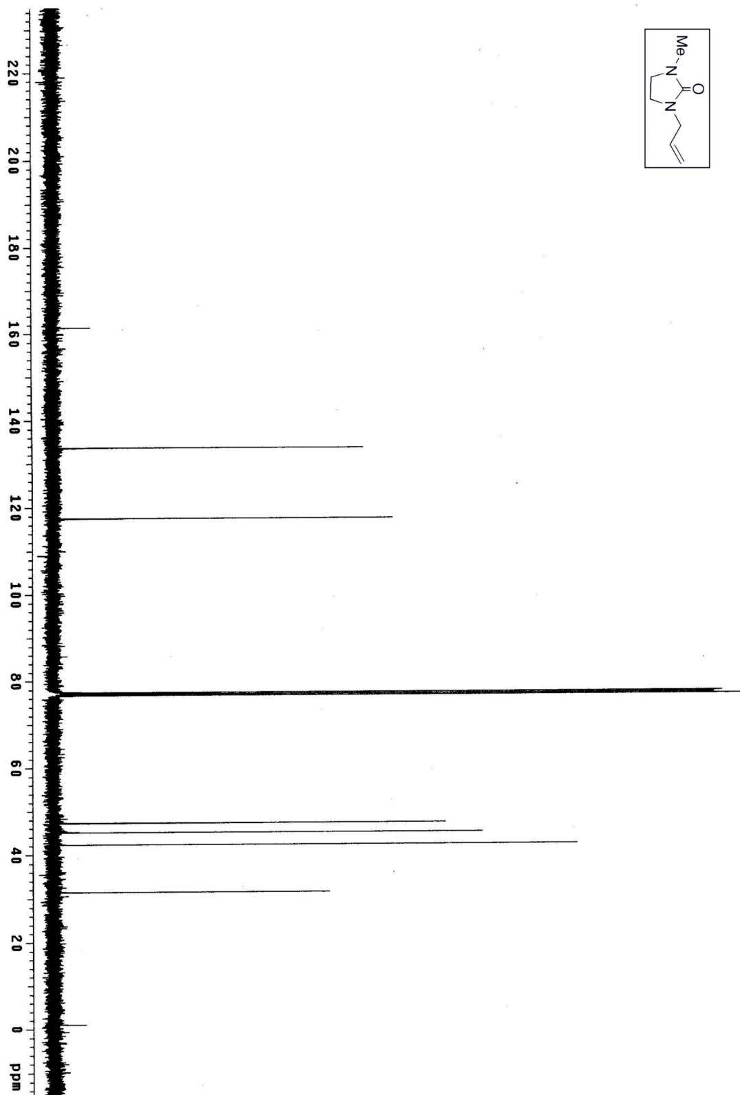
Figure S14. ^{13}\text{C}\{^1\text{H}\} NMR spectrum of 1-allyl-3-methylimidazolidin-2-one ( 3 ).
