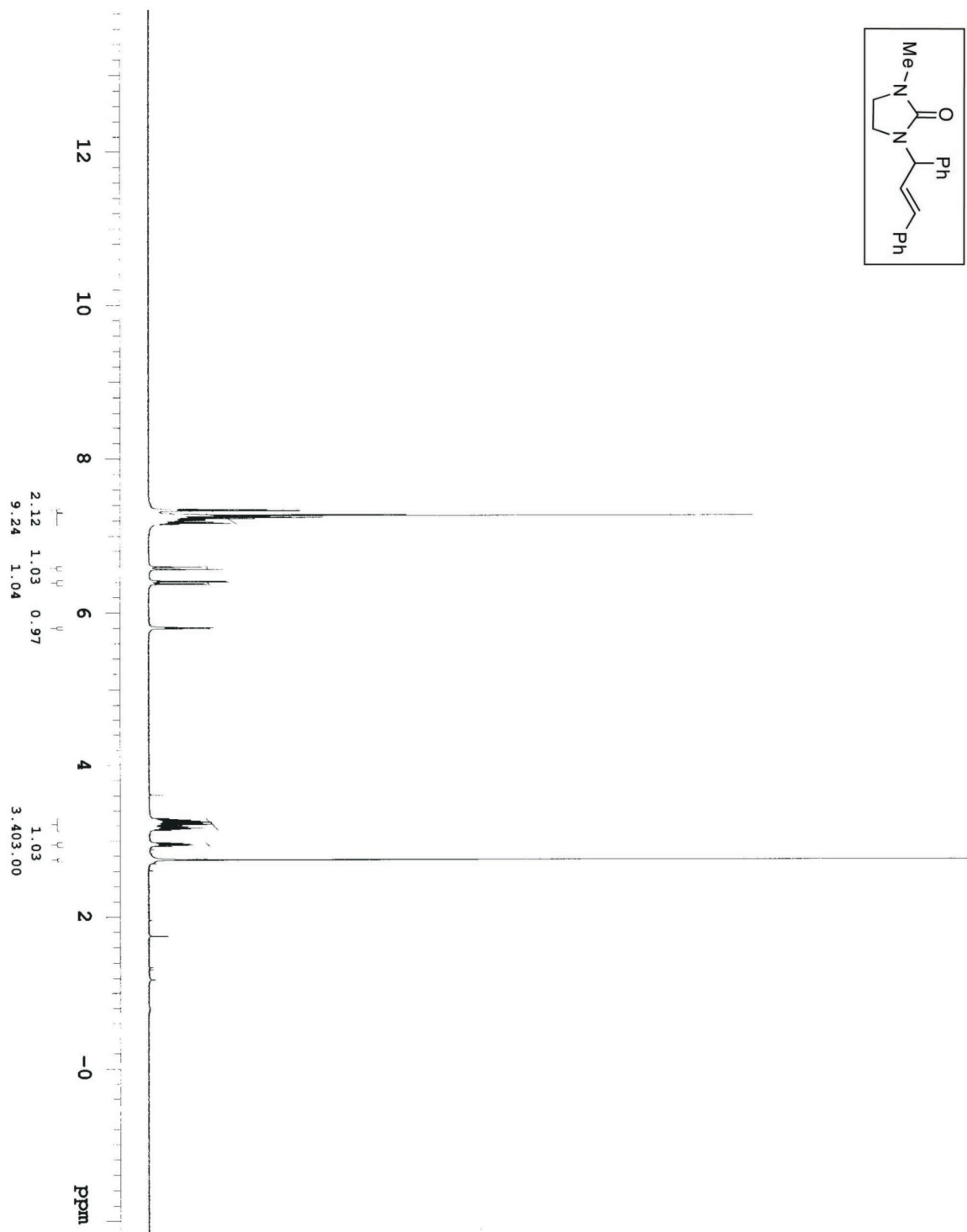
Figure S39. ^1\text{H} NMR spectrum of ( E )-1-(1,3-diphenylallyl)-3-methylimidazolidin-2-one ( 12 ).
