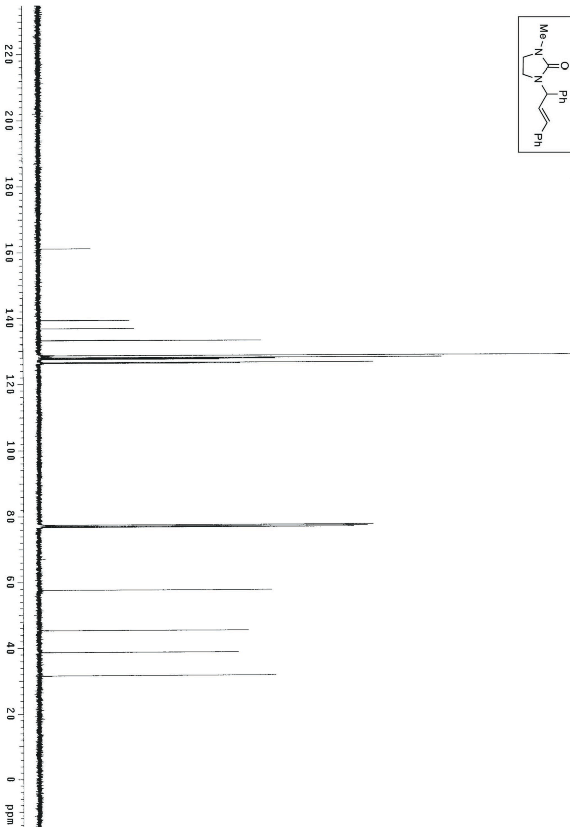
Figure S40. ^{13}\text{C}\{^1\text{H}\} NMR spectrum of ( E )-1-(1,3-diphenylallyl)-3-methylimidazolidin-2-one ( 12 ).
