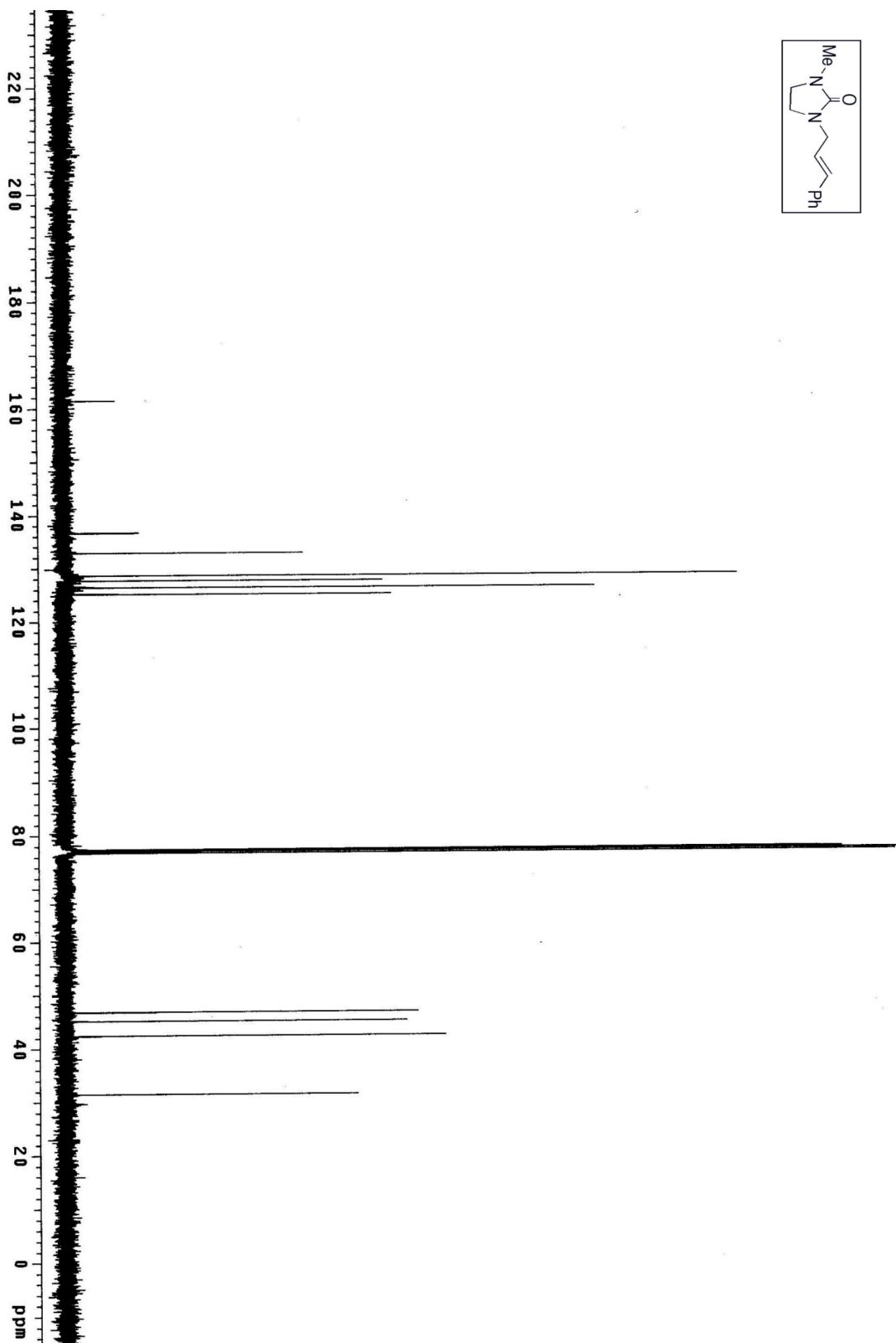
Figure S22. ^{13}\text{C}\{^1\text{H}\} NMR of ( E )-1-cinnamyl-3-methylimidazolidin-2-one [( E )-5].
