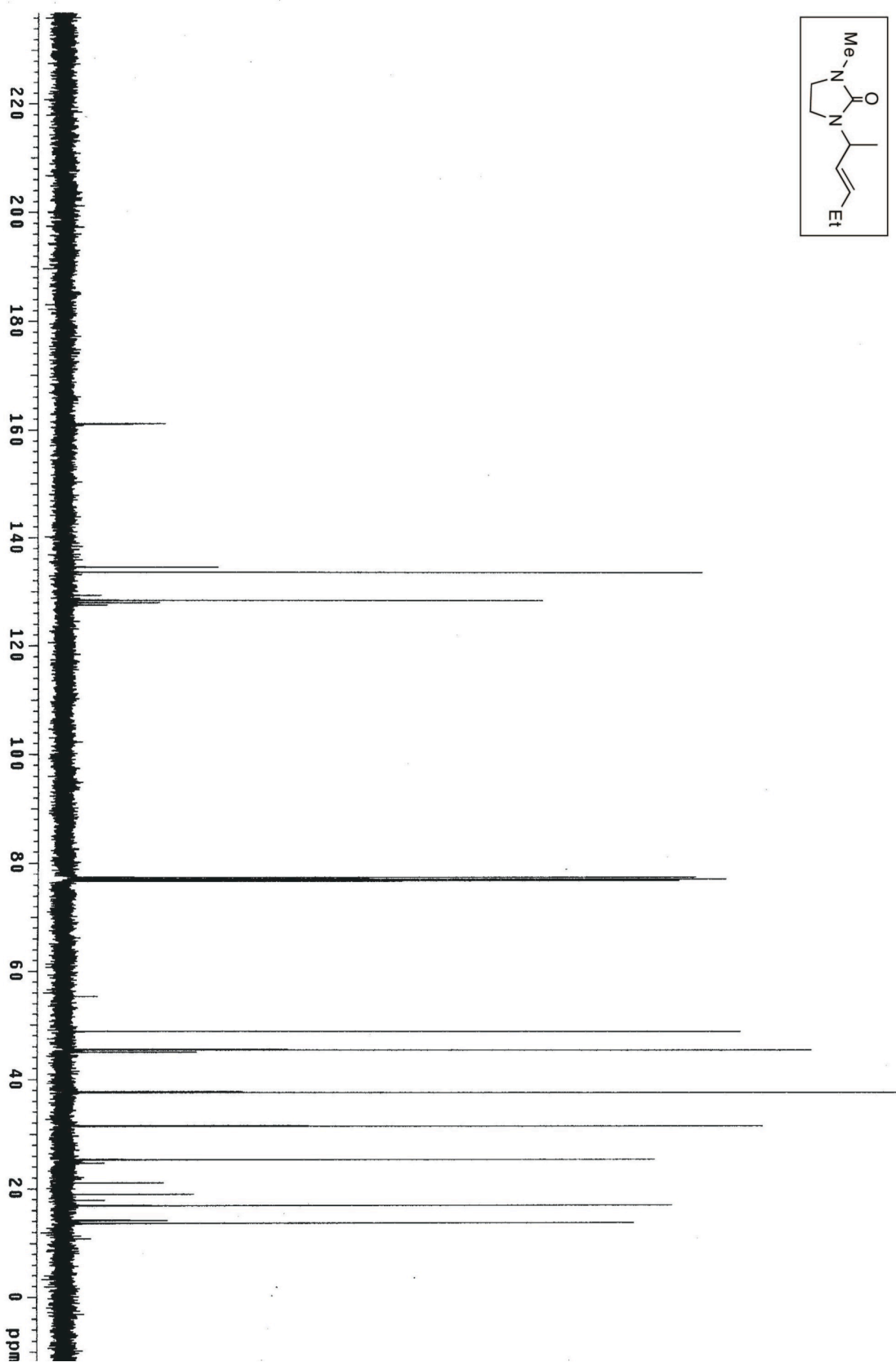
Figure S42. ^{13}\text{C}\{^1\text{H}\} NMR spectrum of 1-(hex-3-en-2-yl)-3-methylimidazolidin-2-one ( 14 ).
