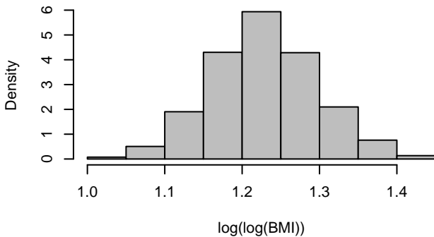
Histogram of Log(Log(BMI))
