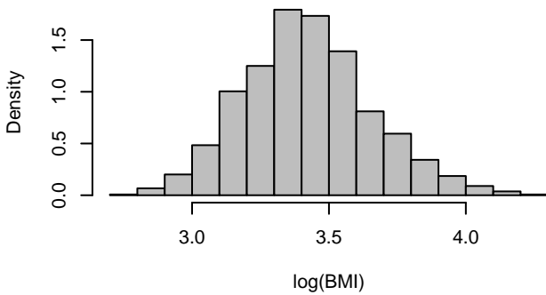
Histogram of Log(BMI)
