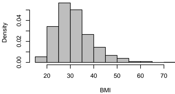
Histogram of BMI
