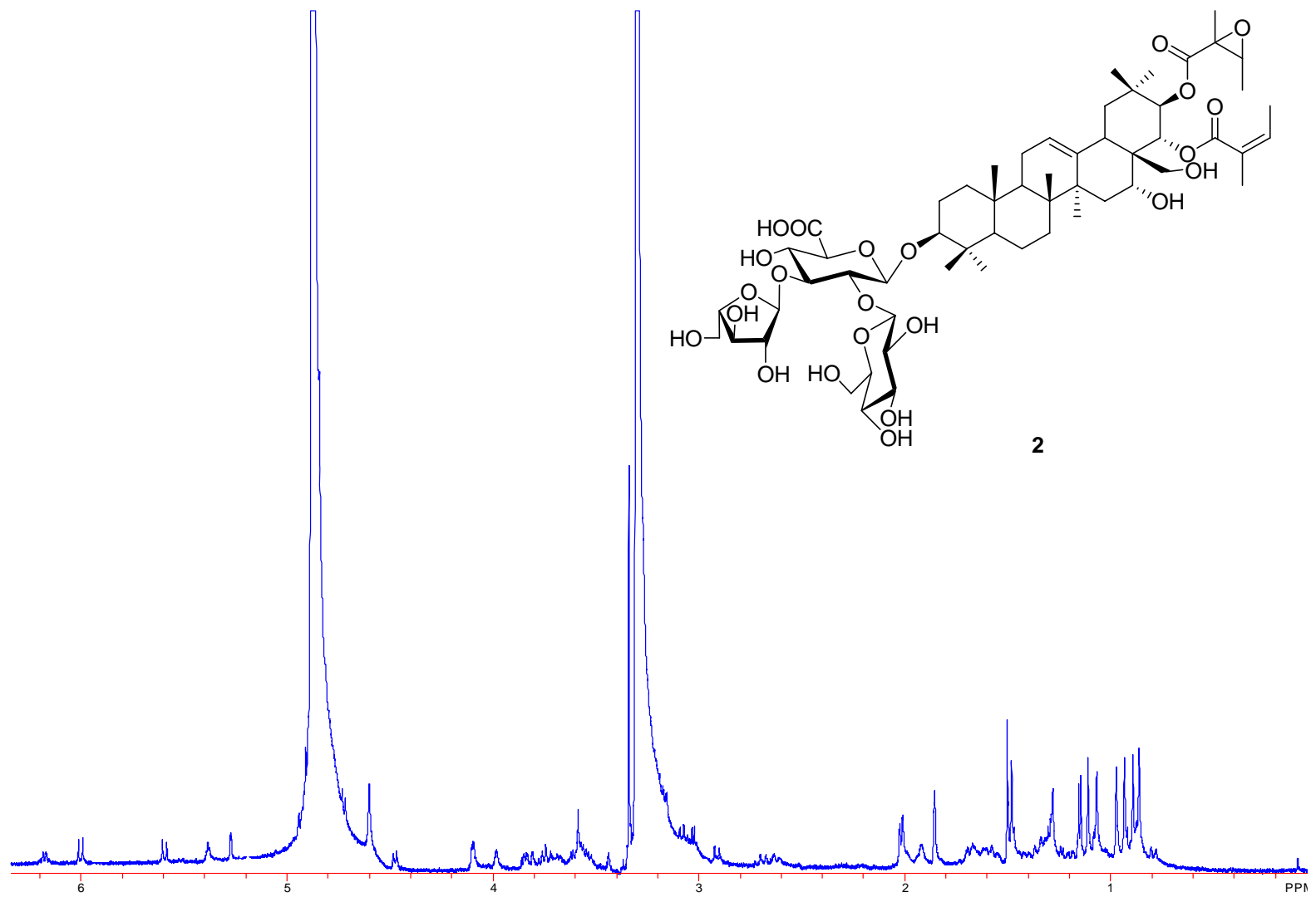
1 H NMR spectrum of compound 2
