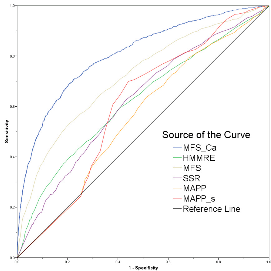
Calcium binding residue prediction Set 1 vs. 0 Receiver Operator Characteristic
