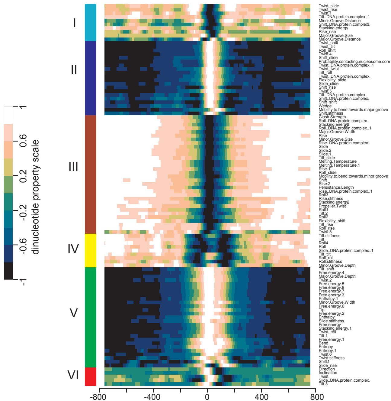
Figure S1: Heatmap of 103 DNA dinucleotide properties clustered into 6 groups using k-means clustering. Each average DNA dinucleotide profile was rescaled into the range -1 to 1, LOESS smoothed, and then clustered using k-means clustering (k=6) following 10000 iterations.
