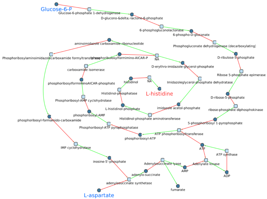
Figure S6. Sub-network corresponding to the production of histidine from glucose, and aspartate in B. cicadellinicola . Squares correspond to reactions and circles to metabolites. The colour of the edges differentiates the two sides of a reaction.
