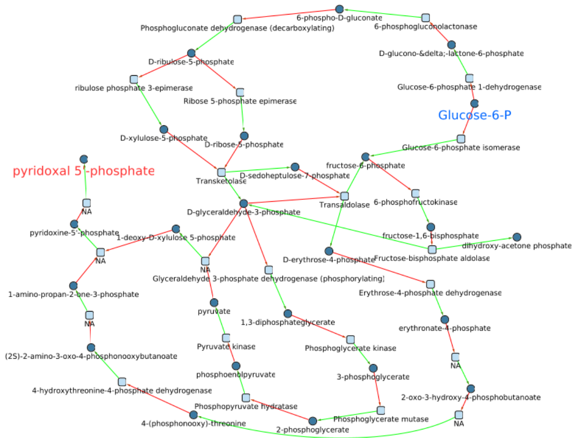
Figure S10. Sub-network corresponding to the production of pyridoxal-5'-phosphate from glucose in B. cicadellinicola . Squares correspond to reactions and circles to metabolites. The colour of the edges differentiates the two sides of a reaction.
