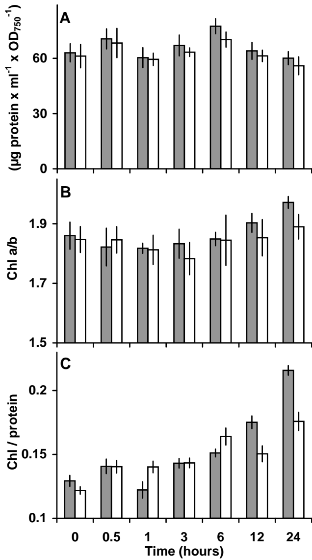
S. Figure 1. Time course comparison of CCM induced and control cultures. A, Protein concentrations standardized to OD 750 . B, Chlorophyll a/b ratios. C, Ratio of total chlorophyll per protein concentration. Control culture bubbled with high CO 2 (grey bars) and induced culture bubbled with low CO 2 (white bars). All bars represent the average ± SD of five individual replicates.
