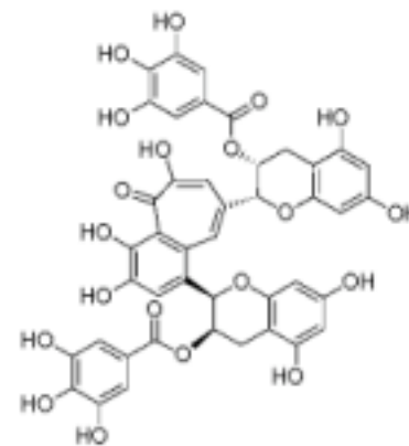
Theaflavin 3,3'-digallate (TFDG)
