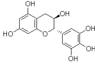
Gallocatechin (GC)
