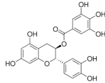
Catechin gallate (CG)
