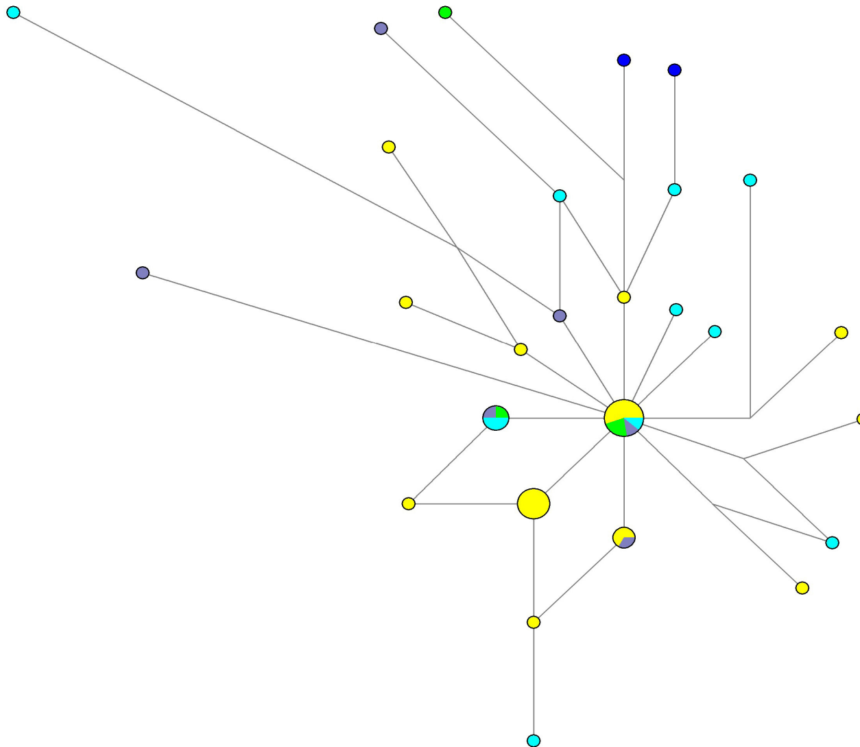
Figure S3. Network of the STR haplotypes belonging to haplogroup J-M241.
