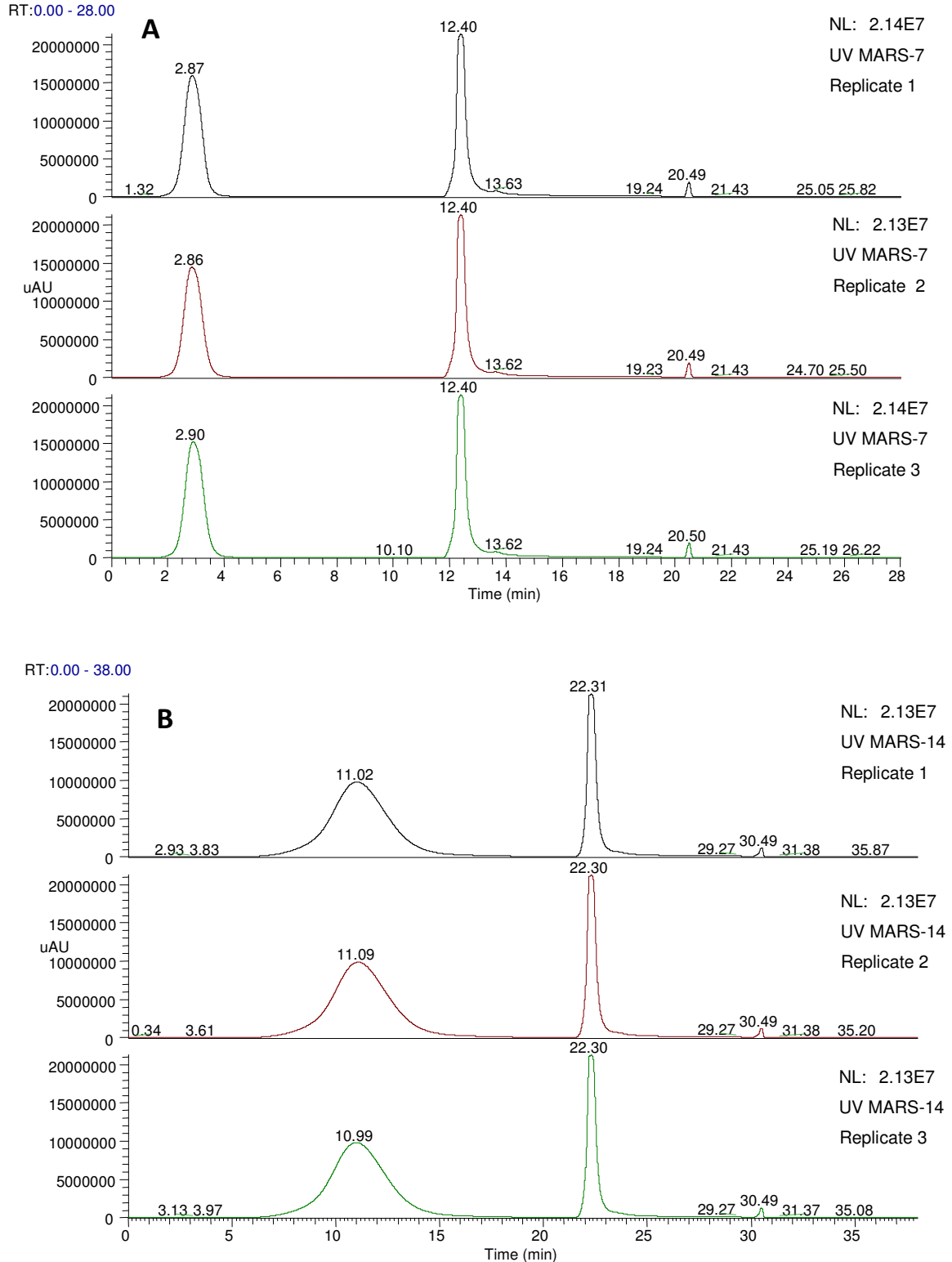
Figure S1. UV traces of three replicate runs of MARS-7 column (A) and MARS-14 column (B) separately
