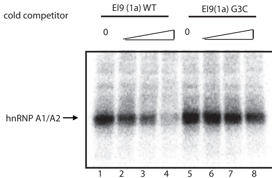
Supplementary Figure 3: hnRNP A1 binding to EI9(1a) is specifically decreased by G3C mutation. ^{32} P-UTP labeled EI9(1a) RNA (see diagram in Supplementary Figure 1) was incubated with HeLa NE, in the presence of increasing amount (0, 1.5, 3, 7.5 \mu M) of cold WT EI9(1a) RNA (lanes 1-4) or cold EI9(1a) G3C mutant RNA (lanes 5-8), followed by UV crosslinking..
