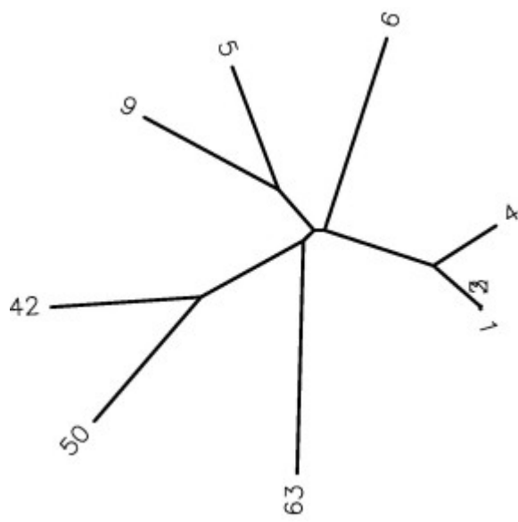
Group 2 : channel
