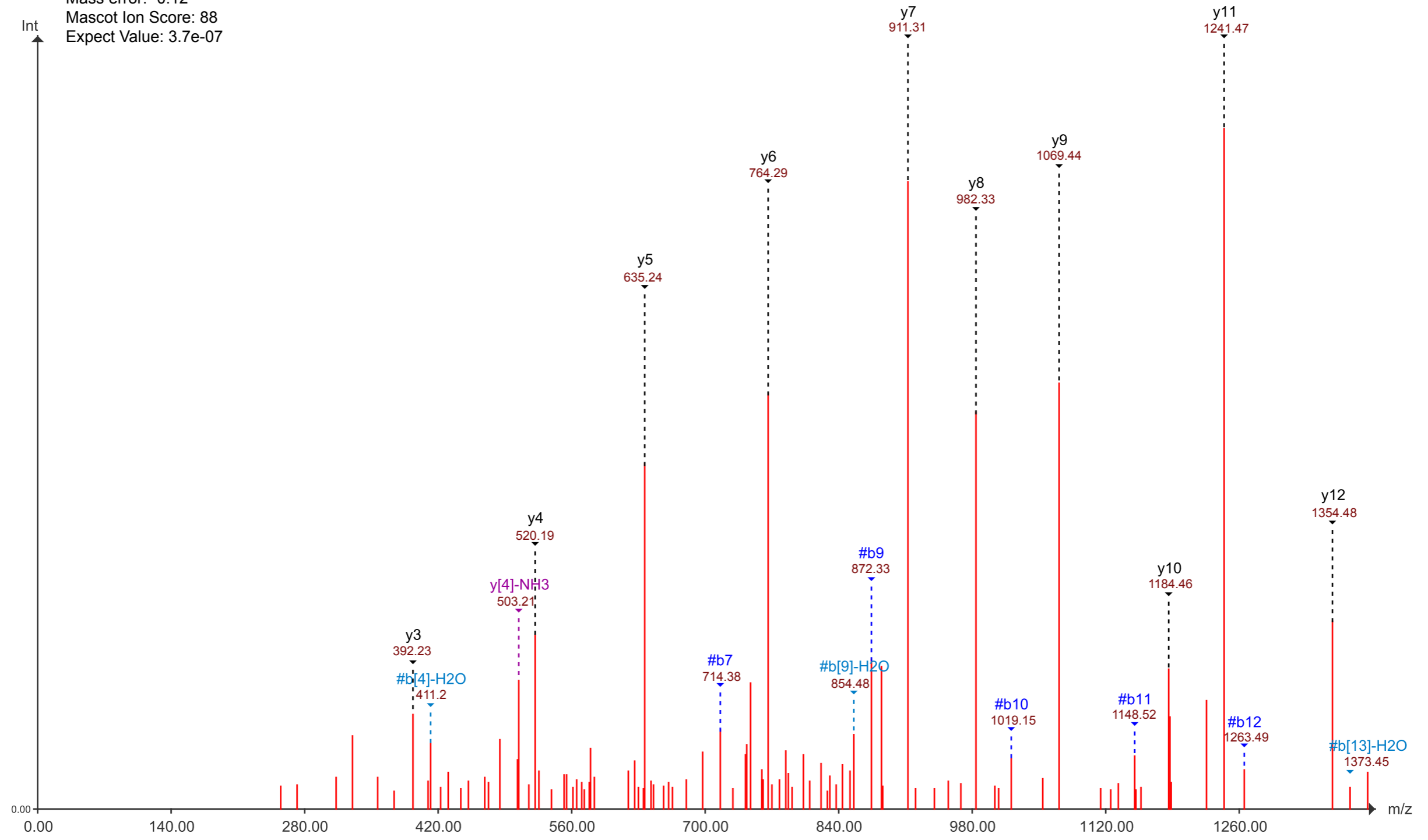
Supplementary Figure 3. An anotated spectrum of Spot 51.
