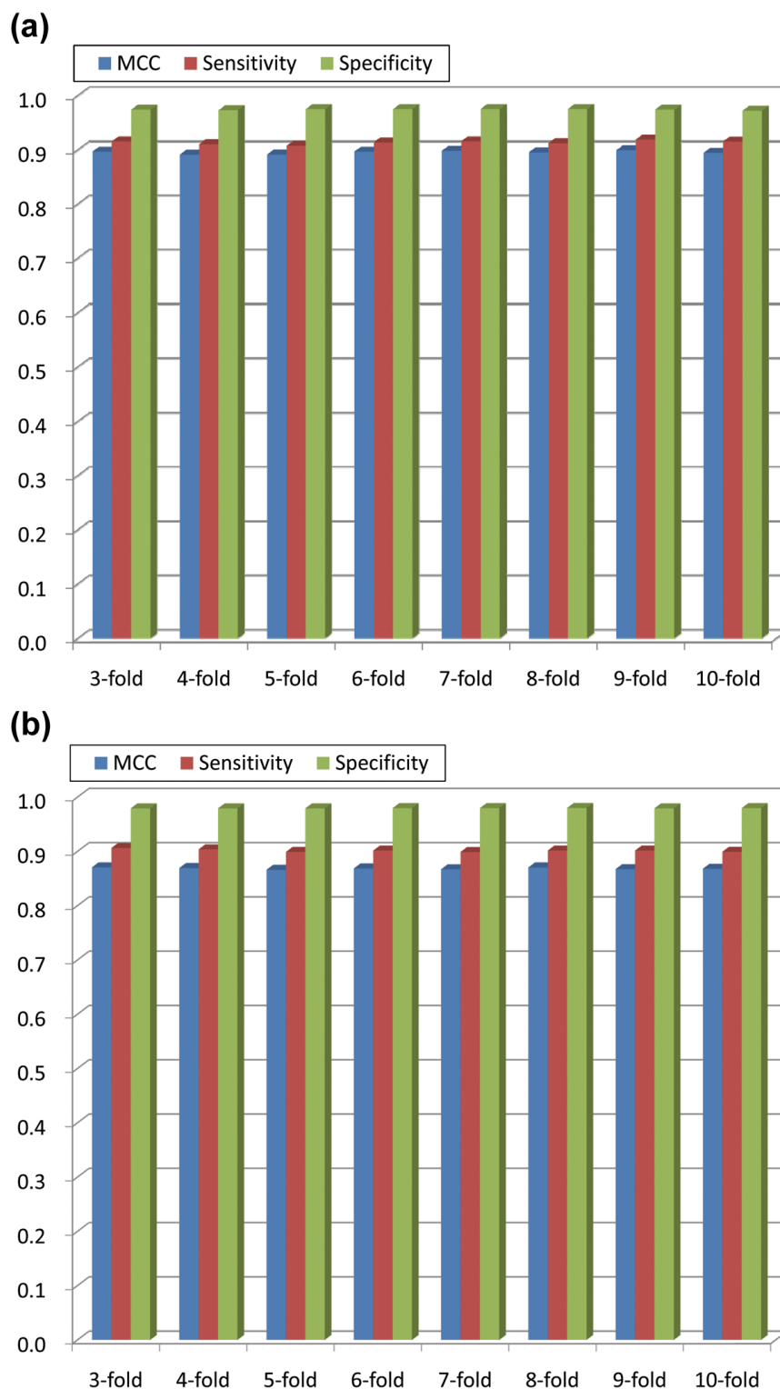
Figure S2. Stability evaluations of the discriminatory model of the proposed method by k -fold cross-validations. The stability of the discriminatory model applied in the proposed DS-scoring scheme was evaluated based on two datasets. (a) Evaluations based on Dataset L. (b) Evaluations based on Dataset M. In both experiments, only the DS-related homologs were treated as the positive data, while common homologs and non-homologs were used as the negative data.
