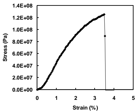
Figure S1. Stress-strain curve for a typical 100-bilayer freestanding PEI/PVDMA film. See text for additional details related to the fabrication and handling of these freestanding films.
