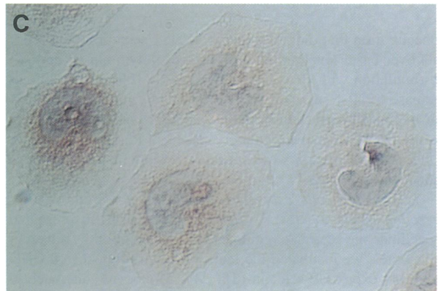
Figure 5. Tethering of monocytes by P-selectin enhances nuclear translocation of NF- \kappa B. (A) Monocytes were allowed to adhere to immobilized P-selectin for 2 h in the absence of an additional stimulus, followed by incubation with an antibody to p65 and staining as described in Methods. Adjustment of the focal plane allowed visualization of blue nuclei with little nuclear staining by the anti-p65 antibody. (B) Monocytes adherent to P-selectin were stimulated with PAF (100 nM), and staining with anti-p65 was done after a 2-h incubation as described above. (C) Plastic wells were coated with anti-ICAM-3 as described in Methods. Monocytes were added, and staining using the anti-p65 antibody was done after a 2-h incubation in the presence of PAF (100 nM). A-C are representative results of four experiments.
