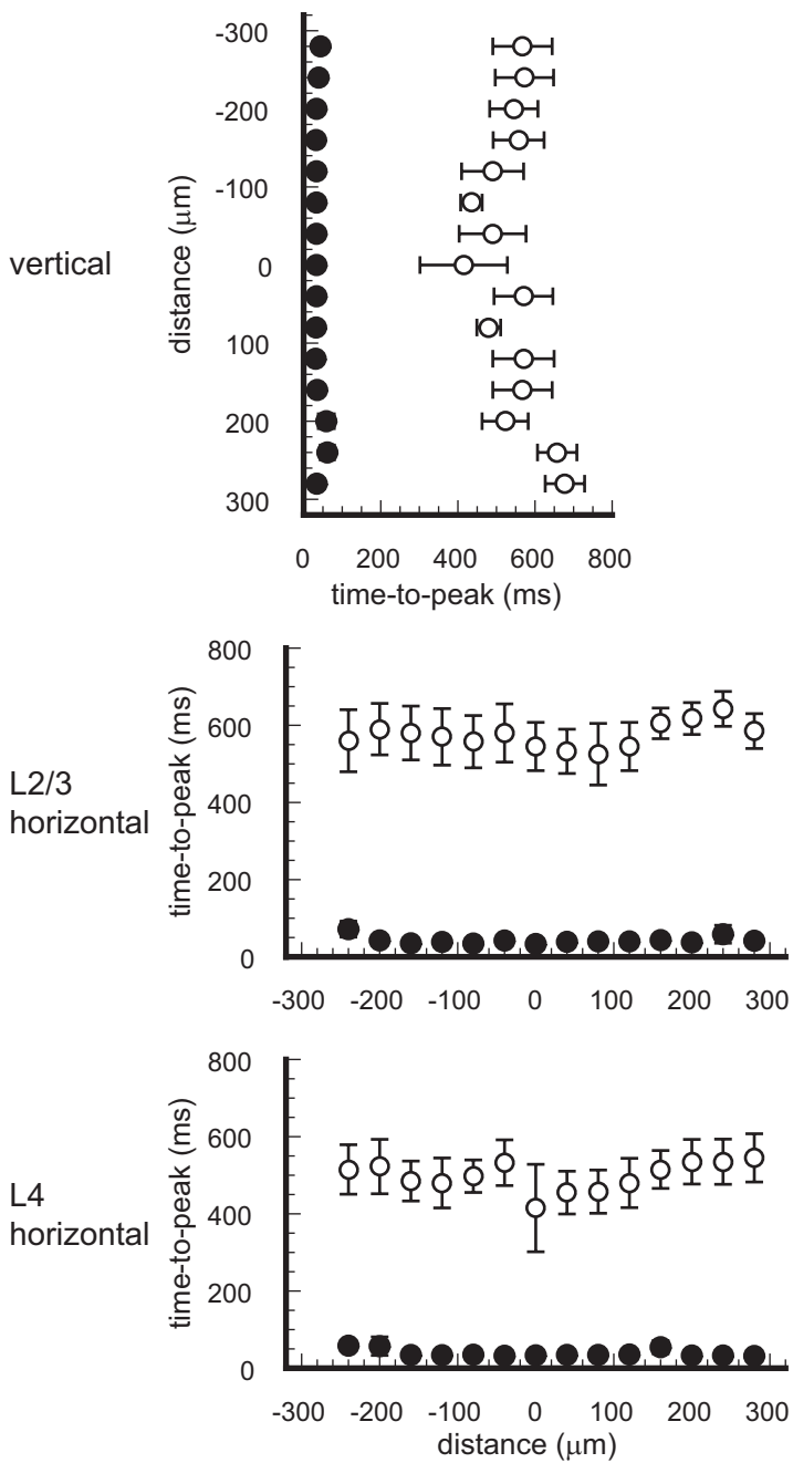
B time-to-peak
