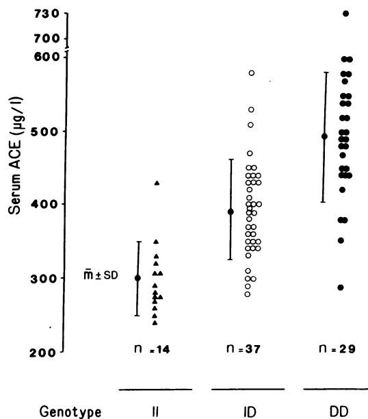
Figure 2. Serum immunoreactive ACE concentrations ( \mu\text{g}/\text{liter} ) for individual with the II, ID, and DD genotypes, respectively, shown in left, middle, and right panels. Solid vertical bars indicate mean concentration and standard deviation for each group.
